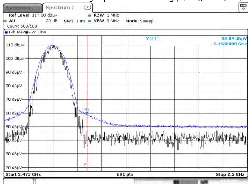
Radiated Restricted Band Edges plot – Peak Reading ( \pi/4 DQPSK, Ch.78, Z-H)
