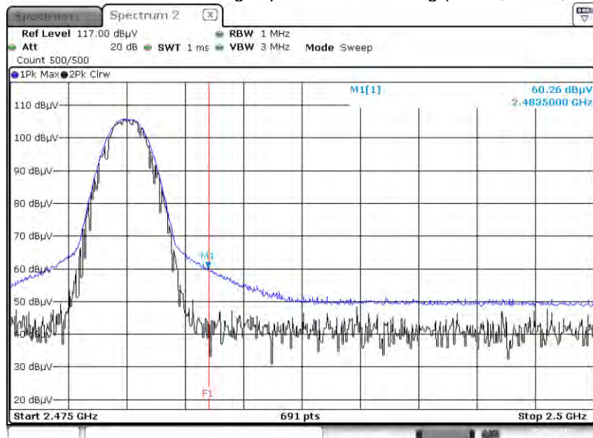
Radiated Restricted Band Edges plot – Peak Reading (GFSK, Ch.78, X-H)
