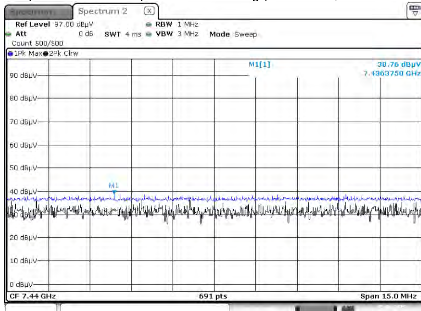
Radiated Spurious Emissions plot – Peak Reading ( \pi/4 DQPSK, Ch.78 3rd Harmonic)
