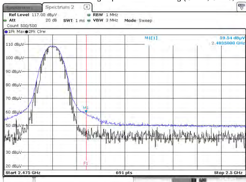
Radiated Restricted Band Edges plot – Peak Reading (GFSK, Ch.78, Z-H)
