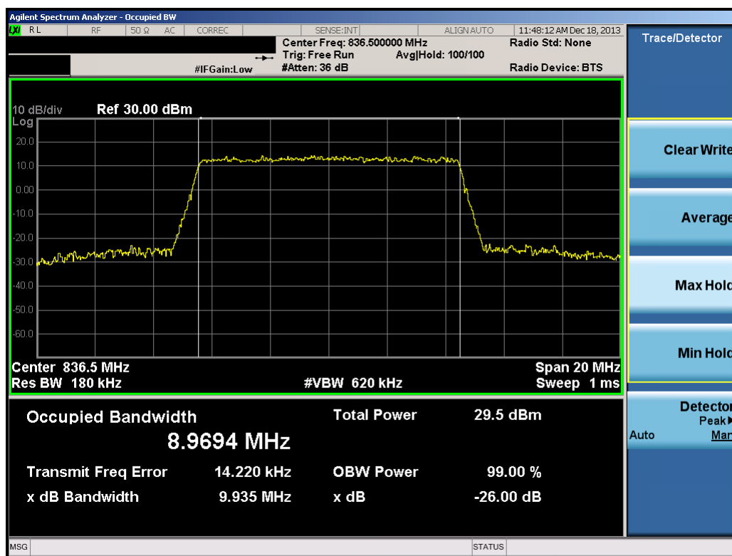
Plot 7-19. Occupied Bandwidth Plot (10.0MHz QPSK – RB Size 50)
