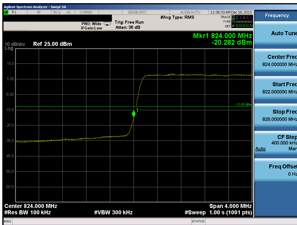
Plot 7-5. Lower Band Edge Plot (3.0MHz QPSK – RB Size 15)
