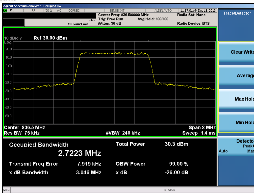
Plot 7-6. Occupied Bandwidth Plot (3.0MHz QPSK – RB Size 15)
