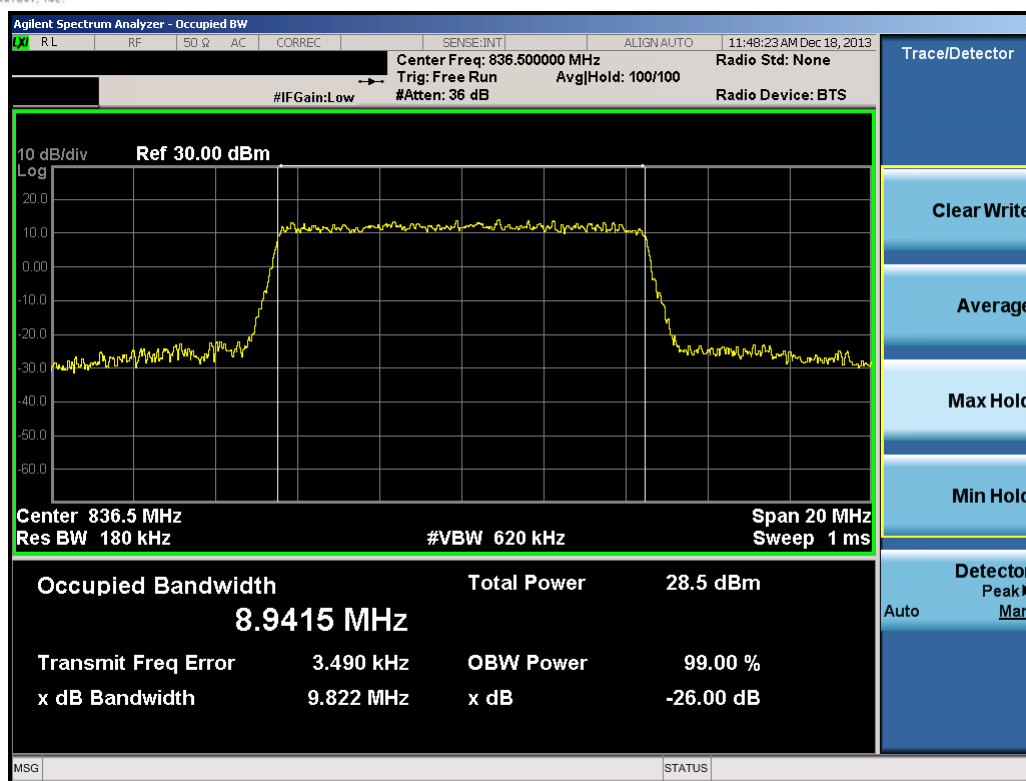
Plot 7-20. Occupied Bandwidth Plot (10.0MHz 16-QAM – RB Size 50)
