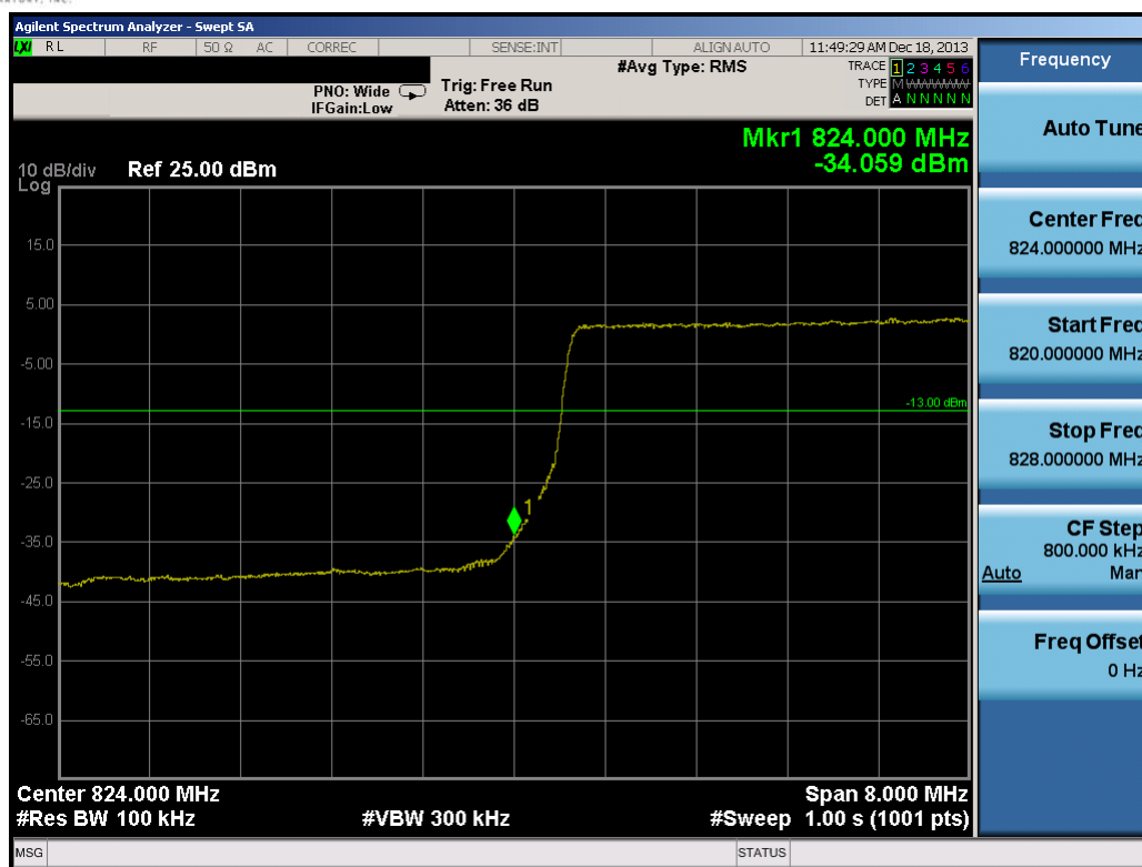
Plot 7-18. Lower Band Edge Plot (10.0MHz QPSK – RB Size 50)
