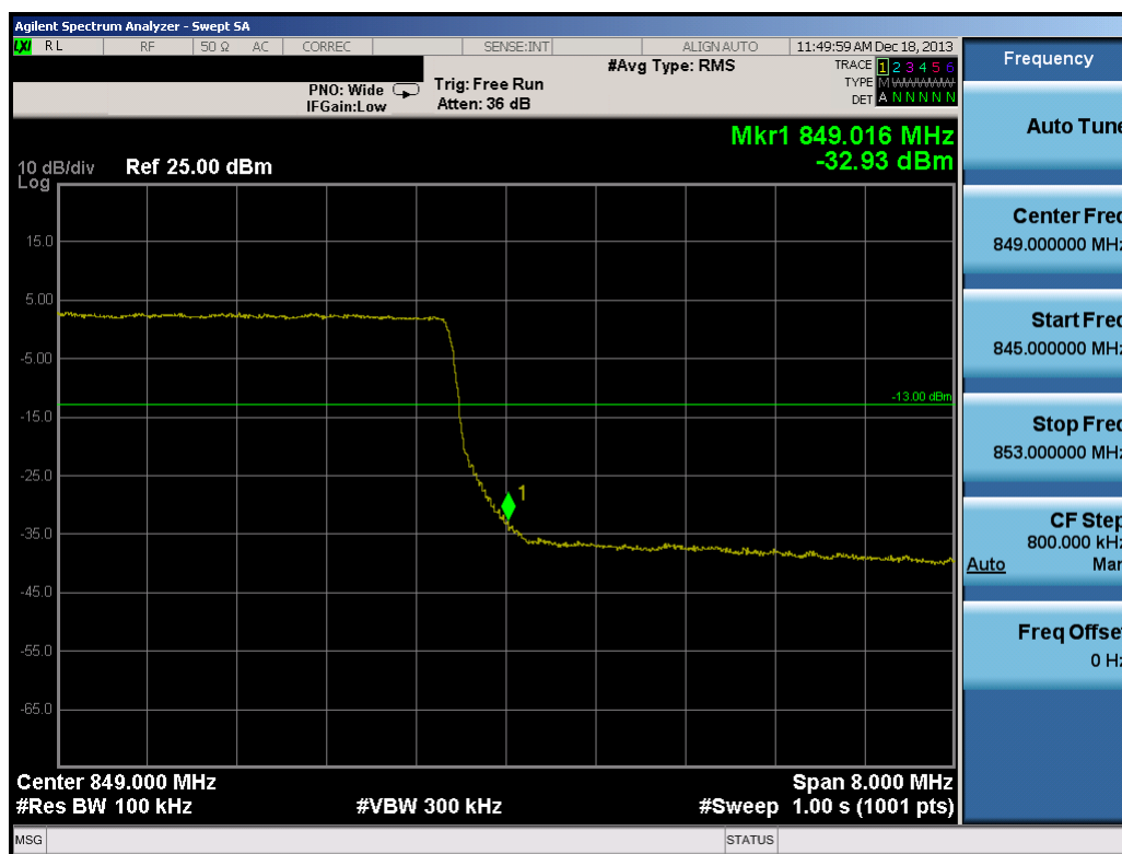
Plot 7-21. Upper Band Edge Plot (10.0MHz QPSK – RB Size 50)
