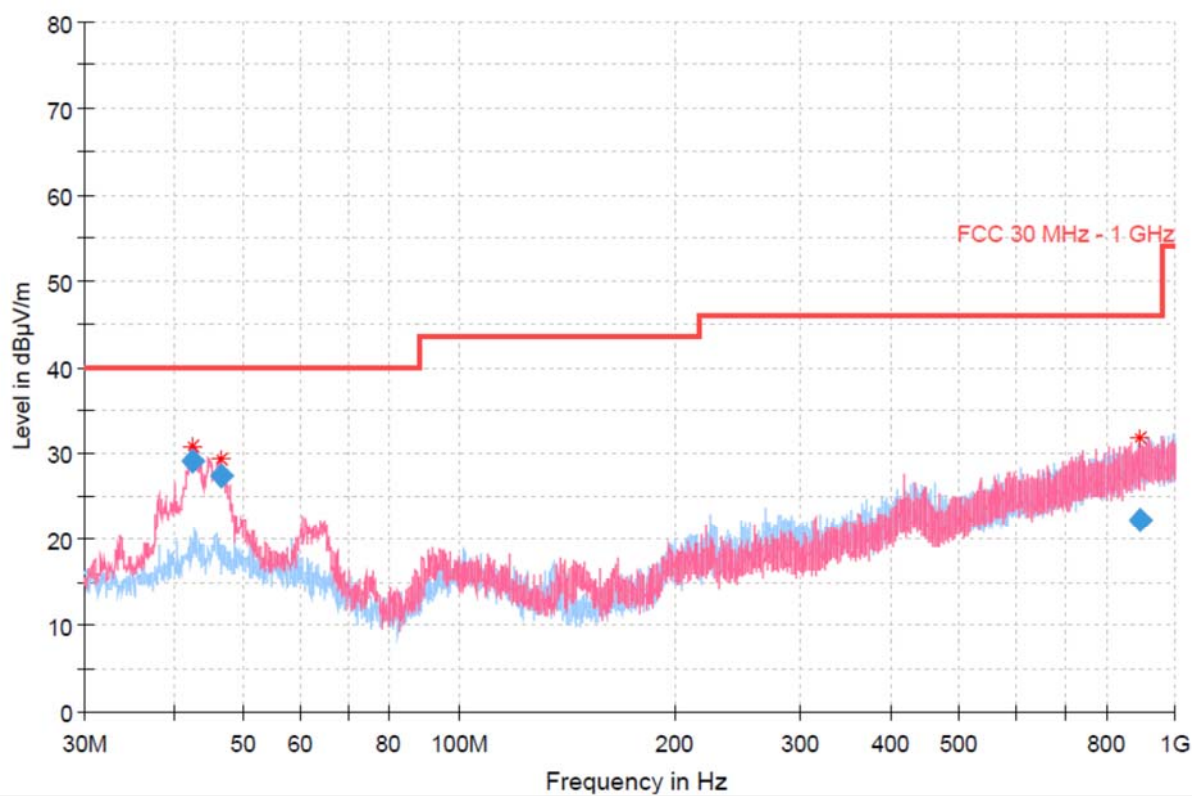
RSE(Below 1 GHz)_MIMO_UNII-2A_802.11ax HE20_5320
