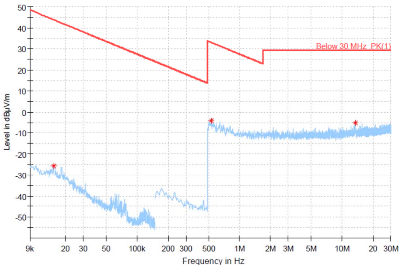
RSE(Below 30 MHz)_MIMO_UNII-2C_802.11ax HE20_5500_X
