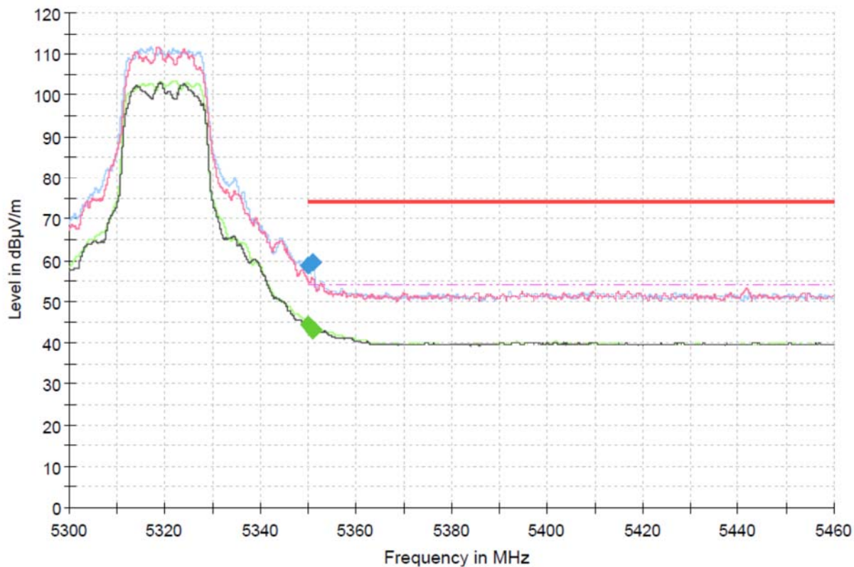
Band Edge_MIMO_UNII-2A_802.11a_5320
