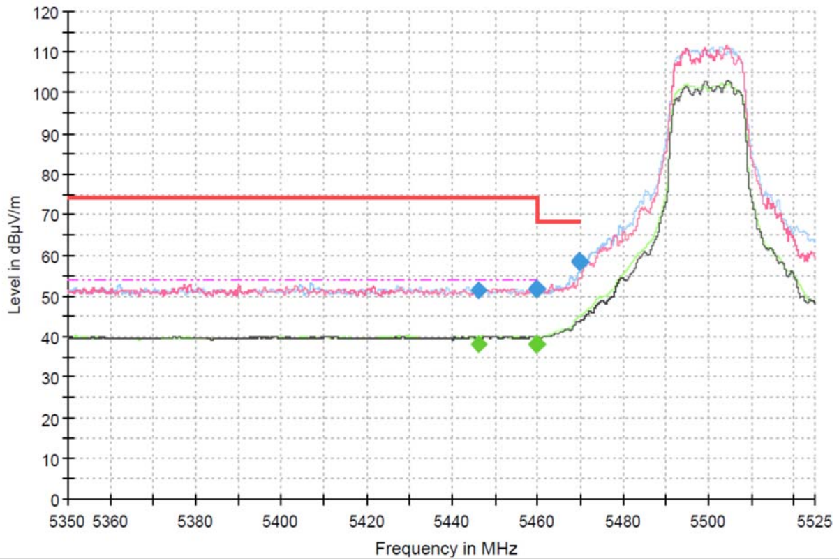
Band Edge_MIMO_UNII-2C_802.11a_5500
