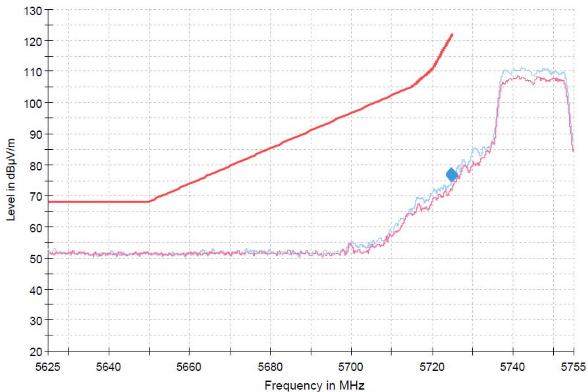
Band Edge_MIMO_UNII-3_802.11a_5745
