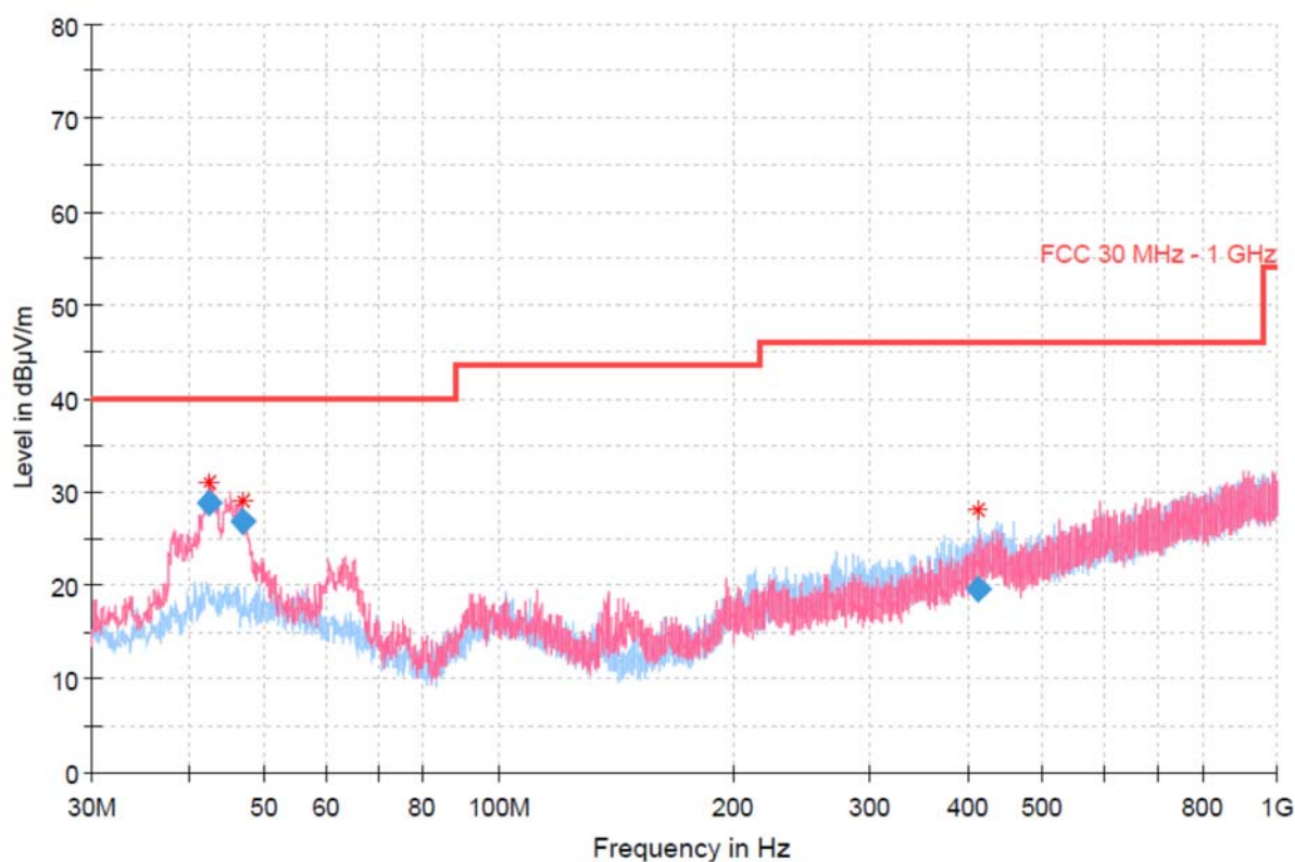
RSE_MIMO_UNII-2A_802.11a_5320
