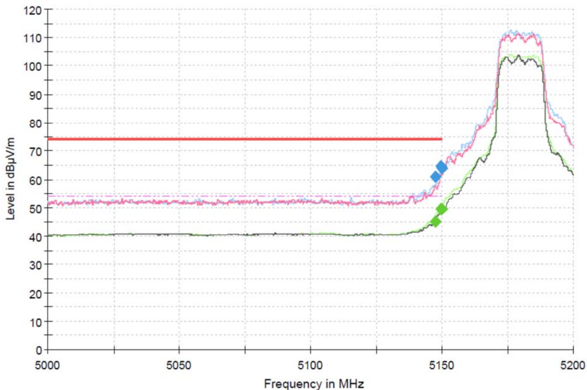
Band Edge_MIMO_UNII-1_802.11a_5180
