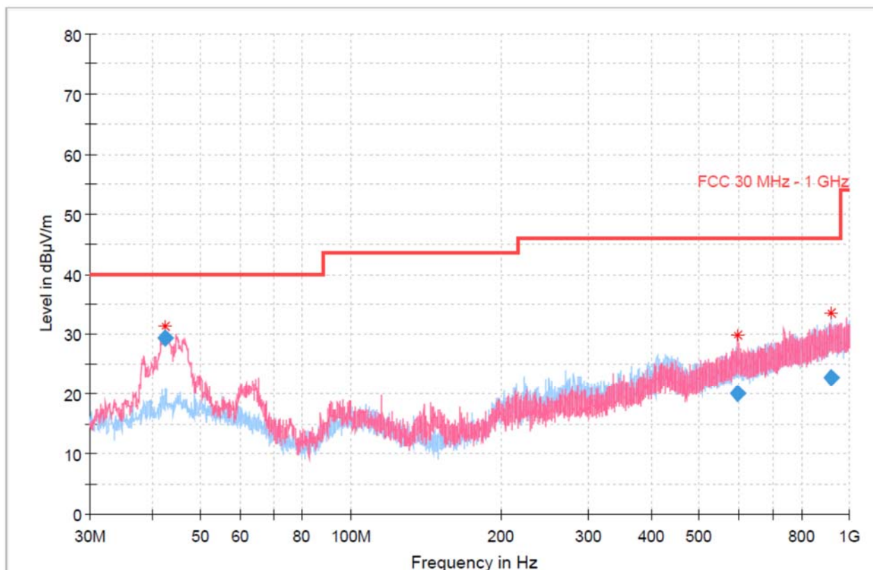
RSE_MIMO_UNII-1_802.11a_5180
