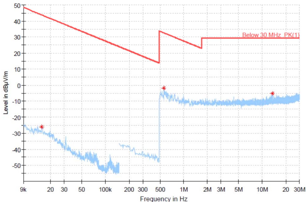
RSE_MIMO_UNII-2C_802.11a_5500_Z
