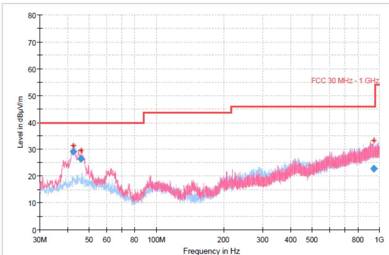
RSE_MIMO_UNII-2C_802.11a_5500
