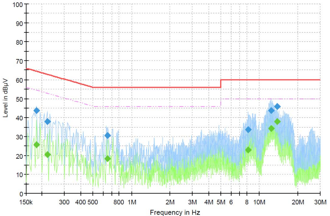
SISO_ANT1_UNII-1_802.11a_5180
