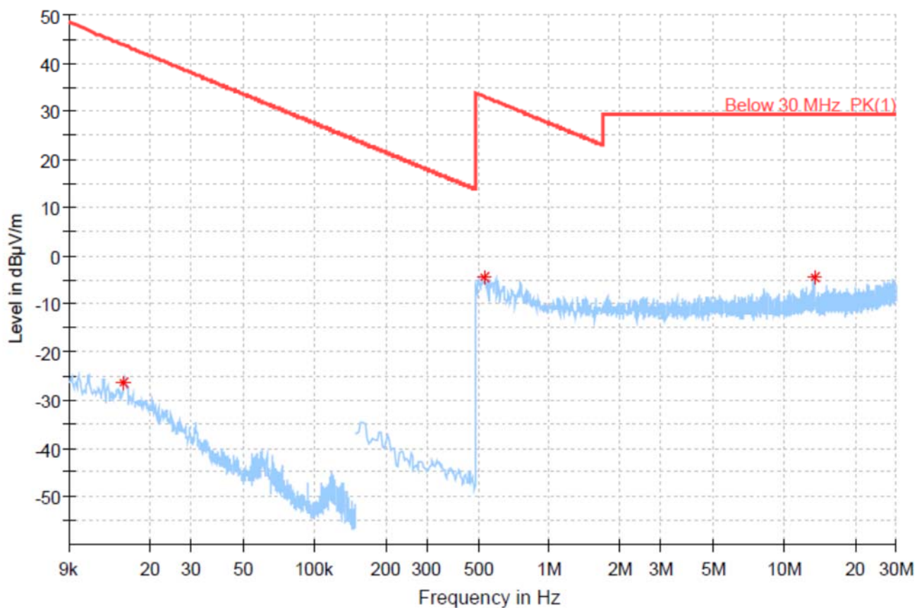
RSE_MIMO_UNII-2A_802.11a_5320_Y
