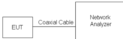
Figure 9-3 Power Measurement Setup
