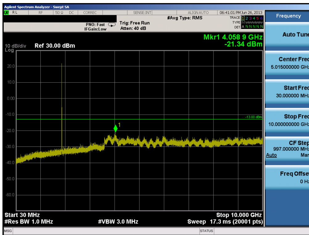
Plot 6-37. Conducted Spurious Plot (PCS WCDMA Mode – Ch. 9400)
