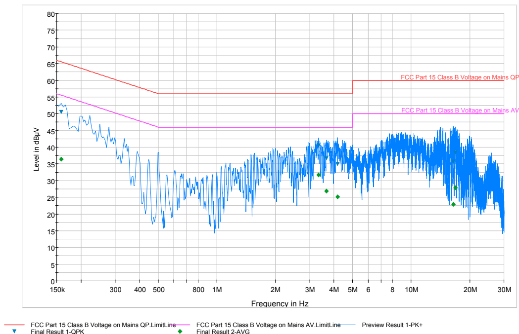
Plot 6-35. Line Conducted Plot with 802.11b (L1)
