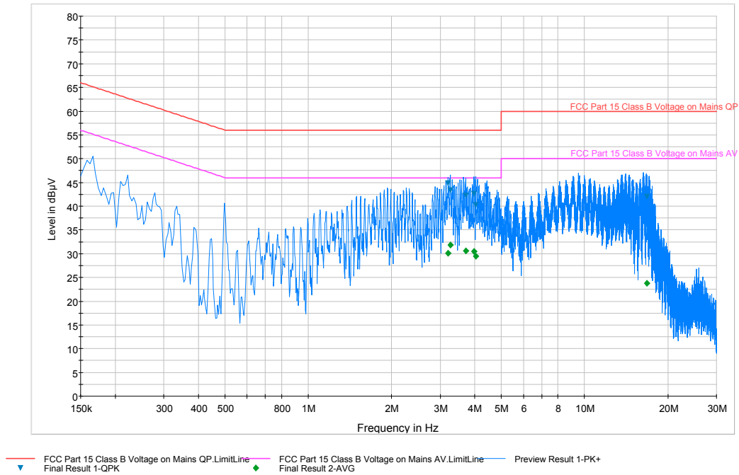
Plot 6-36. Line Conducted Plot with 802.11b (N)
