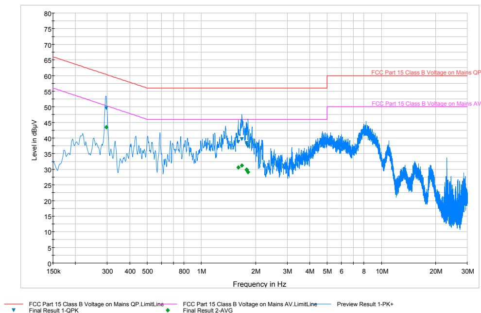
Plot 6-45. Line-Conducted Test Plot (N)
