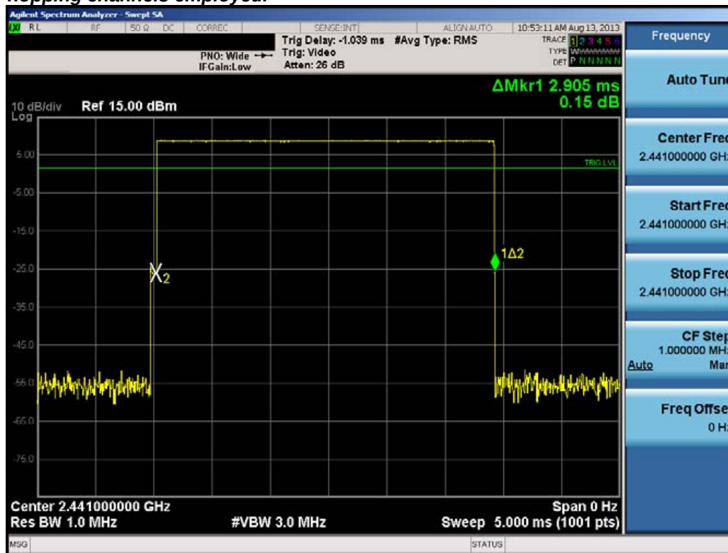
Plot 6-33. Time of Occupancy Plot (Bluetooth)
