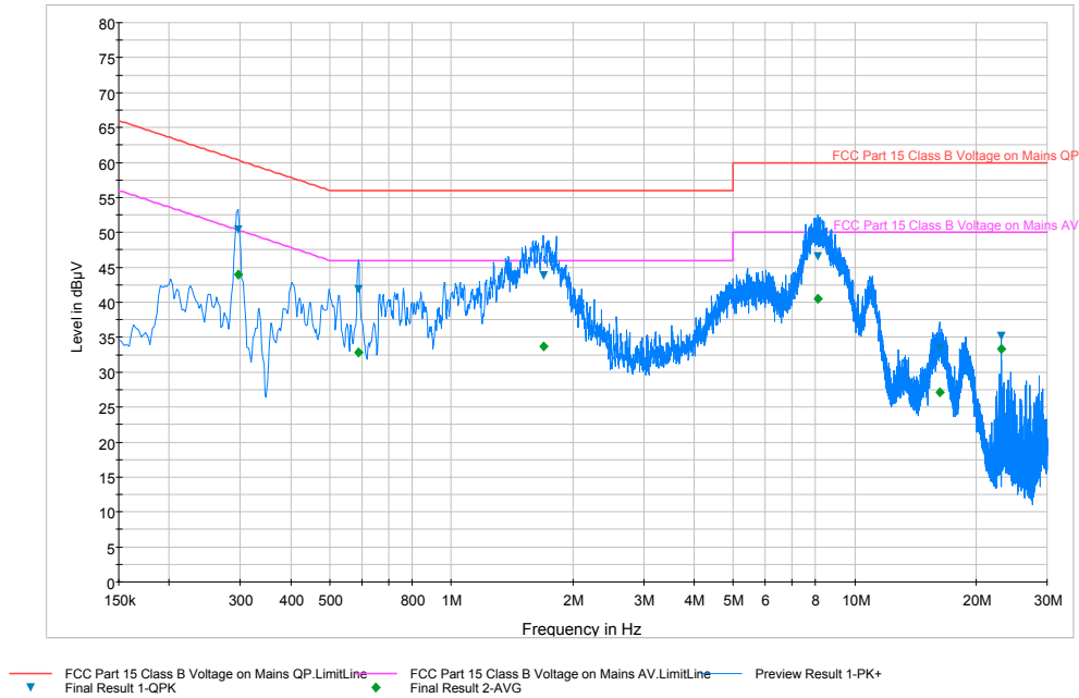
Plot 6-44. Line-Conducted Test Plot (L1)
