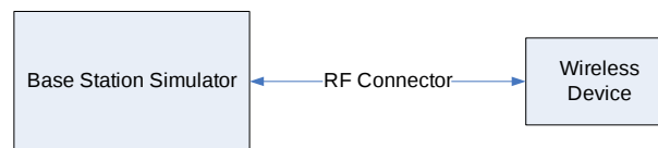
Figure 8-3 Power Measurement Setup – NR Online
