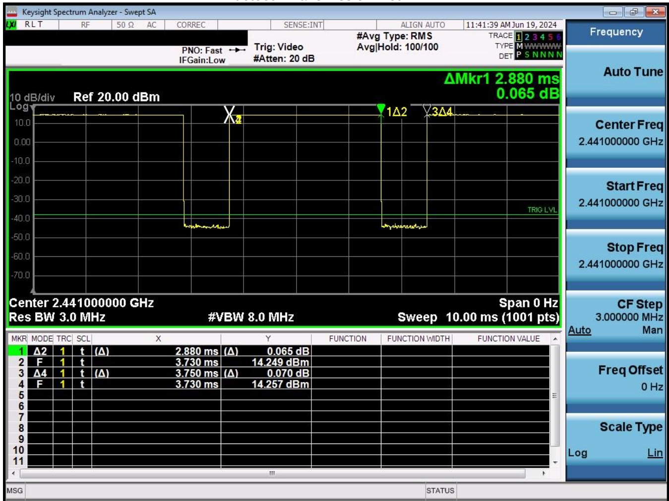
Figure 7-3 Bluetooth Transmission Plot – WIFI1
