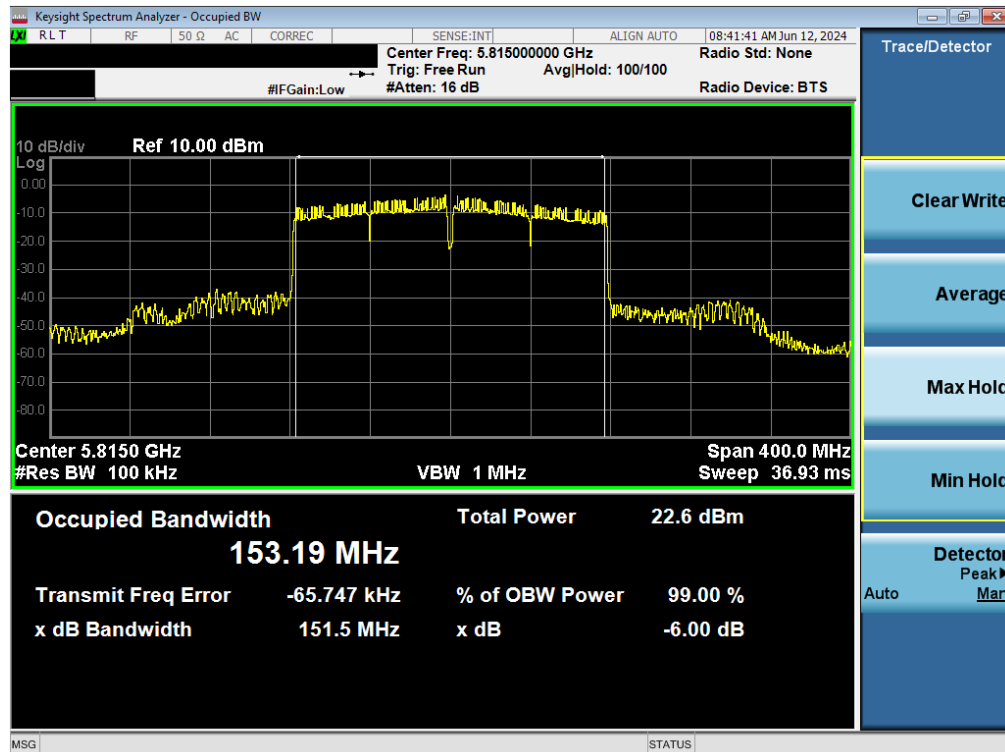
Plot 7-66. 6dB Bandwidth Plot MIMO ANT1 (160MHz BW 802.11ac (UNII Band 3/4) – Ch. 163)
