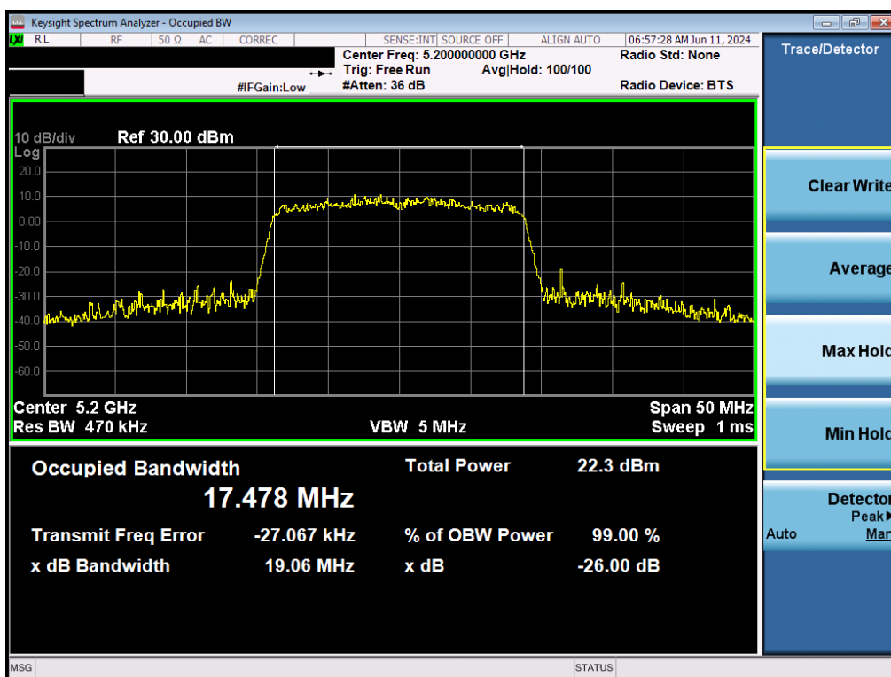
Plot 7-28. 26dB Bandwidth Plot MIMO ANT2 (20MHz BW 802.11n (UNII Band 1) – Ch. 40)
