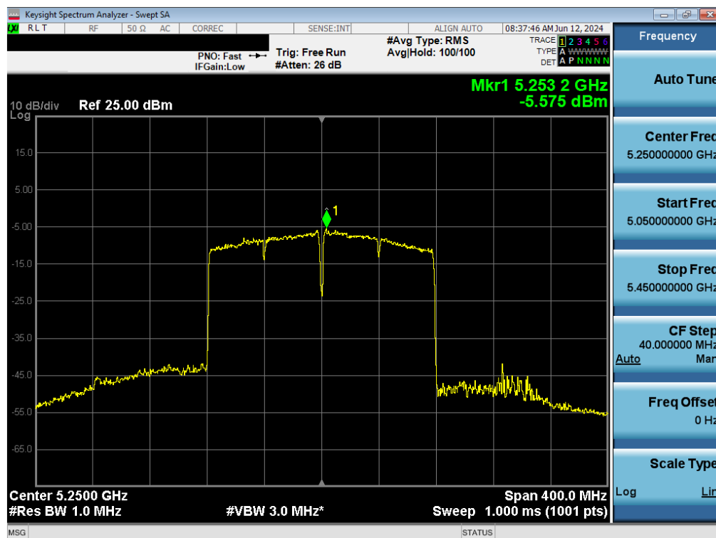
Plot 7-91. Power Spectral Density Plot MIMO ANT1 (160MHz BW 802.11ac (UNII Band 1/2A) – Ch. 50)
