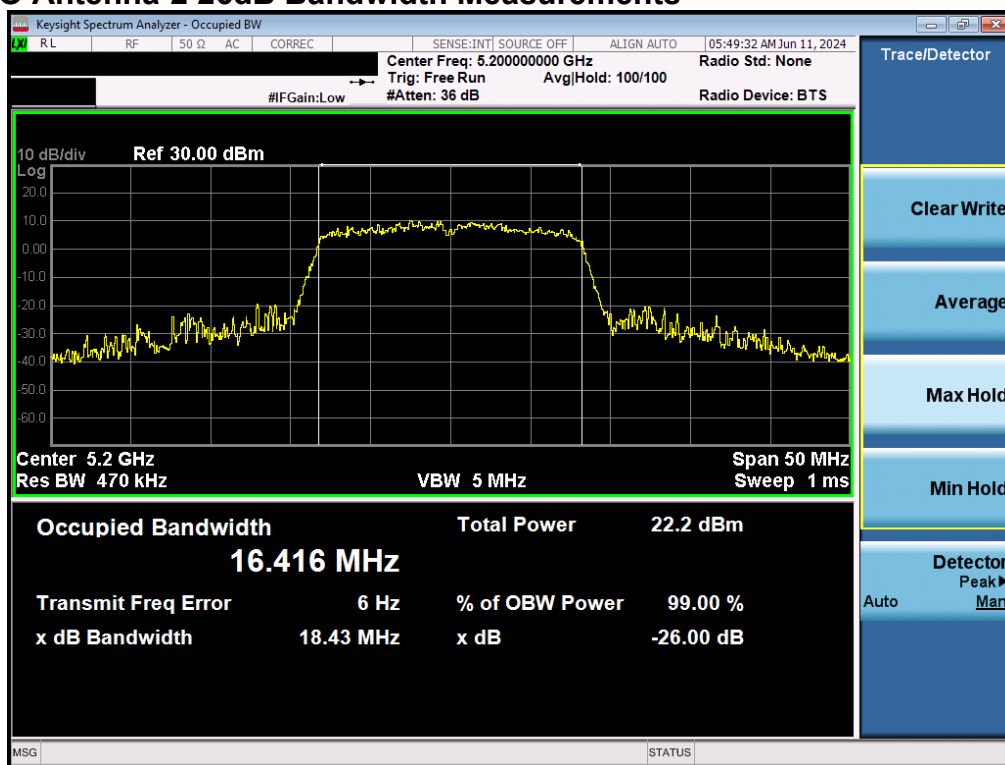
Plot 7-27. 26dB Bandwidth Plot MIMO ANT2 (802.11a (UNII Band 1) – Ch. 40)
