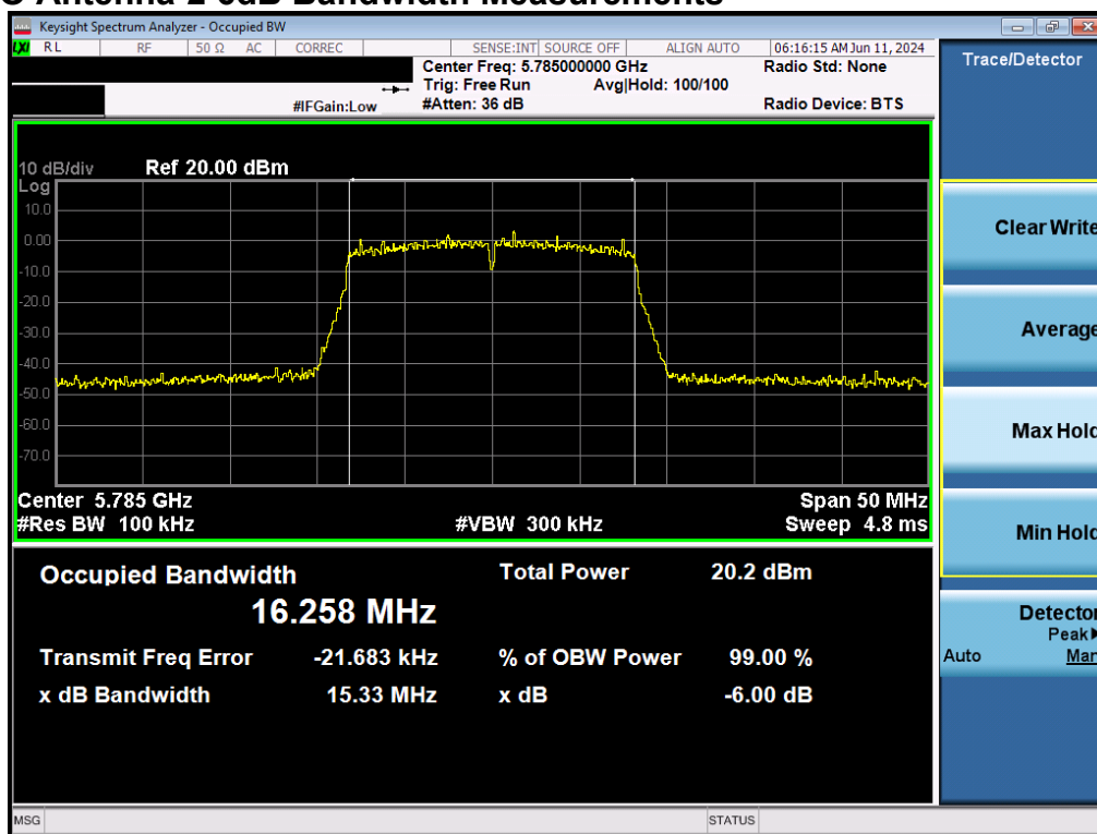
Plot 7-68. 6dB Bandwidth Plot MIMO ANT2 (802.11a (UNII Band 3) – Ch. 157)
