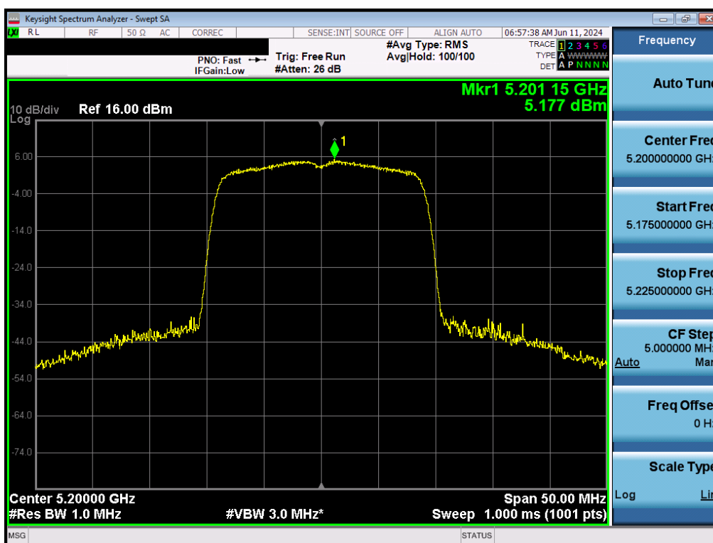
Plot 7-126. Power Spectral Density Plot MIMO ANT2 (20MHz BW 802.11n (UNII Band 1) – Ch. 40)
