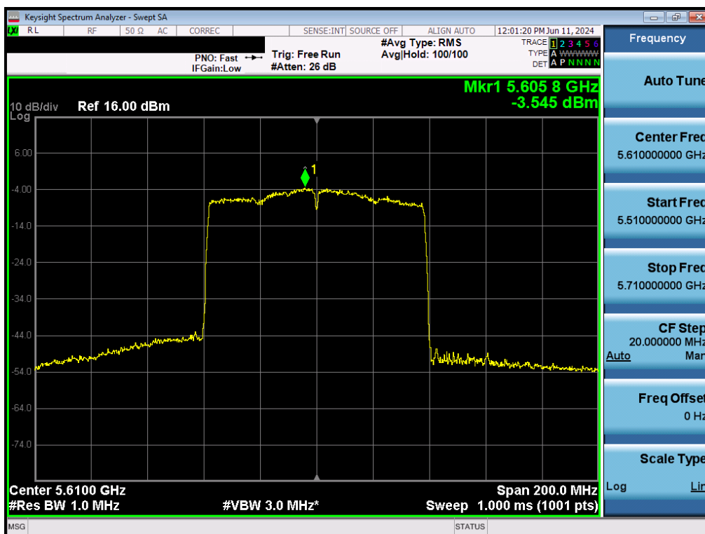
Plot 7-146. Power Spectral Density Plot MIMO ANT2 (80MHz BW 802.11ac (UNII Band 2C) – Ch. 122)
