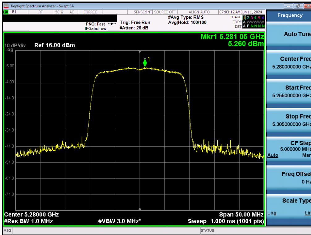
Plot 7-135. Power Spectral Density Plot MIMO ANT2 (20MHz BW 802.11n (UNII Band 2A) – Ch. 56)
