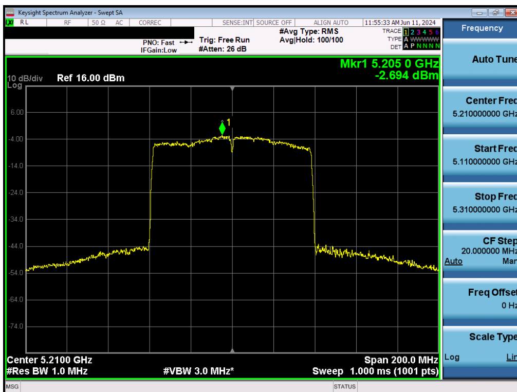
Plot 7-130. Power Spectral Density Plot MIMO ANT2 (80MHz BW 802.11ac (UNII Band 1) – Ch. 42)
