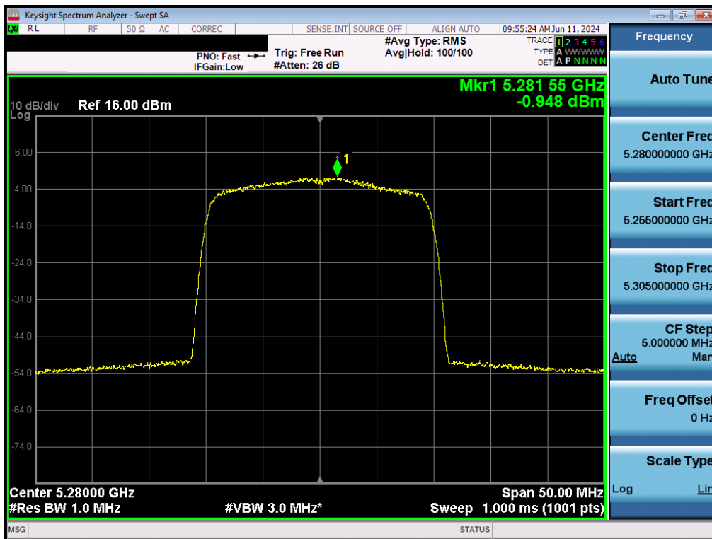
Plot 7-136. Power Spectral Density Plot MIMO ANT2 (20MHz BW 802.11ax (UNII Band 2A) – Ch. 56)
