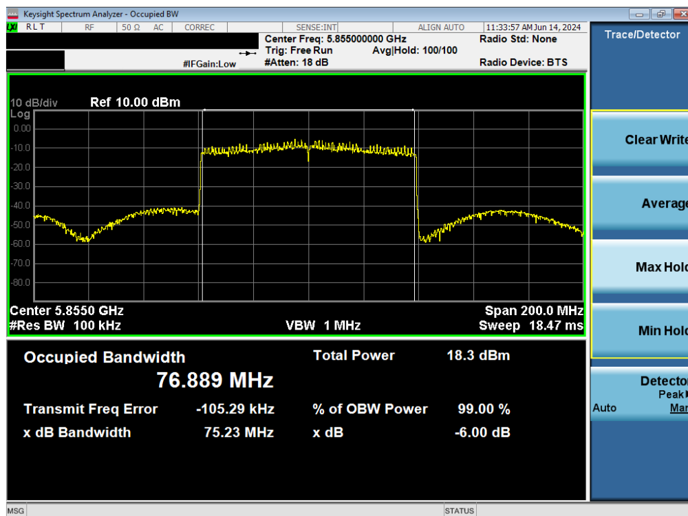
Plot 7-58. 6dB Bandwidth Plot MIMO ANT1 (80MHz BW 802.11ax – 996 Tones (UNII Band 3/4) – Ch. 171)
