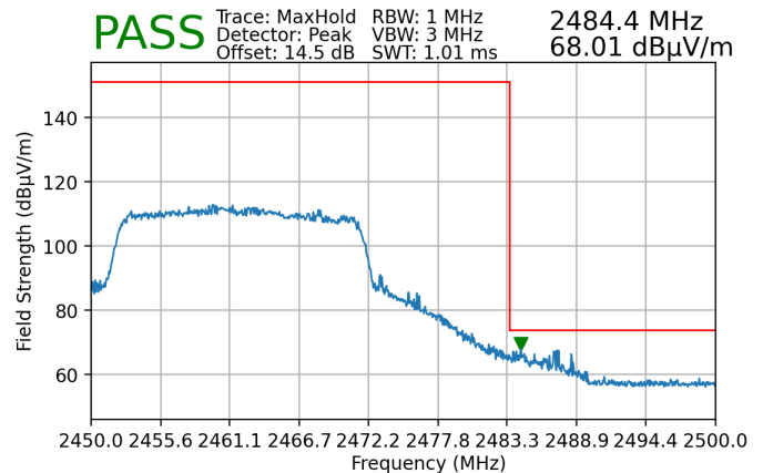
Plot 7-203. Radiated Restricted Upper Band Edge Measurement SISO ANT1 (Peak)
