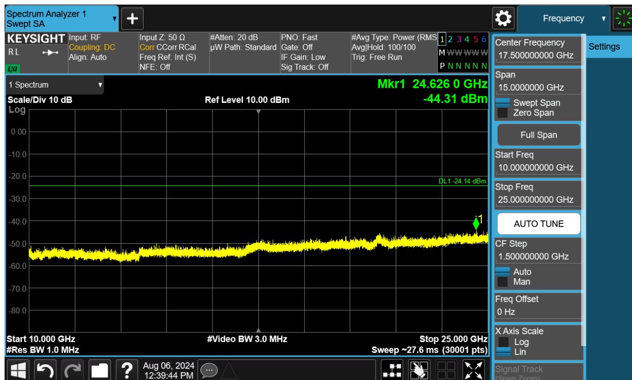
Plot 7-178. Conducted Spurious Plot MIMO ANT1 (802.11b – Ch. 11)
