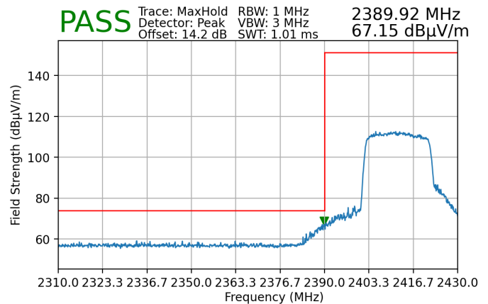
Plot 7-217. Radiated Restricted Lower Band Edge Measurement MIMO (Peak)
