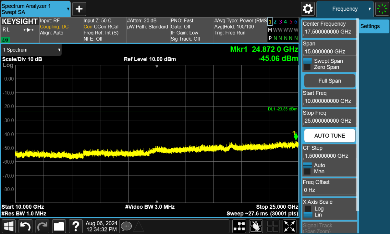
Plot 7-180. Conducted Spurious Plot MIMO ANT2 (802.11b - Ch. 1)
