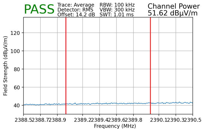
Plot 7-216. Radiated Restricted Lower Band Edge Measurement MIMO (Average)
