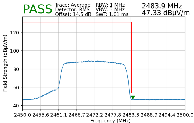
Plot 7-214. Radiated Restricted Upper Band Edge Measurement SISO ANT2 (Average)
