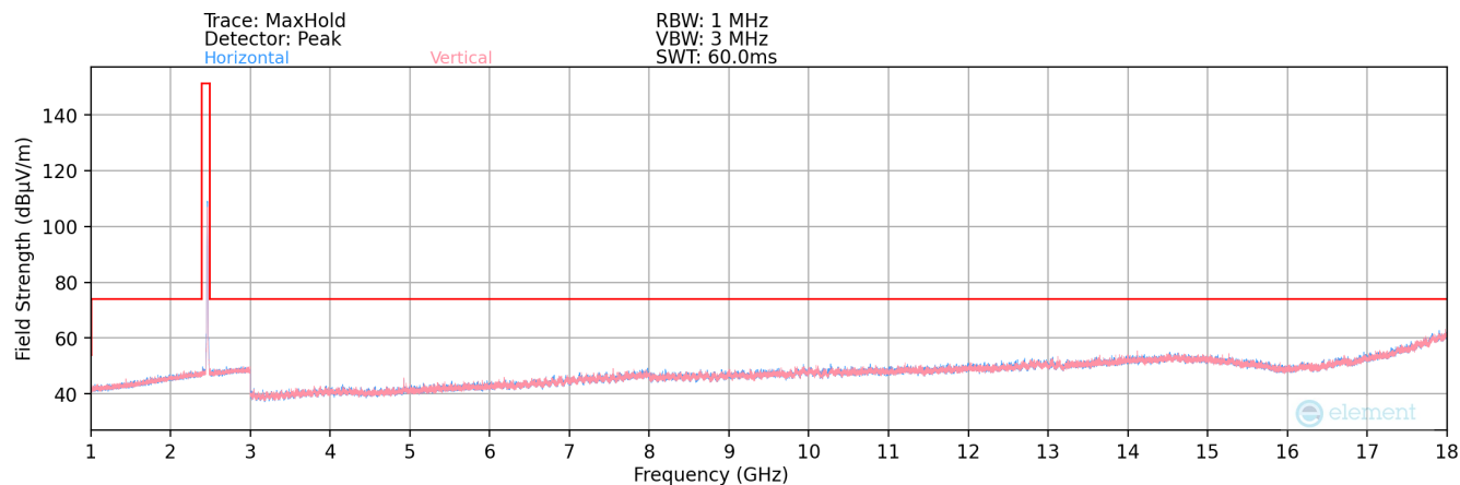
Plot 7-198. Radiated Spurious Plot above 1GHz MIMO (802.11b – Ch. 11)
