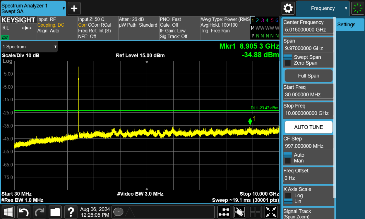
Plot 7-181. Conducted Spurious Plot MIMO ANT2 (802.11b – Ch. 6)
