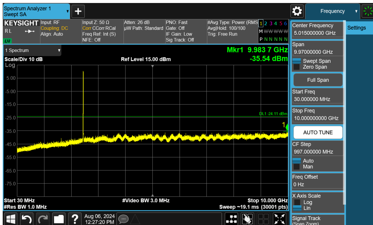
Plot 7-183. Conducted Spurious Plot MIMO ANT2 (802.11b – Ch. 11)
