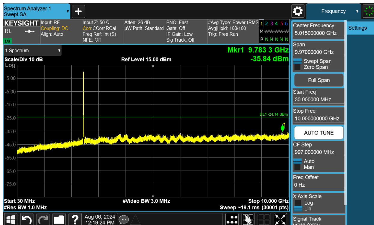
Plot 7-177. Conducted Spurious Plot MIMO ANT1 (802.11b – Ch. 11)
