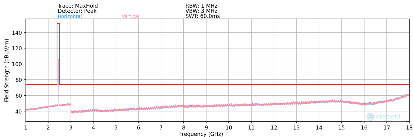
Plot 7-188. Radiated Spurious Plot above 1GHz SISO ANT1 (802.11b – Ch. 11)
