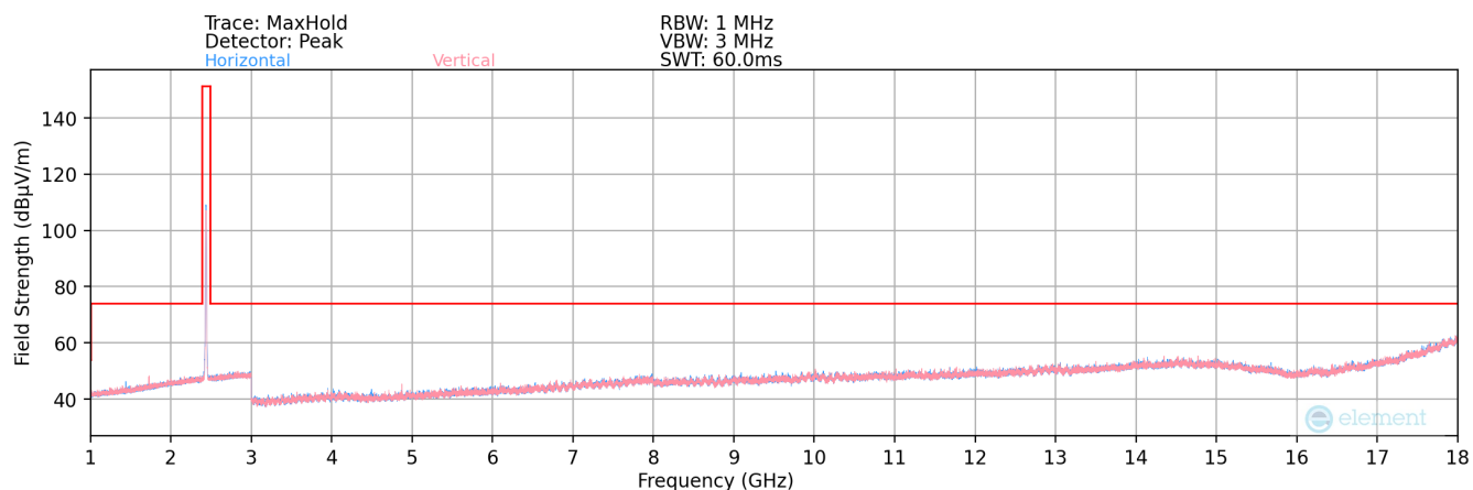
Plot 7-197. Radiated Spurious Plot above 1GHz MIMO (802.11b – Ch. 6)
