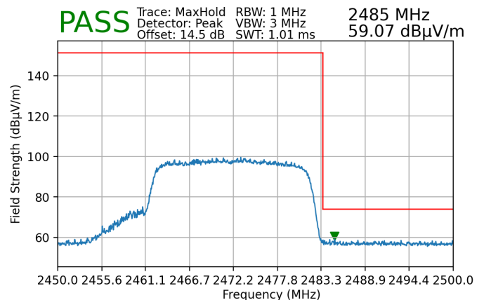
Plot 7-215. Radiated Restricted Upper Band Edge Measurement SISO ANT2 (Peak)
