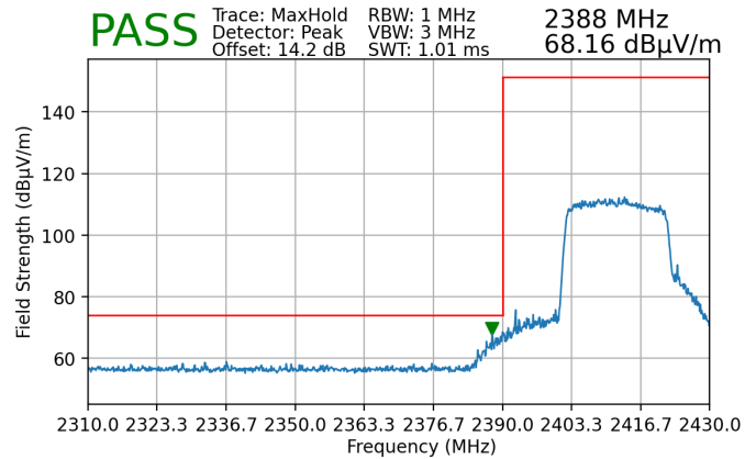
Plot 7-201. Radiated Restricted Lower Band Edge Measurement SISO ANT1 (Peak)
