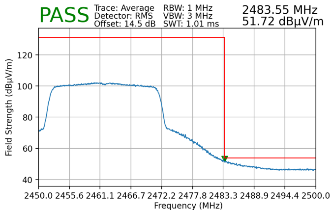
Plot 7-218. Radiated Restricted Upper Band Edge Measurement MIMO (Average)
