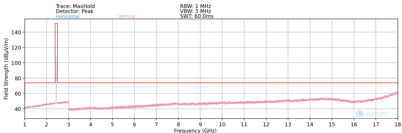
Plot 7-187. Radiated Spurious Plot above 1GHz SISO ANT1 (802.11b – Ch. 6)
