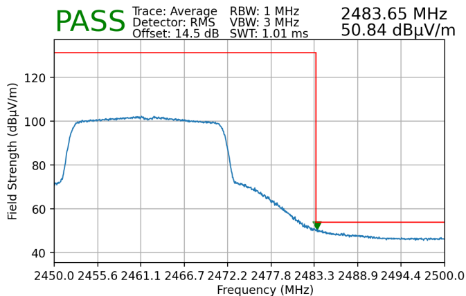
Plot 7-210. Radiated Restricted Upper Band Edge Measurement SISO ANT2 (Average)
