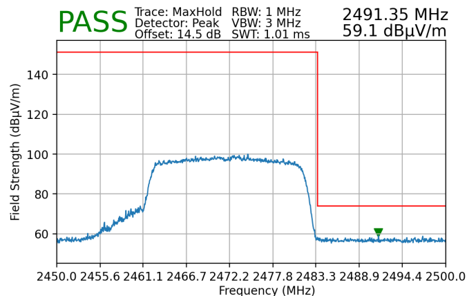
Plot 7-223. Radiated Restricted Upper Band Edge Measurement MIMO (Peak)
