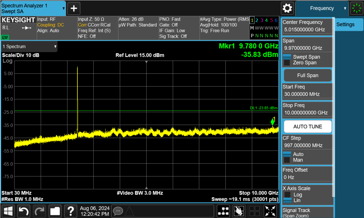
Plot 7-179. Conducted Spurious Plot MIMO ANT2 (802.11b - Ch. 1)
