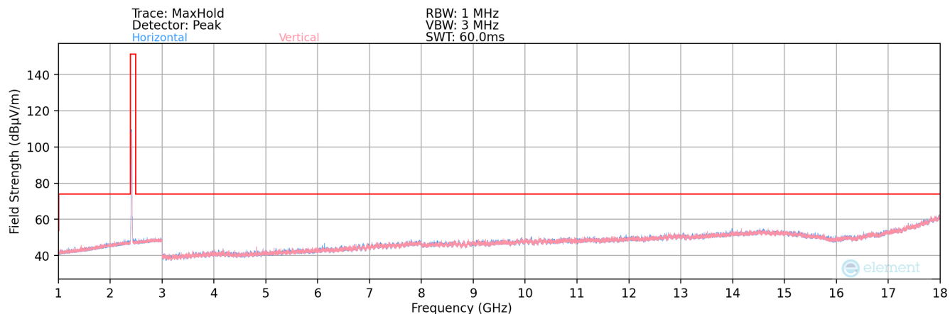
Plot 7-196. Radiated Spurious Plot above 1GHz MIMO (802.11b – Ch. 1)
