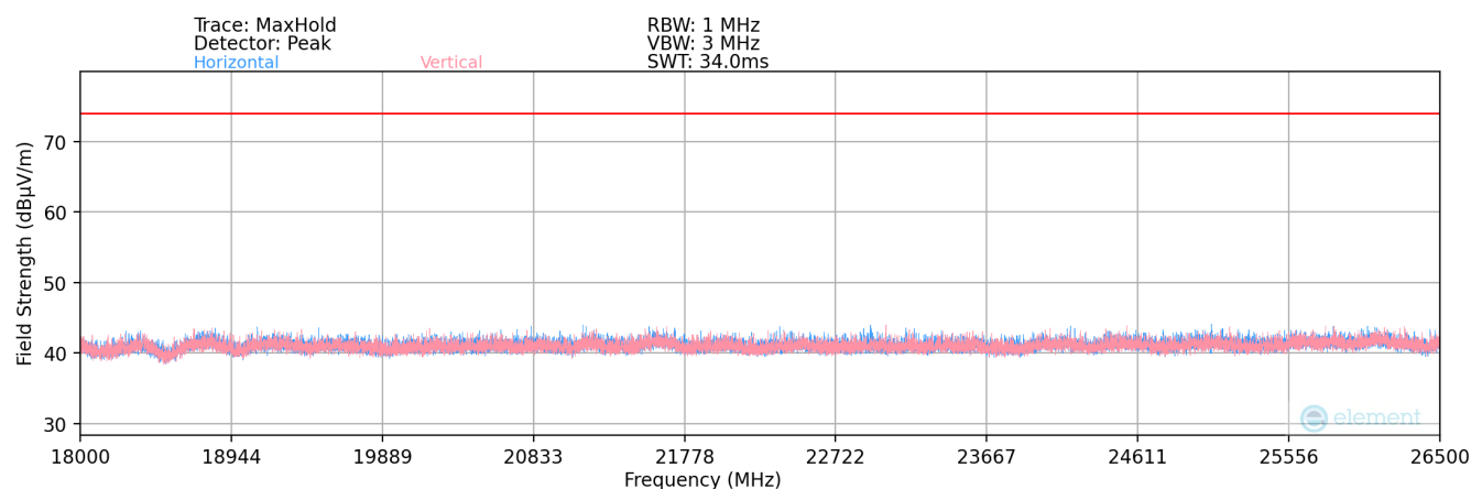
Plot 7-189. Radiated Spurious Plot above 18GHz SISO ANT1
