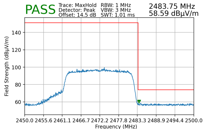
Plot 7-207. Radiated Restricted Upper Band Edge Measurement SISO ANT1 (Peak)
