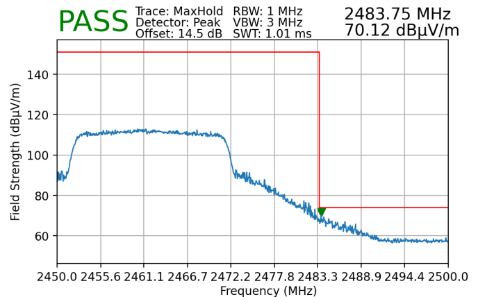
Plot 7-219. Radiated Restricted Upper Band Edge Measurement MIMO (Peak)
