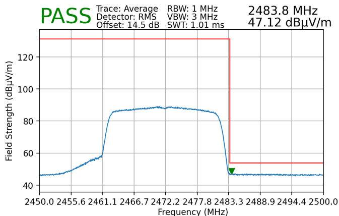
Plot 7-222. Radiated Restricted Upper Band Edge Measurement MIMO (Average)
