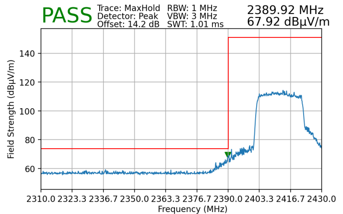
Plot 7-209. Radiated Restricted Lower Band Edge Measurement SISO ANT2 (Peak)
