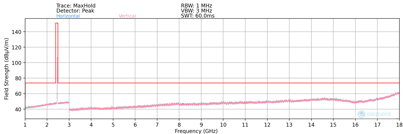
Plot 7-193. Radiated Spurious Plot above 1GHz SISO ANT2 (802.11b – Ch. 11)
