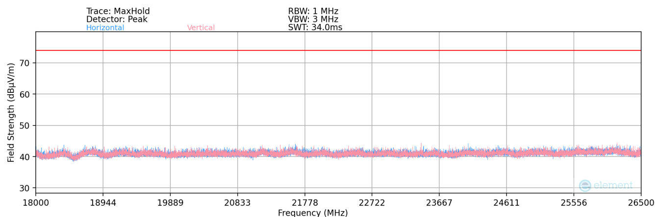
Plot 7-194. Radiated Spurious Plot above 18GHz SISO ANT2
