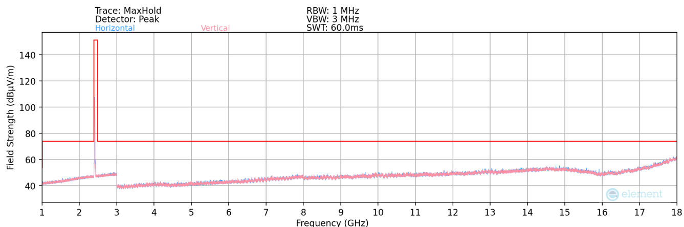
Plot 7-186. Radiated Spurious Plot above 1GHz SISO ANT1 (802.11b – Ch. 1)
