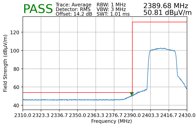
Plot 7-208. Radiated Restricted Lower Band Edge Measurement SISO ANT2 (Average)
