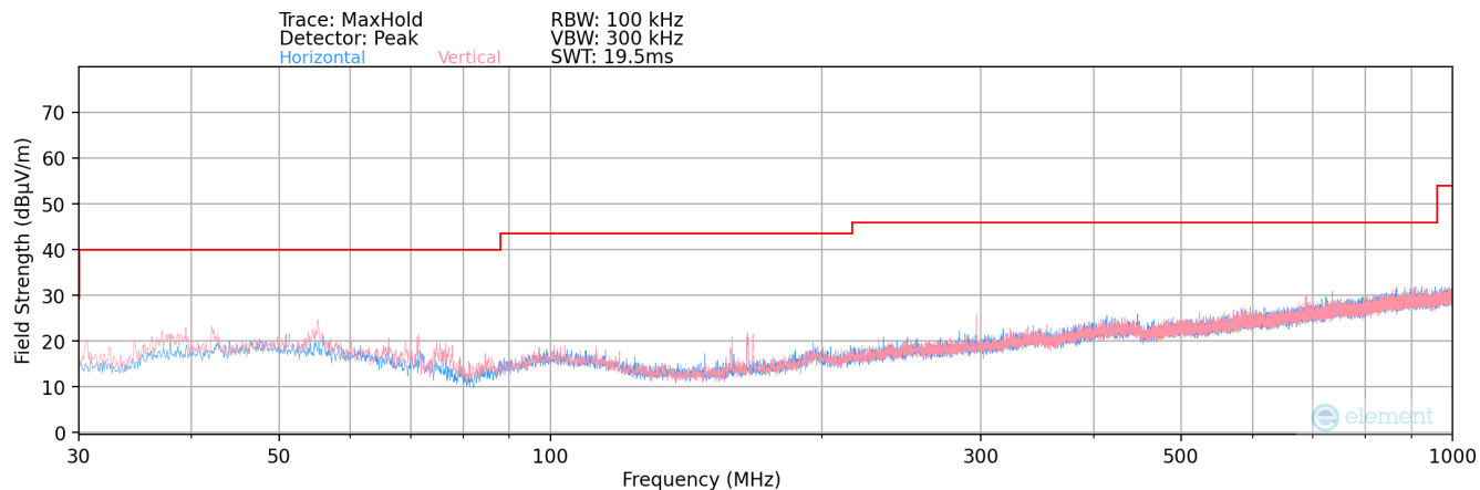
Plot 7-185. Radiated Spurious Plot below 1GHz SISO ANT1
