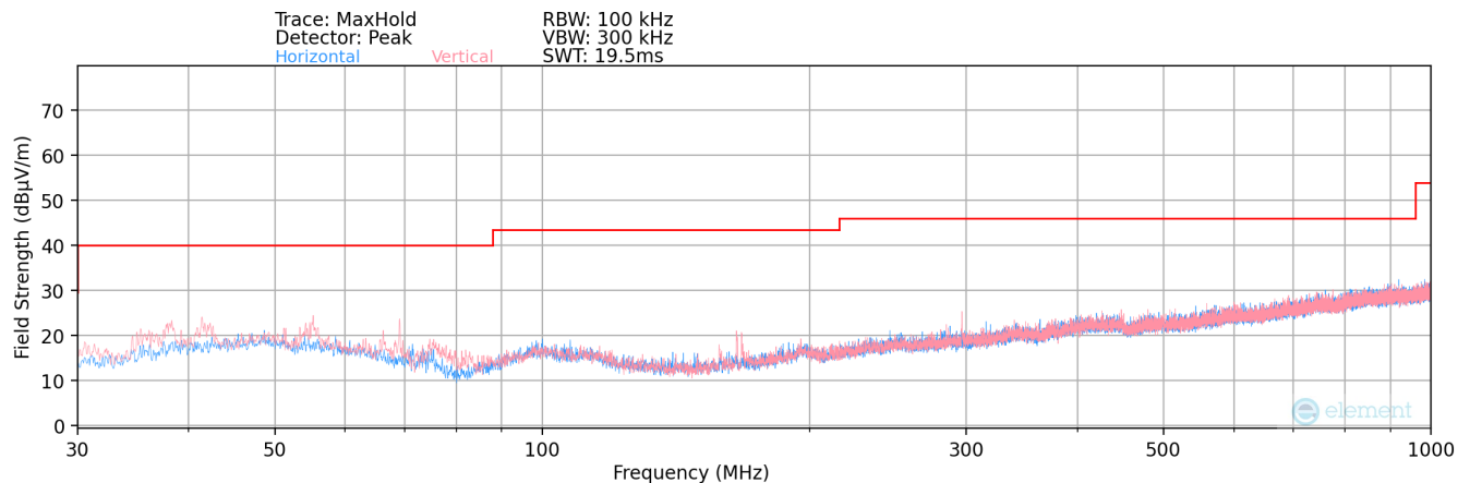
Plot 7-195. Radiated Spurious Plot below 1GHz MIMO
