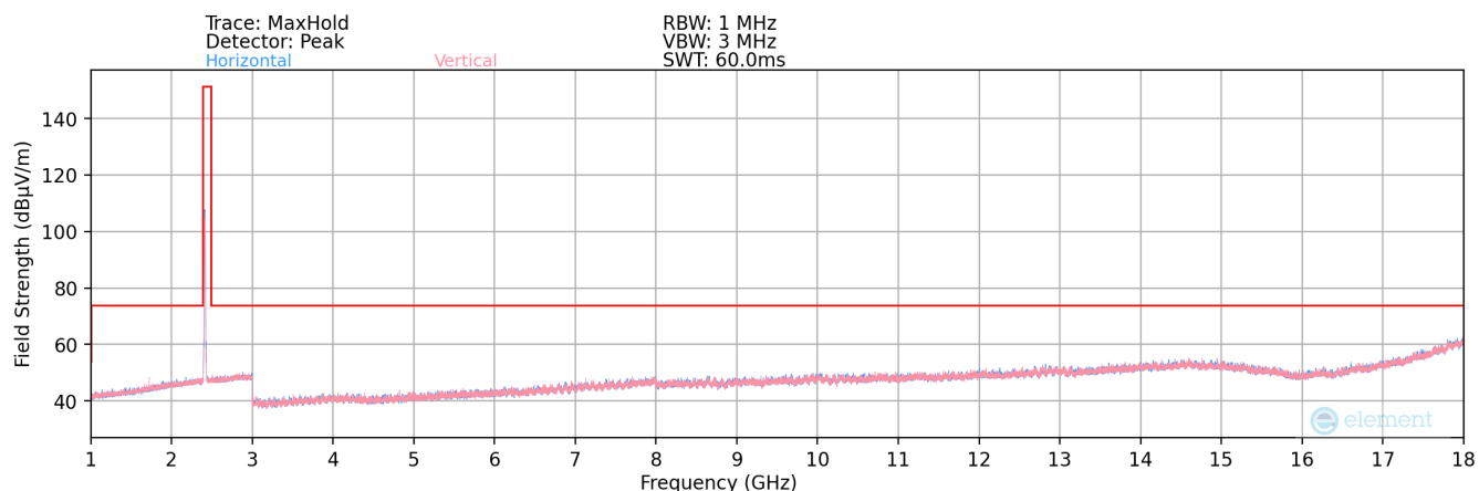
Plot 7-191. Radiated Spurious Plot above 1GHz SISO ANT2 (802.11b – Ch. 1)
