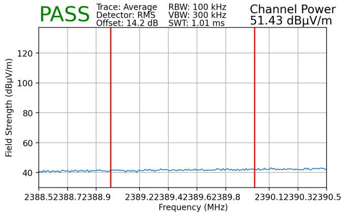
Plot 7-200. Radiated Restricted Lower Band Edge Measurement SISO ANT1 (Average)
