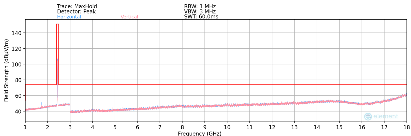
Plot 7-192. Radiated Spurious Plot above 1GHz SISO ANT2 (802.11b – Ch. 6)
