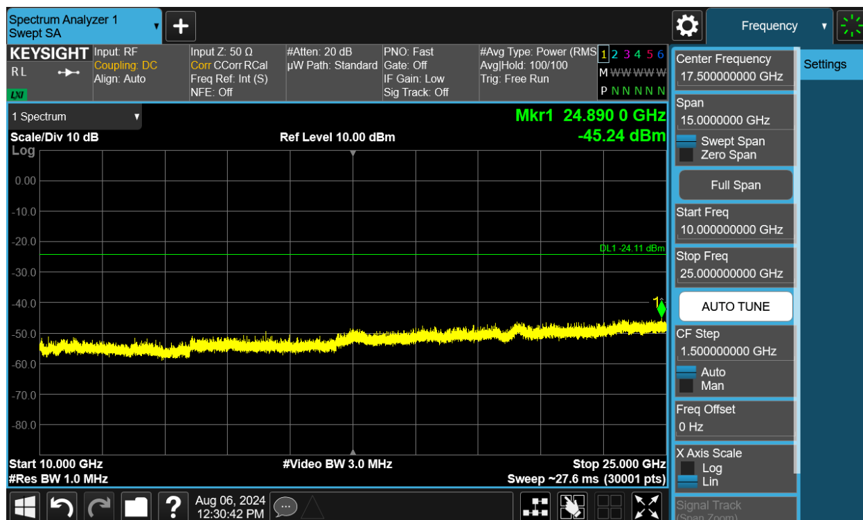
Plot 7-184. Conducted Spurious Plot MIMO ANT2 (802.11b – Ch. 11)
