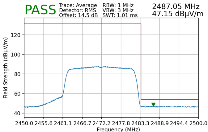
Plot 7-206. Radiated Restricted Upper Band Edge Measurement SISO ANT1 (Average)
