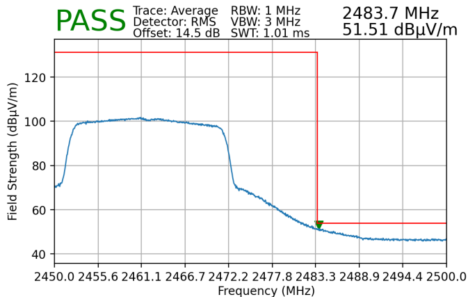
Plot 7-202. Radiated Restricted Upper Band Edge Measurement SISO ANT1 (Average)
