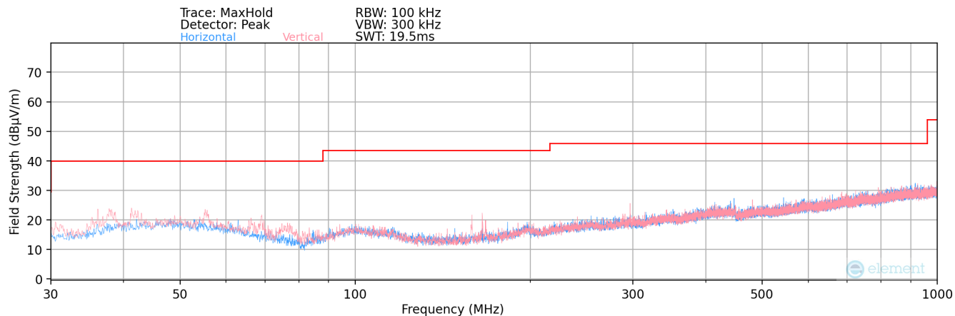
Plot 7-190. Radiated Spurious Plot below 1GHz SISO ANT2
