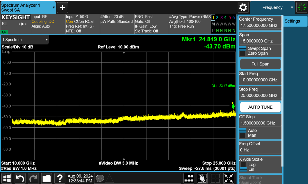
Plot 7-182. Conducted Spurious Plot MIMO ANT2 (802.11b – Ch. 6)
