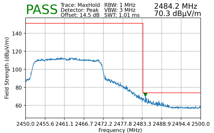
Plot 7-211. Radiated Restricted Upper Band Edge Measurement SISO ANT2 (Peak)
