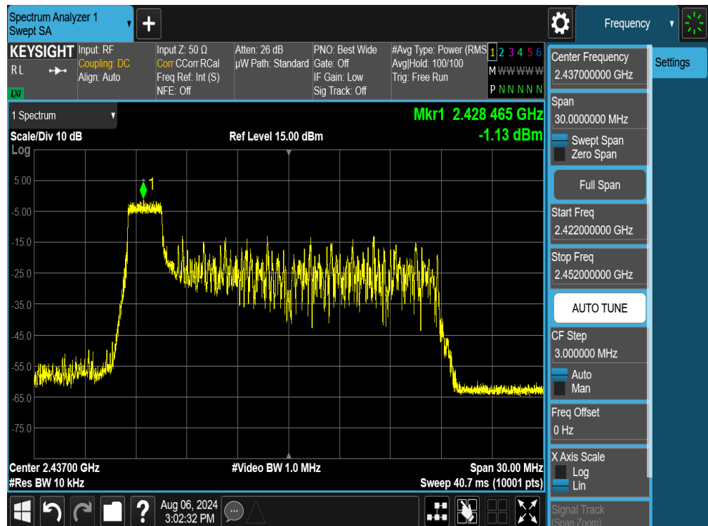
Plot 7-32. Power Spectral Density Plot SISO ANT2 (802.11ax/be OFDMA – 26 Tones – Ch. 6)
