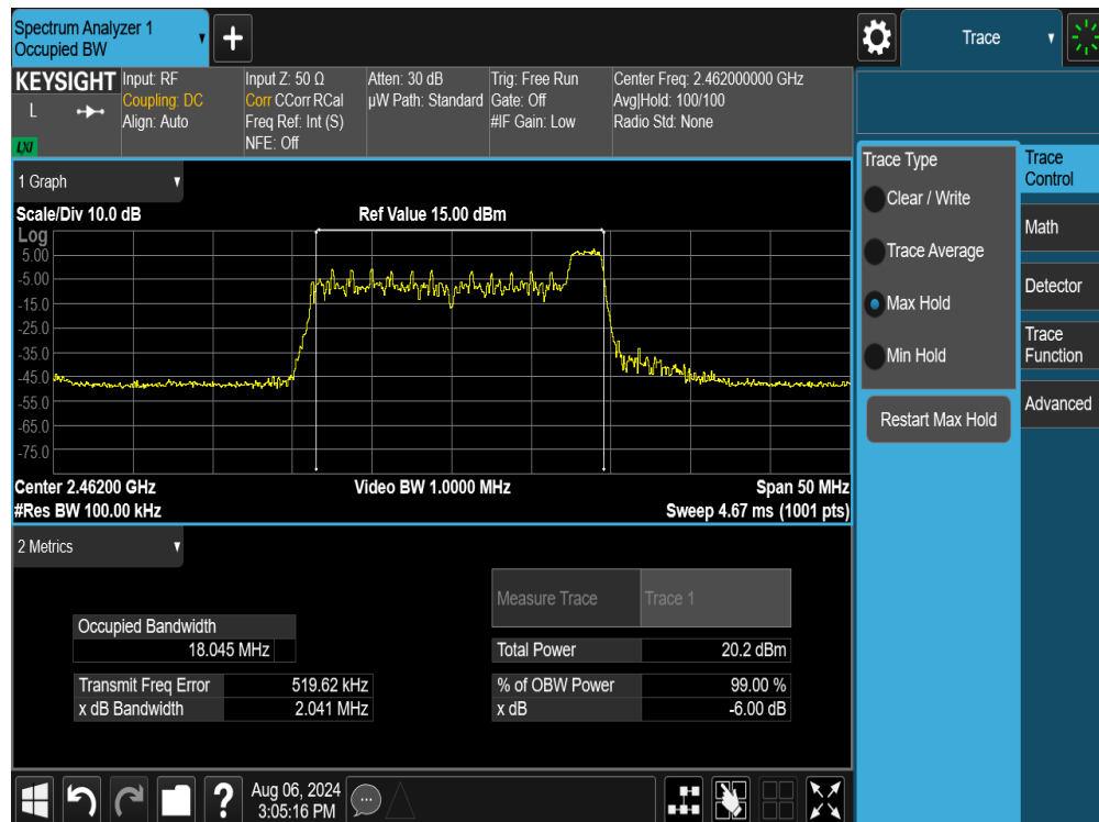
Plot 7-9. 6dB Bandwidth Plot SISO ANT2 (802.11ax/be OFDMA – 26 Tones – Ch. 11)
