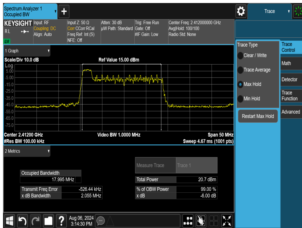
Plot 7-1. 6dB Bandwidth Plot SISO ANT1 (802.11ax/be OFDMA – 26 Tones – Ch. 1)
