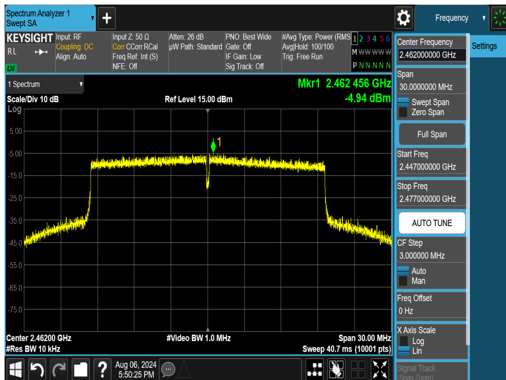
Plot 7-36. Power Spectral Density Plot SISO ANT2 (802.11ax/be OFDMA – 242 Tones – Ch. 11)
