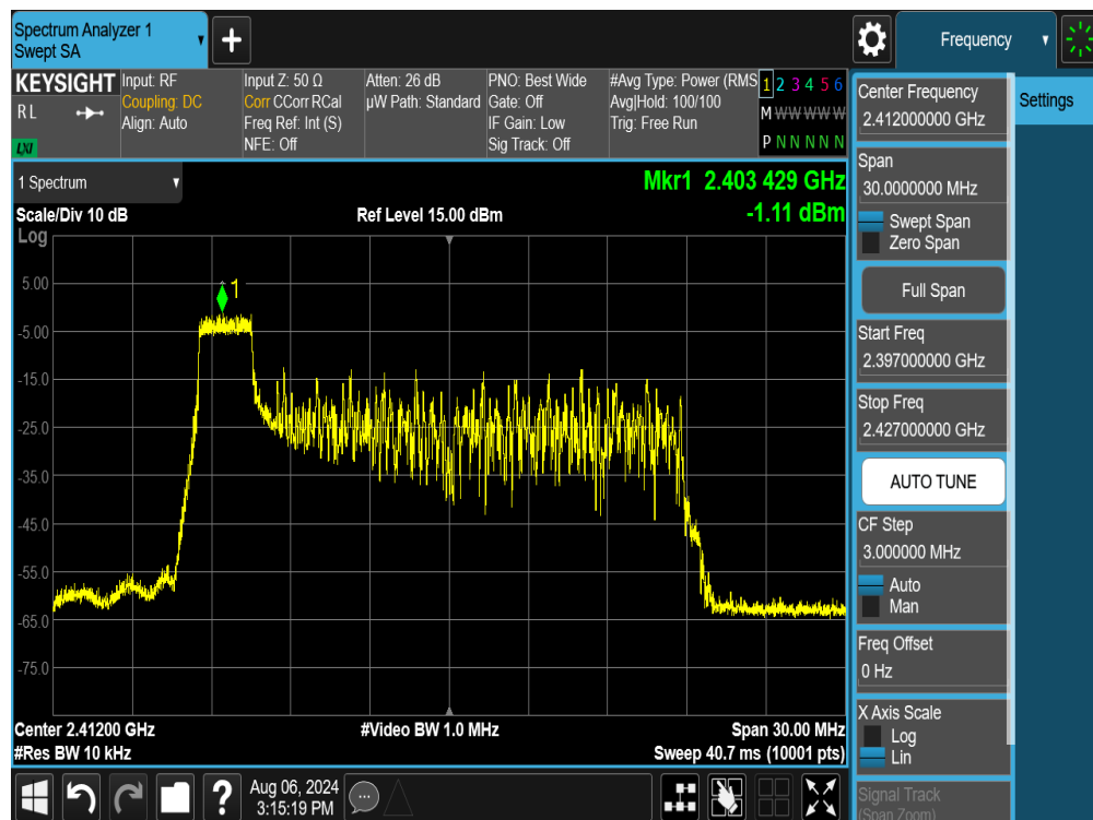
Plot 7-25. Power Spectral Density Plot SISO ANT1 (802.11ax/be OFDMA – 26 Tones – Ch. 1)
