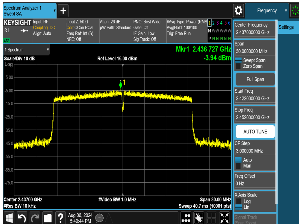
Plot 7-35. Power Spectral Density Plot SISO ANT2 (802.11ax/be OFDMA – 242 Tones – Ch. 6)
