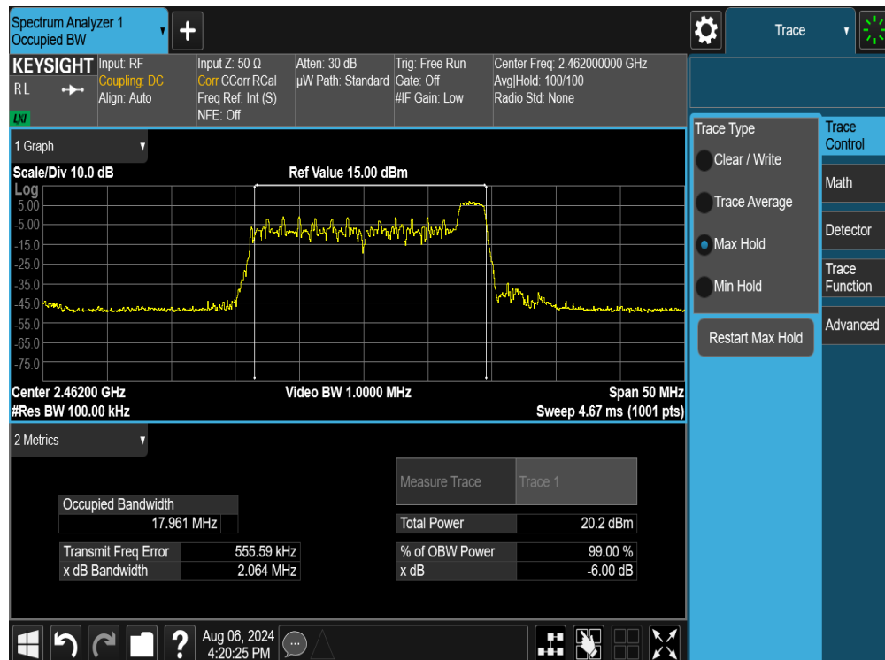
Plot 7-3. 6dB Bandwidth Plot SISO ANT1 (802.11ax/be OFDMA – 26 Tones – Ch. 11)
