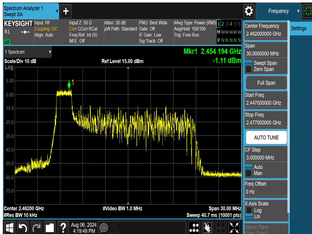
Plot 7-27. Power Spectral Density Plot SISO ANT1 (802.11ax/be OFDMA – 26 Tones – Ch. 11)
