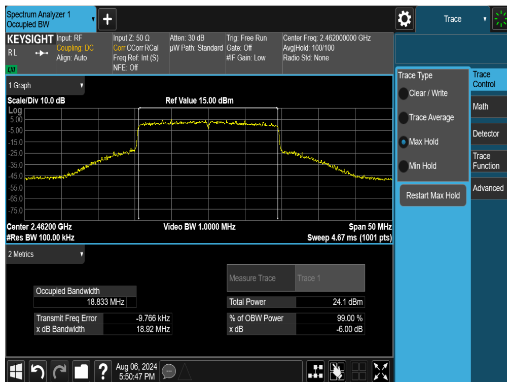
Plot 7-12. 6dB Bandwidth Plot SISO ANT2 (802.11ax/be OFDMA – 242 Tones – Ch. 11)
