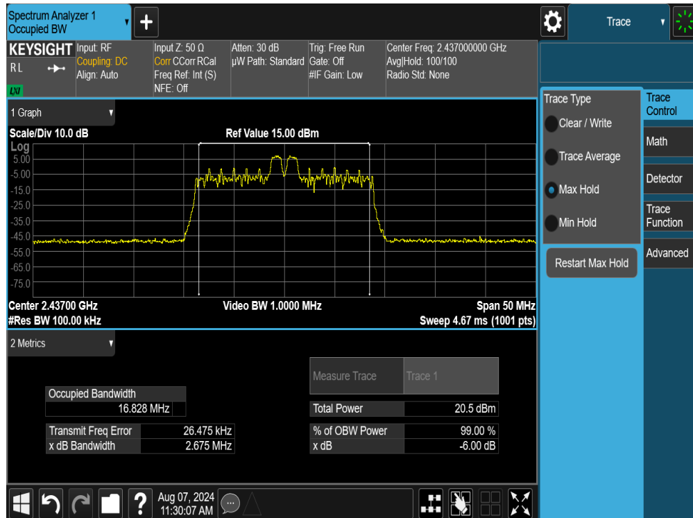
Plot 7-20. 6dB Bandwidth Plot MIMO ANT2 (802.11ax/be OFDMA – 26Tones – Ch. 6)
