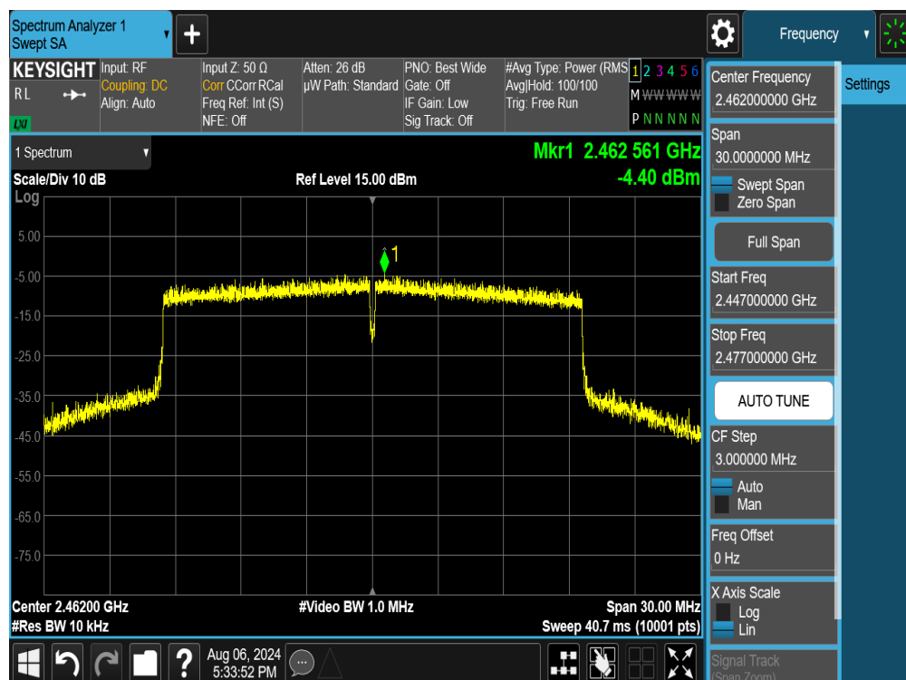
Plot 7-30. Power Spectral Density Plot SISO ANT1 (802.11ax/be OFDMA – 242 Tones – Ch. 11)
