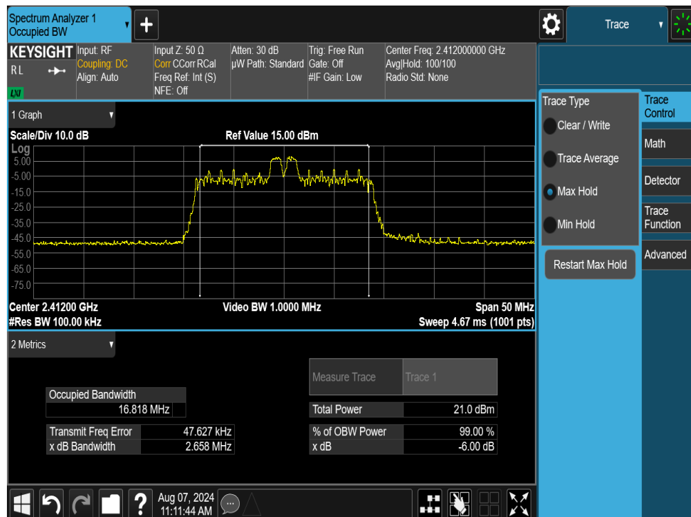
Plot 7-13. 6dB Bandwidth Plot MIMO ANT1 (802.11ax/be OFDMA – 26Tones – Ch. 1)
