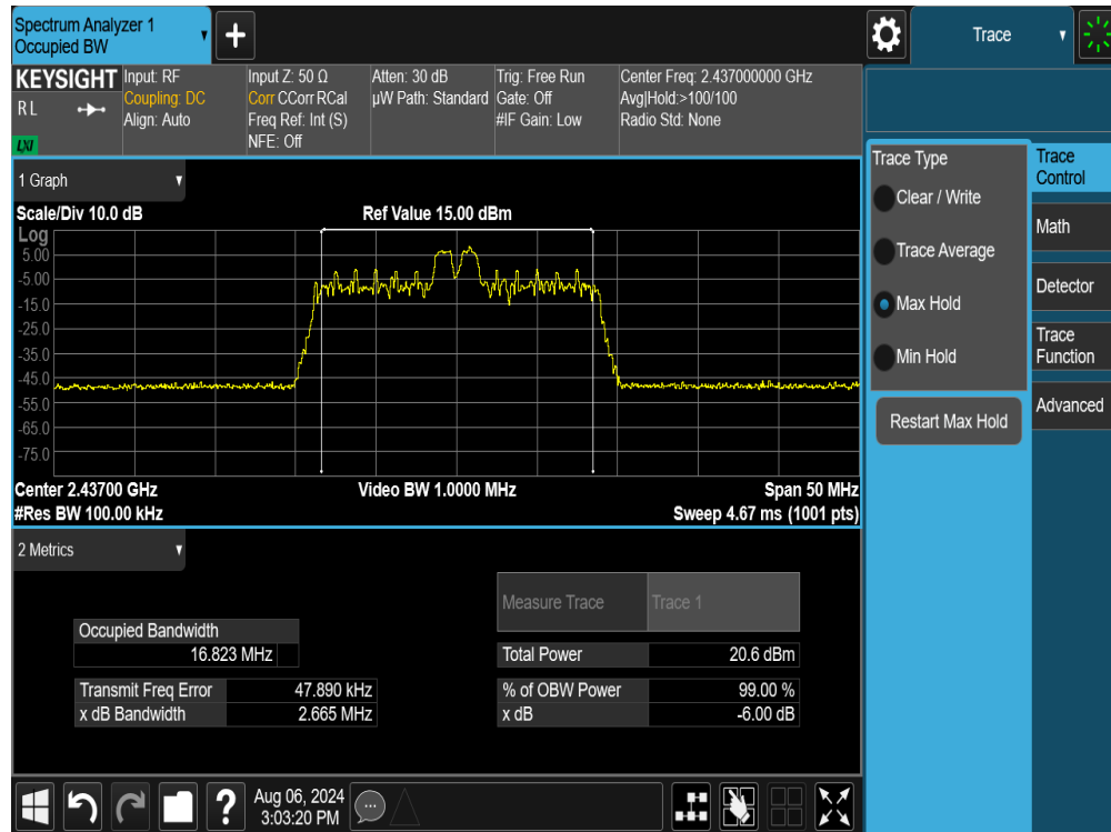
Plot 7-8. 6dB Bandwidth Plot SISO ANT2 (802.11ax/be OFDMA – 26 Tones – Ch. 6)
