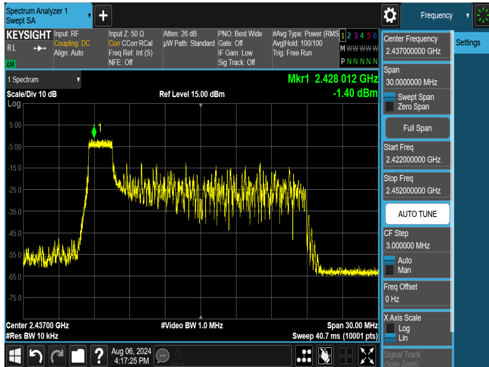
Plot 7-26. Power Spectral Density Plot SISO ANT1 (802.11ax/be OFDMA – 26 Tones – Ch. 6)
