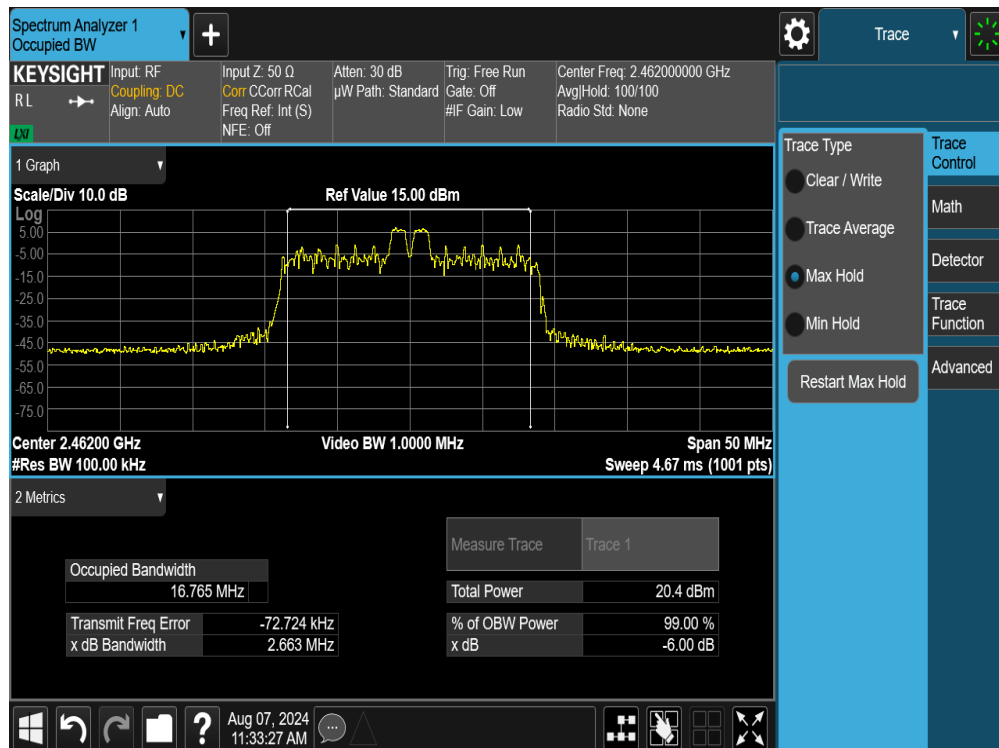
Plot 7-21. 6dB Bandwidth Plot MIMO ANT2 (802.11ax/be OFDMA – 26Tones – Ch. 11)
