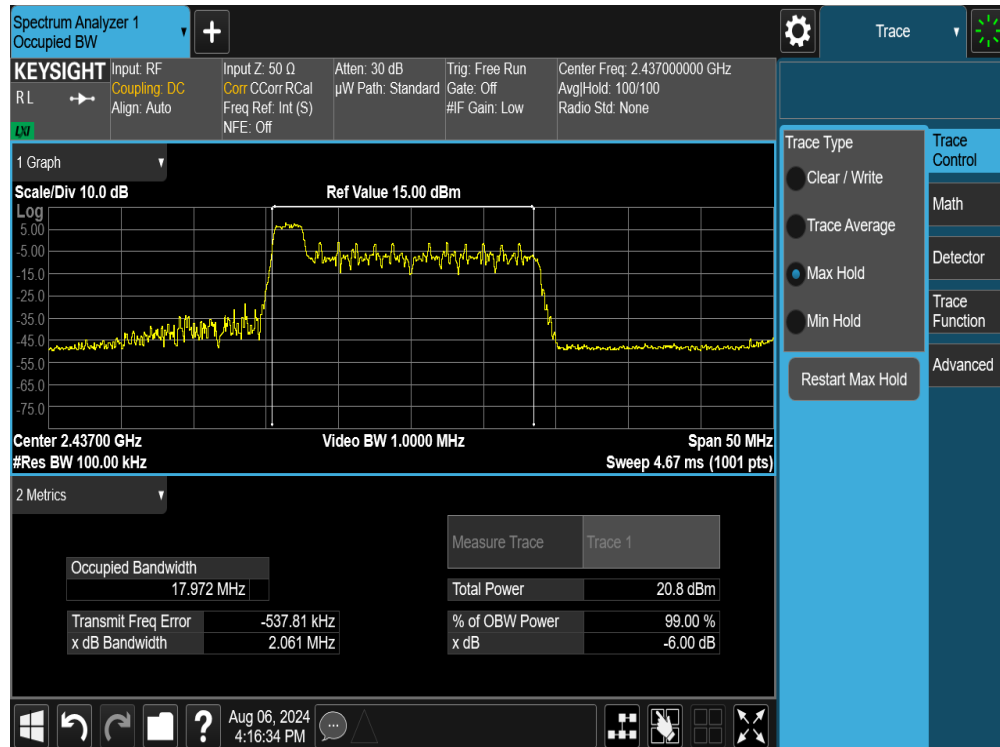
Plot 7-2. 6dB Bandwidth Plot SISO ANT1 (802.11ax/be OFDMA – 26 Tones – Ch. 6)
