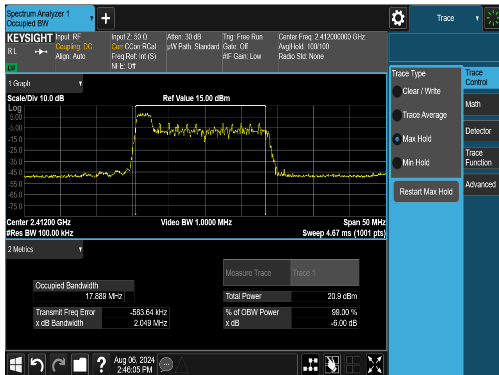
Plot 7-7. 6dB Bandwidth Plot SISO ANT2 (802.11ax/be OFDMA – 26 Tones – Ch. 1)
