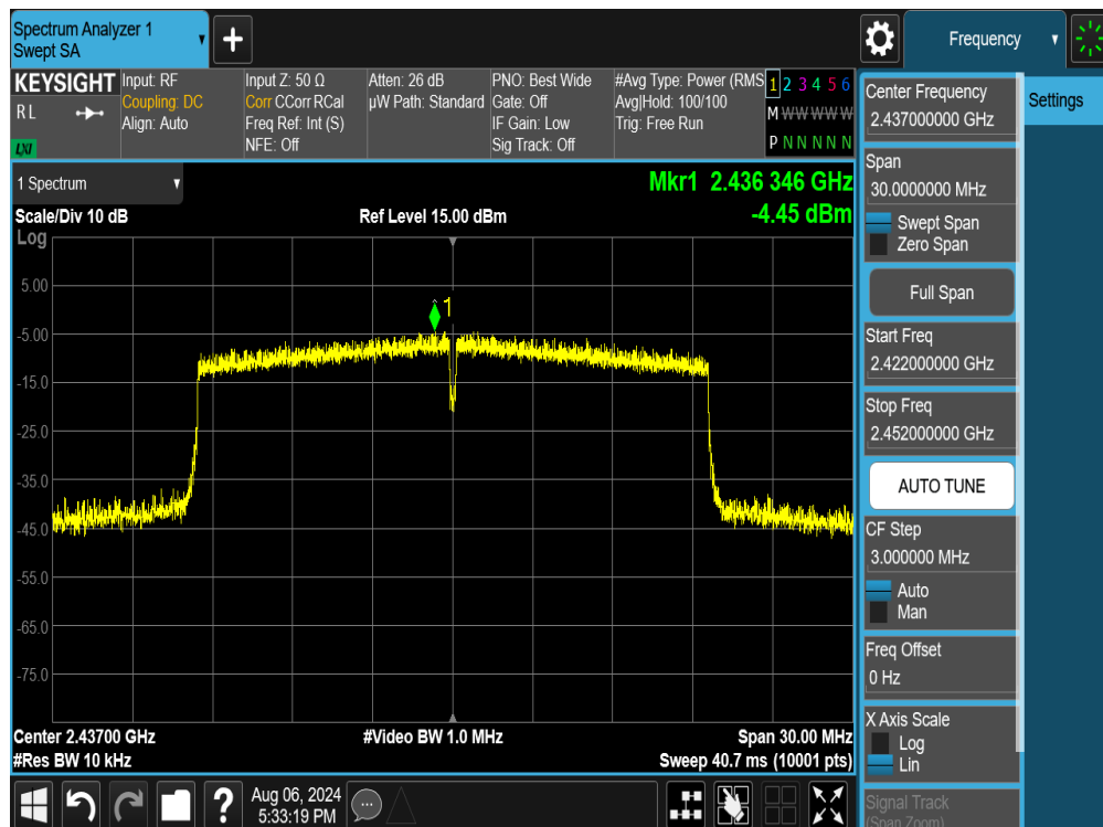
Plot 7-29. Power Spectral Density Plot SISO ANT1 (802.11ax/be OFDMA – 242 Tones – Ch. 6)
