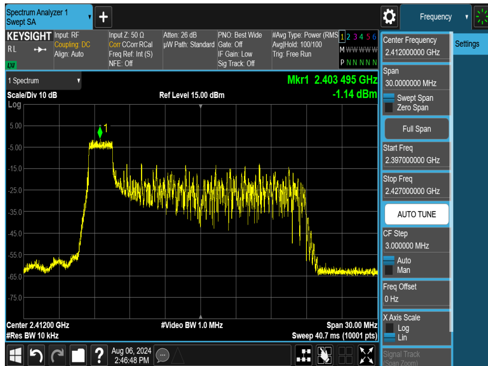
Plot 7-31. Power Spectral Density Plot SISO ANT2 (802.11ax/be OFDMA – 26 Tones – Ch. 1)
