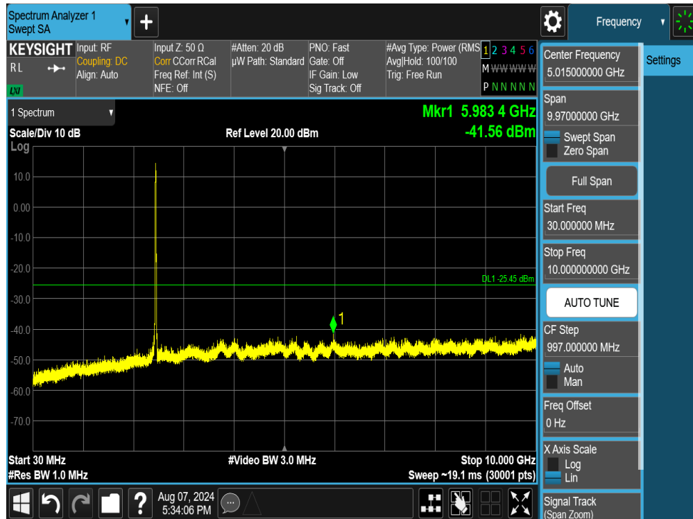
Plot 7-127. Conducted Spurious Plot MIMO ANT2 (802.11ax/be OFDMA – 242 Tones – Ch. 11)
