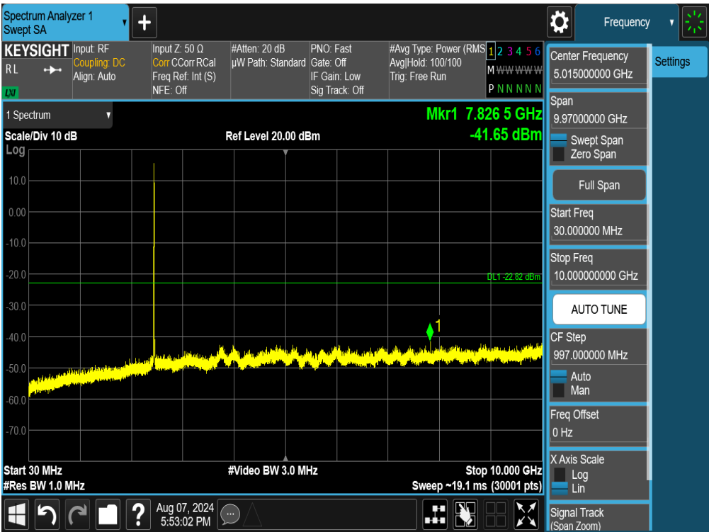
Plot 7-109. Conducted Spurious Plot MIMO ANT1 (802.11ax/be OFDMA – 26 Tones – Ch. 11)
