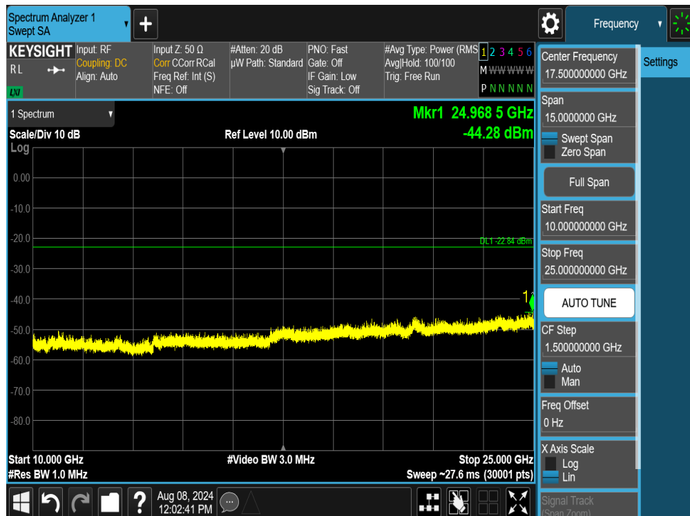
Plot 7-118. Conducted Spurious Plot MIMO ANT2 (802.11ax/be OFDMA – 26 Tones – Ch. 1)
