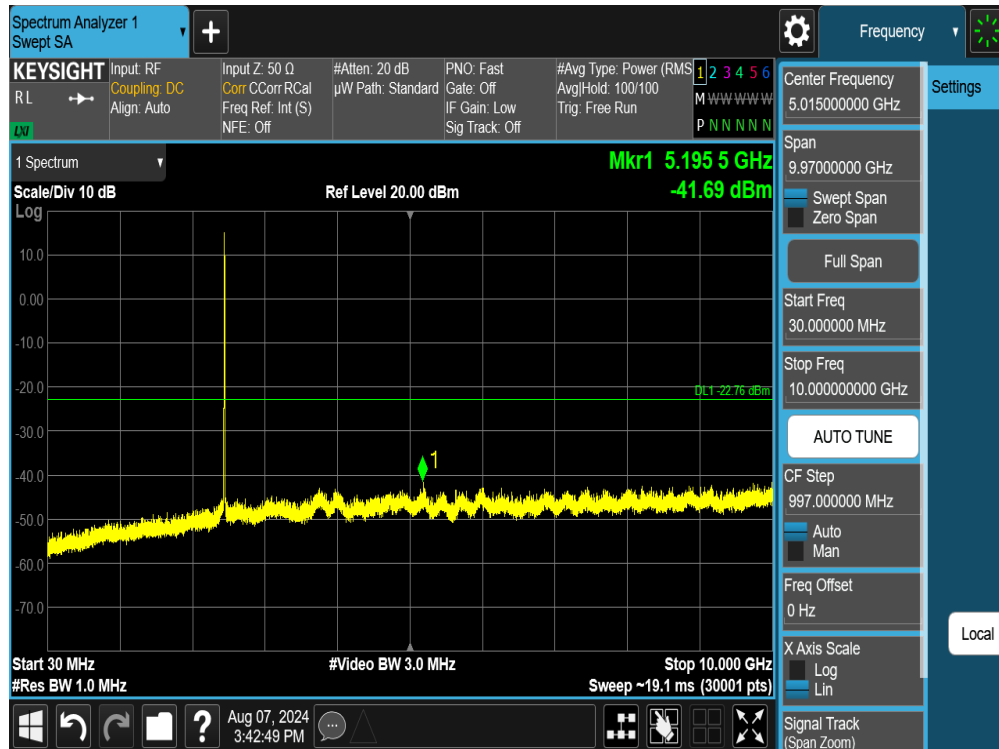
Plot 7-85. Conducted Spurious Plot SISO ANT1 (802.11ax/be OFDMA – 26 Tones – Ch. 11)
