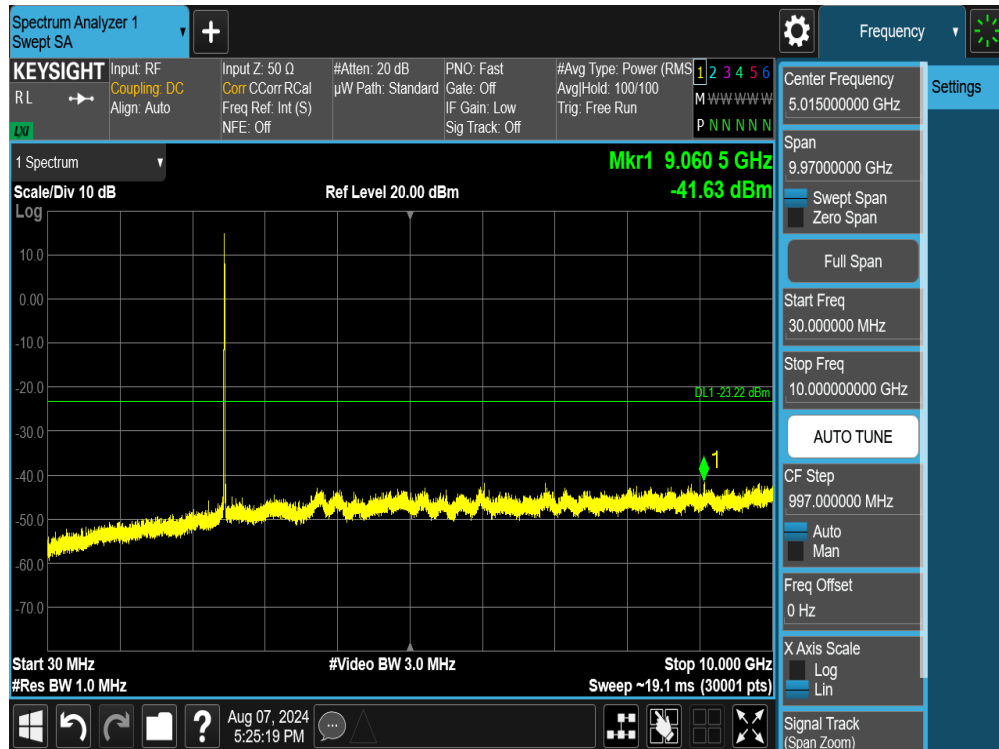
Plot 7-121. Conducted Spurious Plot MIMO ANT2 (802.11ax/be OFDMA – 26 Tones – Ch. 11)
