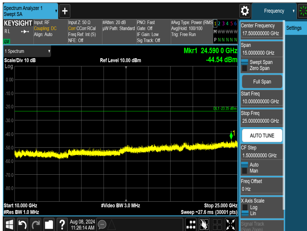
Plot 7-94. Conducted Spurious Plot SISO ANT2 (802.11ax/be OFDMA – 26 Tones – Ch. 1)
