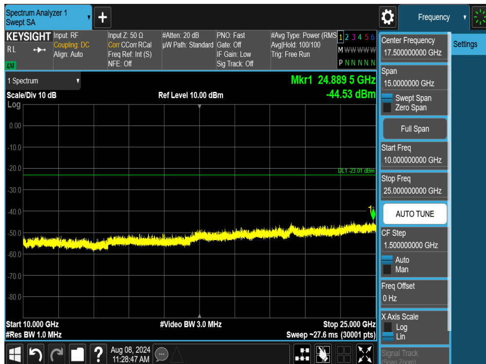
Plot 7-98. Conducted Spurious Plot SISO ANT2 (802.11ax/be OFDMA – 26 Tones – Ch. 11)
