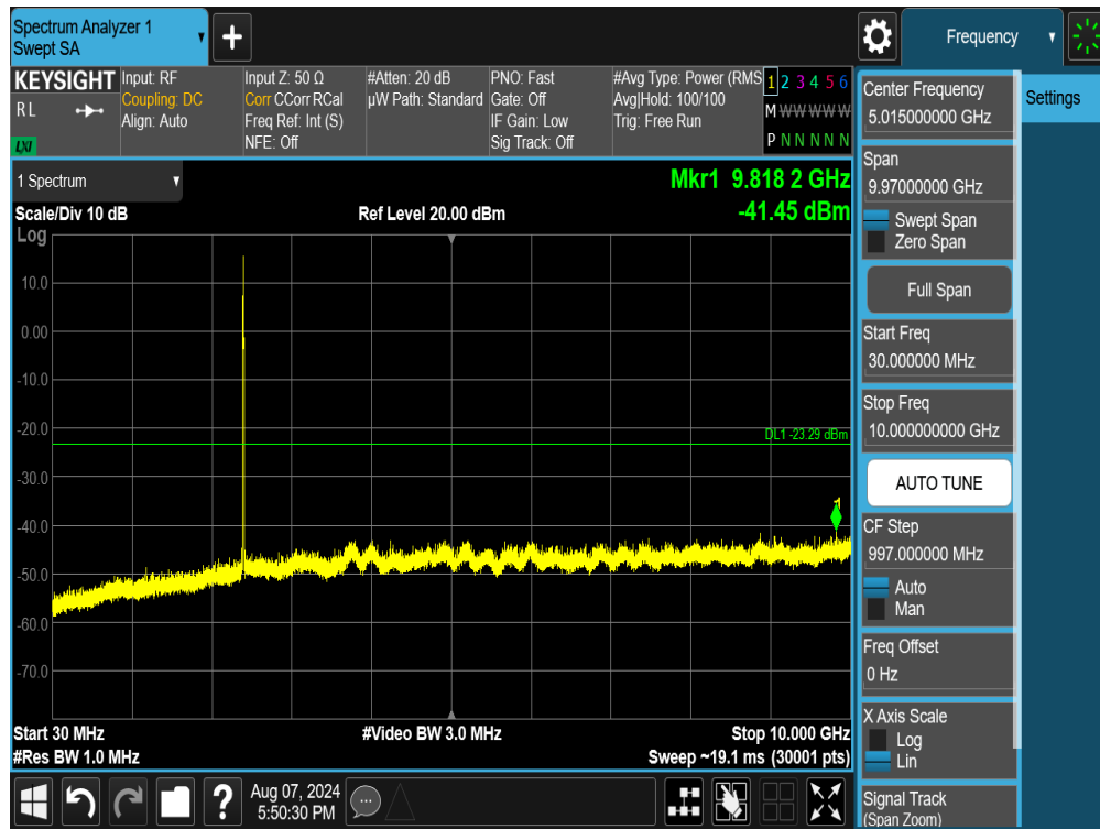
Plot 7-105. Conducted Spurious Plot MIMO ANT1 (802.11ax/be OFDMA – 26 Tones – Ch. 1)
