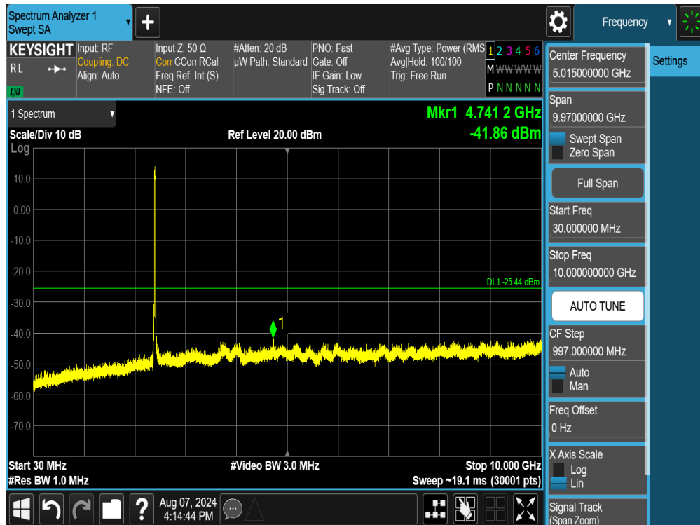
Plot 7-99. Conducted Spurious Plot SISO ANT2 (802.11ax/be OFDMA – 242 Tones – Ch. 1)
