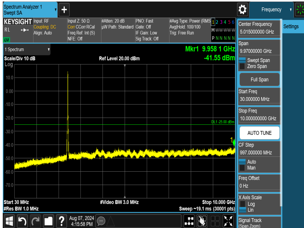
Plot 7-101. Conducted Spurious Plot SISO ANT2 (802.11ax/be OFDMA – 242 Tones – Ch. 6)
