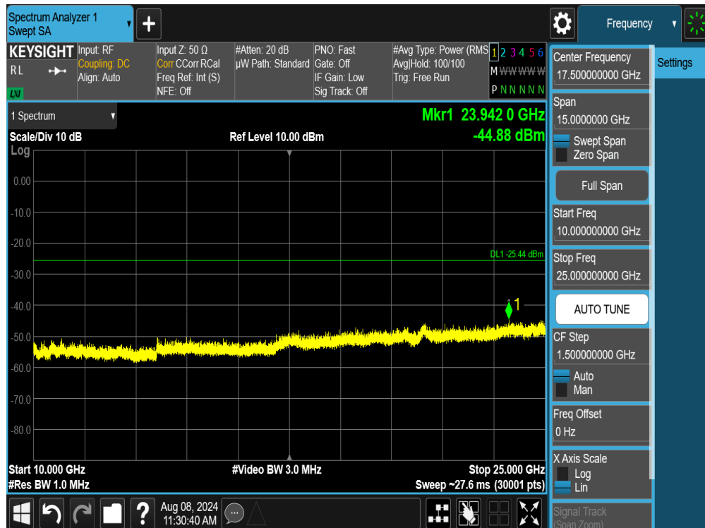
Plot 7-100. Conducted Spurious Plot SISO ANT2 (802.11ax/be OFDMA – 242 Tones – Ch. 1)
