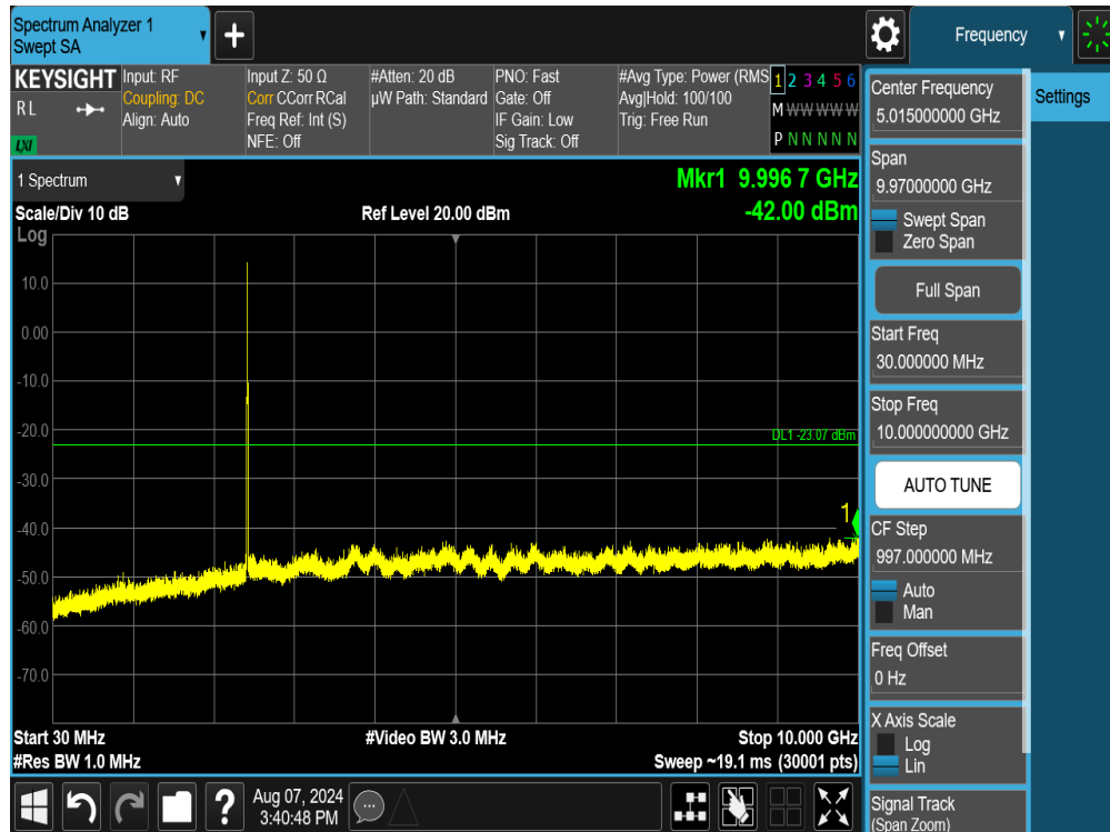
Plot 7-83. Conducted Spurious Plot SISO ANT1 (802.11ax/be OFDMA – 26 Tones – Ch. 6)
