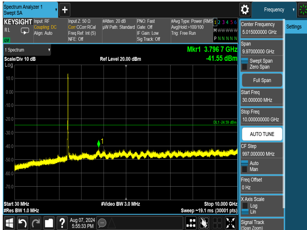
Plot 7-111. Conducted Spurious Plot MIMO ANT1 (802.11ax/be OFDMA – 242 Tones – Ch. 1)
