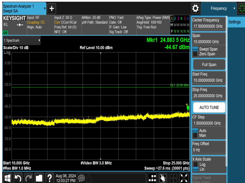
Plot 7-120. Conducted Spurious Plot MIMO ANT2 (802.11ax/be OFDMA – 26 Tones – Ch. 6)
