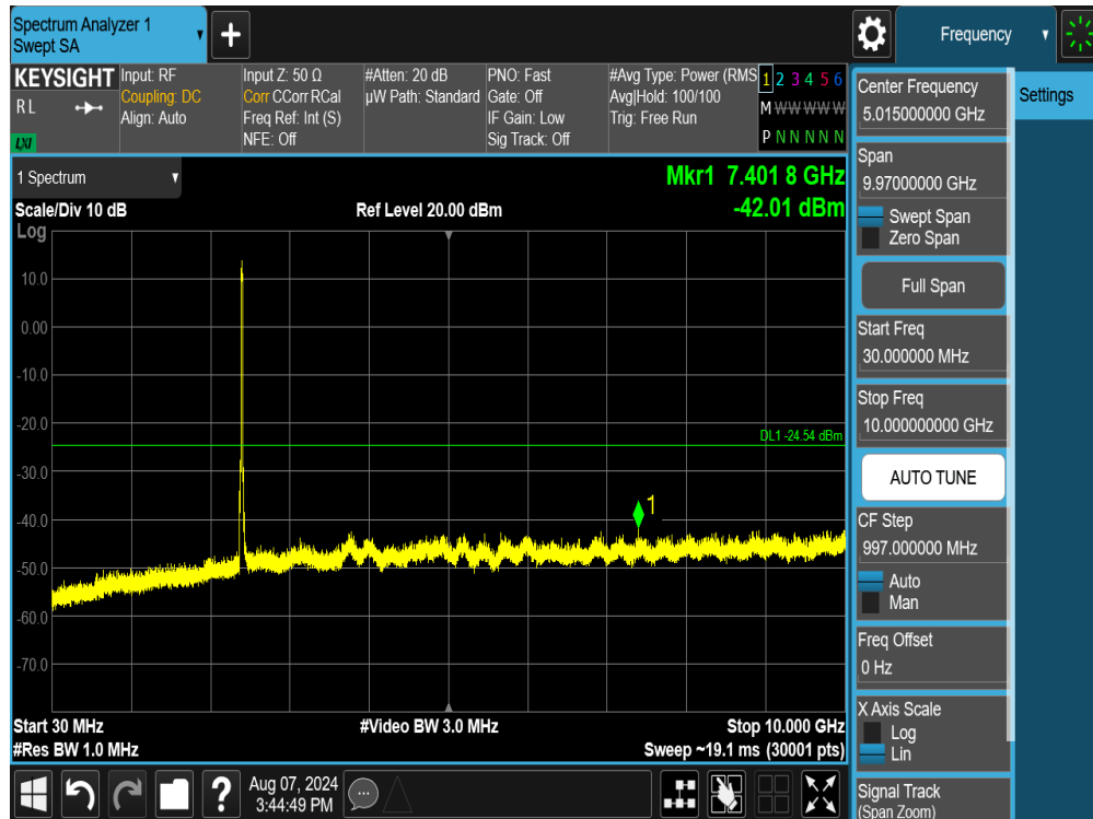
Plot 7-87. Conducted Spurious Plot SISO ANT1 (802.11ax/be OFDMA – 242 Tones – Ch. 1)
