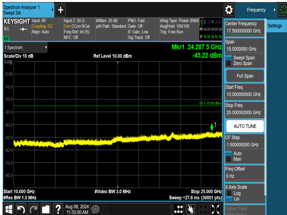
Plot 7-102. Conducted Spurious Plot SISO ANT2 (802.11ax/be OFDMA – 242 Tones – Ch. 6)
