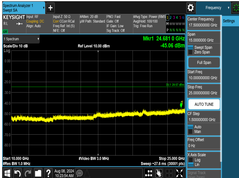
Plot 7-90. Conducted Spurious Plot SISO ANT1 (802.11ax/be OFDMA – 242 Tones – Ch. 6)
