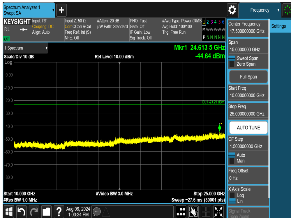
Plot 7-106. Conducted Spurious Plot MIMO ANT1 (802.11ax/be OFDMA – 26 Tones – Ch. 1)
