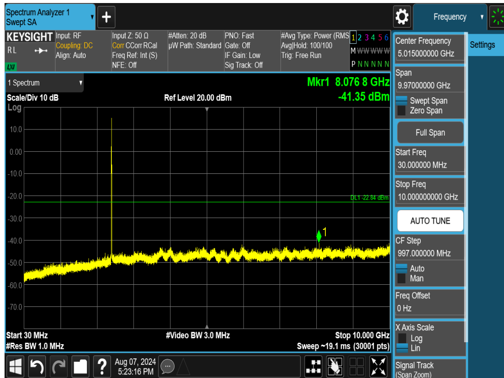
Plot 7-117. Conducted Spurious Plot MIMO ANT2 (802.11ax/be OFDMA – 26 Tones – Ch. 1)
