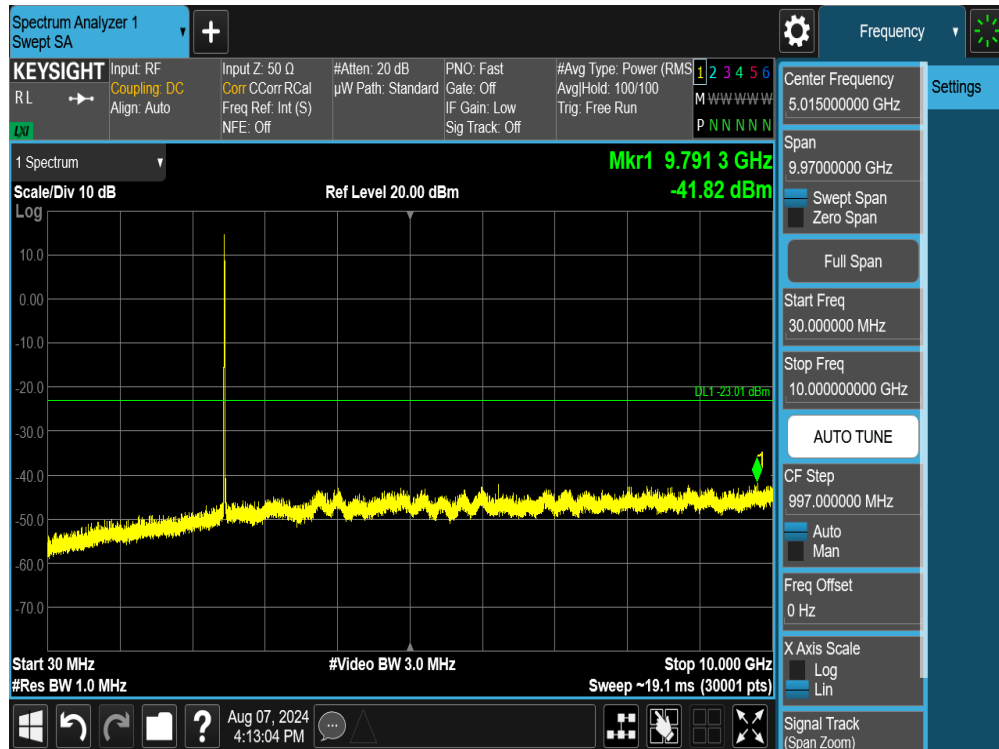
Plot 7-97. Conducted Spurious Plot SISO ANT2 (802.11ax/be OFDMA – 26 Tones – Ch. 11)
