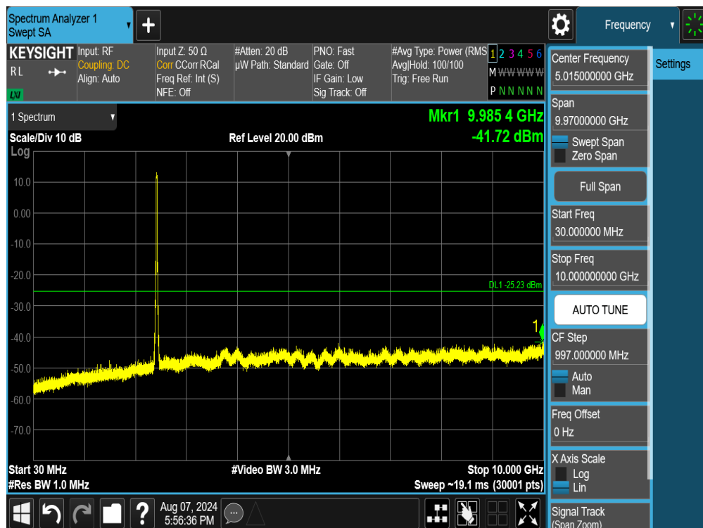
Plot 7-113. Conducted Spurious Plot MIMO ANT1 (802.11ax/be OFDMA – 242 Tones – Ch. 6)
