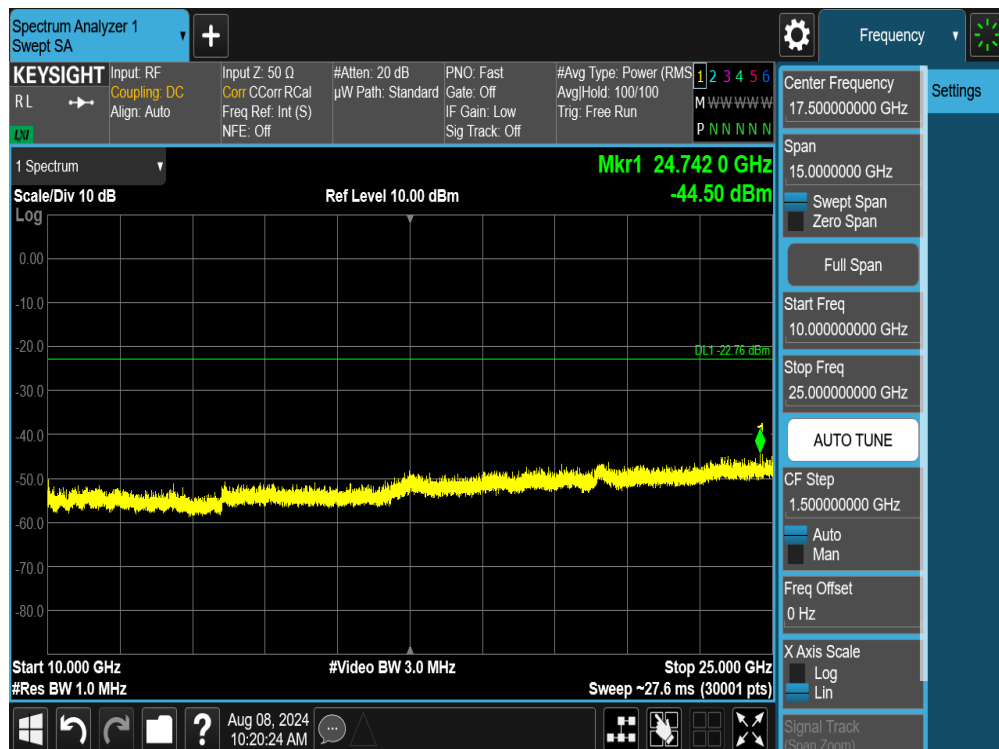
Plot 7-86. Conducted Spurious Plot SISO ANT1 (802.11ax/be OFDMA – 26 Tones – Ch. 11)
