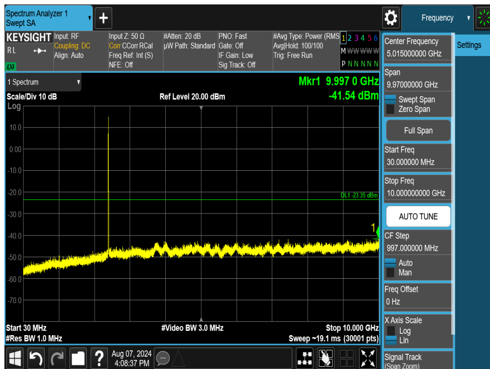
Plot 7-93. Conducted Spurious Plot SISO ANT2 (802.11ax/be OFDMA – 26 Tones – Ch. 1)
