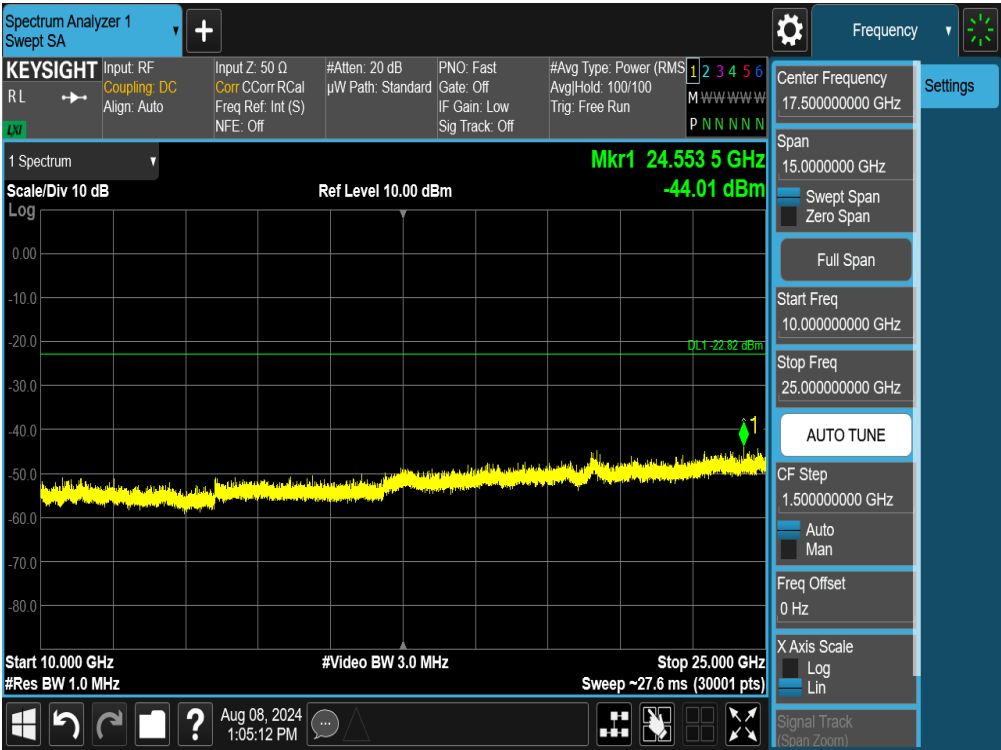
Plot 7-110. Conducted Spurious Plot MIMO ANT1 (802.11ax/be OFDMA – 26 Tones – Ch. 11)
