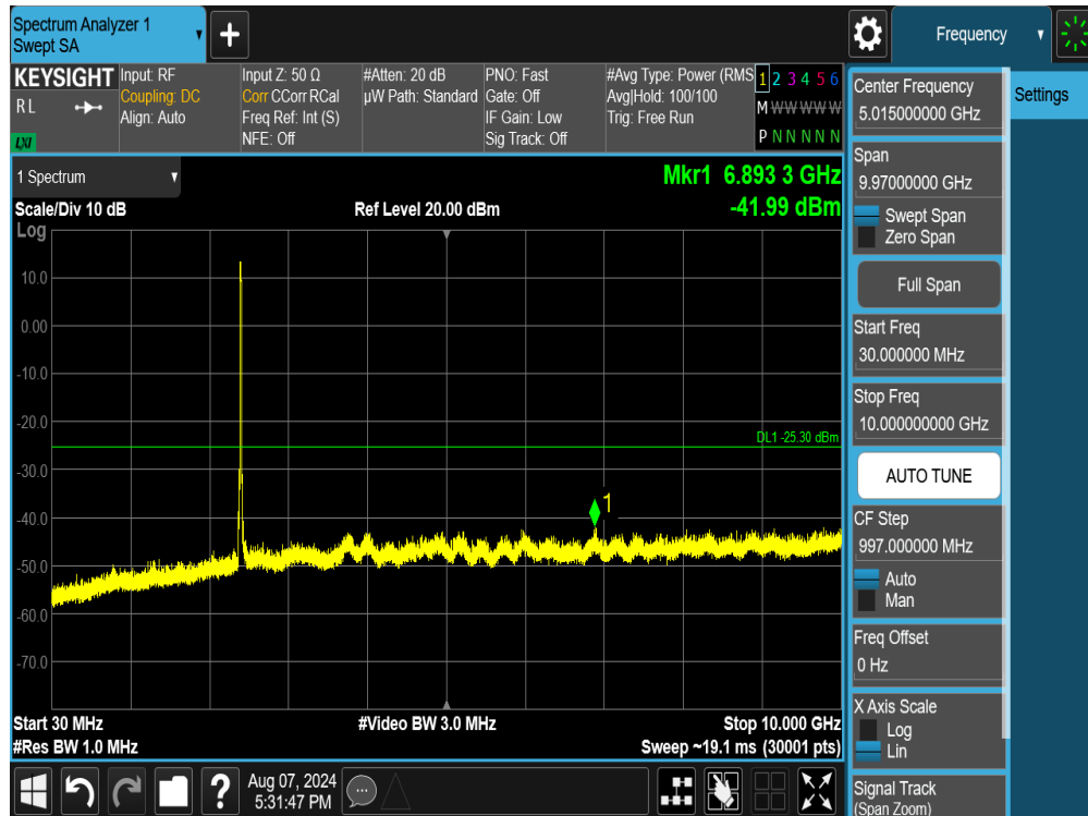
Plot 7-123. Conducted Spurious Plot MIMO ANT2 (802.11ax/be OFDMA – 242 Tones – Ch. 1)
