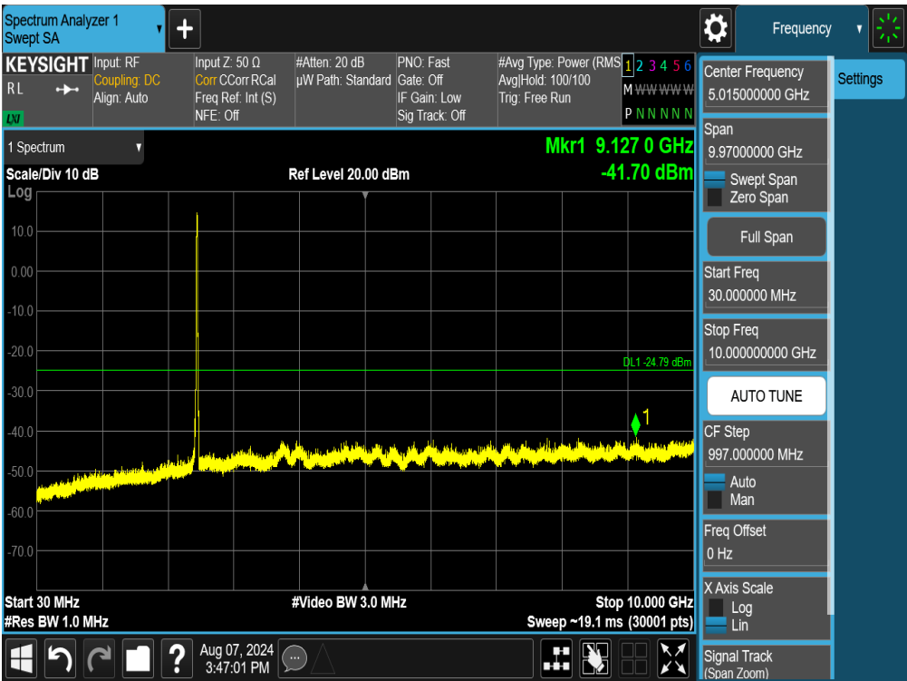
Plot 7-91. Conducted Spurious Plot SISO ANT1 (802.11ax/be OFDMA – 242 Tones – Ch. 11)
