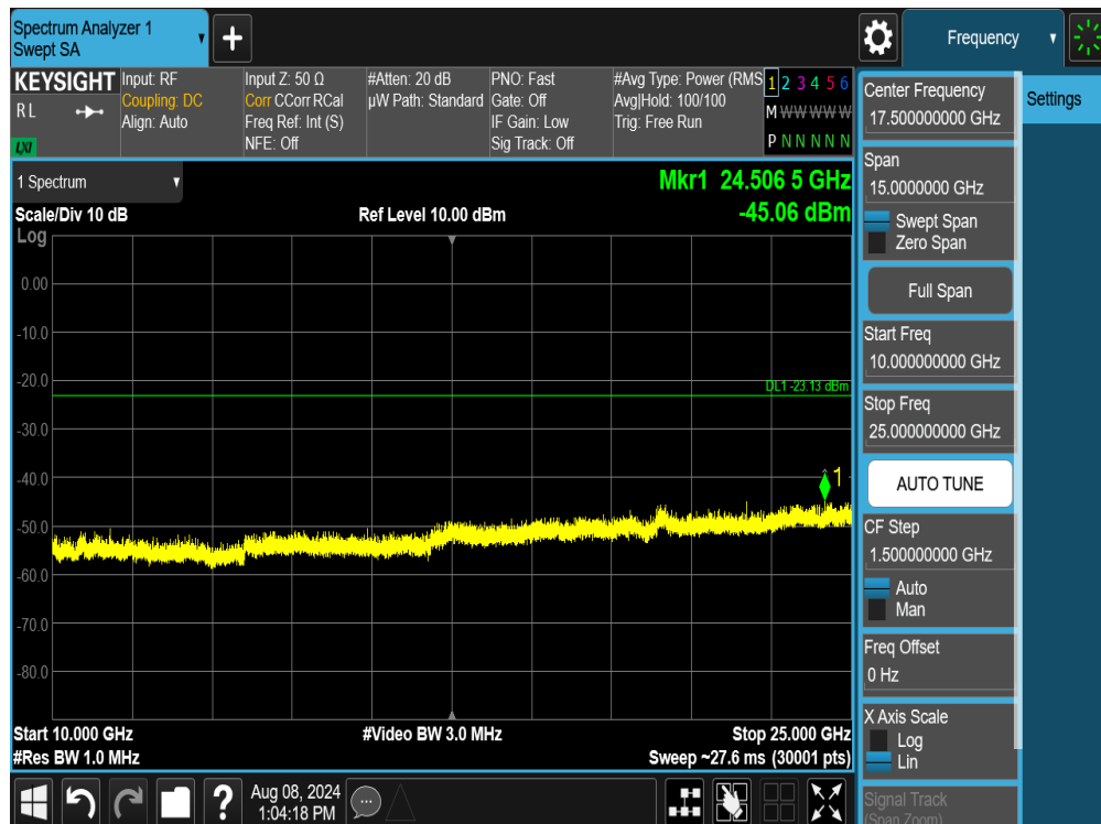
Plot 7-108. Conducted Spurious Plot MIMO ANT1 (802.11ax/be OFDMA – 26 Tones – Ch. 6)
