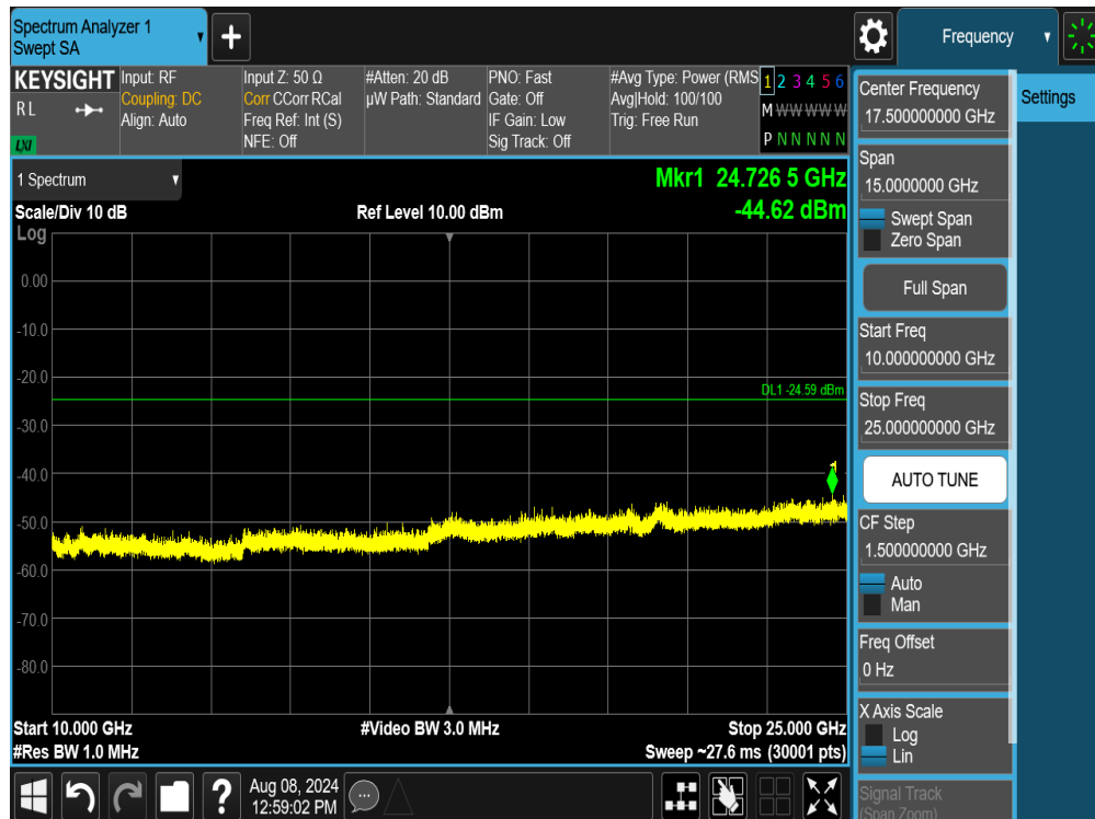
Plot 7-112. Conducted Spurious Plot MIMO ANT1 (802.11ax/be OFDMA – 242 Tones – Ch. 1)
