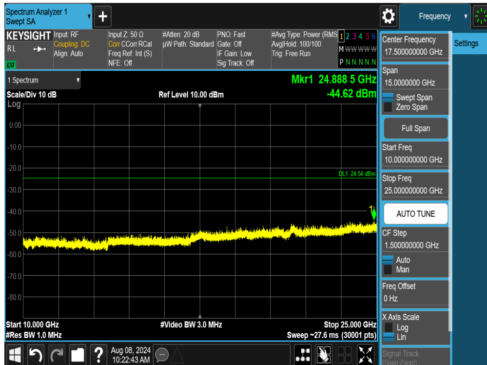
Plot 7-88. Conducted Spurious Plot SISO ANT1 (802.11ax/be OFDMA – 242 Tones – Ch. 1)
