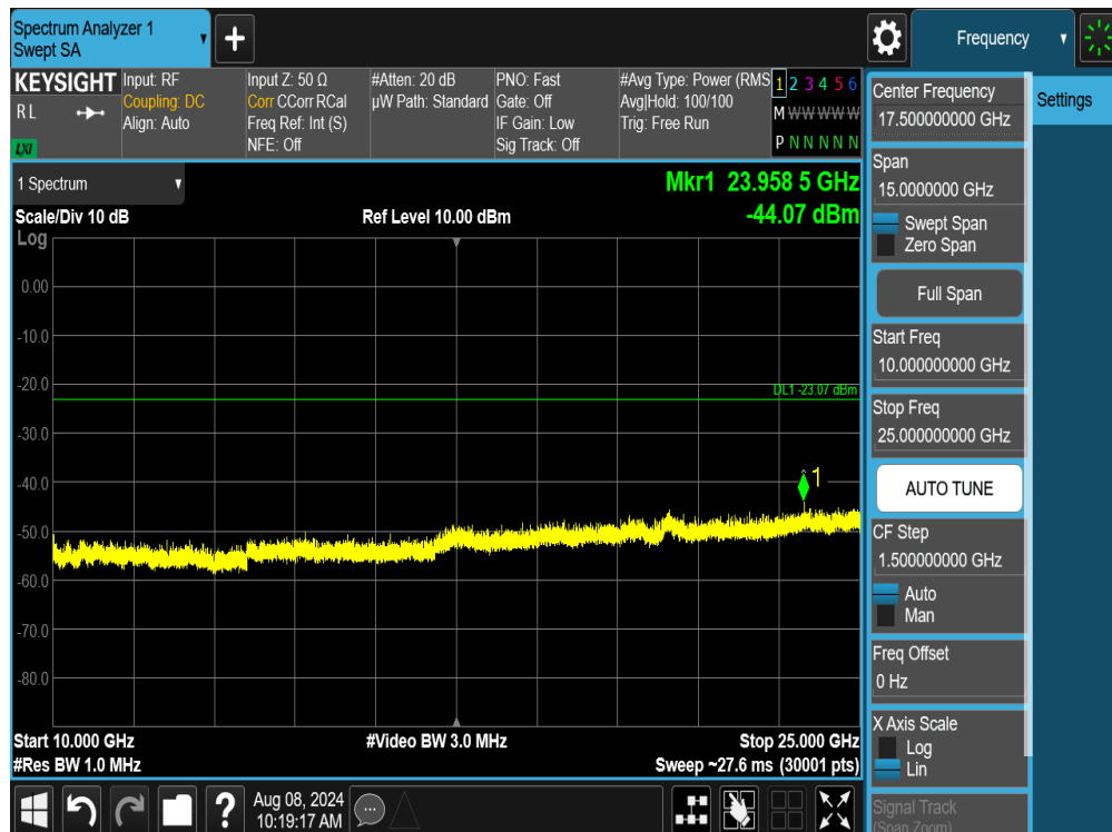
Plot 7-84. Conducted Spurious Plot SISO ANT1 (802.11ax/be OFDMA – 26 Tones – Ch. 6)
