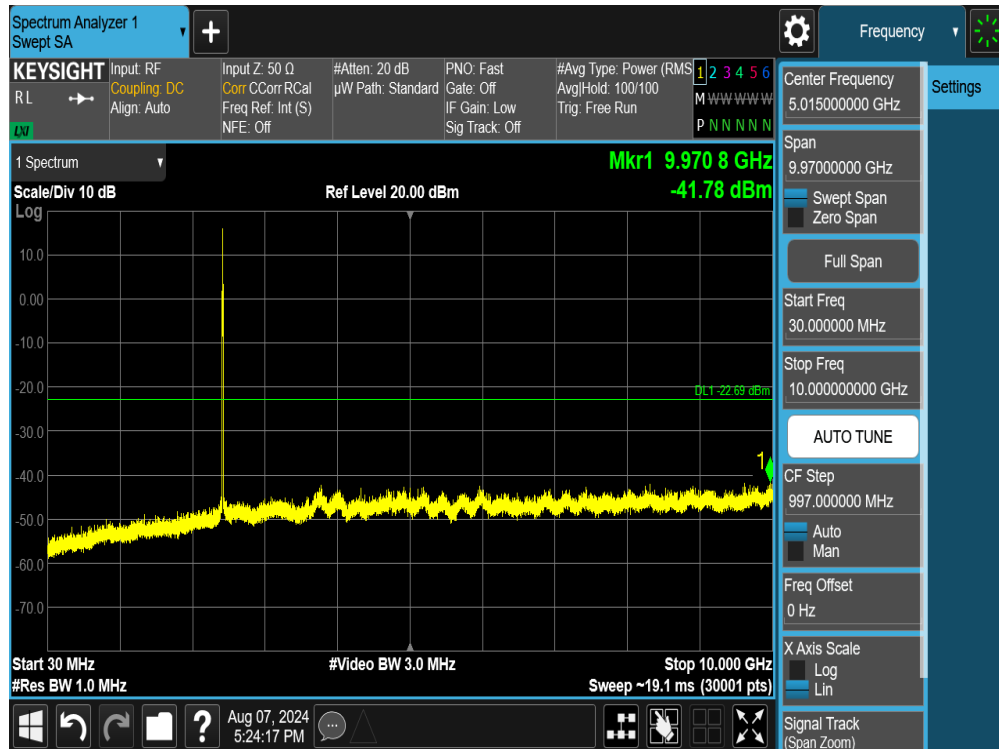
Plot 7-119. Conducted Spurious Plot MIMO ANT2 (802.11ax/be OFDMA – 26 Tones – Ch. 6)
