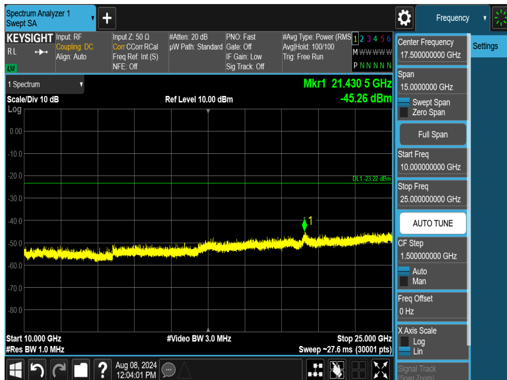
Plot 7-122. Conducted Spurious Plot MIMO ANT2 (802.11ax/be OFDMA – 26 Tones – Ch. 11)
