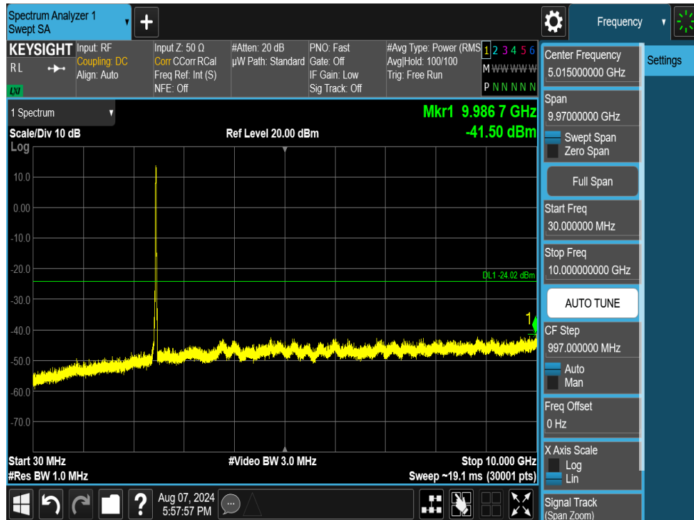
Plot 7-115. Conducted Spurious Plot MIMO ANT1 (802.11ax/be OFDMA – 242 Tones – Ch. 11)
