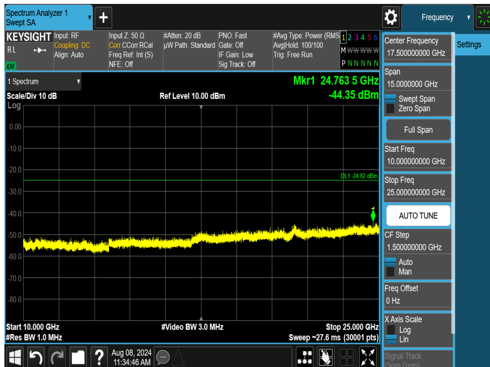
Plot 7-104. Conducted Spurious Plot SISO ANT2 (802.11ax/be OFDMA – 242 Tones – Ch. 11)
