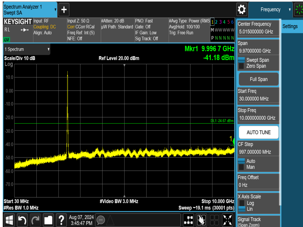
Plot 7-89. Conducted Spurious Plot SISO ANT1 (802.11ax/be OFDMA – 242 Tones – Ch. 6)
