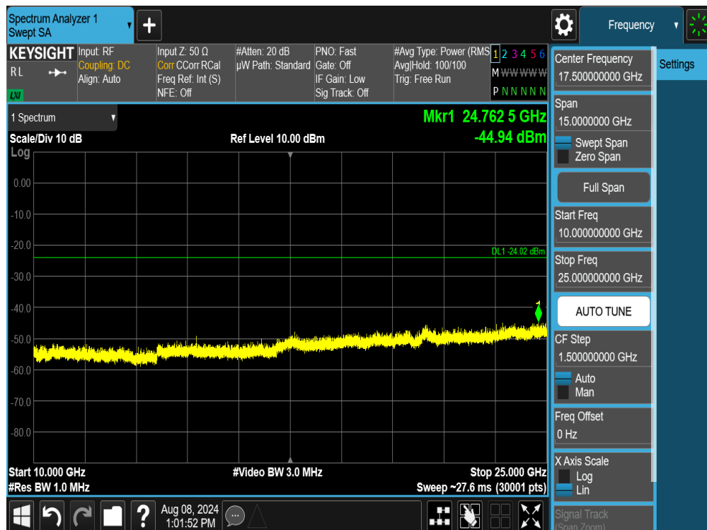
Plot 7-116. Conducted Spurious Plot MIMO ANT1 (802.11ax/be OFDMA – 242 Tones – Ch. 11)
