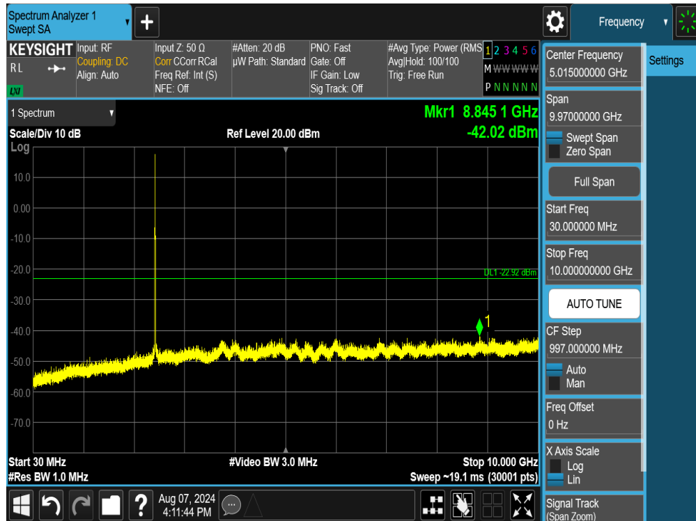
Plot 7-95. Conducted Spurious Plot SISO ANT2 (802.11ax/be OFDMA – 26 Tones – Ch. 6)
