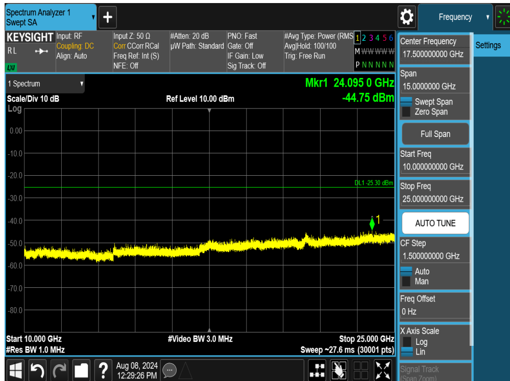
Plot 7-124. Conducted Spurious Plot MIMO ANT2 (802.11ax/be OFDMA – 242 Tones – Ch. 1)
