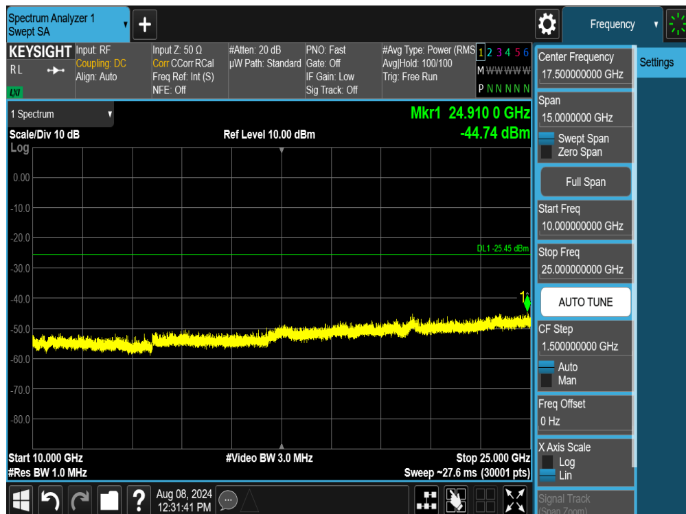
Plot 7-128. Conducted Spurious Plot MIMO ANT2 (802.11ax/be OFDMA – 242 Tones – Ch. 11)
