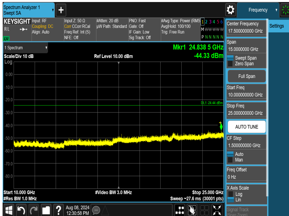
Plot 7-126. Conducted Spurious Plot MIMO ANT2 (802.11ax/be OFDMA – 242 Tones – Ch. 6)
