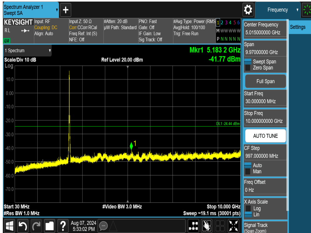
Plot 7-125. Conducted Spurious Plot MIMO ANT2 (802.11ax/be OFDMA – 242 Tones – Ch. 6)
