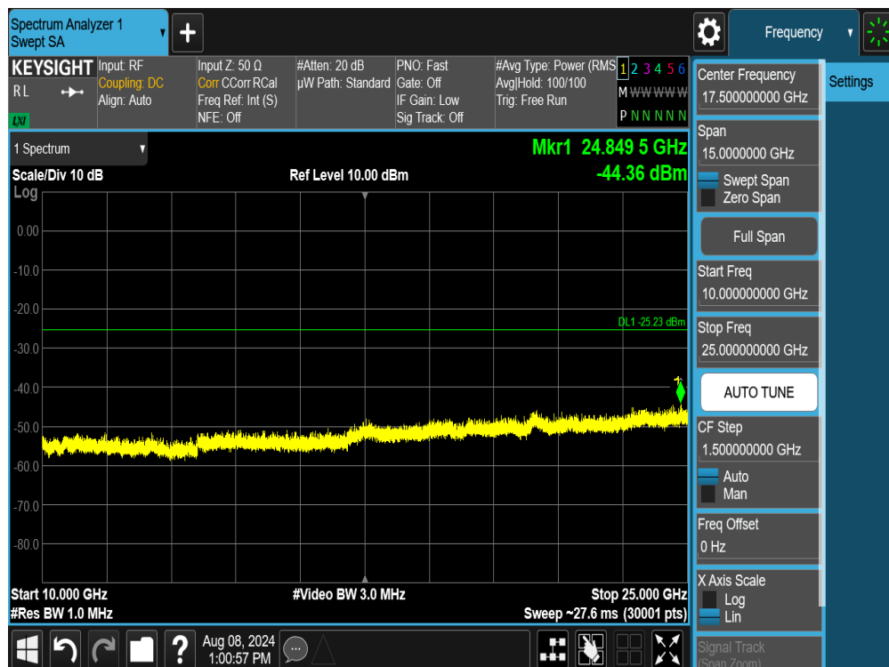
Plot 7-114. Conducted Spurious Plot MIMO ANT1 (802.11ax/be OFDMA – 242 Tones – Ch. 6)
