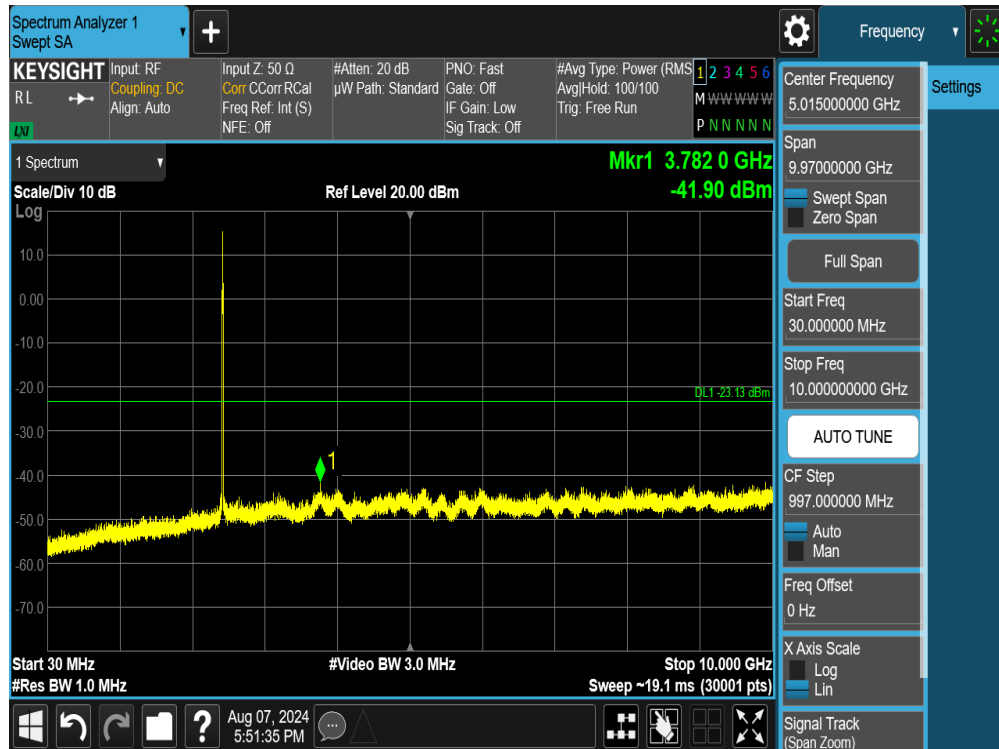
Plot 7-107. Conducted Spurious Plot MIMO ANT1 (802.11ax/be OFDMA – 26 Tones – Ch. 6)
