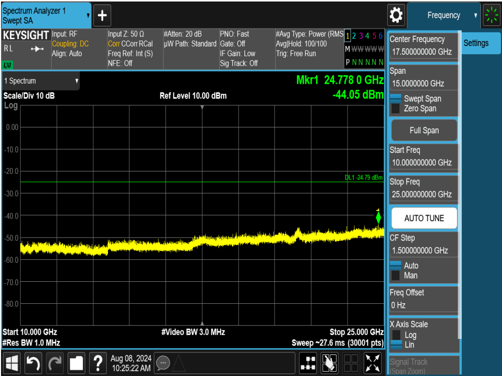
Plot 7-92. Conducted Spurious Plot SISO ANT1 (802.11ax/be OFDMA – 242 Tones – Ch. 11)
