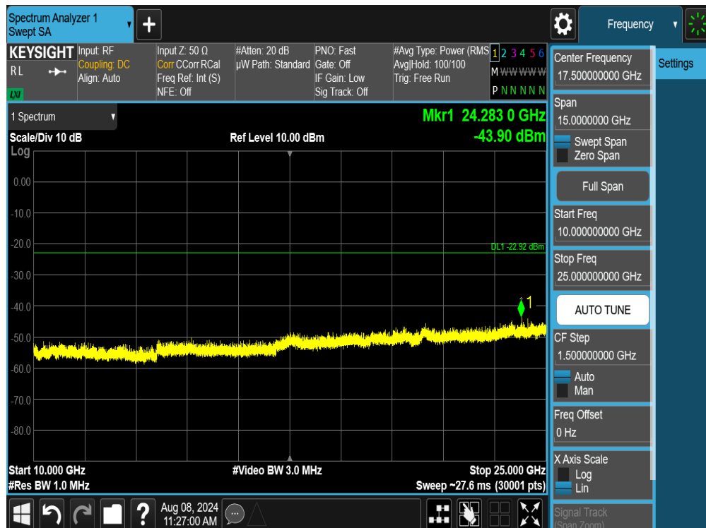
Plot 7-96. Conducted Spurious Plot SISO ANT2 (802.11ax/be OFDMA – 26 Tones – Ch. 6)
