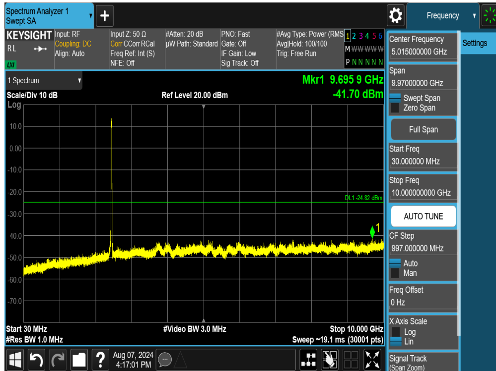
Plot 7-103. Conducted Spurious Plot SISO ANT2 (802.11ax/be OFDMA – 242 Tones – Ch. 11)
