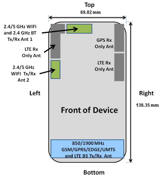
Figure 1-1 DUT Antenna Locations
