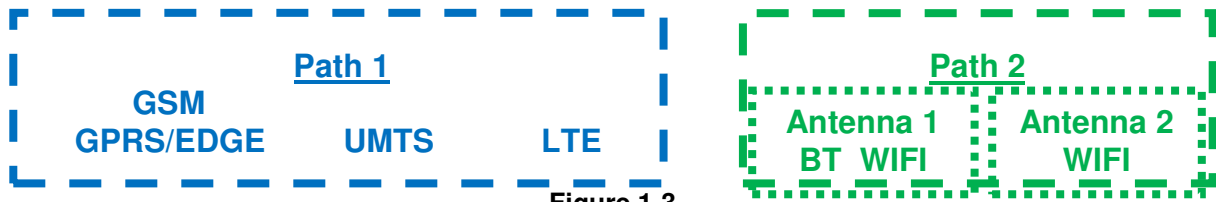
Figure 1-3 Simultaneous Transmission Paths
