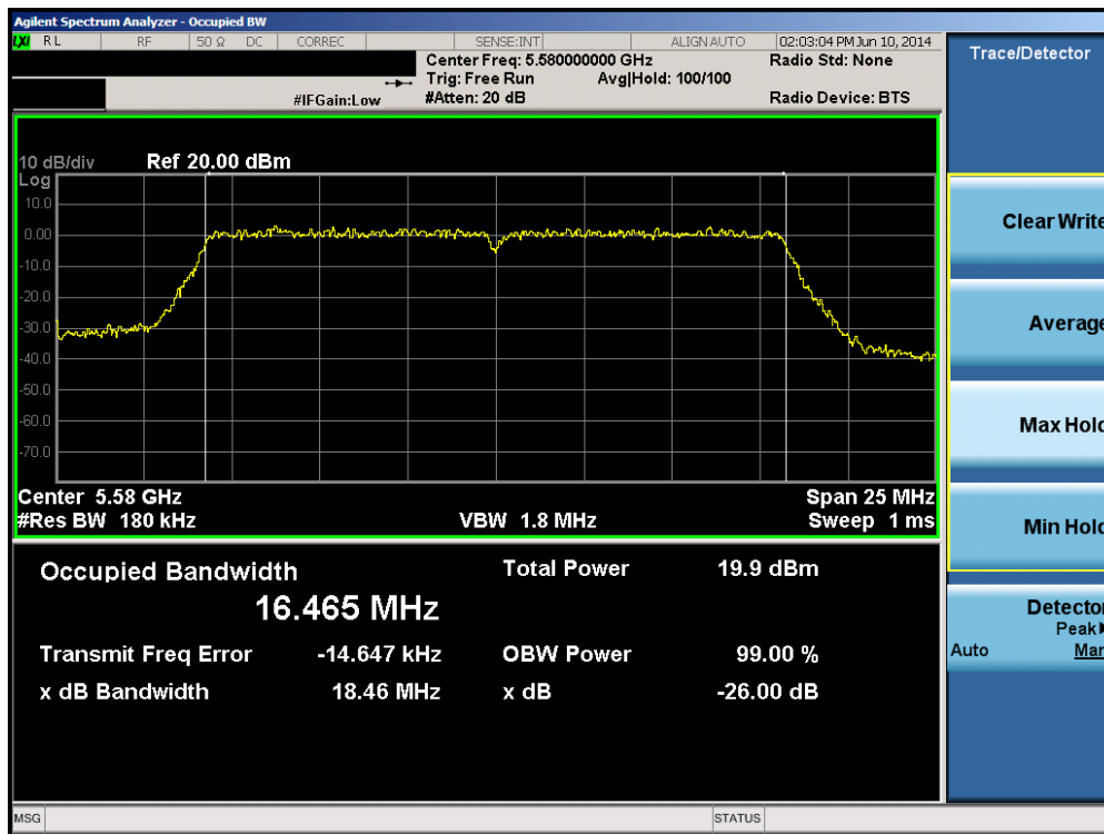
Plot 6-44. 26dB Bandwidth Plot (802.11a (UNII Band 2C) – Ch. 116)
