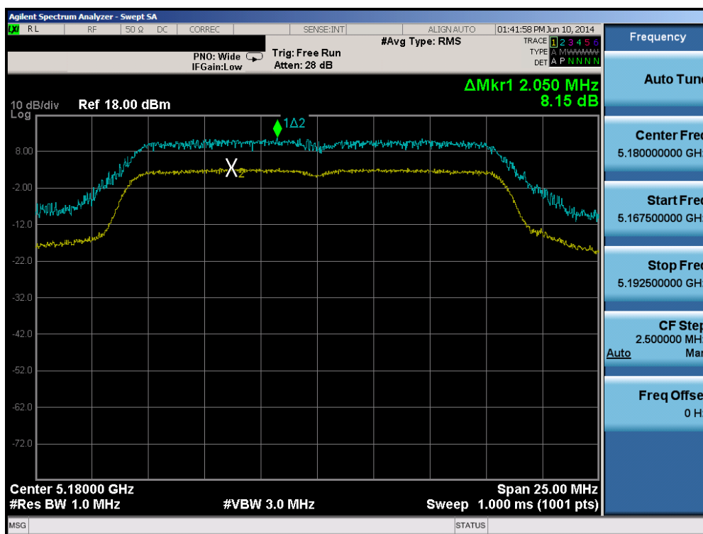
Plot 6-107. Peak Excursion Ratio Plot (802.11a (UNII Band 1) – Ch. 36)
