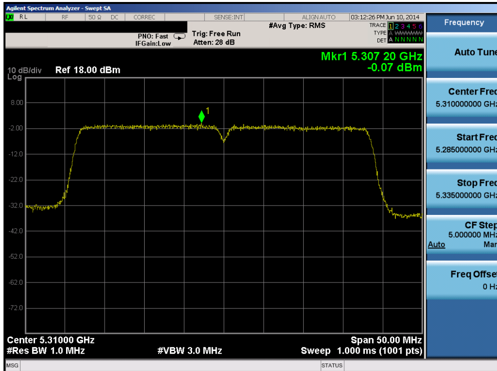
Plot 6-94. Peak Power Spectral Density Plot (40MHz BW 802.11n (UNII Band 2A) – Ch. 62)
