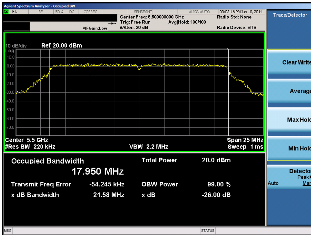
Plot 6-46. 26dB Bandwidth Plot (20MHz BW 802.11n (UNII Band 2C) – Ch. 100)
