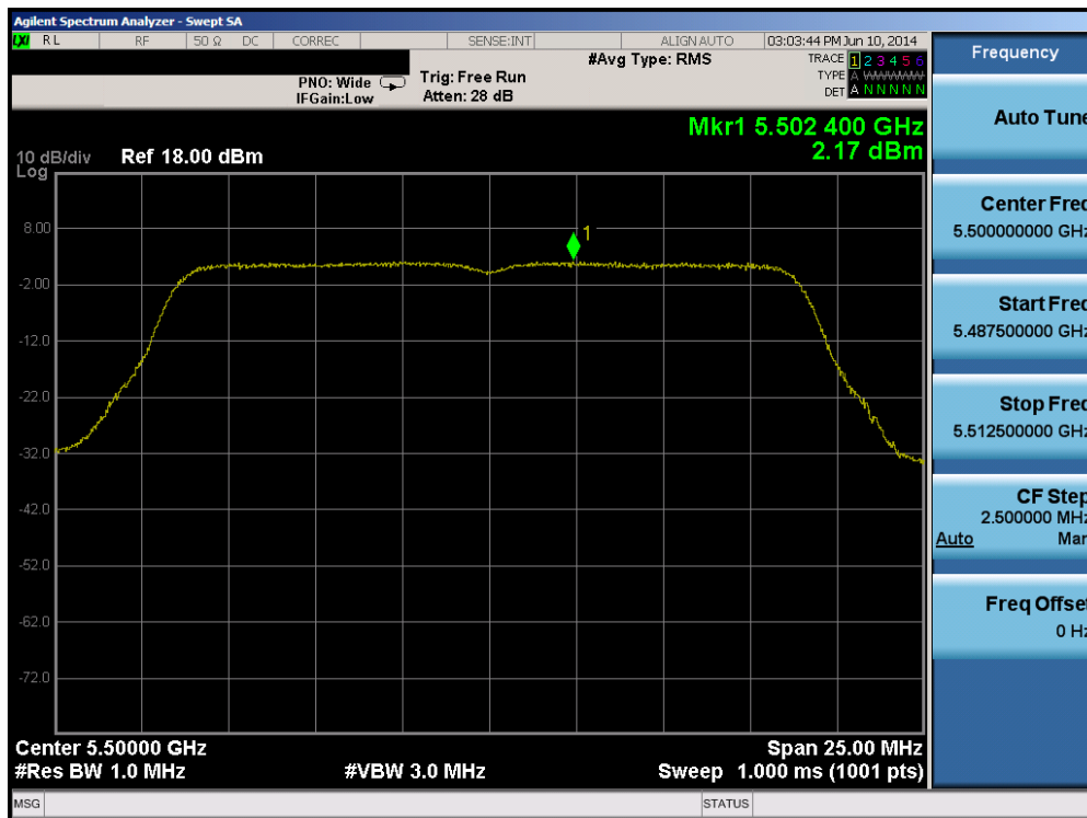
Plot 6-98. Peak Power Spectral Density Plot (20MHz BW 802.11n (UNII Band 2C) – Ch. 100)
