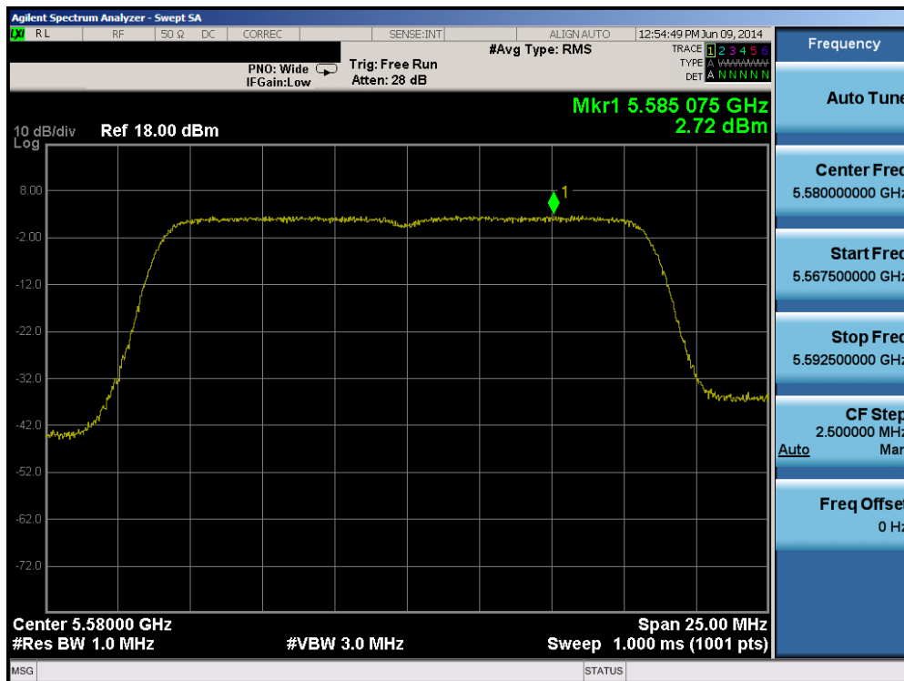
Plot 6-71. Peak Power Spectral Density Plot (802.11a (UNII Band 2C) – Ch. 116)
