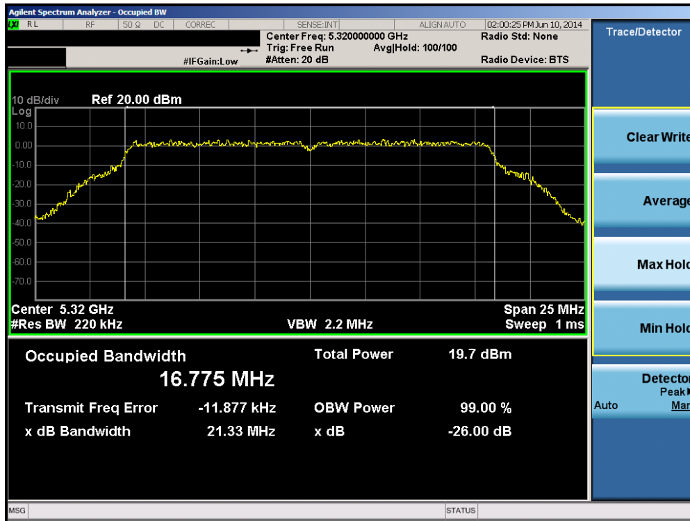
Plot 6-37. 26dB Bandwidth Plot (802.11a (UNII Band 2A) – Ch. 64)
