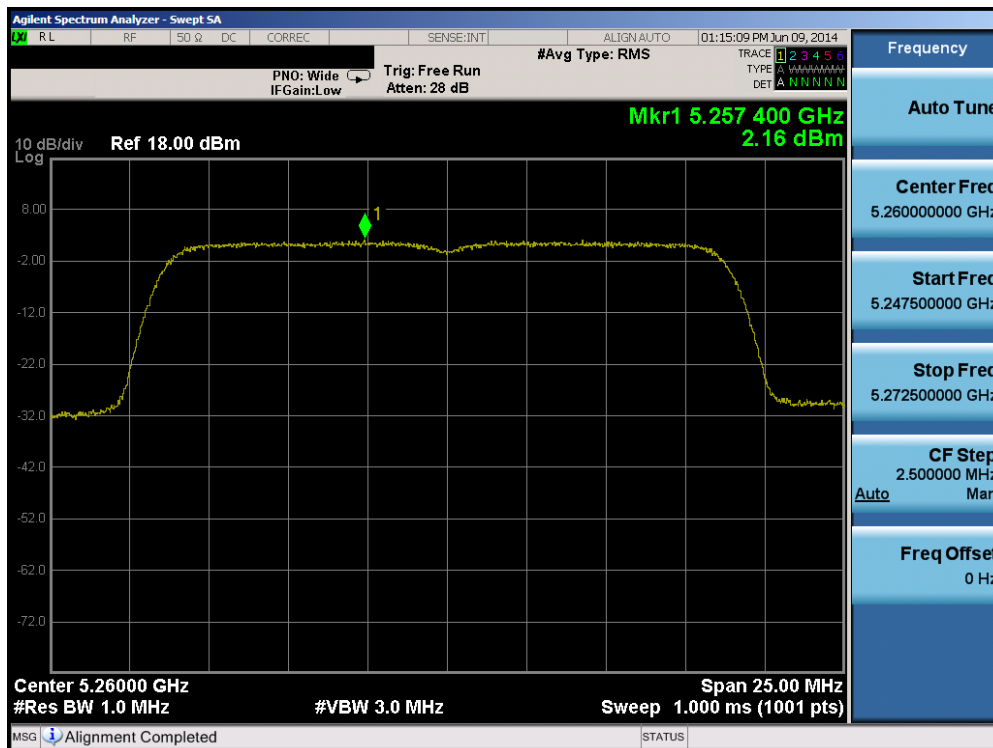
Plot 6-65. Peak Power Spectral Density Plot (20MHz BW 802.11n (UNII Band 2A) – Ch. 52)
