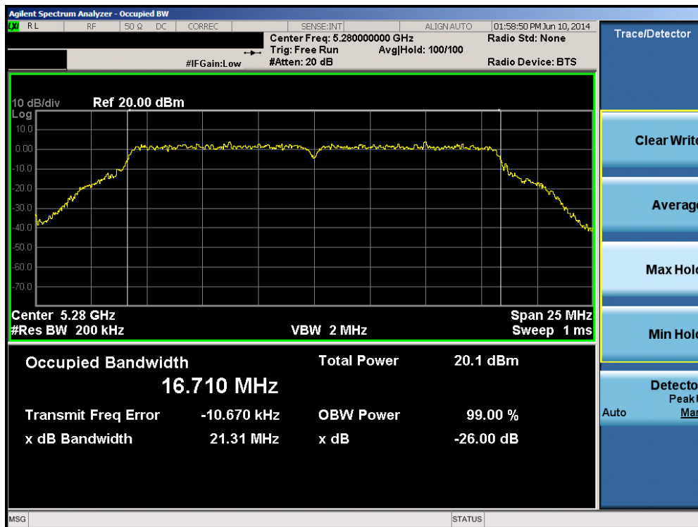
Plot 6-36. 26dB Bandwidth Plot (802.11a (UNII Band 2A) – Ch. 56)
