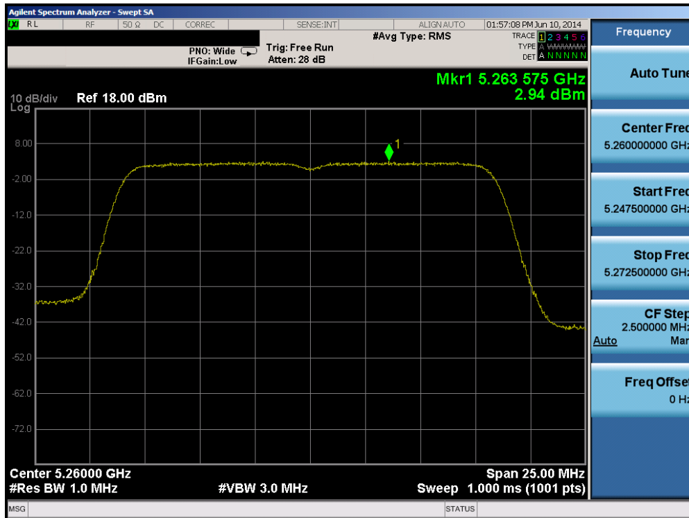
Plot 6-87. Peak Power Spectral Density Plot (802.11a (UNII Band 2A) – Ch. 52)
