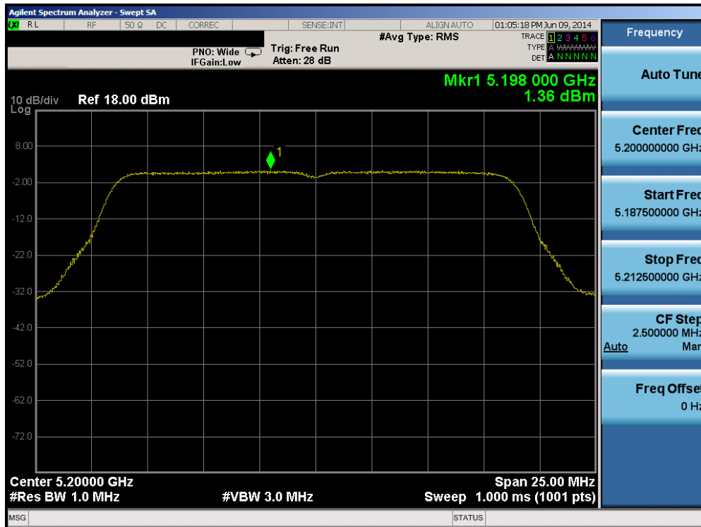
Plot 6-58. Peak Power Spectral Density Plot (20MHz BW 802.11n (UNII Band 1) – Ch. 40)
