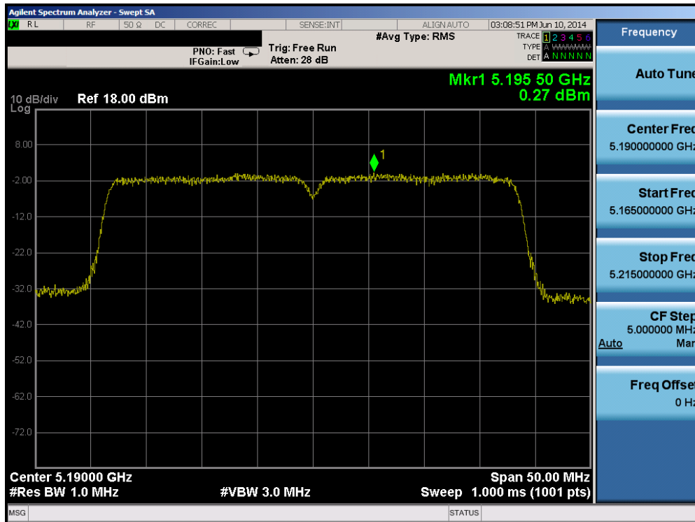
Plot 6-85. Peak Power Spectral Density Plot (40MHz BW 802.11n (UNII Band 1) – Ch. 38)
