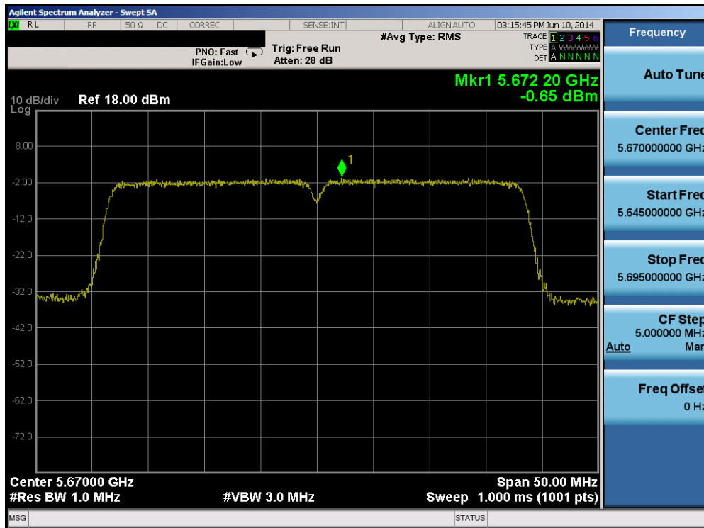
Plot 6-103. Peak Power Spectral Density Plot (40MHz BW 802.11n (UNII Band 2C) – Ch. 134)
