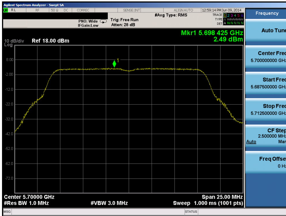
Plot 6-72. Peak Power Spectral Density Plot (802.11a (UNII Band 2C) – Ch. 140)
