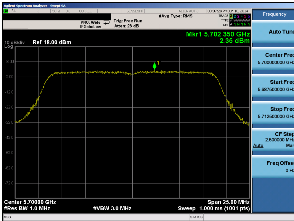
Plot 6-100. Peak Power Spectral Density Plot (20MHz BW 802.11n (UNII Band 2C) – Ch. 140)
