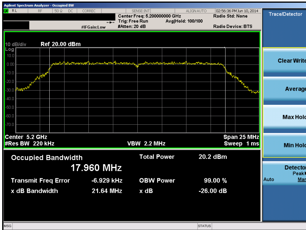
Plot 6-31. 26dB Bandwidth Plot (20MHz BW 802.11n (UNII Band 1) – Ch. 40)
