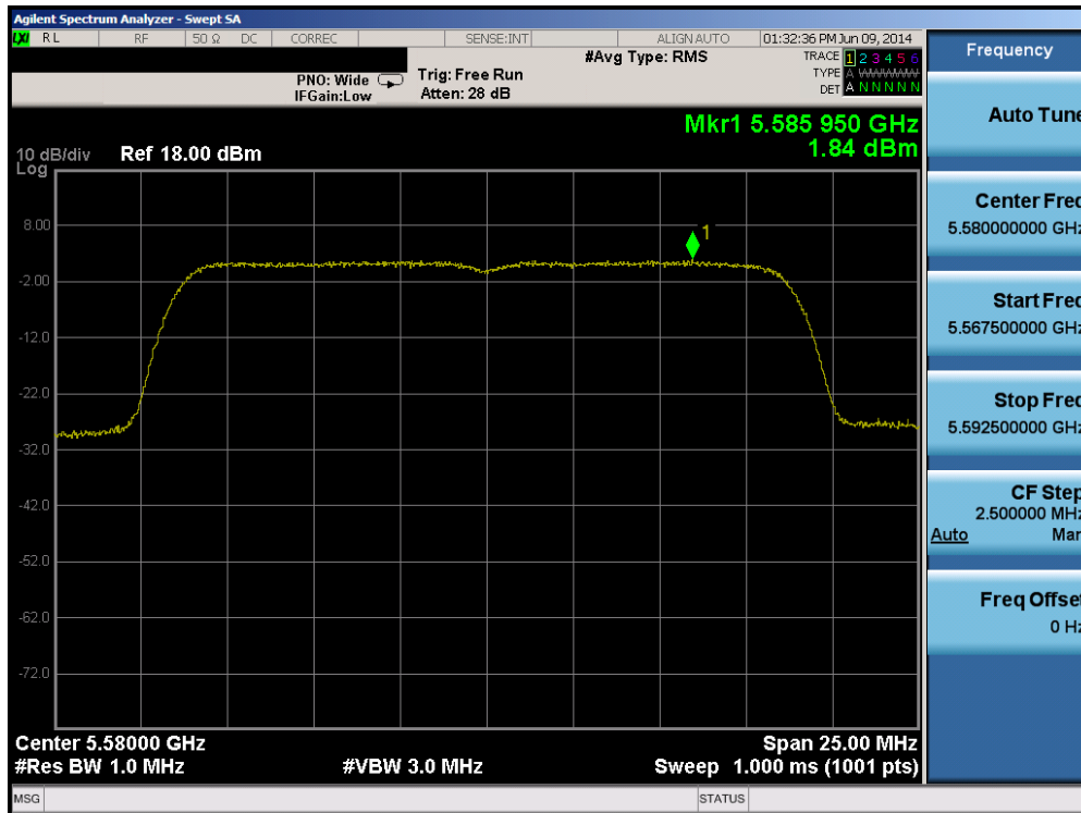
Plot 6-74. Peak Power Spectral Density Plot (20MHz BW 802.11n (UNII Band 2C) – Ch. 116)
