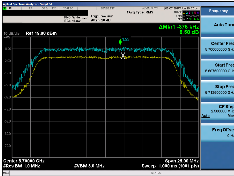
Plot 6-108. Peak Excursion Ratio Plot (20MHz BW 802.11n (UNII Band 2C) – Ch. 140)
