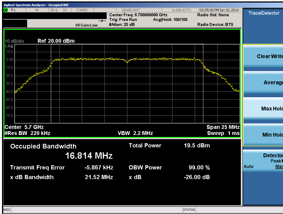
Plot 6-45. 26dB Bandwidth Plot (802.11a (UNII Band 2C) – Ch. 140)
