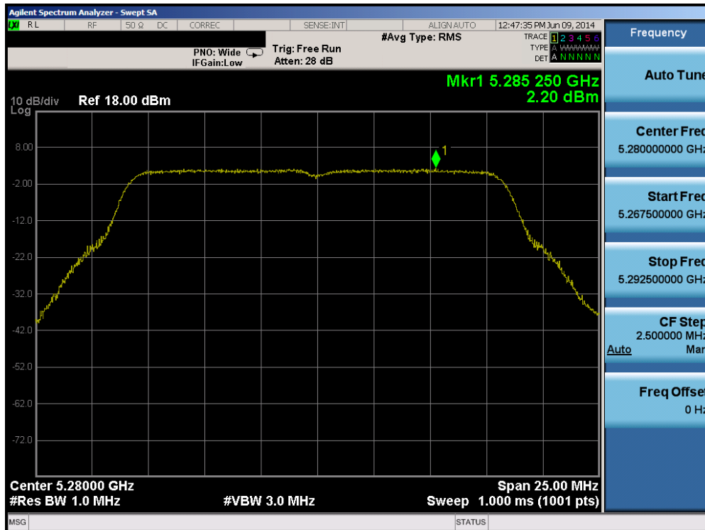
Plot 6-63. Peak Power Spectral Density Plot (802.11a (UNII Band 2A) – Ch. 56)
