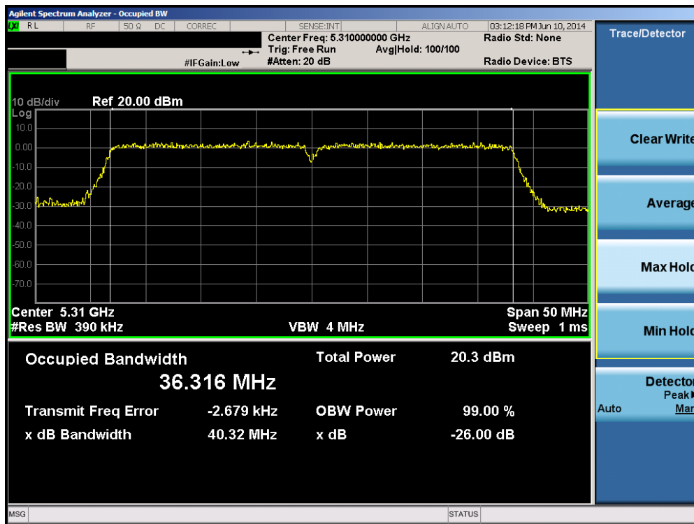
Plot 6-42. 26dB Bandwidth Plot (40MHz BW 802.11n (UNII Band 2A) – Ch. 62)
