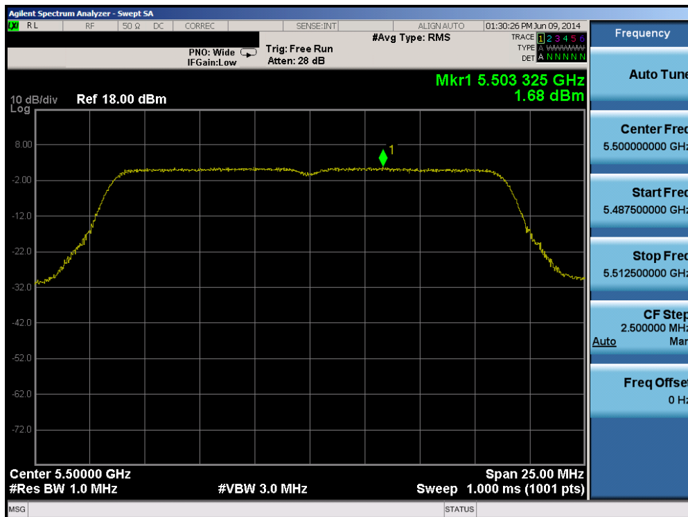
Plot 6-73. Peak Power Spectral Density Plot (20MHz BW 802.11n (UNII Band 2C) – Ch. 100)
