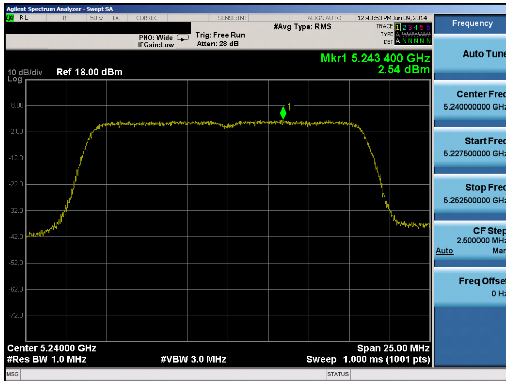
Plot 6-56. Peak Power Spectral Density Plot (802.11a (UNII Band 1) – Ch. 48)
