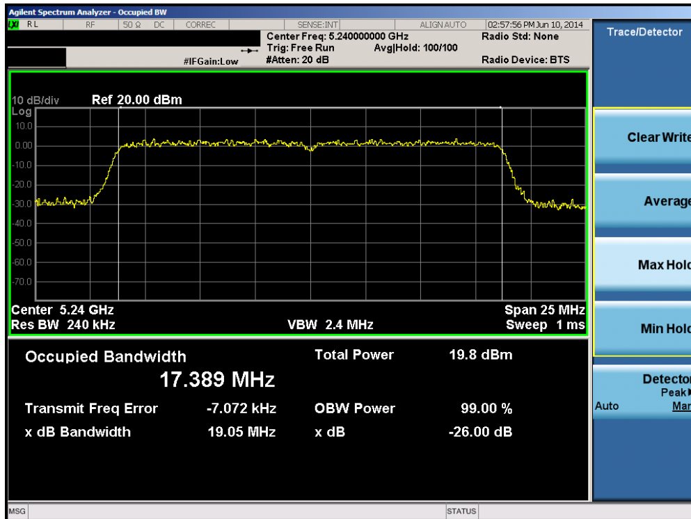
Plot 6-32. 26dB Bandwidth Plot (20MHz BW 802.11n (UNII Band 1) – Ch. 48)
