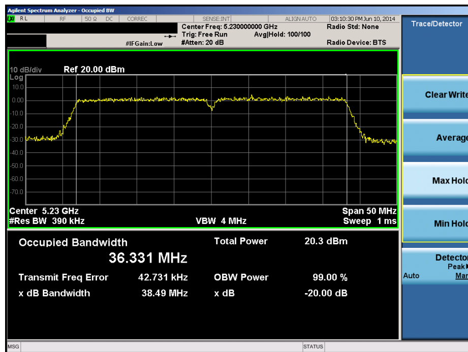
Plot 6-52. 20dB Bandwidth Plot (40MHz BW 802.11n (UNII Band 1) – Ch. 46)
