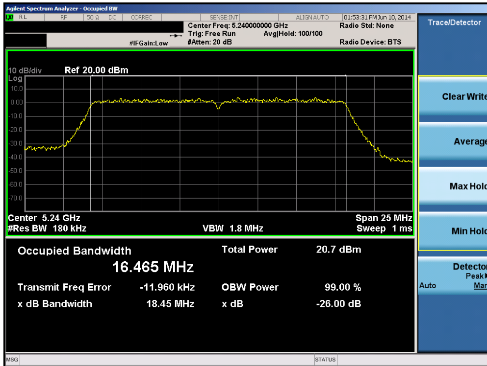
Plot 6-29. 26dB Bandwidth Plot (802.11a (UNII Band 1) – Ch. 48)
