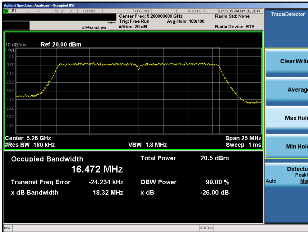
Plot 6-35. 26dB Bandwidth Plot (802.11a (UNII Band 2A) – Ch. 52)
