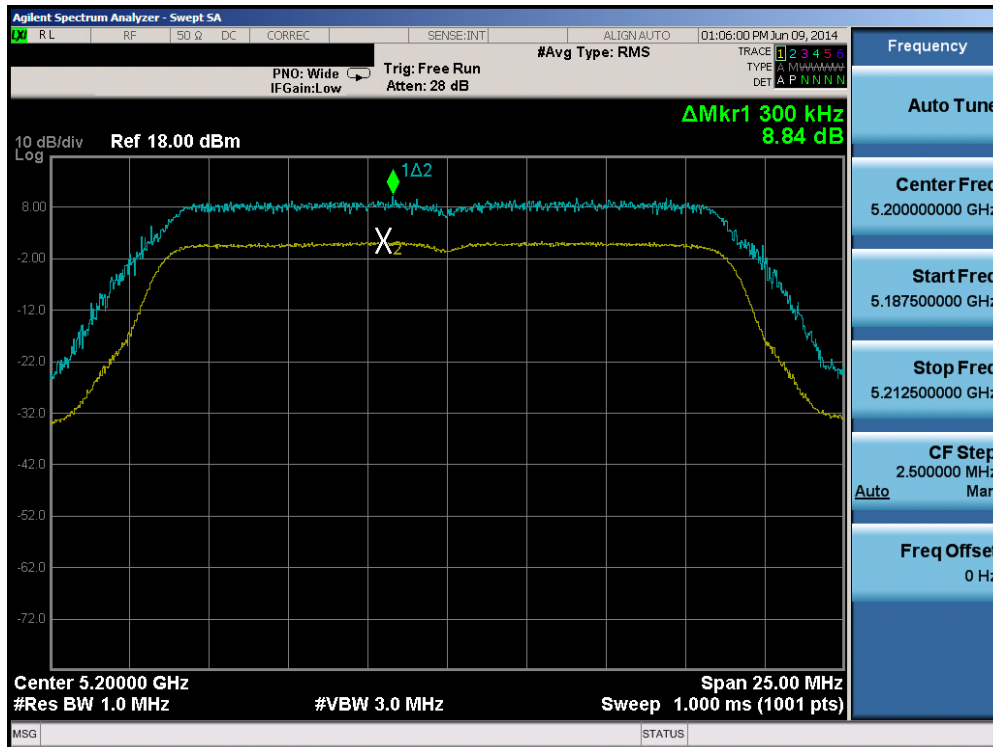
Plot 6-105. Peak Excursion Ratio Plot (20MHz BW 802.11n (UNII Band 1) – Ch. 40)
