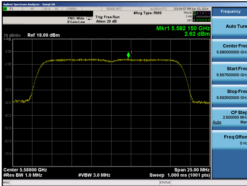
Plot 6-99. Peak Power Spectral Density Plot (20MHz BW 802.11n (UNII Band 2C) – Ch. 116)
