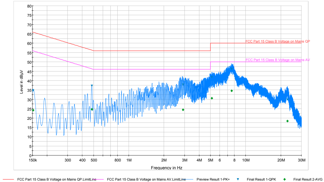
Plot 6-155. Line Conducted Plot with 802.11a UNII Band 2A (N)
