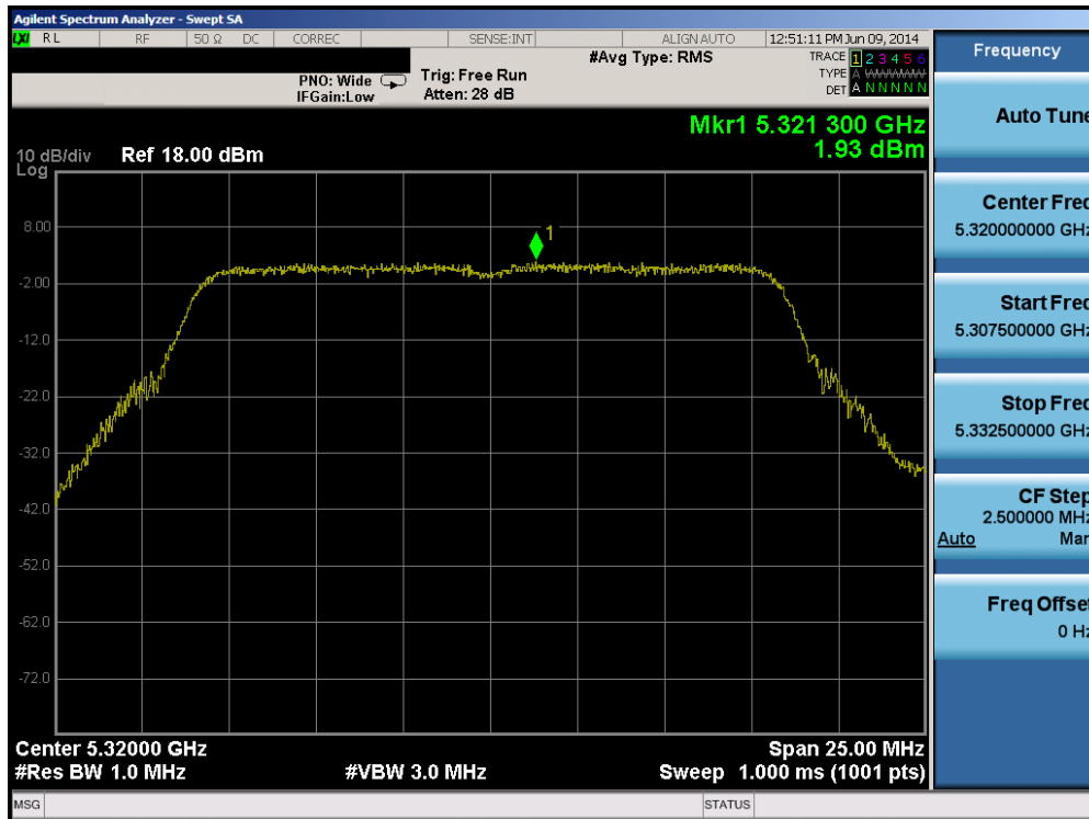
Plot 6-64. Peak Power Spectral Density Plot (802.11a (UNII Band 2A) – Ch. 64)
