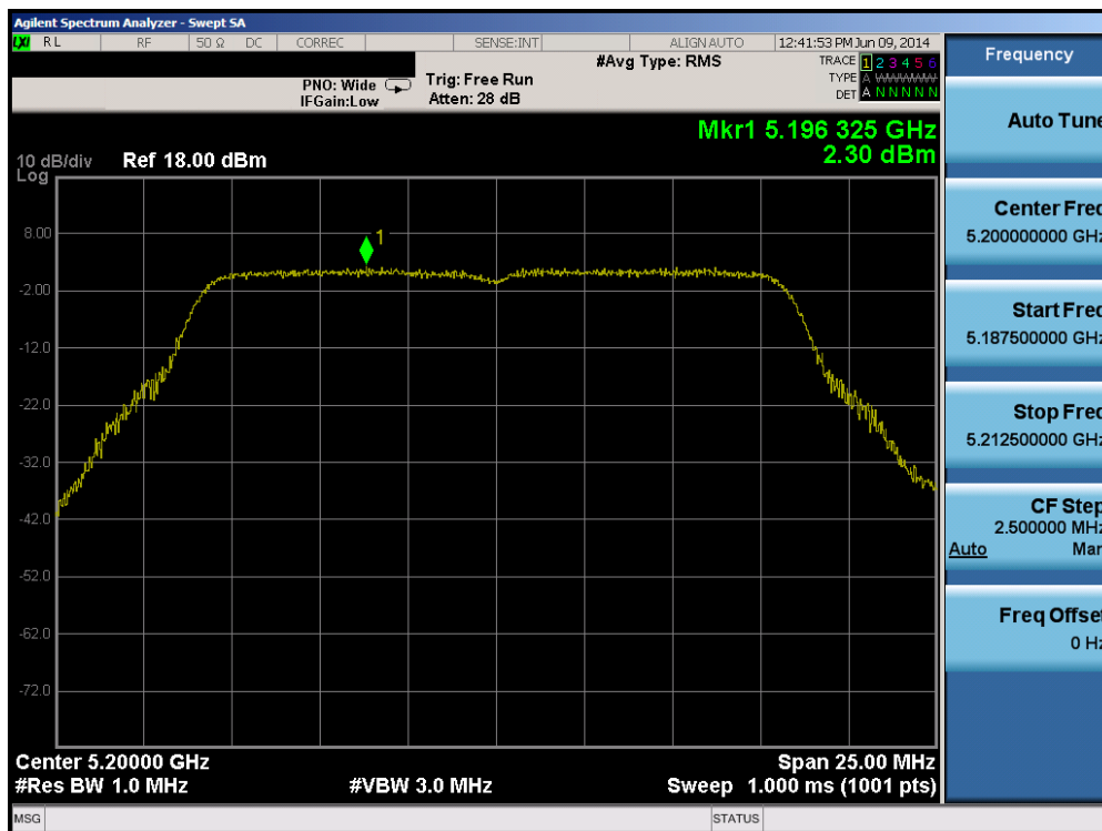
Plot 6-55. Peak Power Spectral Density Plot (802.11a (UNII Band 1) – Ch. 40)
