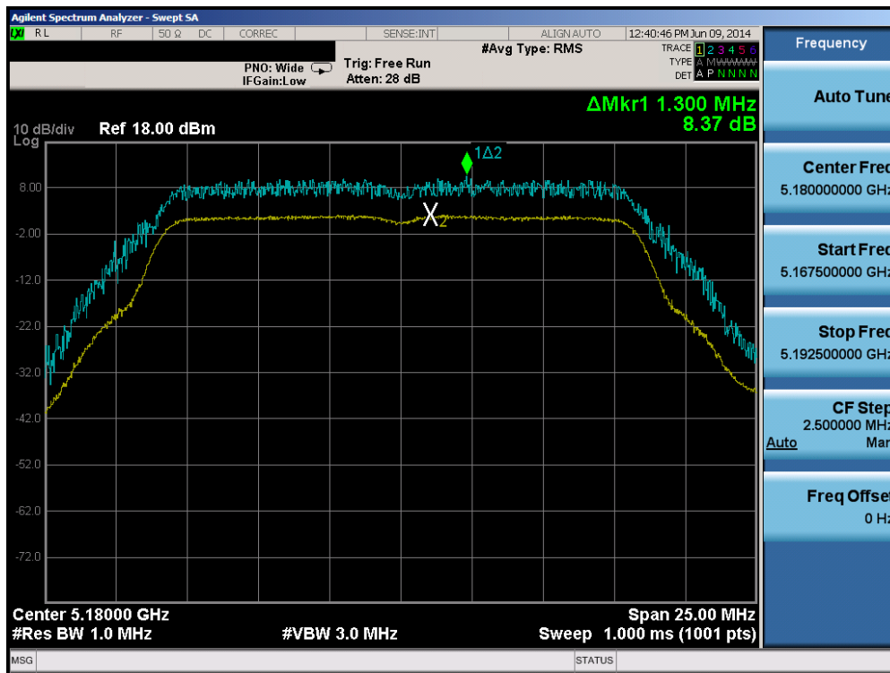
Plot 6-104. Peak Excursion Ratio Plot (802.11a (UNII Band 1) – Ch. 36)
