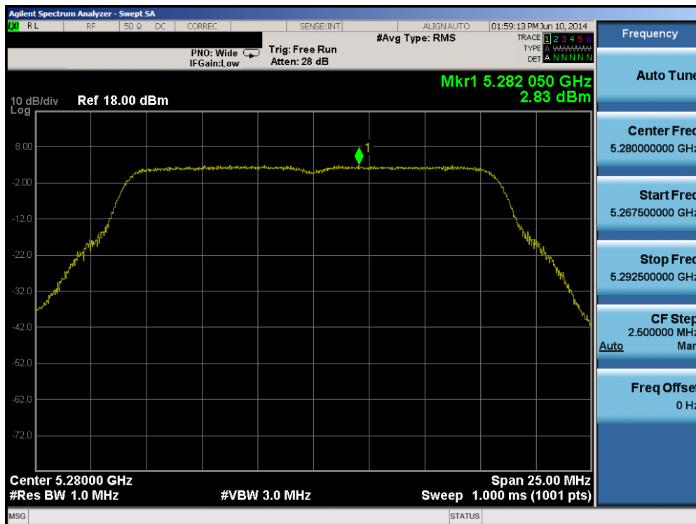
Plot 6-88. Peak Power Spectral Density Plot (802.11a (UNII Band 2A) – Ch. 56)
