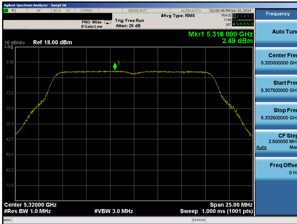
Plot 6-89. Peak Power Spectral Density Plot (802.11a (UNII Band 2A) – Ch. 64)
