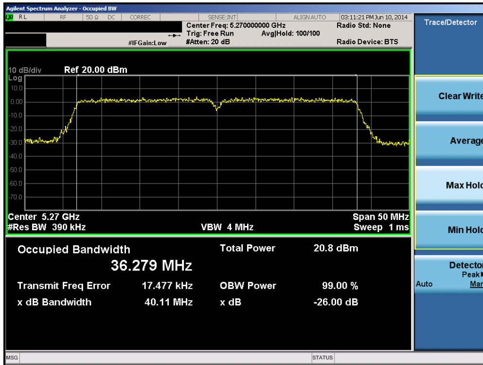
Plot 6-41. 26dB Bandwidth Plot (40MHz BW 802.11n (UNII Band 2A) – Ch. 54)
