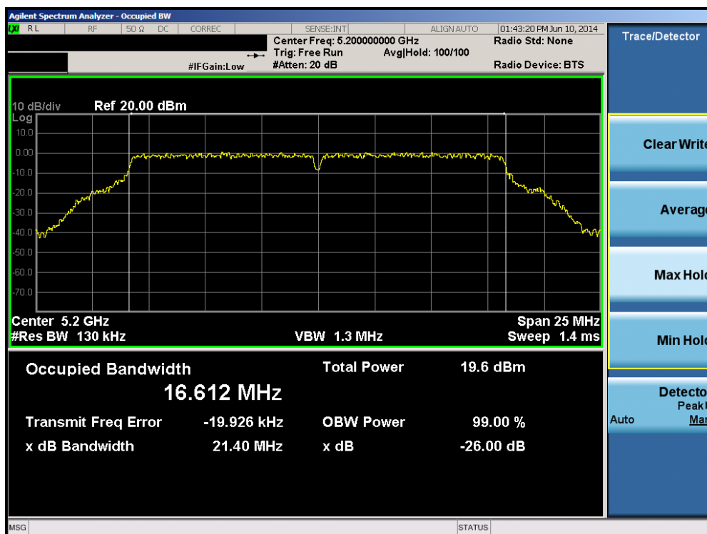
Plot 6-28. 26dB Bandwidth Plot (802.11a (UNII Band 1) – Ch. 40)
