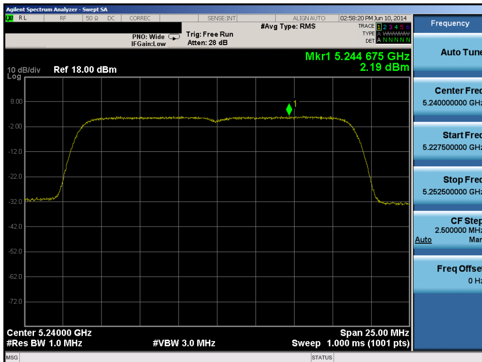
Plot 6-84. Peak Power Spectral Density Plot (20MHz BW 802.11n (UNII Band 1) – Ch. 48)
