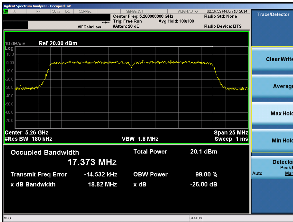
Plot 6-38. 26dB Bandwidth Plot (20MHz BW 802.11n (UNII Band 2A) – Ch. 52)
