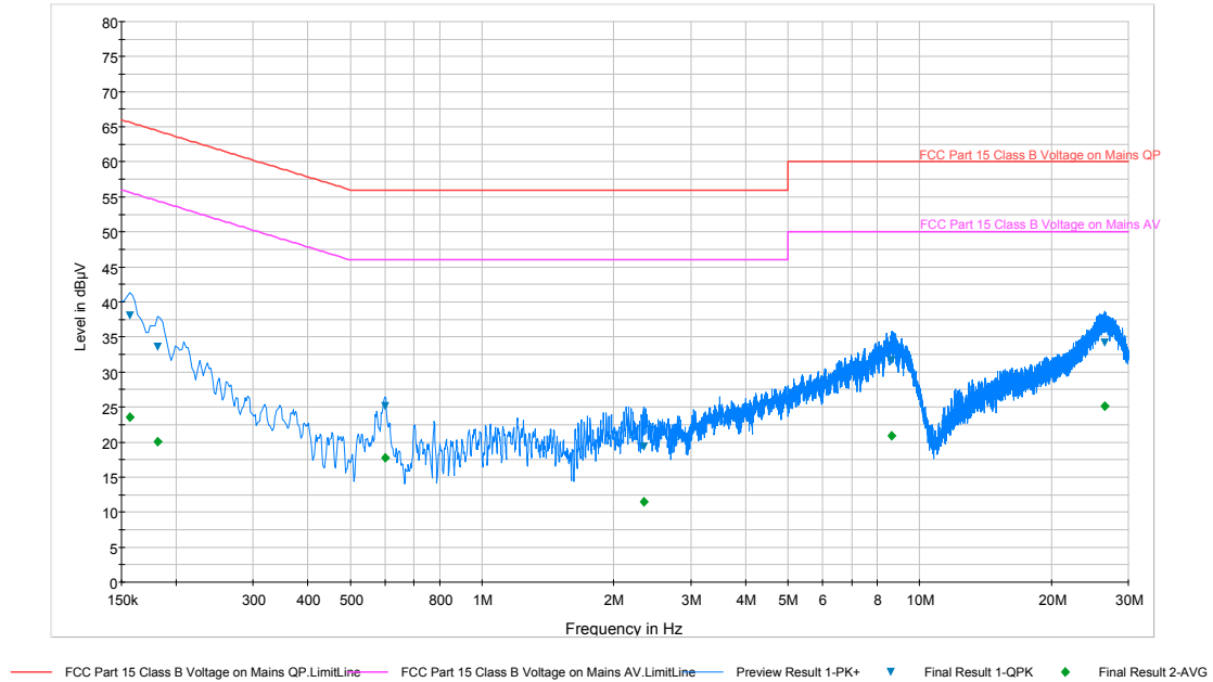
Plot 6-156. Line Conducted Plot with 802.11a UNII Band 2C (L1)
