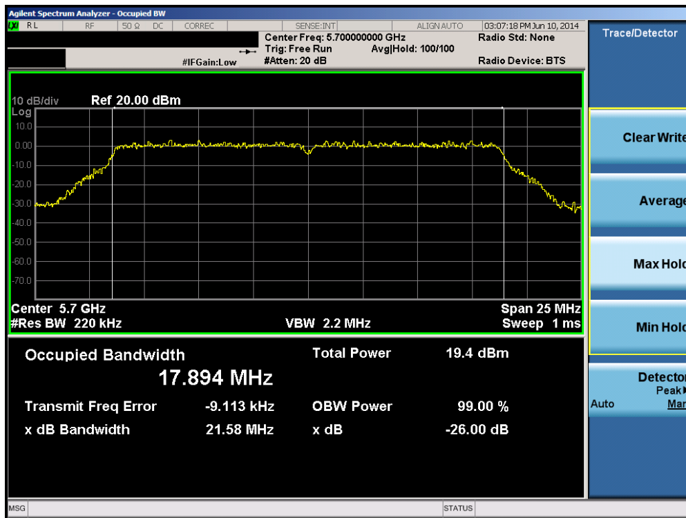
Plot 6-48. 26dB Bandwidth Plot (20MHz BW 802.11n (UNII Band 2C) – Ch. 140)
