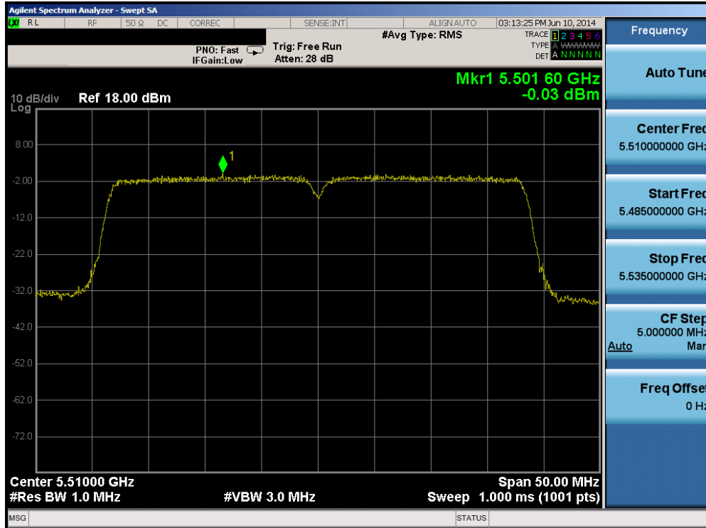
Plot 6-101. Peak Power Spectral Density Plot (40MHz BW 802.11n (UNII Band 2C) – Ch. 102)
