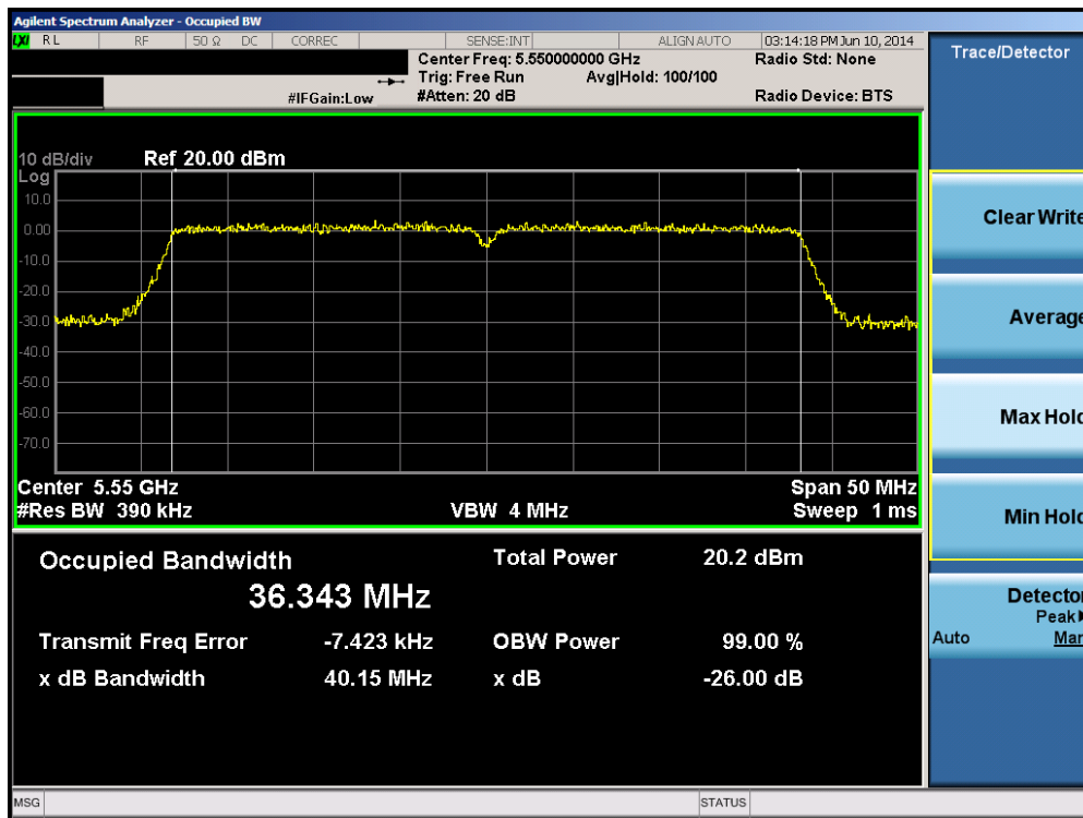
Plot 6-50. 26dB Bandwidth Plot (40MHz BW 802.11n (UNII Band 2C) – Ch. 110)
