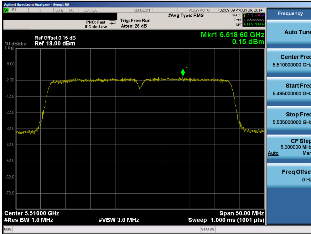
Plot 6-76. Peak Power Spectral Density Plot (40MHz BW 802.11n (UNII Band 2C) – Ch. 102)
