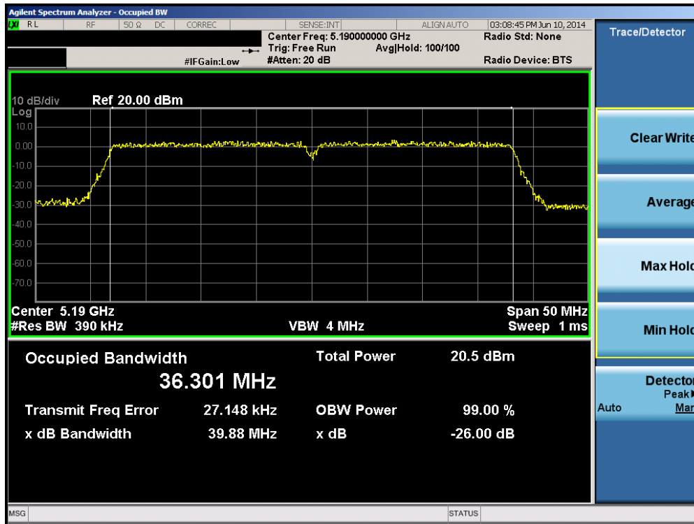
Plot 6-33. 26dB Bandwidth Plot (40MHz BW 802.11n (UNII Band 1) – Ch. 38)
