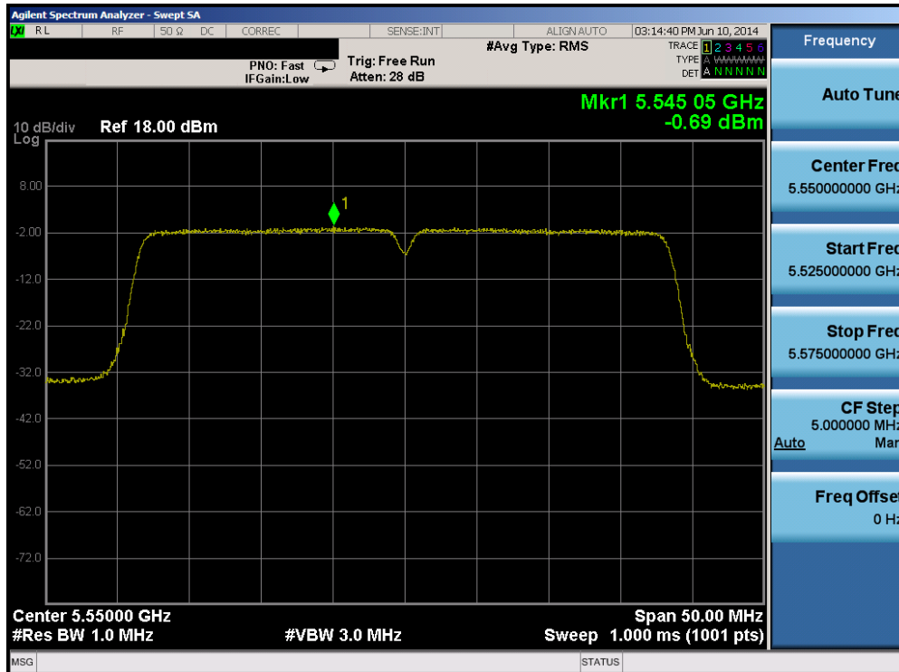
Plot 6-102. Peak Power Spectral Density Plot (40MHz BW 802.11n (UNII Band 2C) – Ch. 110)
