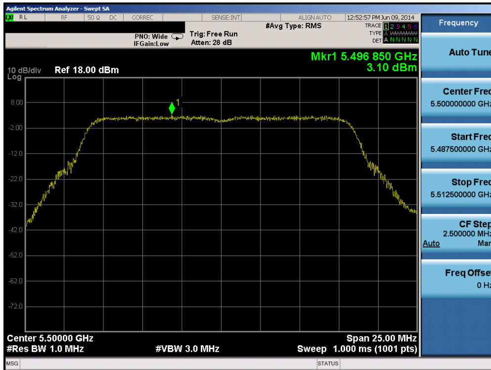
Plot 6-70. Peak Power Spectral Density Plot (802.11a (UNII Band 2C) – Ch. 100)
