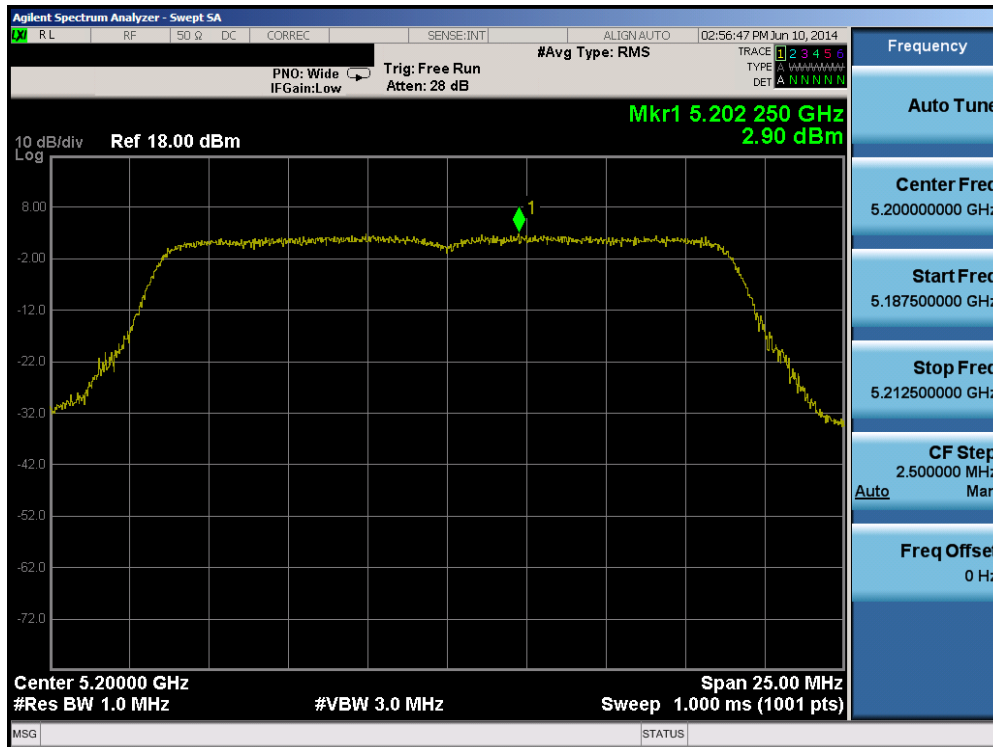
Plot 6-83. Peak Power Spectral Density Plot (20MHz BW 802.11n (UNII Band 1) – Ch. 40)
