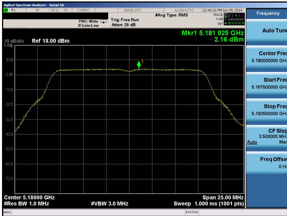
Plot 6-54. Peak Power Spectral Density Plot (802.11a (UNII Band 1) – Ch. 36)
