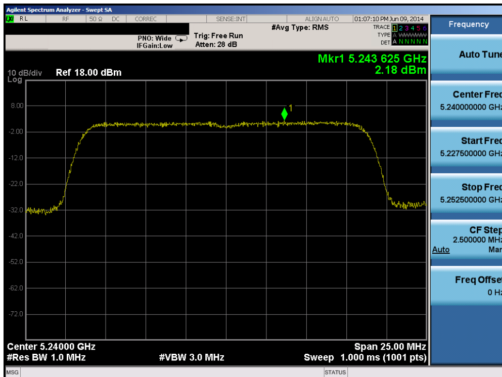
Plot 6-59. Peak Power Spectral Density Plot (20MHz BW 802.11n (UNII Band 1) – Ch. 48)
