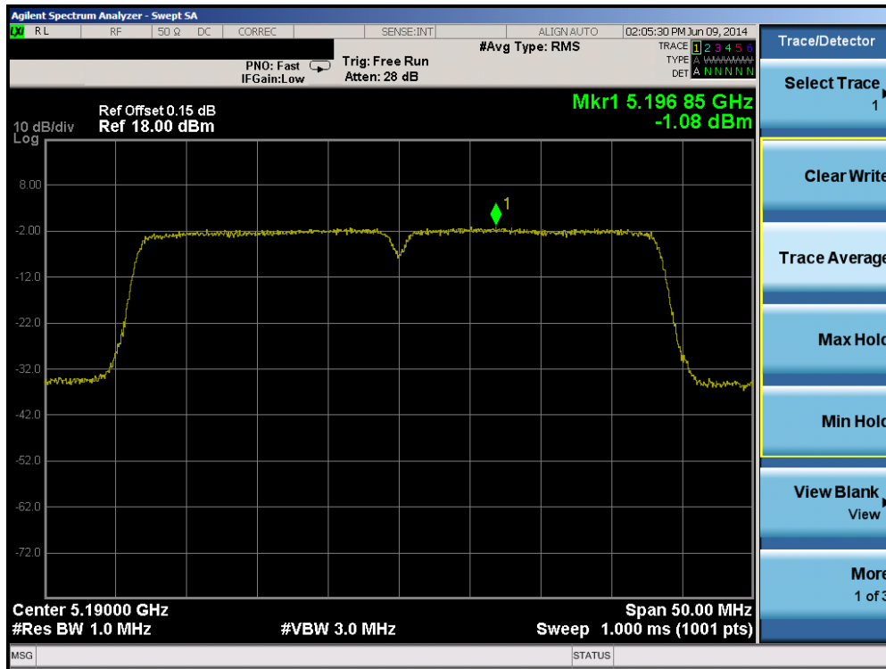
Plot 6-60. Peak Power Spectral Density Plot (40MHz BW 802.11n (UNII Band 1) – Ch. 38)
