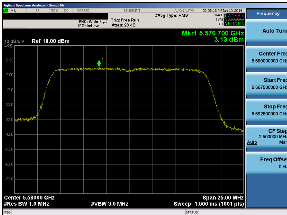
Plot 6-96. Peak Power Spectral Density Plot (802.11a (UNII Band 2C) – Ch. 116)
