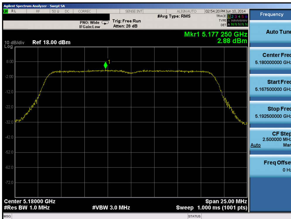
Plot 6-82. Peak Power Spectral Density Plot (20MHz BW 802.11n (UNII Band 1) – Ch. 36)
