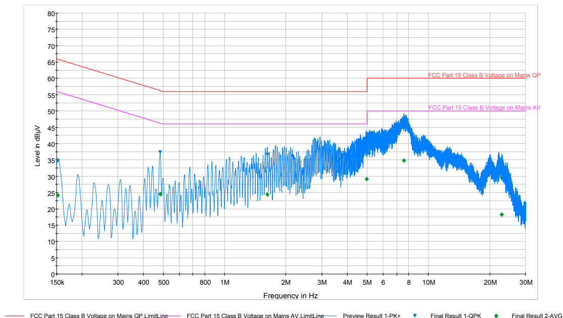
Plot 6-153. Line Conducted Plot with 802.11a UNII Band 1 (N)
