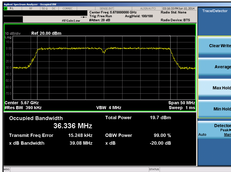
Plot 6-53. 20dB Bandwidth Plot (40MHz BW 802.11n (UNII Band 2C) – Ch. 134)
