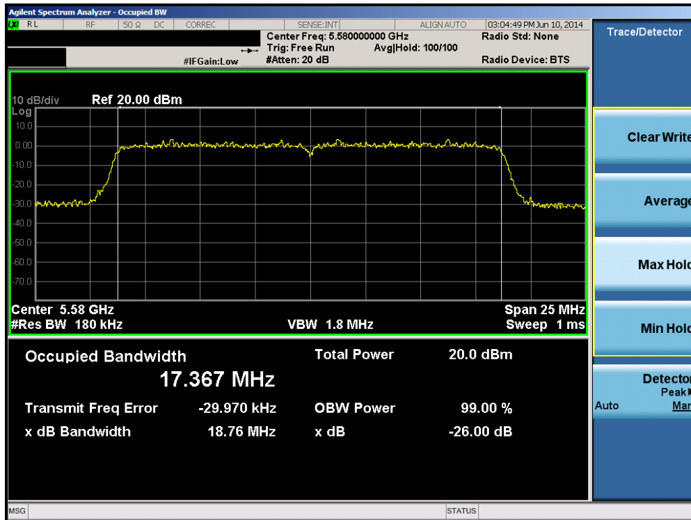
Plot 6-47. 26dB Bandwidth Plot (20MHz BW 802.11n (UNII Band 2C) – Ch. 116)
