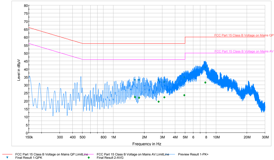
Plot 6-152. Line Conducted Plot with 802.11a UNII Band 1 (L1)
