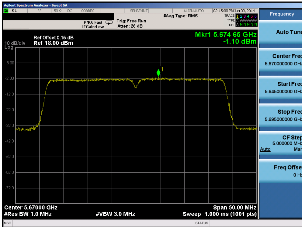
Plot 6-78. Peak Power Spectral Density Plot (40MHz BW 802.11n (UNII Band 2C) – Ch. 134)
