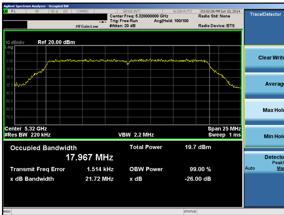
Plot 6-40. 26dB Bandwidth Plot (20MHz BW 802.11n (UNII Band 2A) – Ch. 64)
