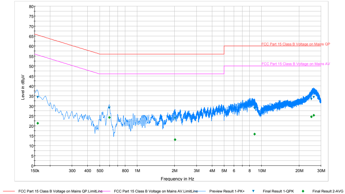
Plot 6-157. Line Conducted Plot with 802.11a UNII Band 2C (N)
