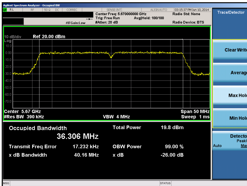
Plot 6-51. 26dB Bandwidth Plot (40MHz BW 802.11n (UNII Band 2C) – Ch. 134)
