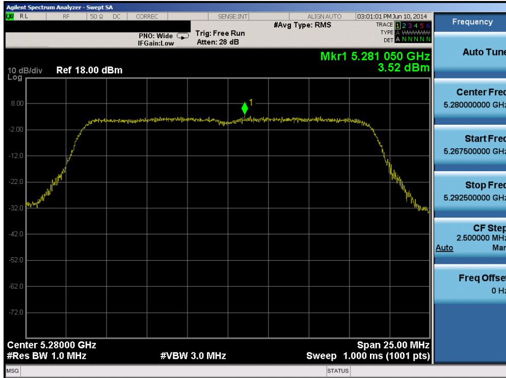
Plot 6-91. Peak Power Spectral Density Plot (20MHz BW 802.11n (UNII Band 2A) – Ch. 56)
