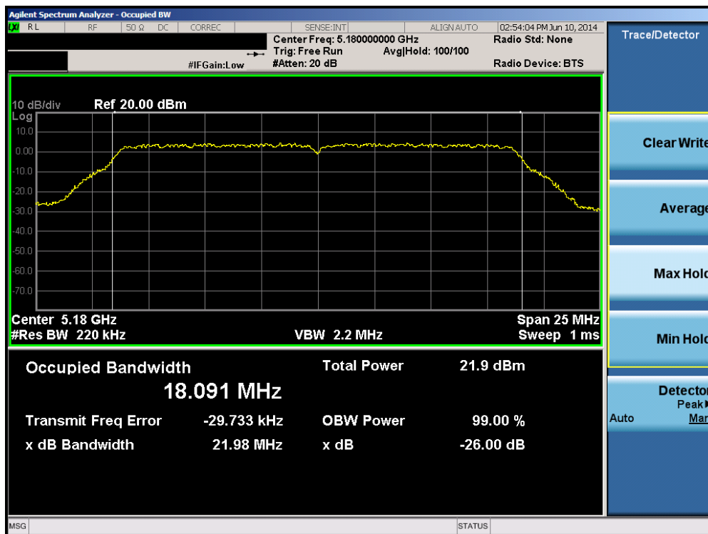
Plot 6-30. 26dB Bandwidth Plot (20MHz BW 802.11n (UNII Band 1) – Ch. 36)
