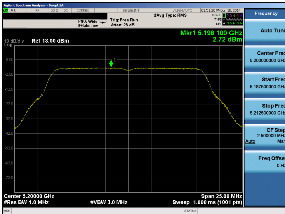
Plot 6-80. Peak Power Spectral Density Plot (802.11a (UNII Band 1) – Ch. 40)
