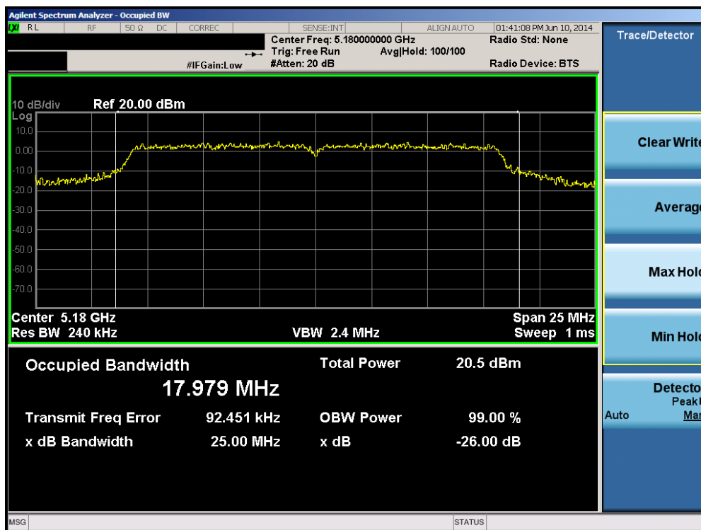
Plot 6-27. 26dB Bandwidth Plot (802.11a (UNII Band 1) – Ch. 36)
