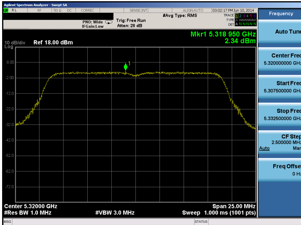
Plot 6-92. Peak Power Spectral Density Plot (20MHz BW 802.11n (UNII Band 2A) – Ch. 64)
