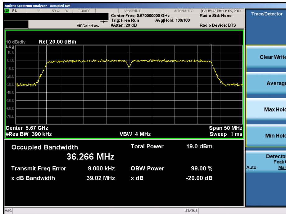
Plot 6-26. 20dB Bandwidth Plot (40MHz BW 802.11n (UNII Band 2C) – Ch. 134)
