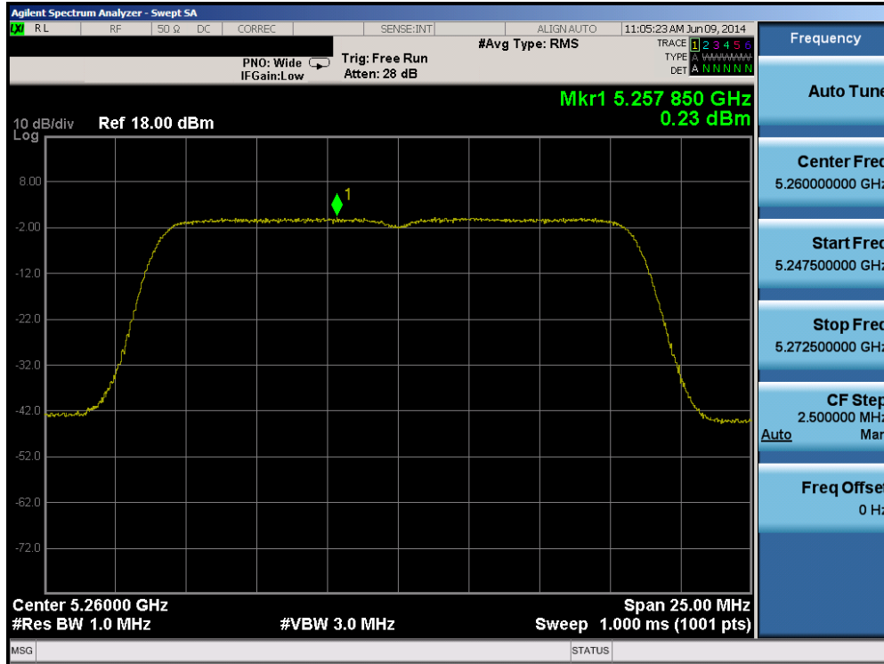
Plot 6-62. Peak Power Spectral Density Plot (802.11a (UNII Band 2A) – Ch. 52)
