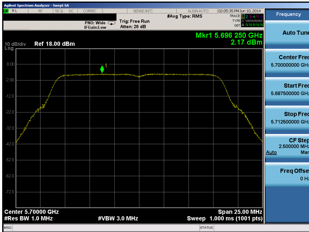
Plot 6-97. Peak Power Spectral Density Plot (802.11a (UNII Band 2C) – Ch. 140)
