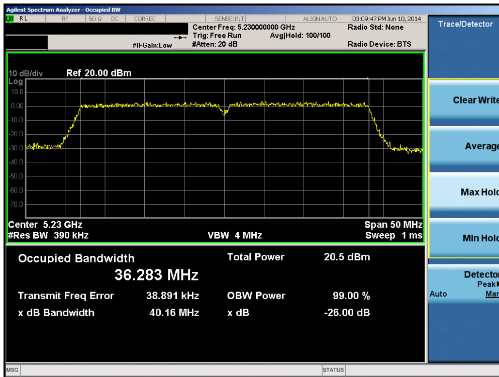
Plot 6-34. 26dB Bandwidth Plot (40MHz BW 802.11n (UNII Band 1) – Ch. 46)
