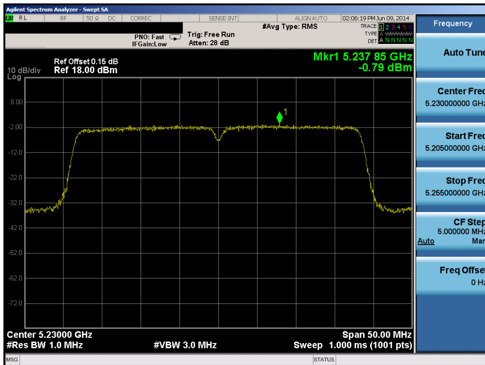
Plot 6-61. Peak Power Spectral Density Plot (40MHz BW 802.11n (UNII Band 1) – Ch. 46)
