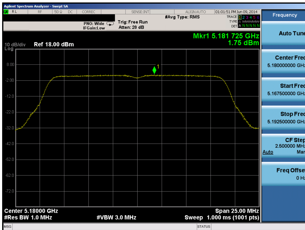
Plot 6-57. Peak Power Spectral Density Plot (20MHz BW 802.11n (UNII Band 1) – Ch. 36)
