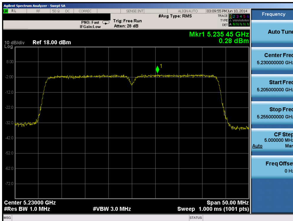
Plot 6-86. Peak Power Spectral Density Plot (40MHz BW 802.11n (UNII Band 1) – Ch. 46)
