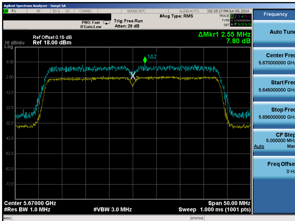
Plot 6-106. Peak Excursion Ratio Plot (40MHz BW 802.11n (UNII Band 2C) – Ch. 134)
