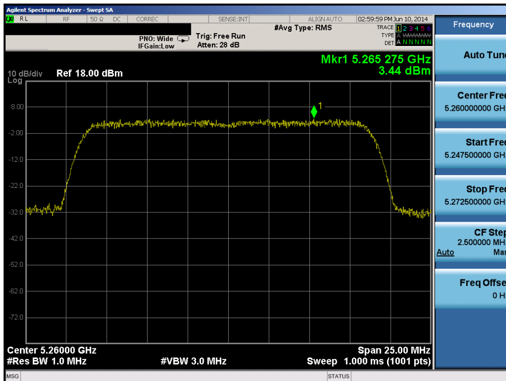
Plot 6-90. Peak Power Spectral Density Plot (20MHz BW 802.11n (UNII Band 2A) – Ch. 52)
