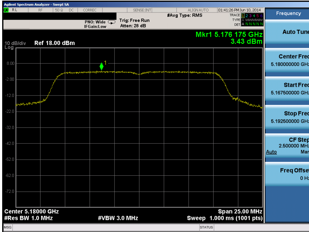
Plot 6-79. Peak Power Spectral Density Plot (802.11a (UNII Band 1) – Ch. 36)
