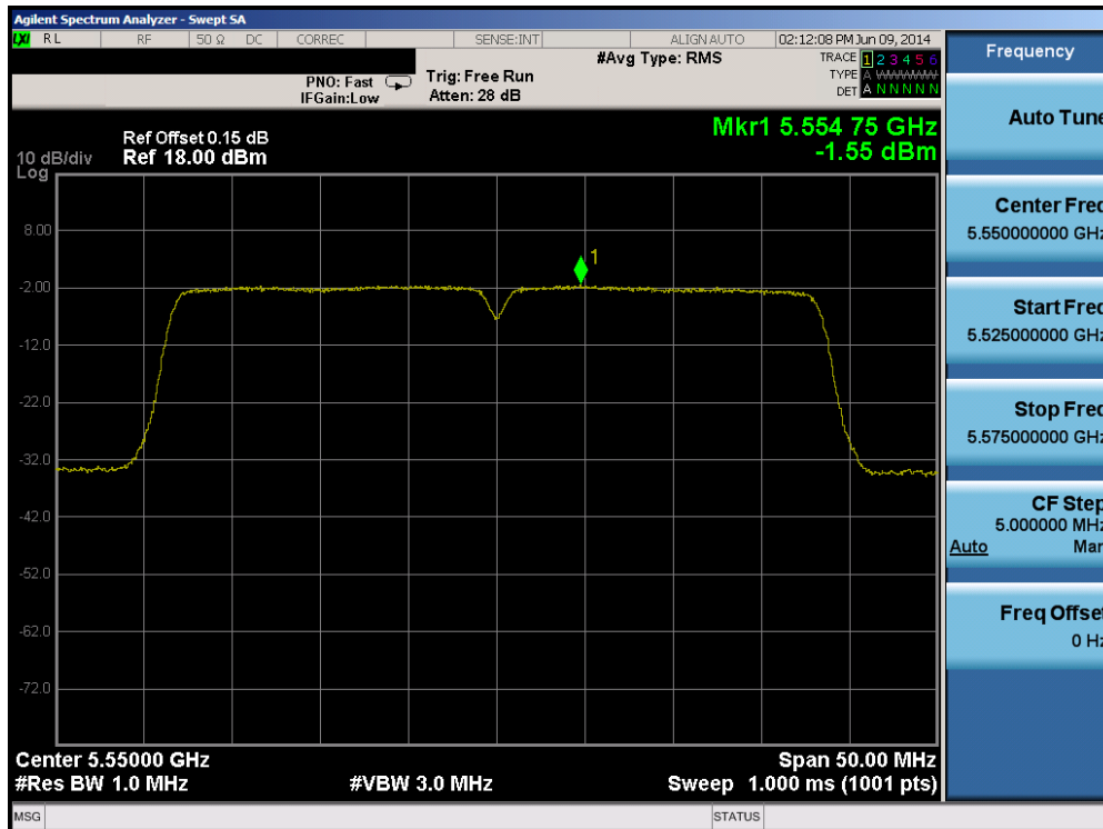
Plot 6-77. Peak Power Spectral Density Plot (40MHz BW 802.11n (UNII Band 2C) – Ch. 110)
