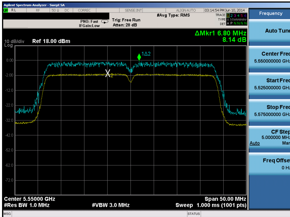
Plot 6-109. Peak Excursion Ratio Plot (40MHz BW 802.11n (UNII Band 2C) – Ch. 110)
