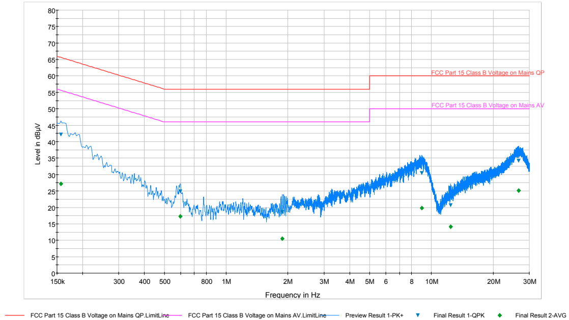
Plot 6-154. Line Conducted Plot with 802.11a UNII Band 2A (L1)
