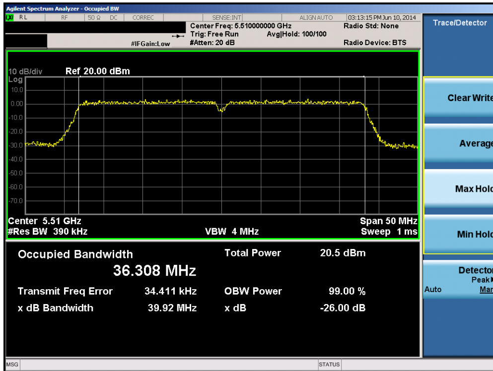
Plot 6-49. 26dB Bandwidth Plot (40MHz BW 802.11n (UNII Band 2C) – Ch. 102)
