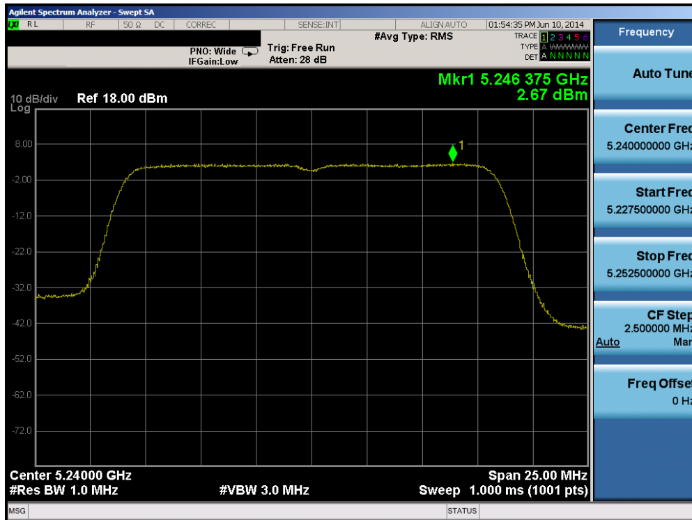
Plot 6-81. Peak Power Spectral Density Plot (802.11a (UNII Band 1) – Ch. 48)
