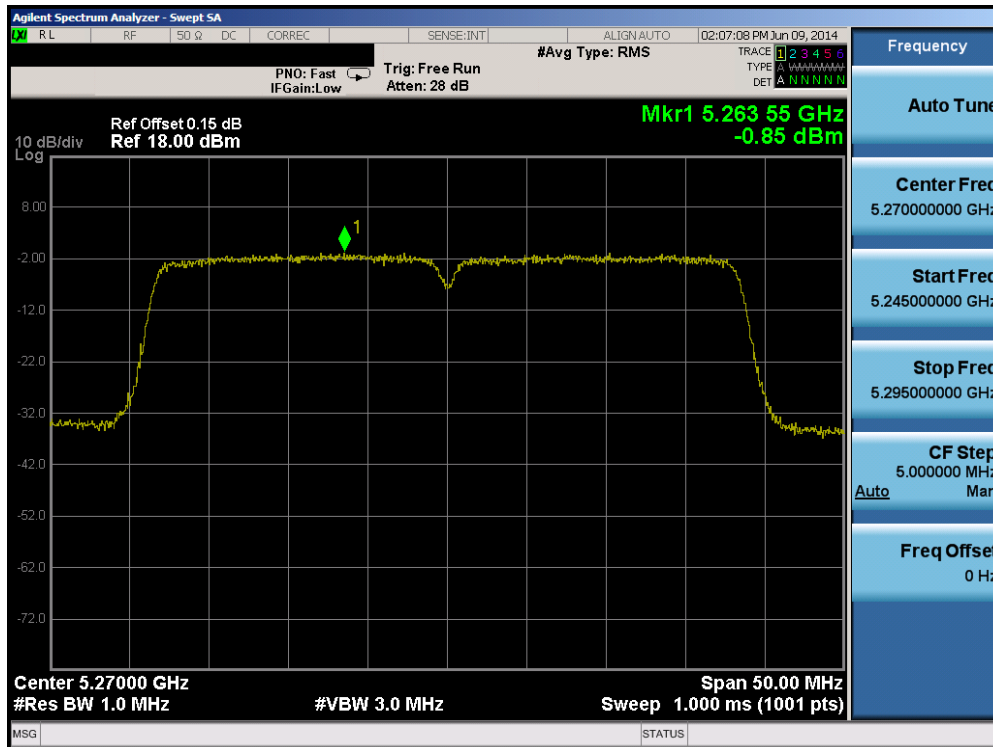
Plot 6-68. Peak Power Spectral Density Plot (40MHz BW 802.11n (UNII Band 2A) – Ch. 54)
