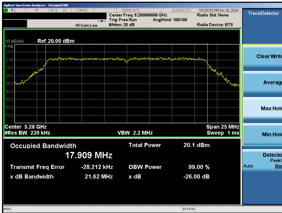
Plot 6-39. 26dB Bandwidth Plot (20MHz BW 802.11n (UNII Band 2A) – Ch. 56)
