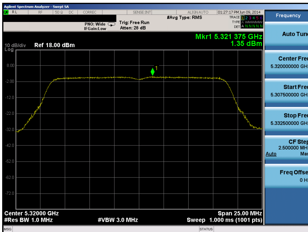
Plot 6-67. Peak Power Spectral Density Plot (20MHz BW 802.11n (UNII Band 2A) – Ch. 64)
