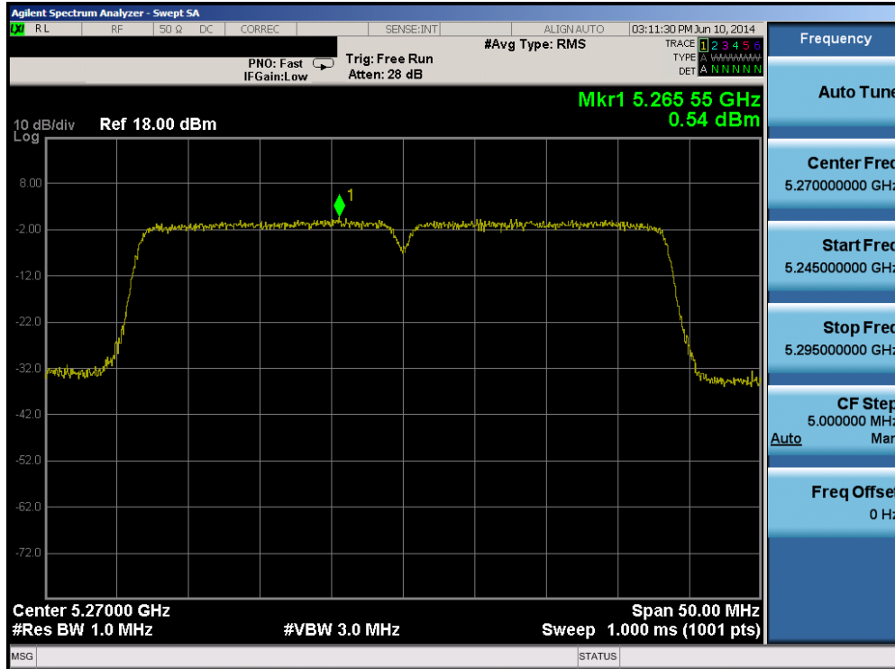
Plot 6-93. Peak Power Spectral Density Plot (40MHz BW 802.11n (UNII Band 2A) – Ch. 54)
