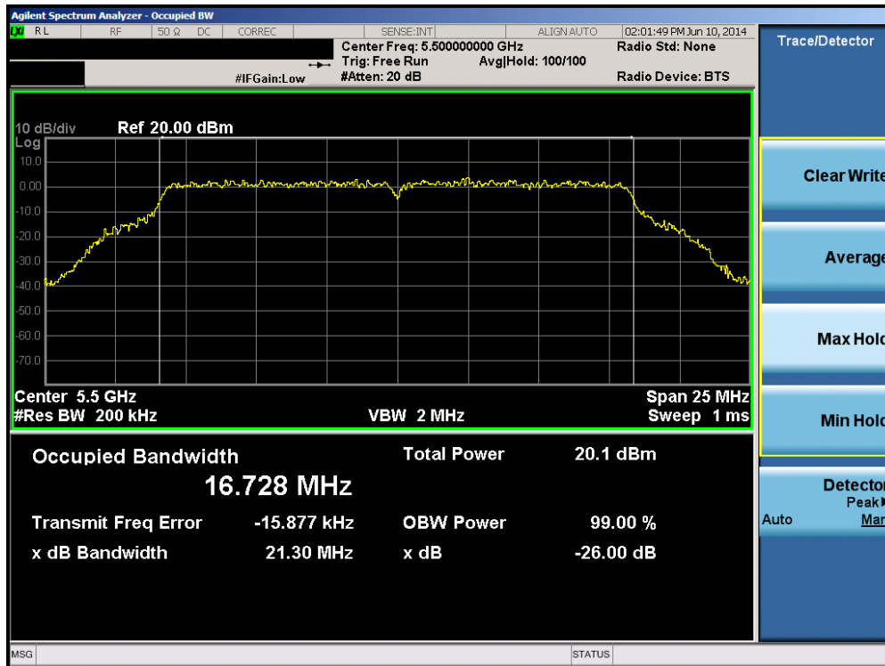
Plot 6-43. 26dB Bandwidth Plot (802.11a (UNII Band 2C) – Ch. 100)
