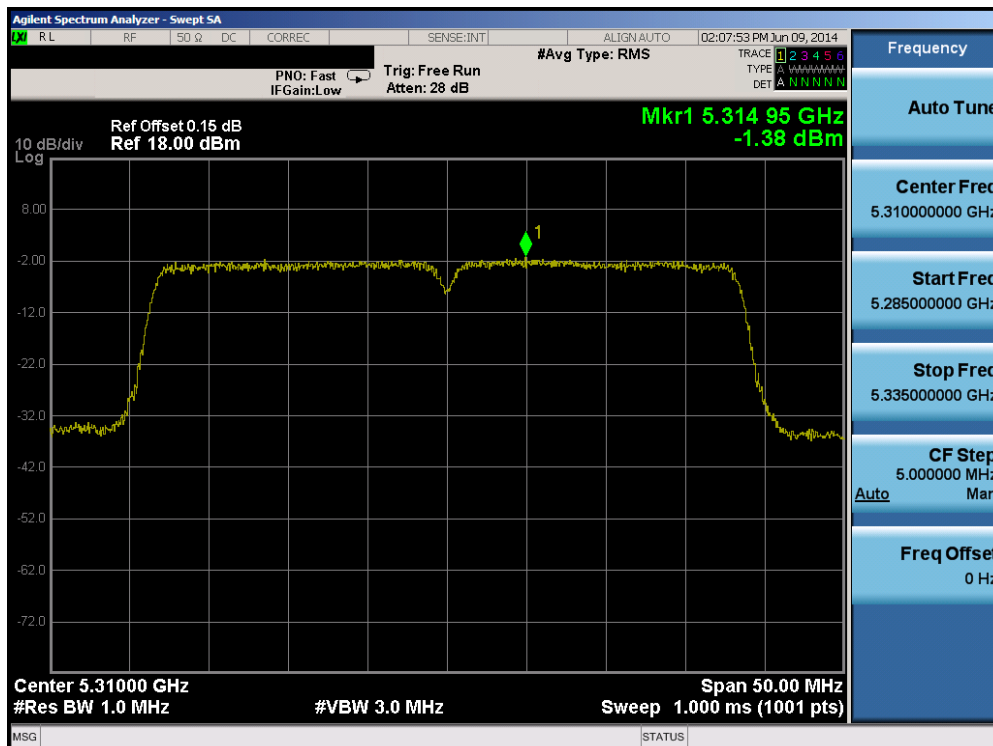
Plot 6-69. Peak Power Spectral Density Plot (40MHz BW 802.11n (UNII Band 2A) – Ch. 62)
