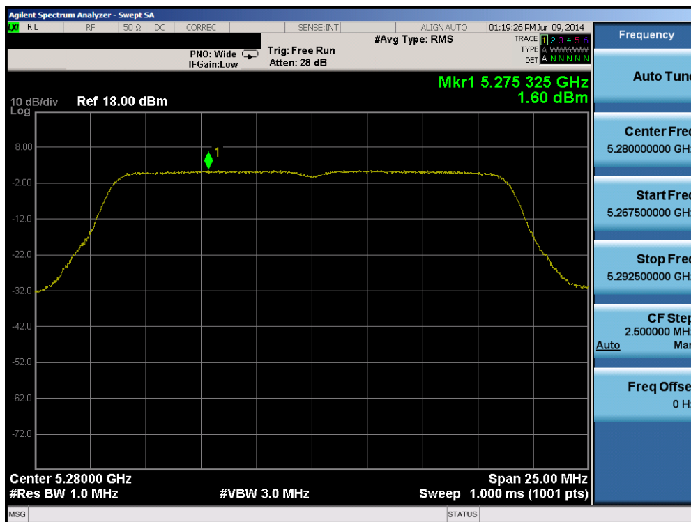
Plot 6-66. Peak Power Spectral Density Plot (20MHz BW 802.11n (UNII Band 2A) – Ch. 56)
