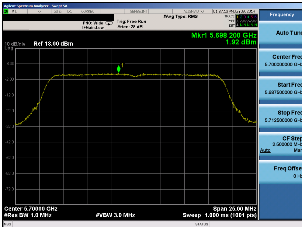
Plot 6-75. Peak Power Spectral Density Plot (20MHz BW 802.11n (UNII Band 2C) – Ch. 140)
