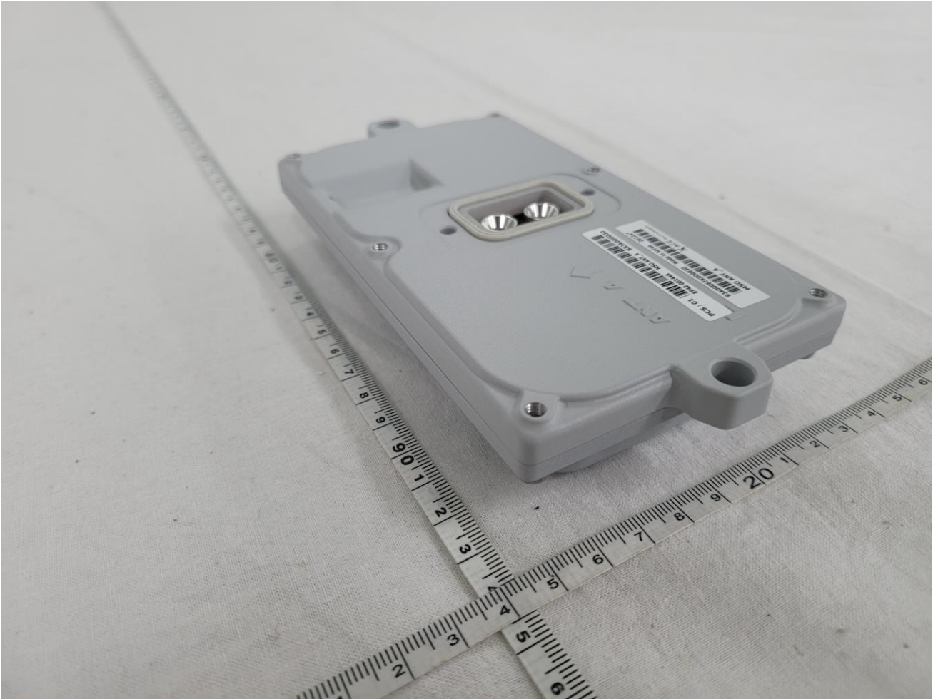
Rear view Antenna A
