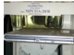
Figure 14.1 DSSS Body SAR Test Setup
