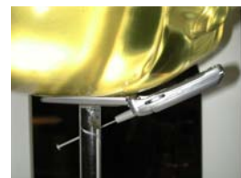
Figure 14.8 Right Head SAR Test Setup -- Cheek / Touch Position --
