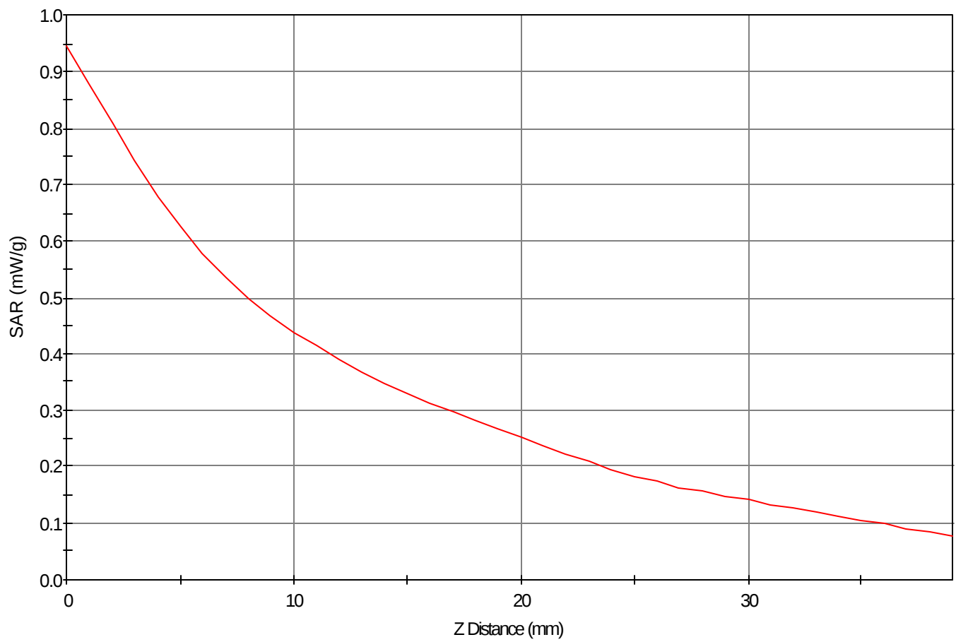
SAR - Z Axis at Hotspot x:32.0 y:17.0
