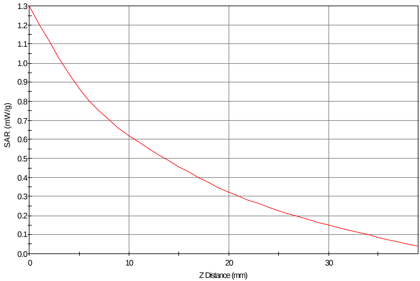
SAR - Z Axis at Hotspot x:19.0 y:-7.0
