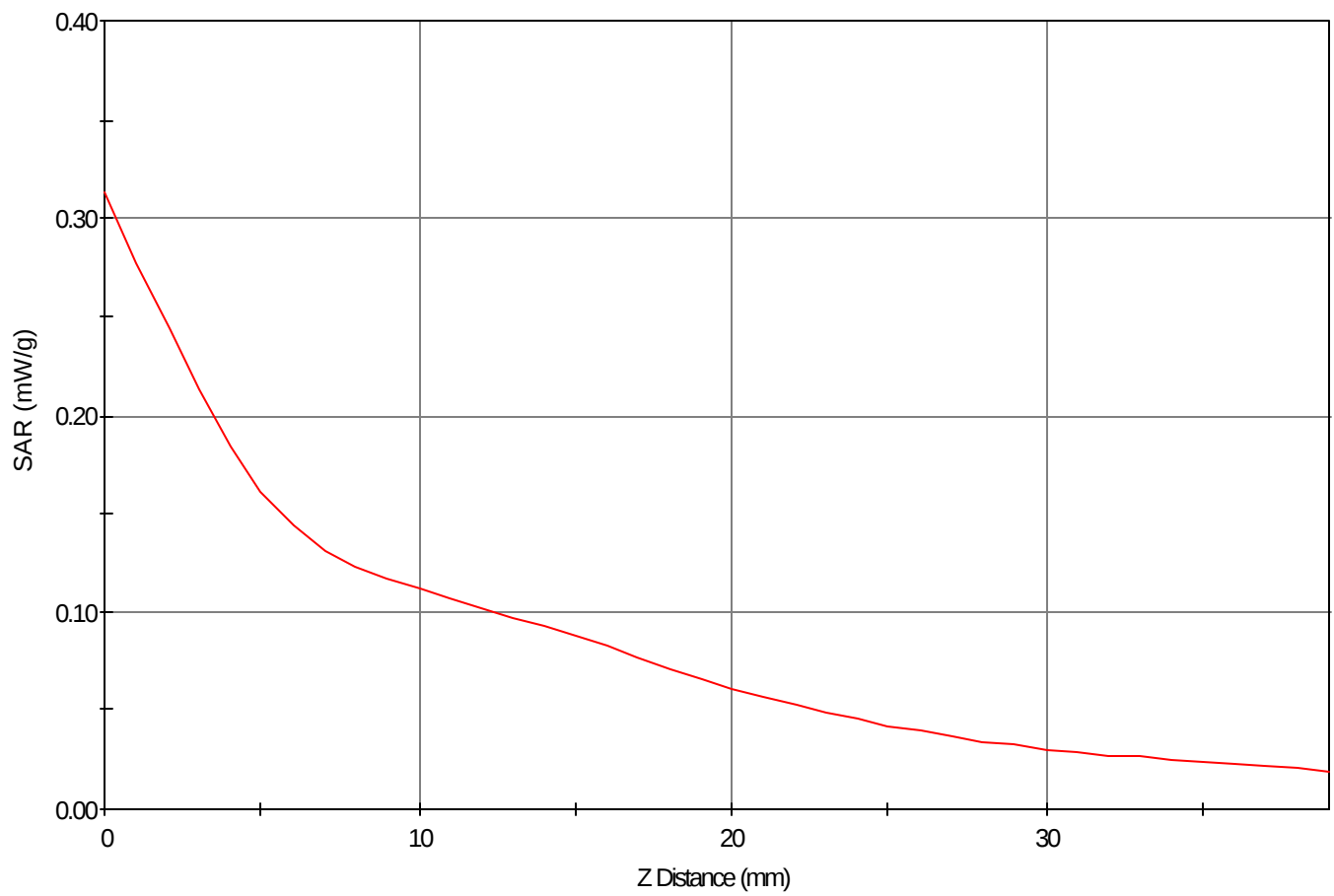
SAR - Z Axis at Hotspot x:71.0 y:2.0
