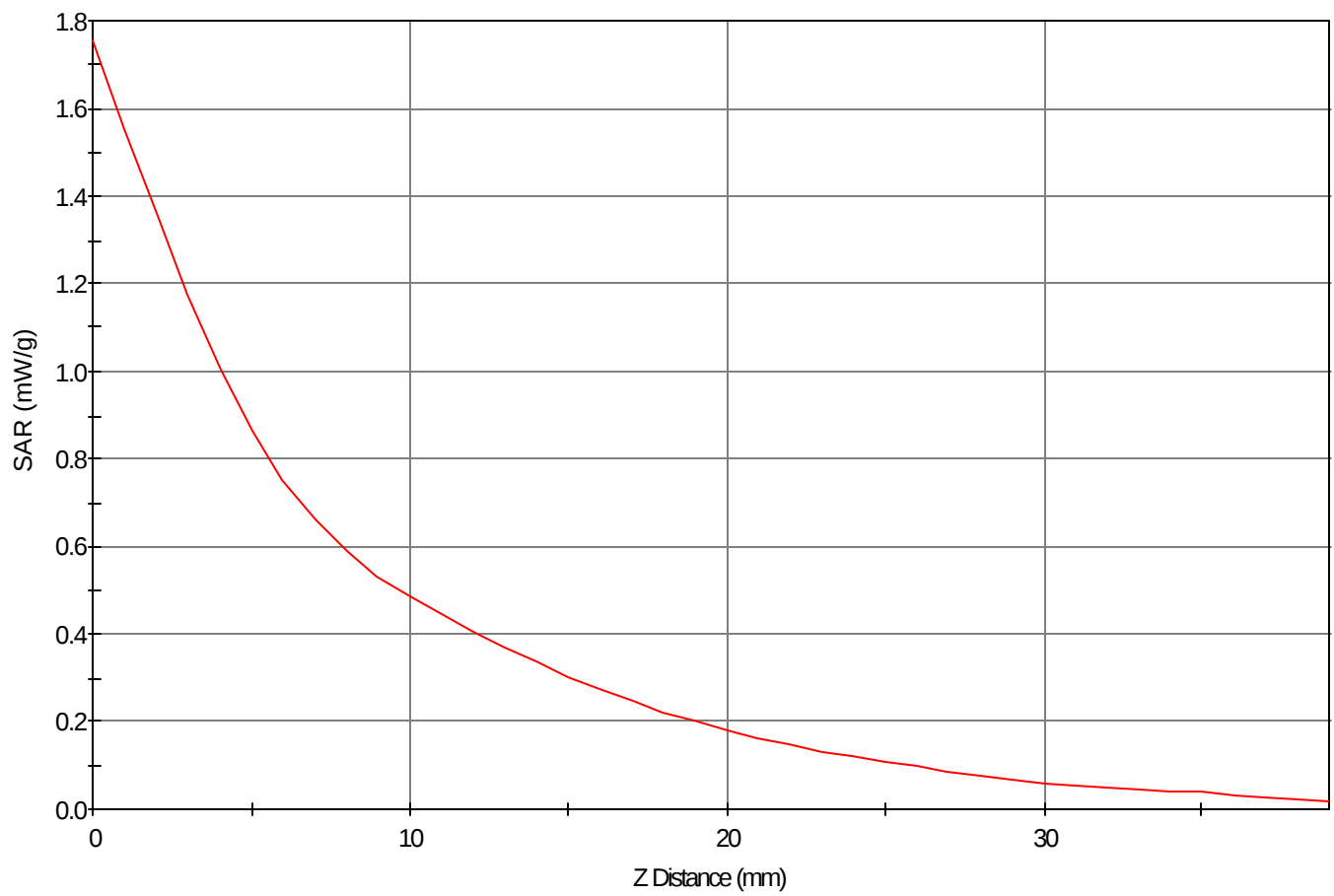
SAR - Z Axis at Hotspot x:-5.0 y:18.0
