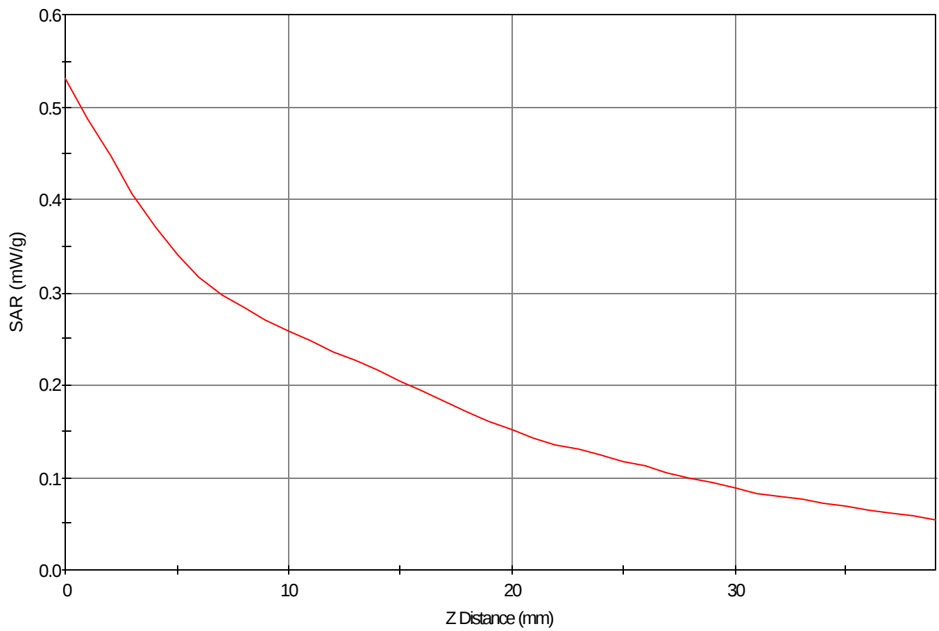
SAR - Z Axis at Hotspot x:51.0 y:10.0
