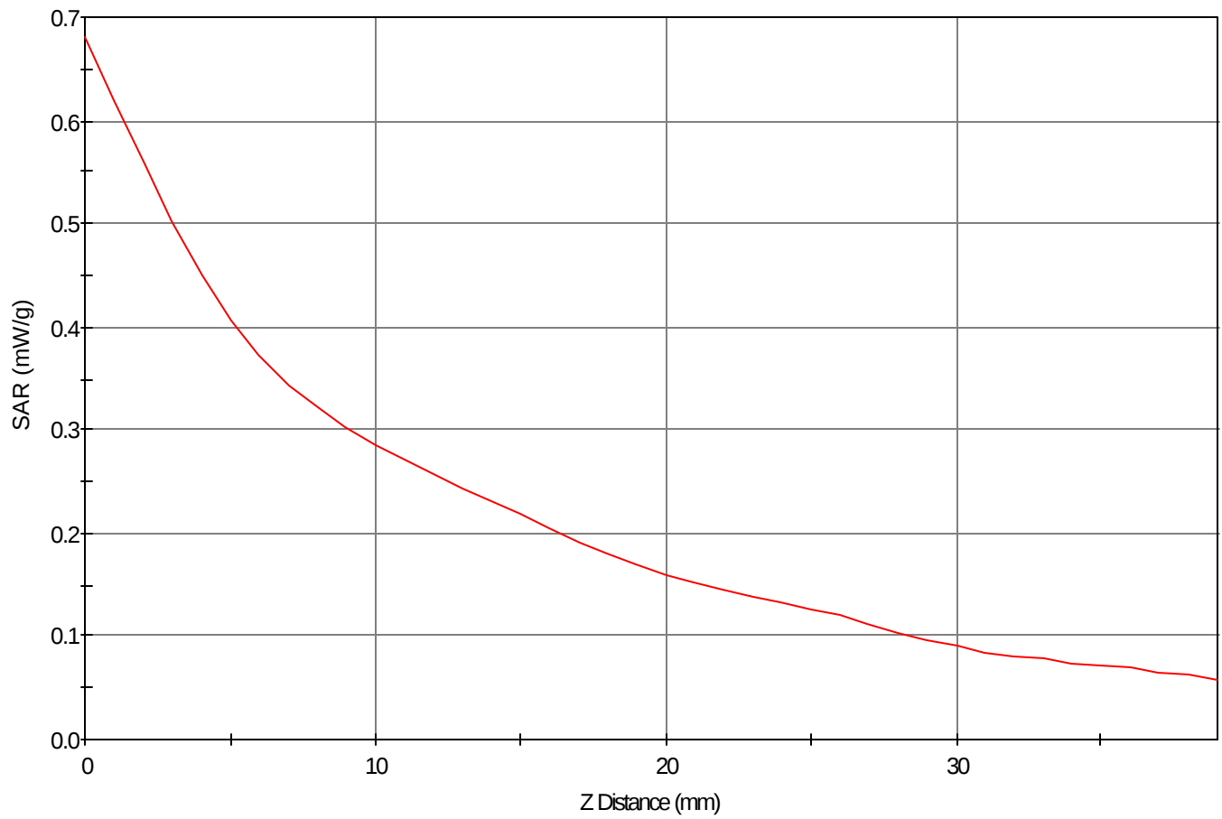
SAR - Z Axis at Hotspot x:31.0 y:6.0
