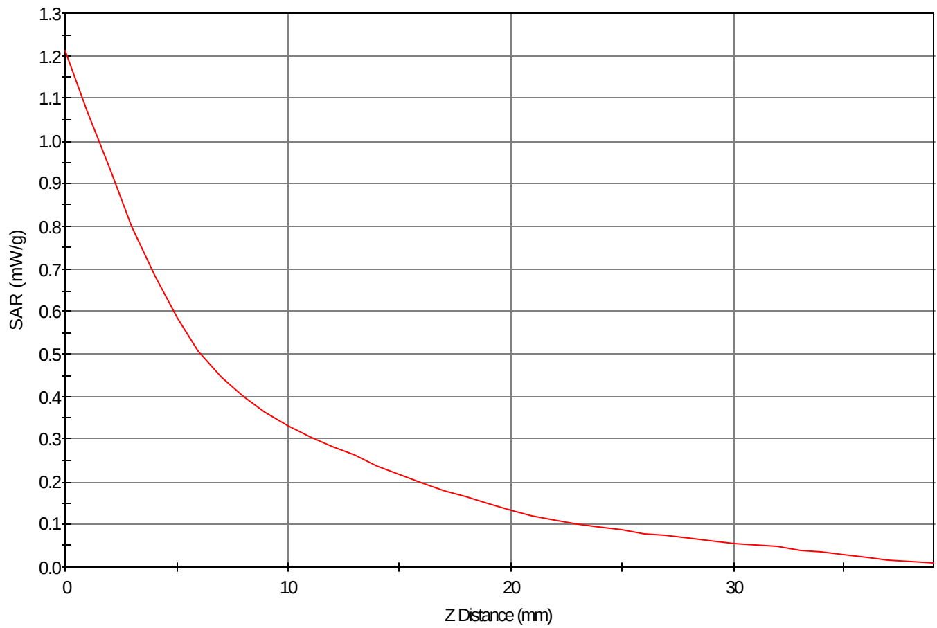
SAR - Z Axis at Hotspot x:3.0 y:-17.0
