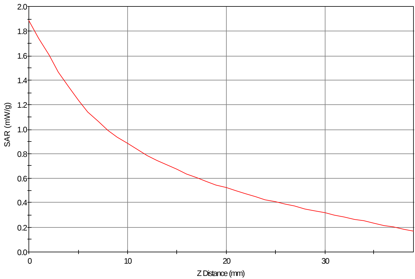
SAR - Z Axis at Hotspot x:79.0 y:-14.0
