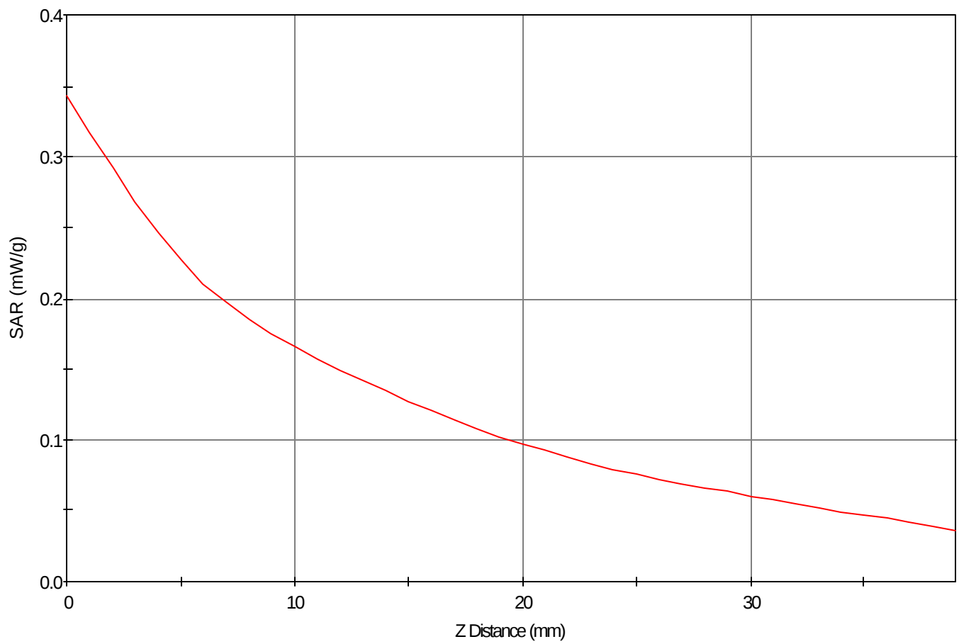
SAR - Z Axis at Hotspot x:41.0 y:13.0
