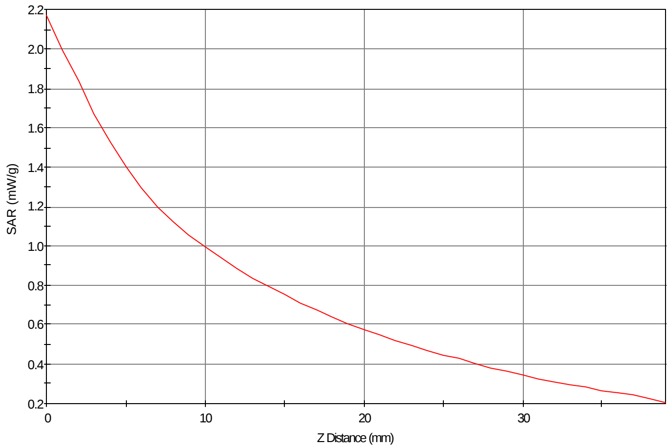
SAR - Z Axis at Hotspot x:76.0 y:11.0
