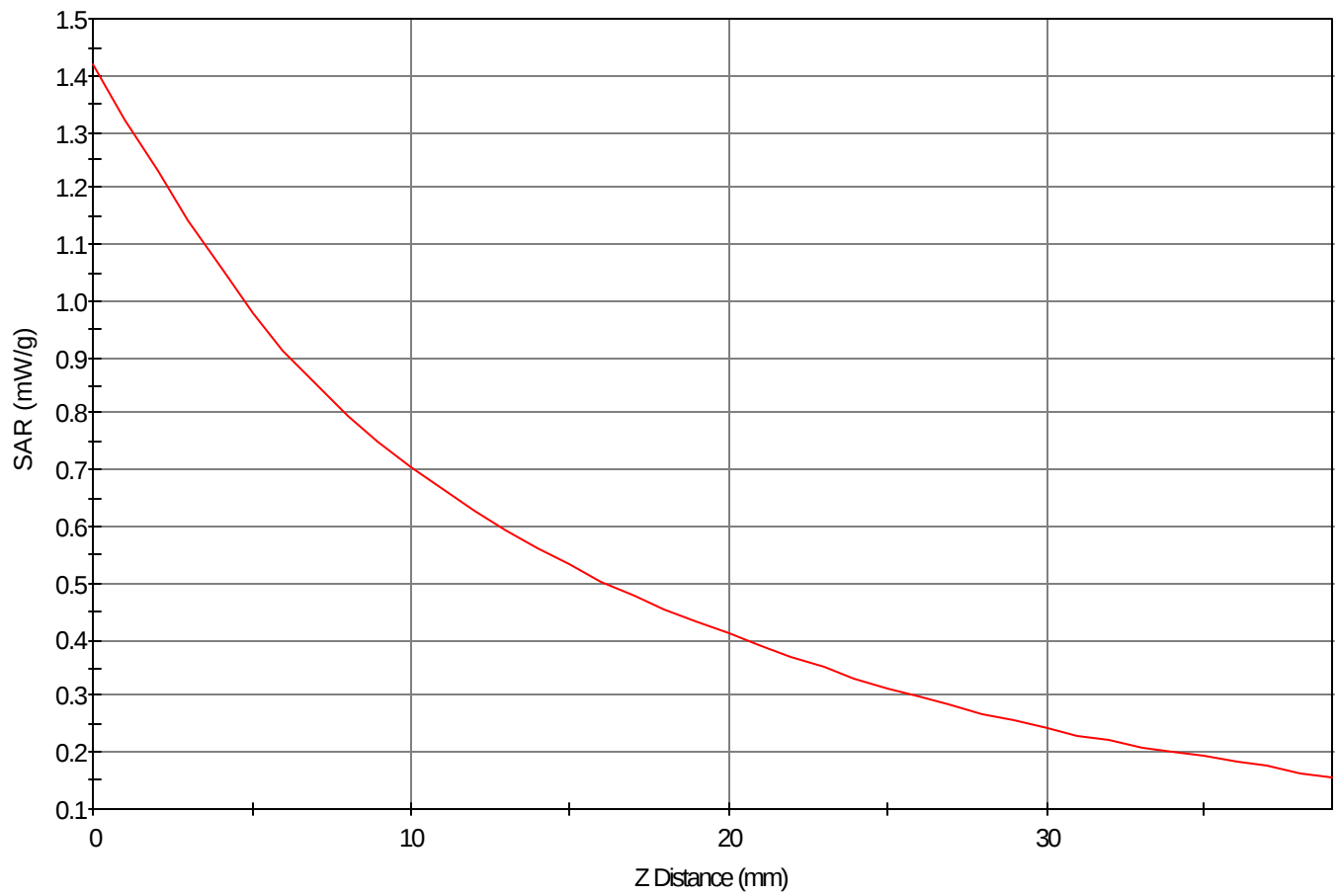
SAR - Z Axis at Hotspot x:77.0 y:11.0
