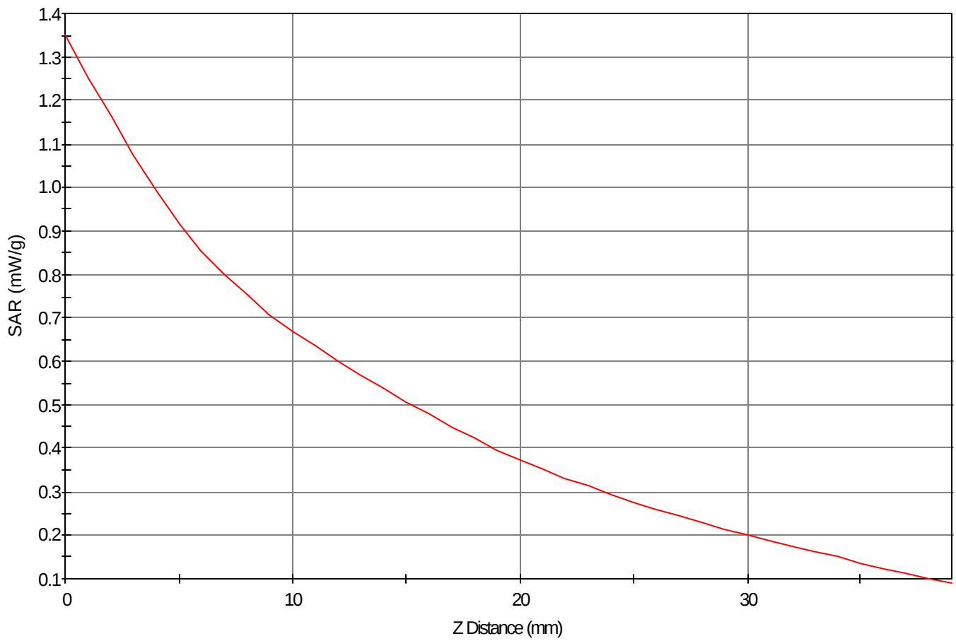
SAR - Z Axis at Hotspot x:77.0 y:8.0
