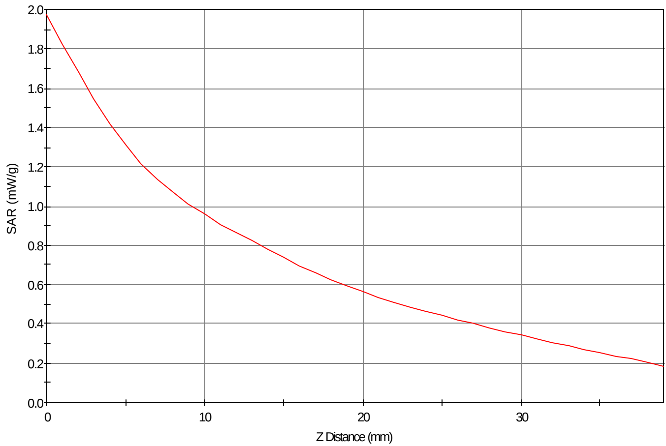
SAR - Z Axis at Hotspot x:73.0 y:10.0
