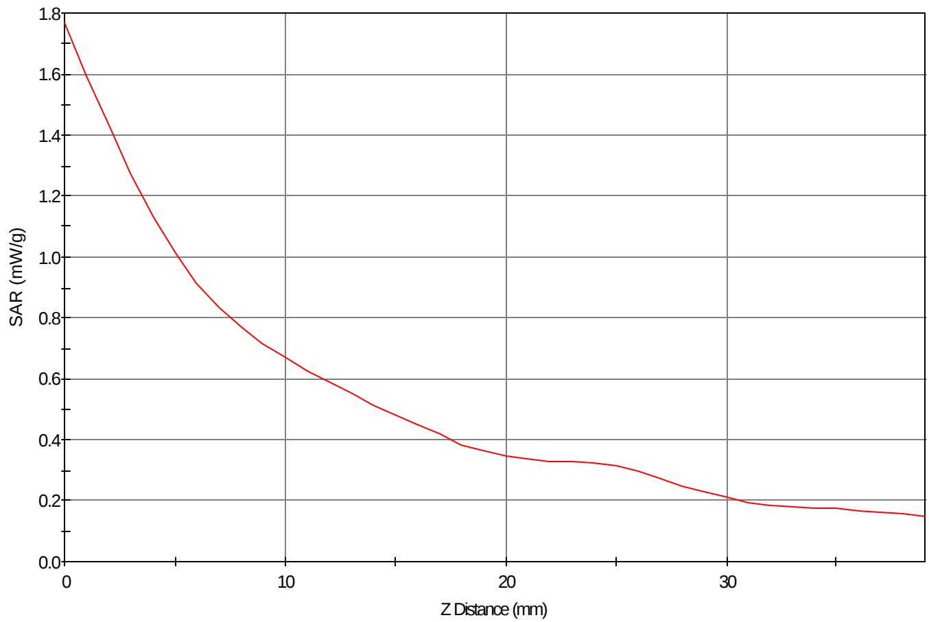
SAR - Z Axis at Hotspot x:79.0 y:8.0
