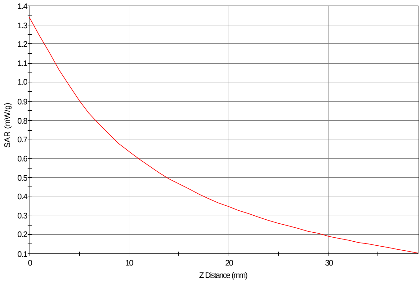
SAR - Z Axis at Hotspot x:2.0 y:-15.0
