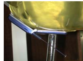
Figure 14.8 Left Head SAR Test Setup -- Cheek / Touch Position --
