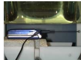
Figure 14.12 Body SAR Test Setup -- w/o Holster --
