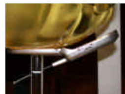
Figure A.5 Right Head SAR Test Setup -- Cheek / Touch Position --
