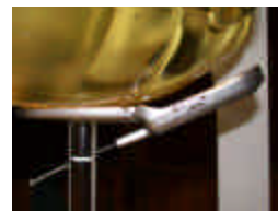
Figure A.9 Right Head SAR Test Setup -- Cheek / Touch Position --
