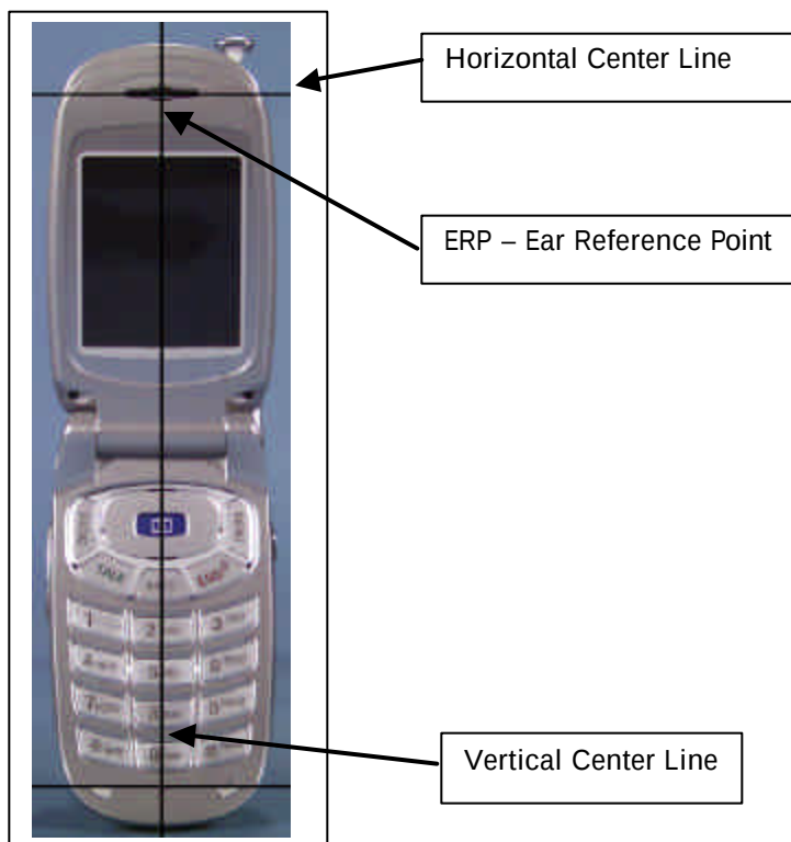
Figure 12.1 Handset Reference Points
