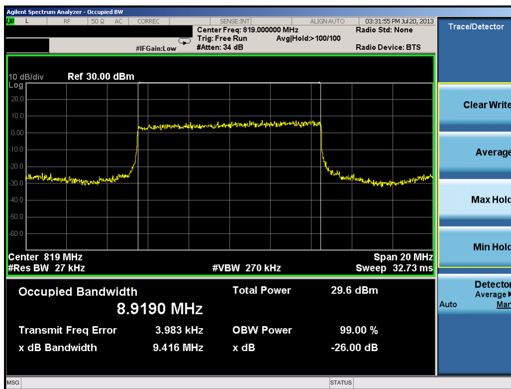
Plot 7-50. Occupied Bandwidth Plot (10MHz QPSK – RB Size 50 – High Channel)
