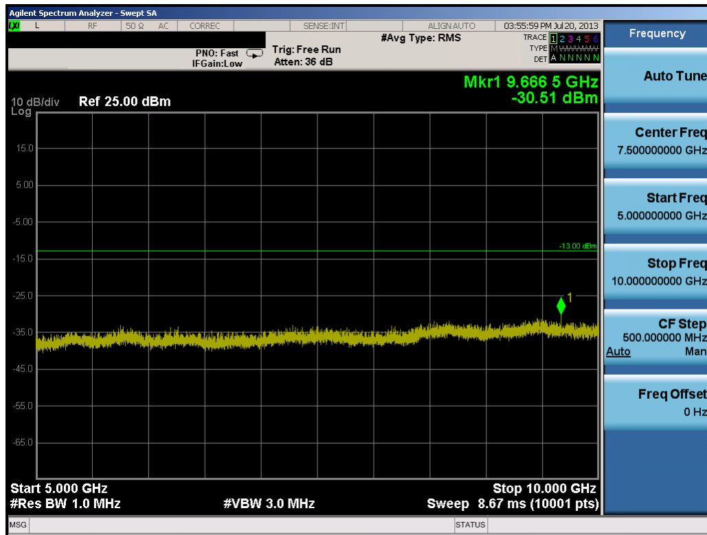
Plot 7-14. Conducted Spurious Plot (1.4MHz QPSK – RB Size 1, RB Offset 0 – Low Channel)
