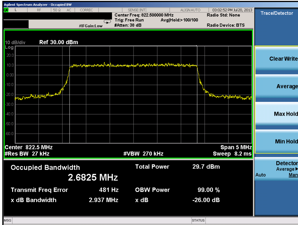
Plot 7-31. Occupied Bandwidth Plot (3MHz 16-QAM – RB Size 15– Low Channel)
