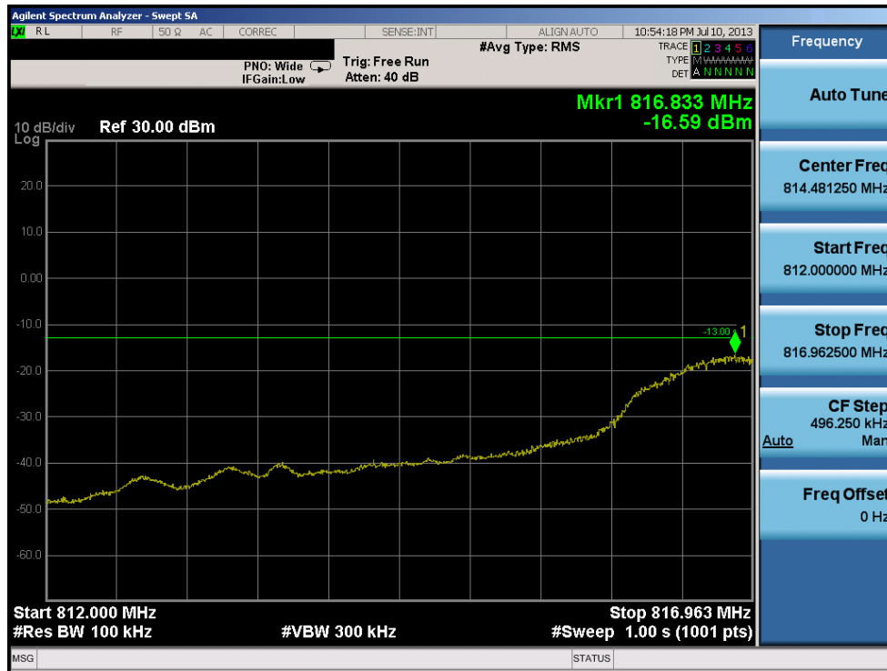
Plot 7-4. Extended Band Edge Plot (Ch. 476)
