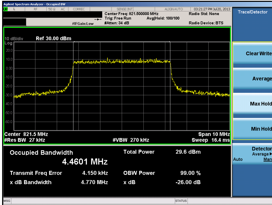
Plot 7-45. Occupied Bandwidth Plot (5MHz QPSK – RB Size 25 – High Channel)
