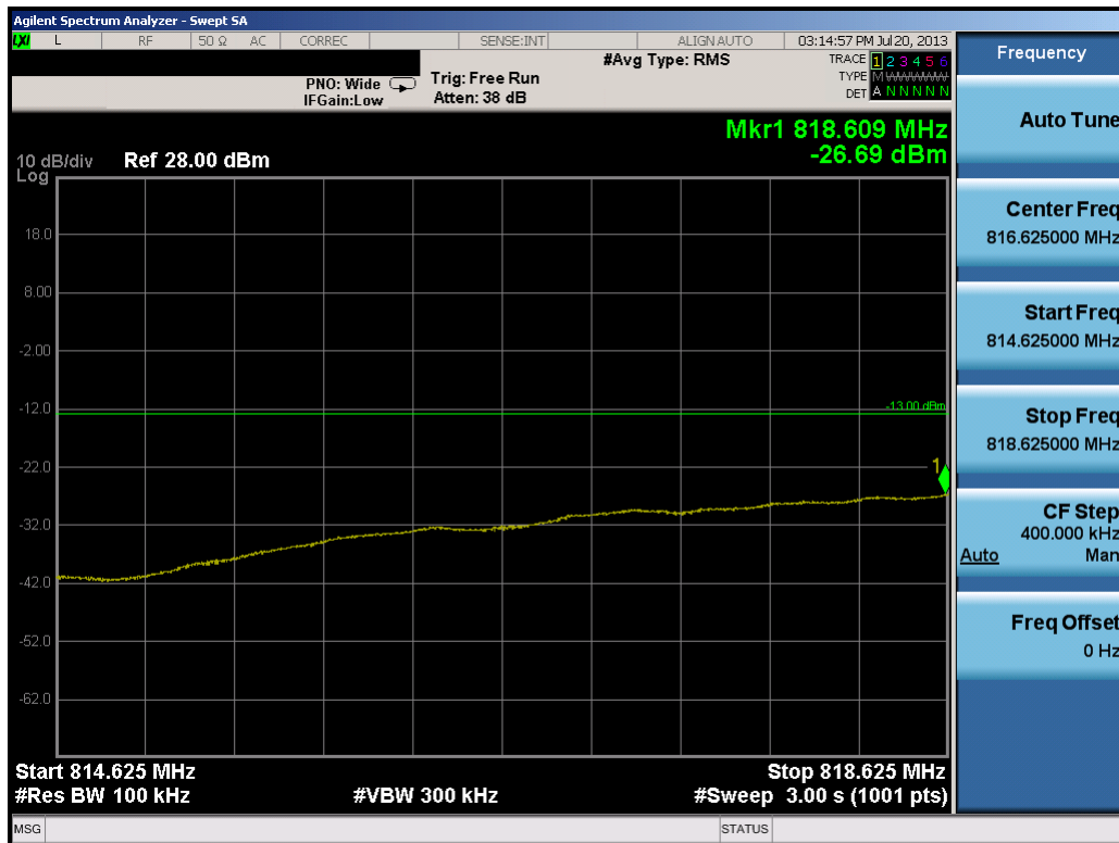
Plot 7-44. Extended Band Edge Plot (5MHz QPSK – RB Size 25 – High Channel)
