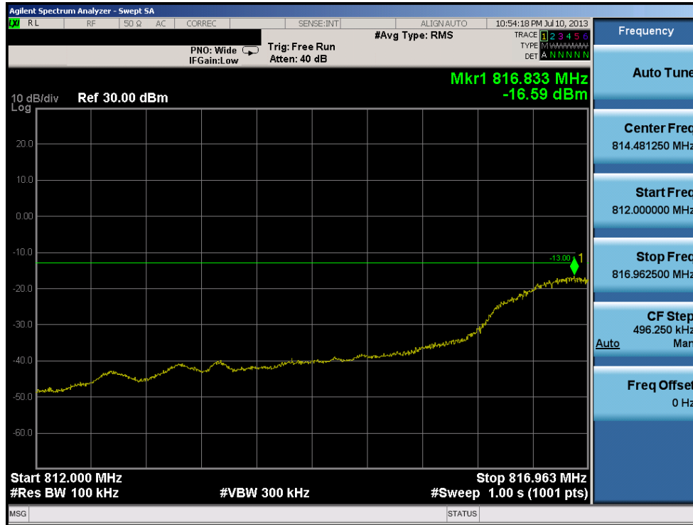
Plot 7-9. Extended Band Edge Plot (Ch. 684)
