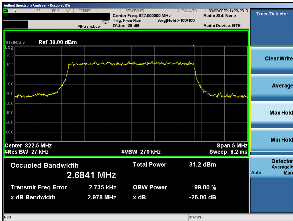
Plot 7-30. Occupied Bandwidth Plot (3MHz QPSK - RB Size 15- Low Channel)
