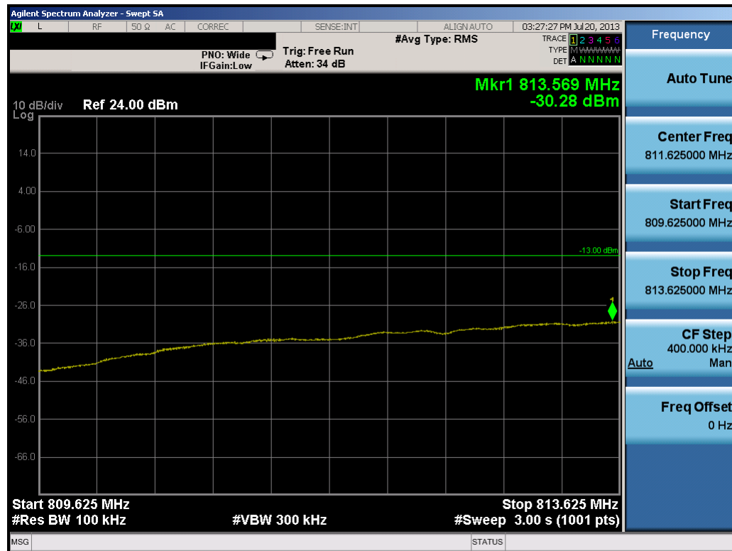
Plot 7-38. Extended Band Edge Plot (5MHz QPSK – RB Size 25– Low Channel)
