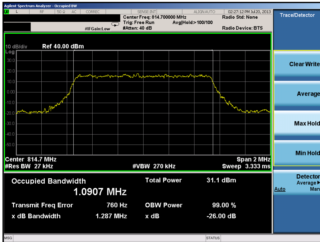
Plot 7-18. Occupied Bandwidth Plot (1.4MHz QPSK - RB Size 6- Low Channel)
