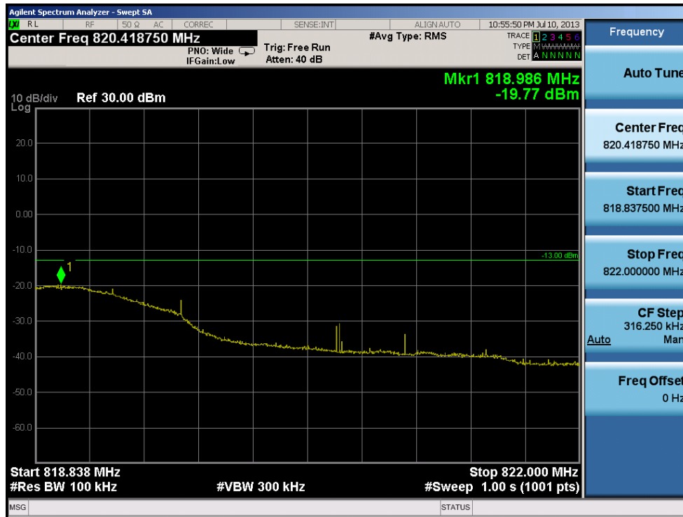
Plot 7-10. Extended Band Edge Plot - Interior (Ch. 684)
