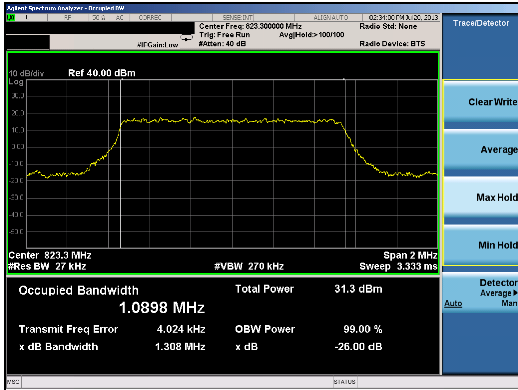
Plot 7-25. Occupied Bandwidth Plot (1.4MHz QPSK – RB Size 6 – High Channel)
