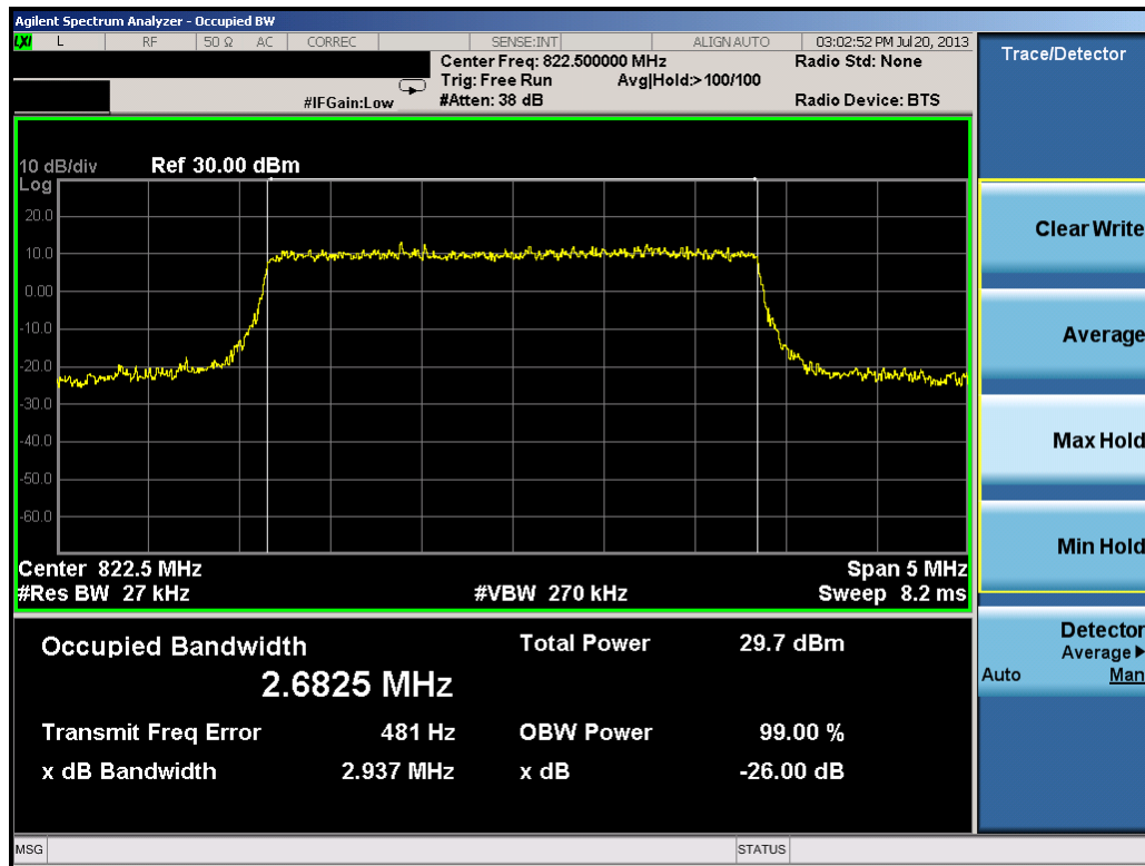
Plot 7-36. Occupied Bandwidth Plot (3MHz 16-QAM – RB Size 15 – High Channel)
