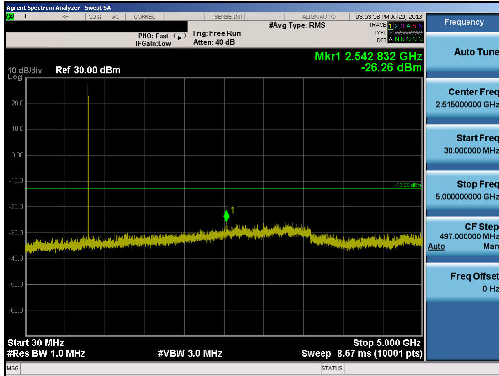
Plot 7-13. Conducted Spurious Plot (1.4MHz QPSK – RB Size 1, RB Offset 0 – Low Channel)
