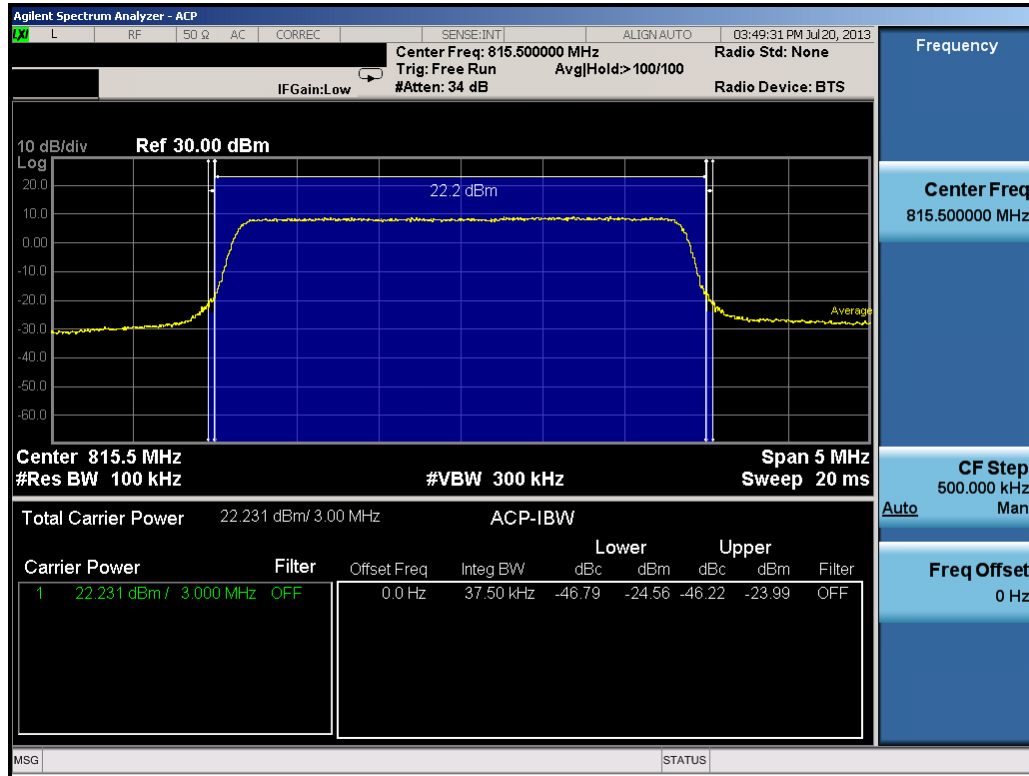
Plot 7-27. Channel Edge Plot (3MHz QPSK – RB Size 15– Low Channel)
