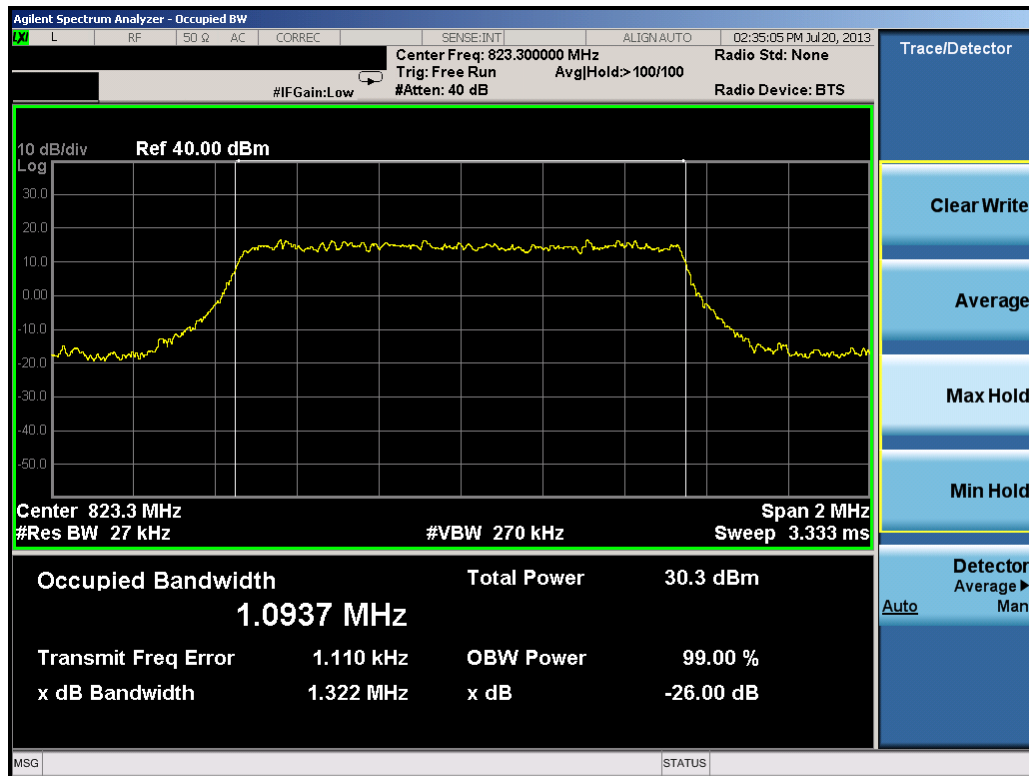
Plot 7-26. Occupied Bandwidth Plot (1.4MHz 16-QAM – RB Size 6 – High Channel)
