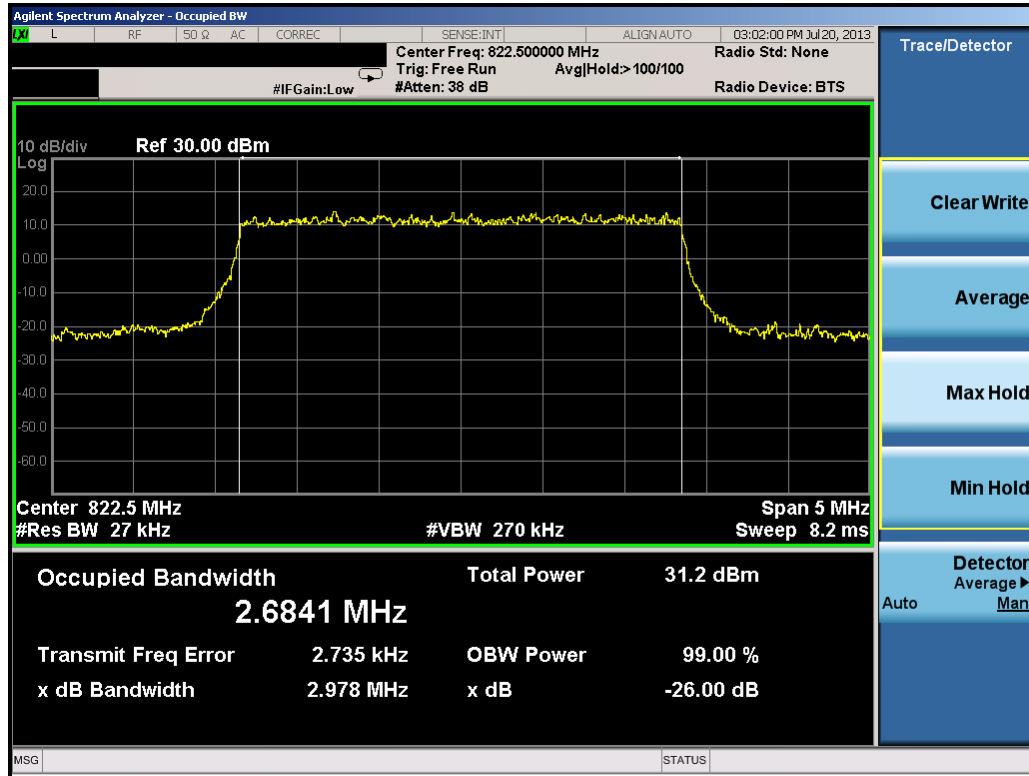
Plot 7-35. Occupied Bandwidth Plot (3MHz QPSK – RB Size 15 – High Channel)
