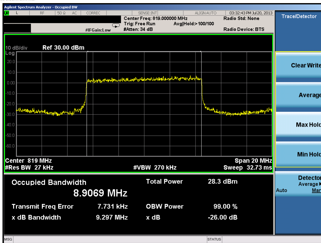
Plot 7-51. Occupied Bandwidth Plot (10MHz 16-QAM – RB Size 50 – High Channel)
