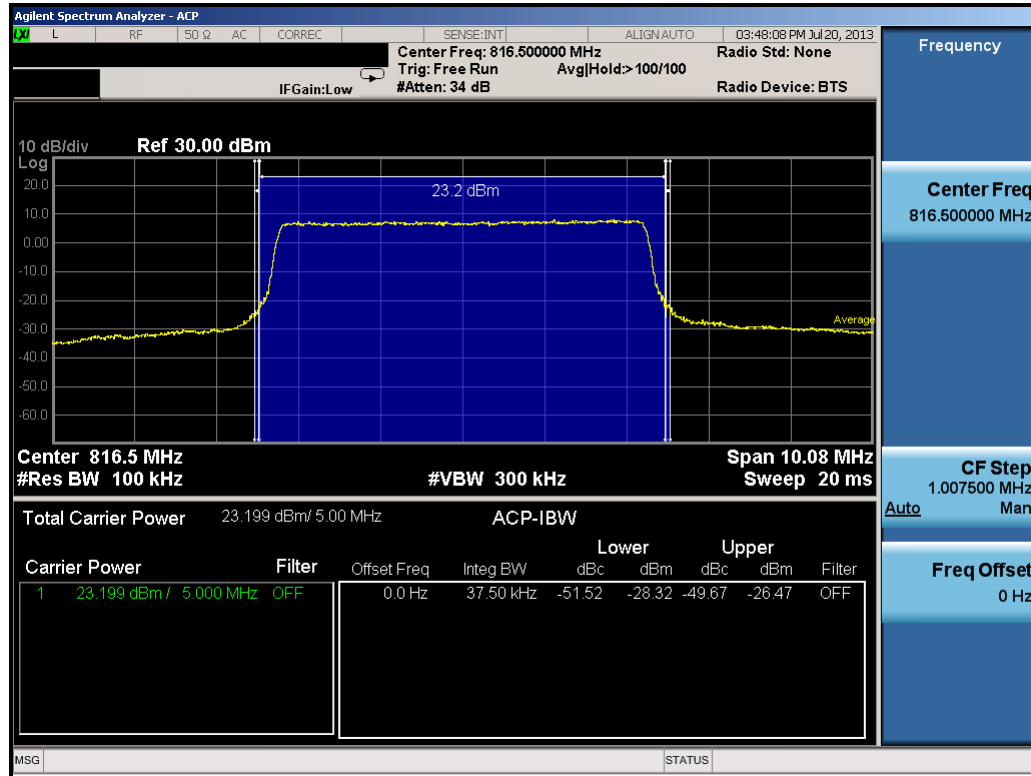
Plot 7-37. Channel Edge Plot (5MHz QPSK – RB Size 25– Low Channel)
