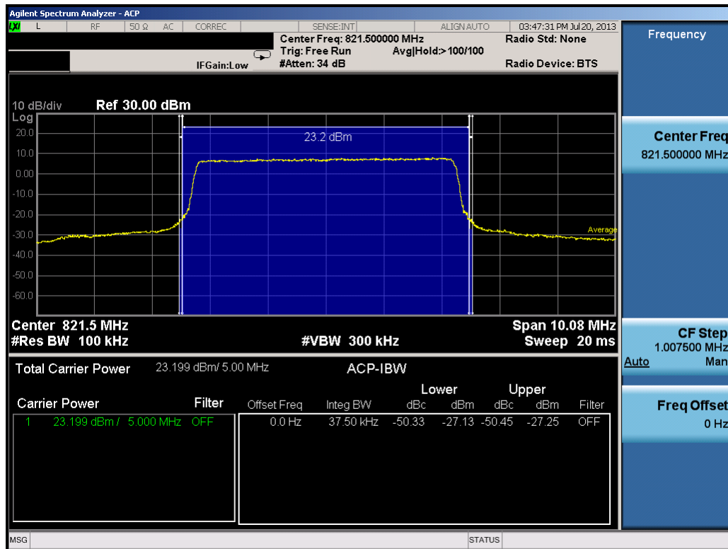
Plot 7-42. Channel Edge Plot (5MHz QPSK – RB Size 25 – High Channel)
