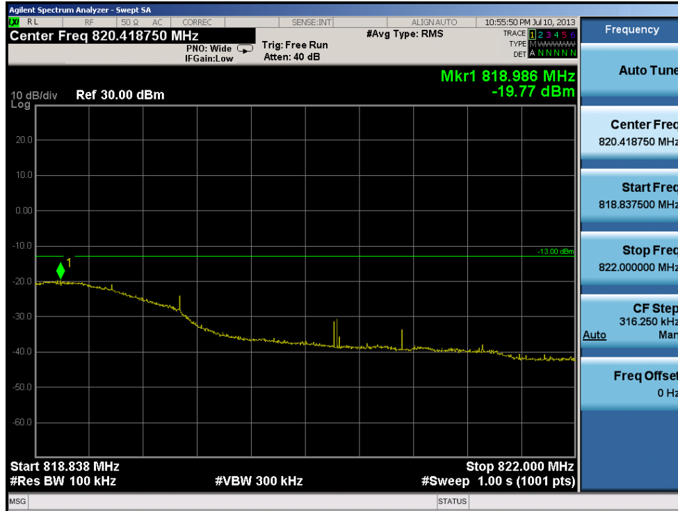
Plot 7-5. Extended Band Edge Plot - Interior (Ch. 476)
