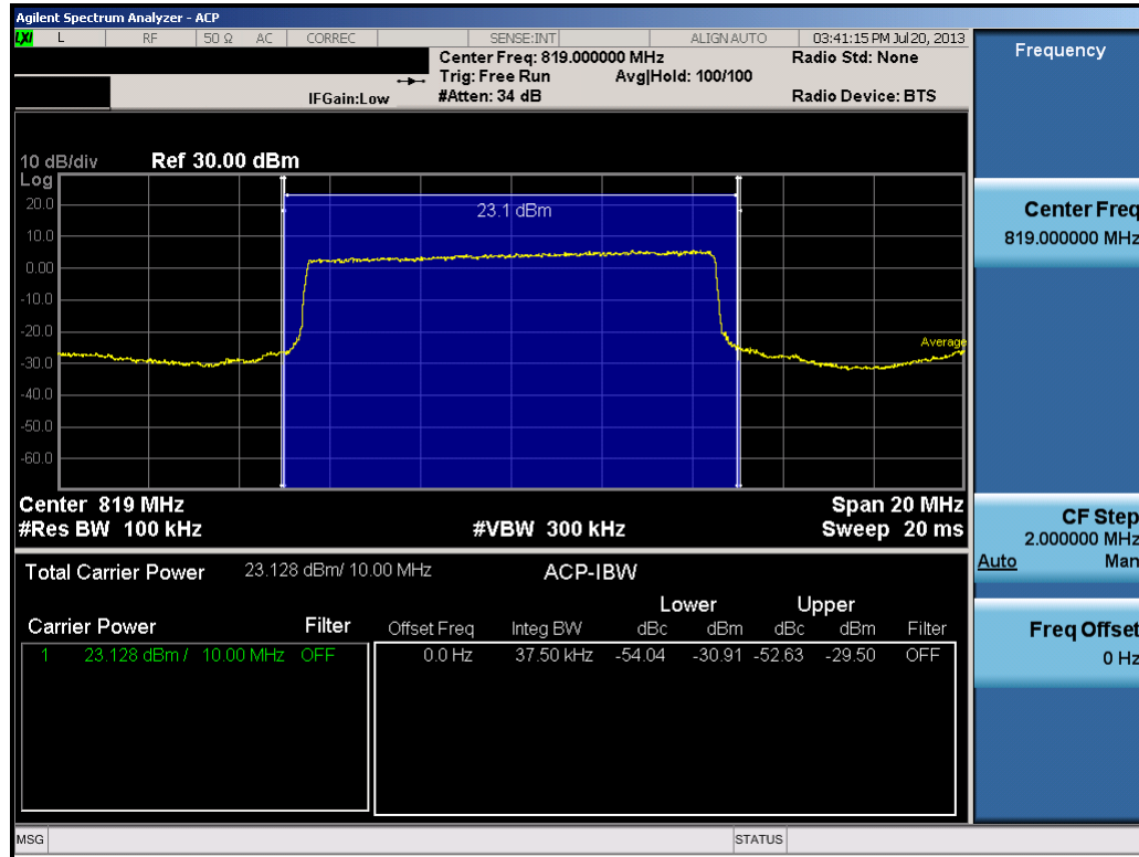
Plot 7-47. Channel Edge Plot (10MHz QPSK – RB Size 50)
