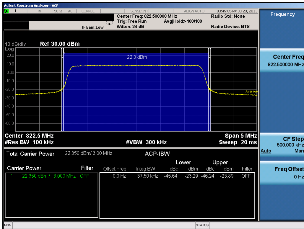
Plot 7-32. Channel Edge Plot (3MHz QPSK – RB Size 15 – High Channel)
