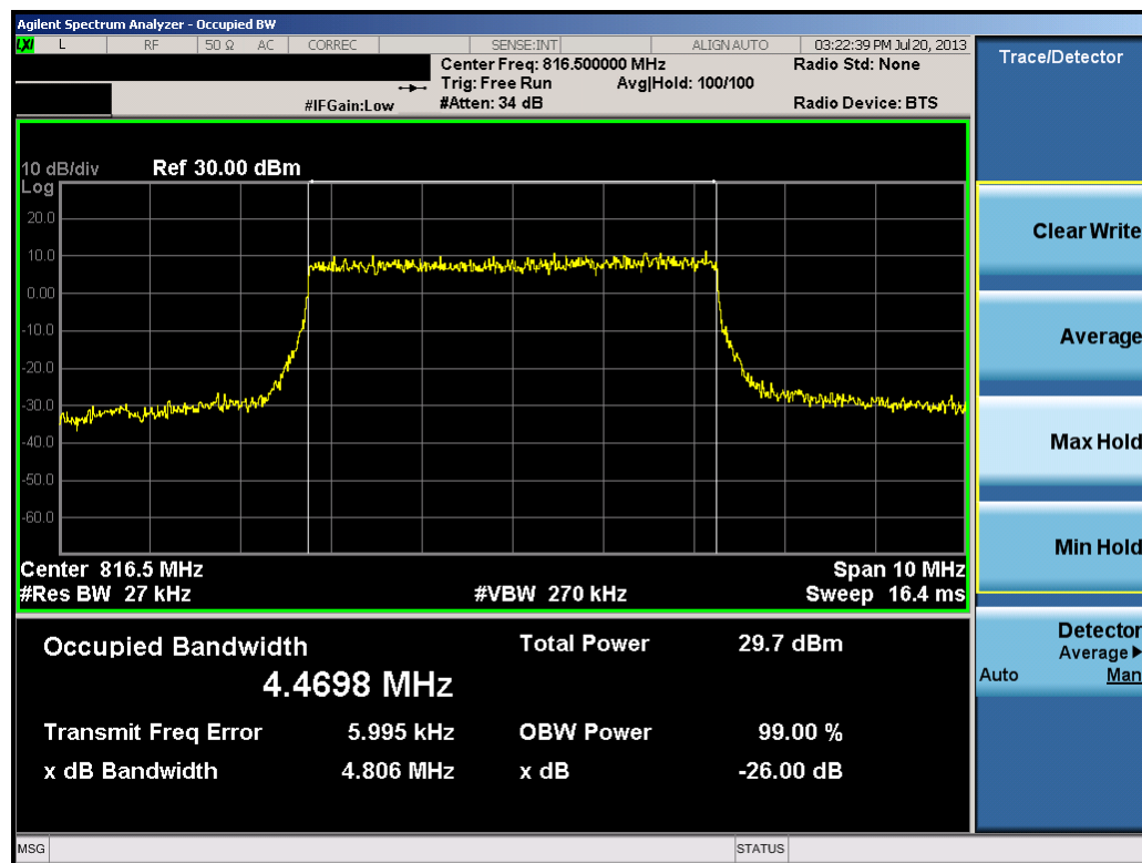
Plot 7-40. Occupied Bandwidth Plot (5MHz QPSK – RB Size 25– Low Channel)
