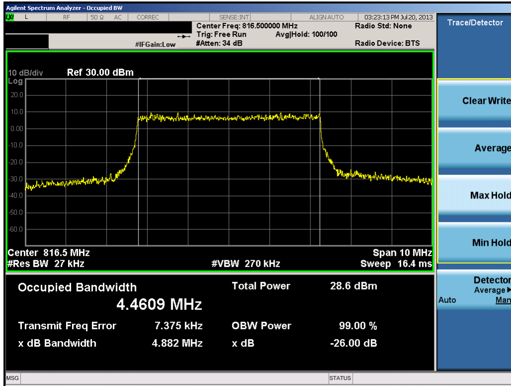
Plot 7-41. Occupied Bandwidth Plot (5MHz 16-QAM – RB Size 25– Low Channel))
