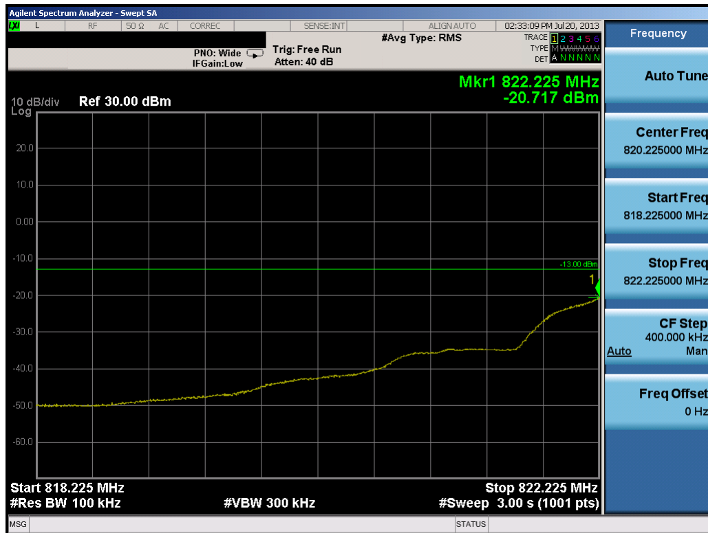
Plot 7-24. Extended Band Edge Plot (1.4MHz QPSK – RB Size 6 – High Channel)
