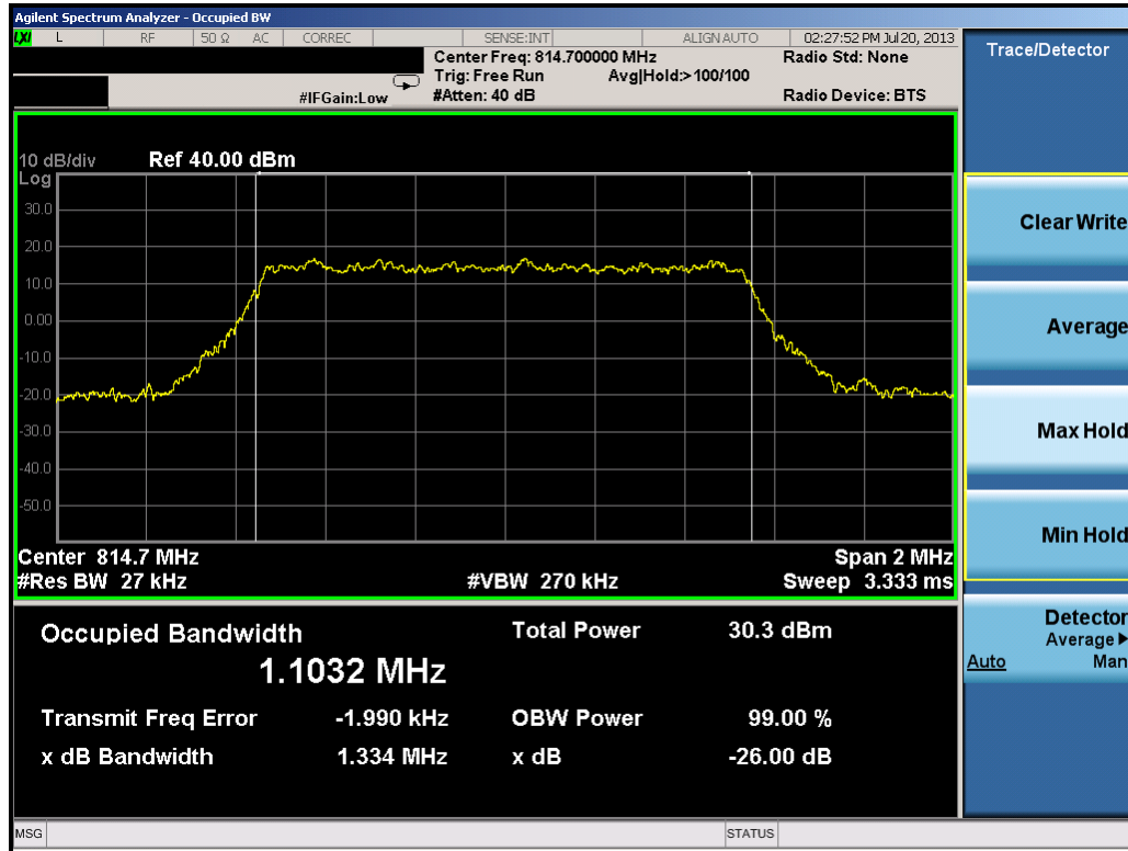
Plot 7-19. Occupied Bandwidth Plot (1.4MHz 16-QAM – RB Size 6– Low Channel)
