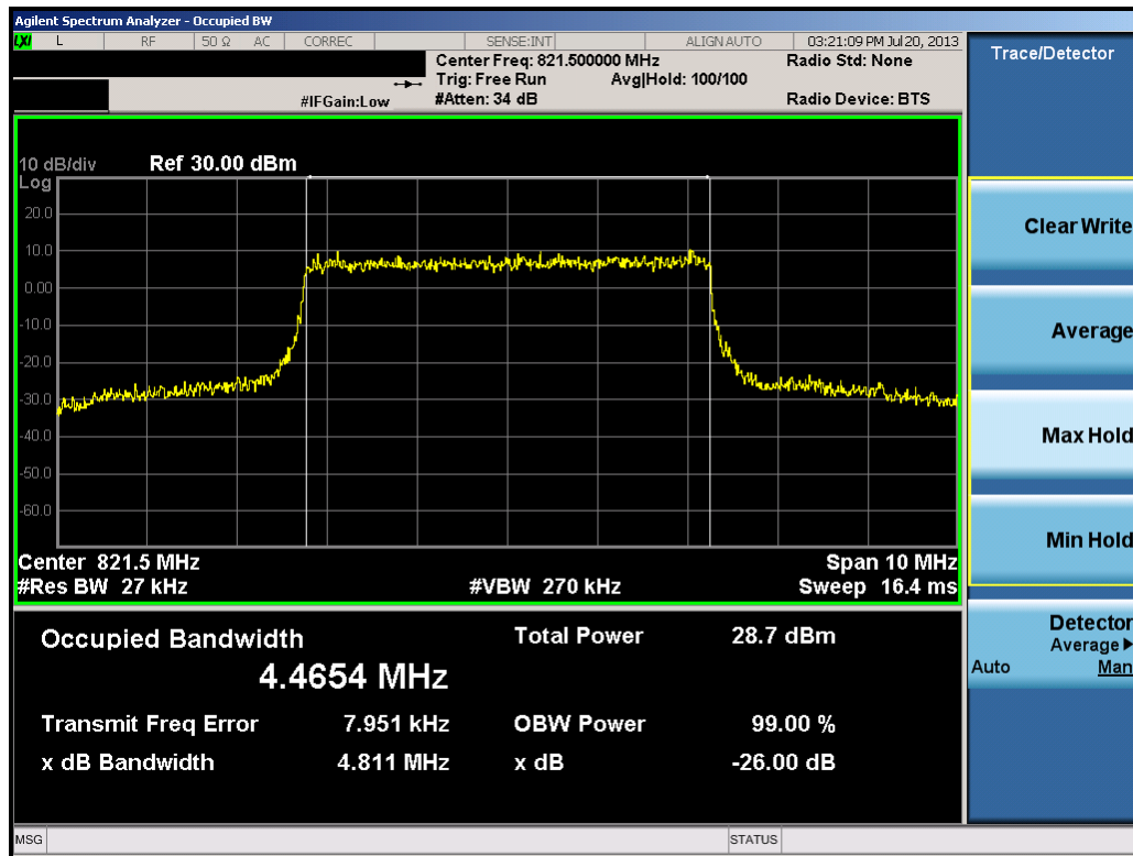
Plot 7-46. Occupied Bandwidth Plot (5MHz 16-QAM – RB Size 25 – High Channel)
