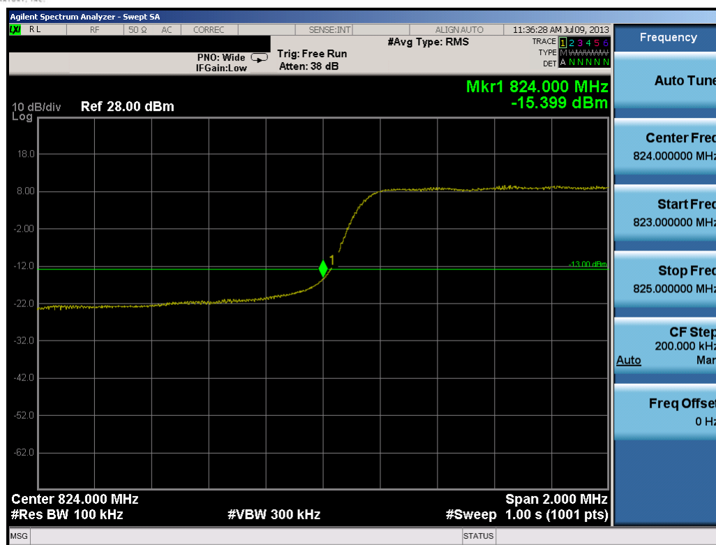
Plot 7-7. Lower Band Edge Plot (3.0MHz QPSK – RB Size 15)
