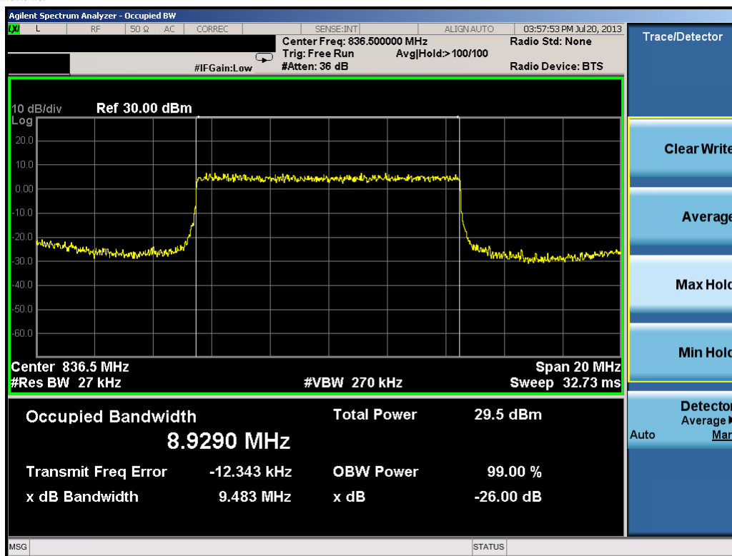
Plot 7-27. Occupied Bandwidth Plot (10.0MHz QPSK – RB Size 50)
