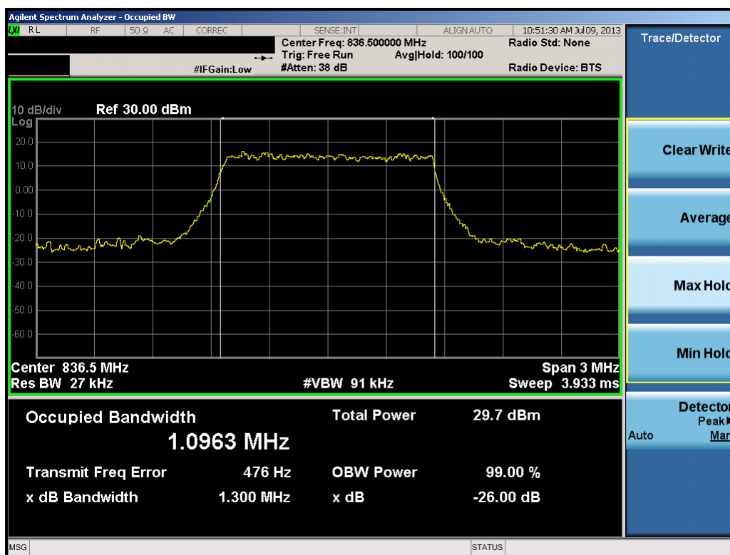
Plot 7-4. Occupied Bandwidth Plot (1.4MHz 16-QAM – RB Size 6)
