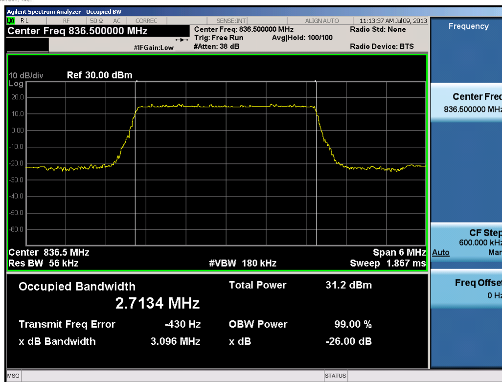
Plot 7-9. Occupied Bandwidth Plot (3.0MHz QPSK – RB Size 15)
