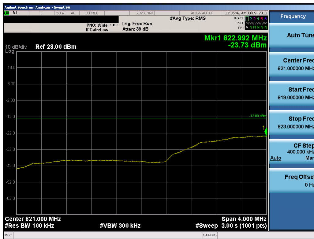
Plot 7-8. Lower Extended Band Edge Plot (3.0MHz QPSK – RB Size 15)
