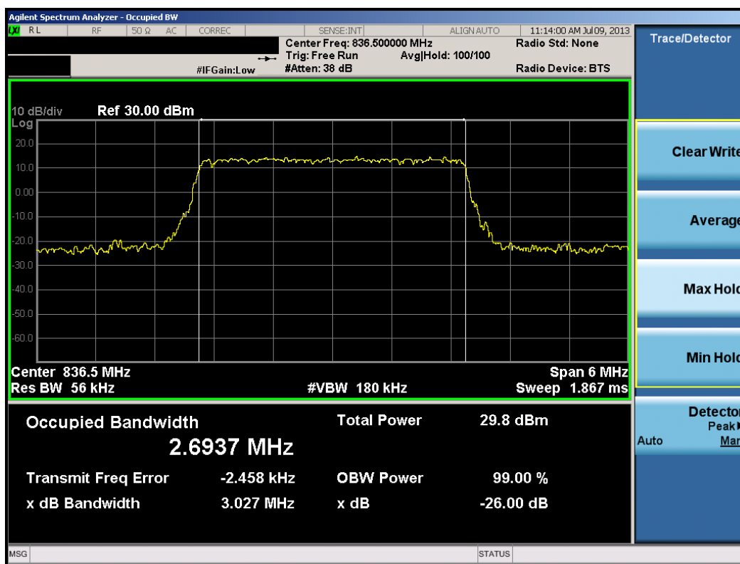
Plot 7-10. Occupied Bandwidth Plot (3.0MHz 16-QAM – RB Size 15)
