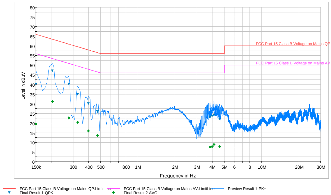
Plot 7-2. Line Conducted Plot (LN)
