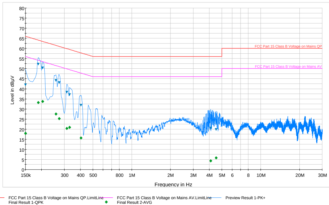
Plot 7-1. Line Conducted Plot (L1)
