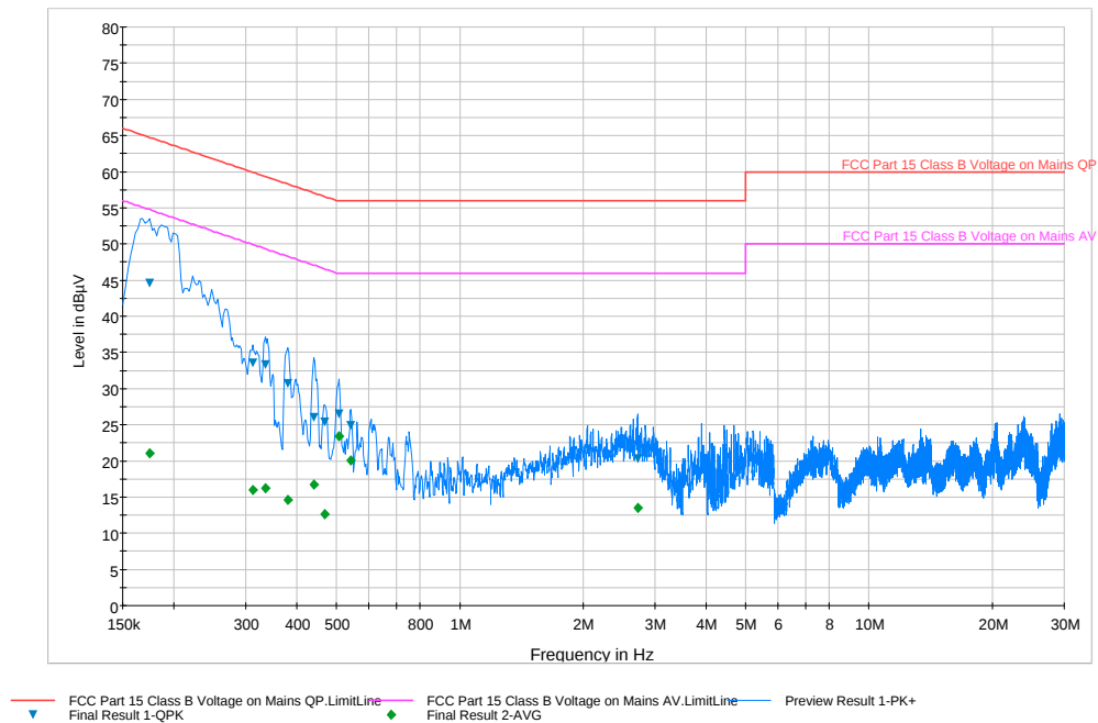
Plot 7-1. Line Conducted Plot (L1)
