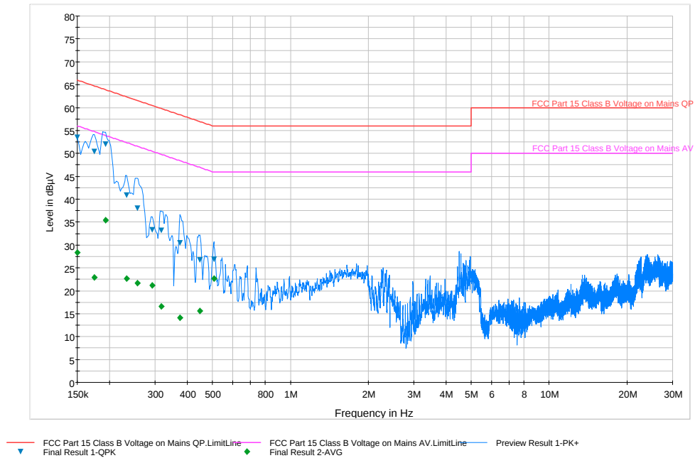
Plot 7-2. Line Conducted Plot (LN)
