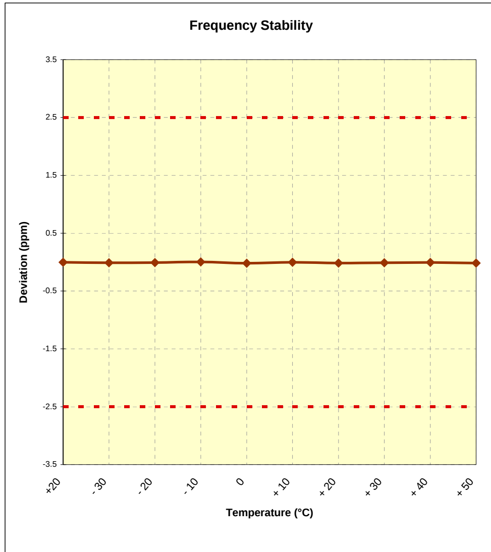
Figure 6-1. Frequency Stability Graph (Ch. 684)
