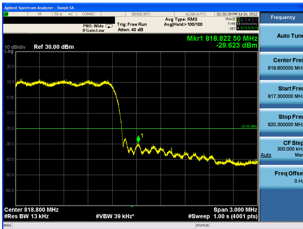
Plot 7-4. Interior Channel Edge Plot (Ch. 476)
