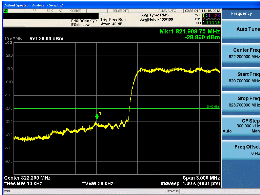
Plot 7-9. Interior Channel Edge Plot (Ch. 684)
