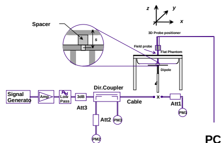
Figure 7.1 Dipole Validation Test Setup
