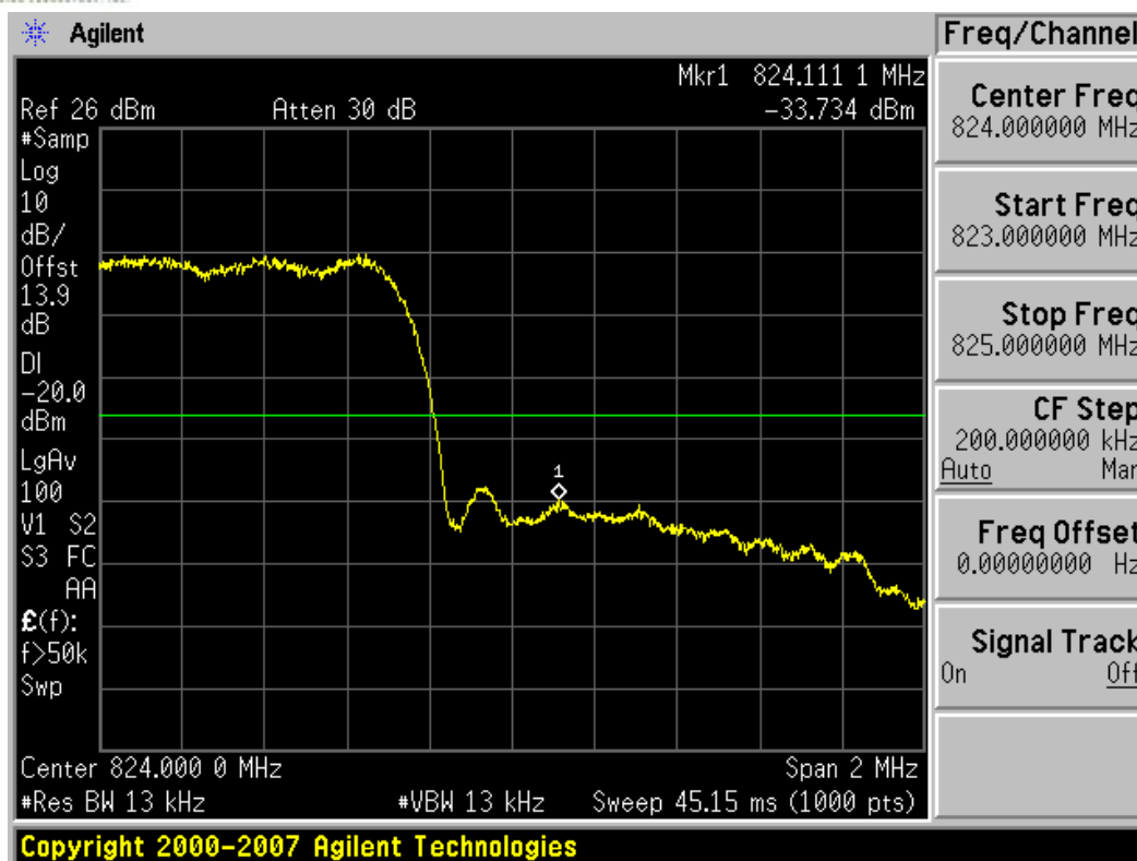
Plot 7-10. Channel Edge Plot (BC10 CDMA Ch. 684) - §90.691
