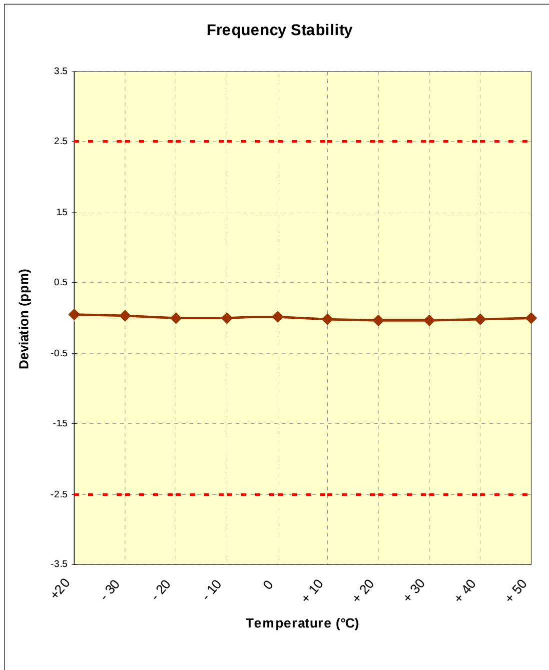
Figure 6-1. Frequency Stability Graph (BC10 CDMA Mode – Ch.684)
