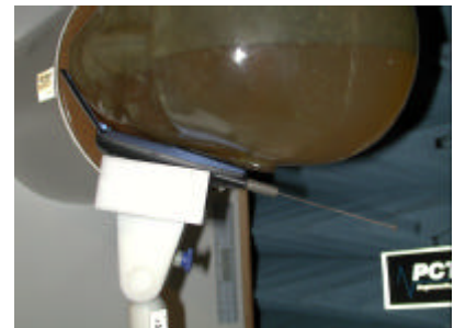
Figure 15. Head SAR Test Setup
