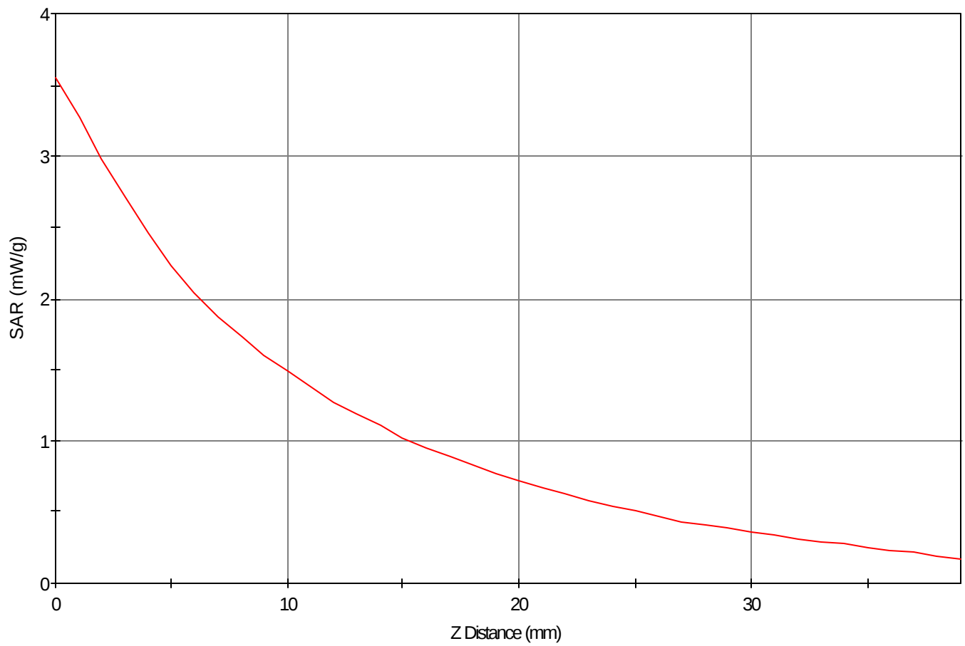
SAR - Z Axis at Hotspot x:1.0 y:-7.0
