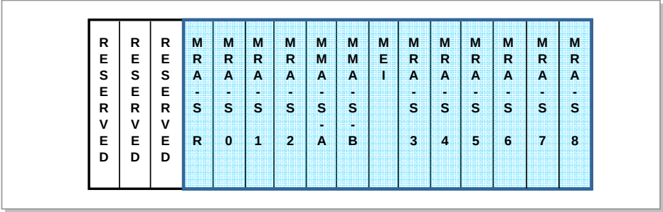
Figure 3.22 UFM Block
