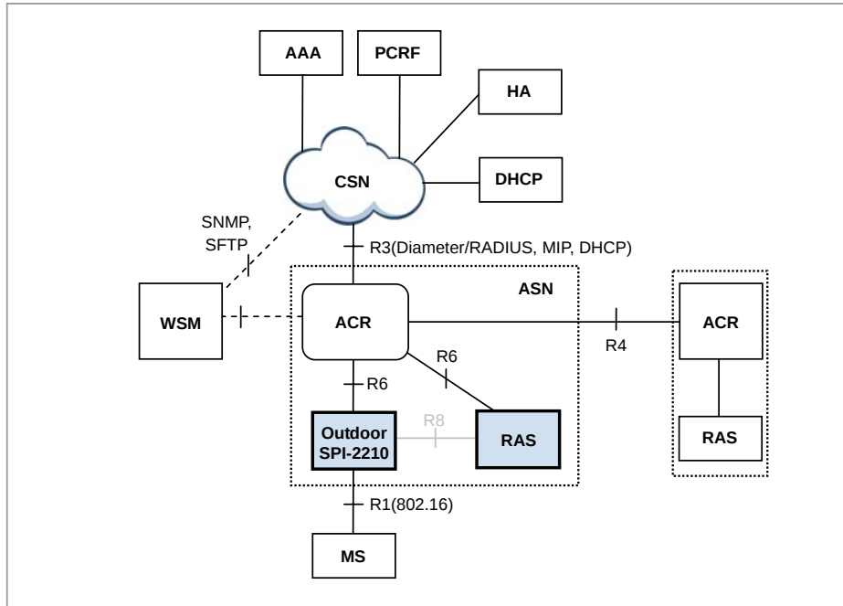
Figure 2.3 Structure of Outdoor SPI-2210 Interface
