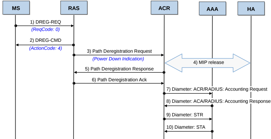
Figure 4.14 Access Termination (Awake Mode)
