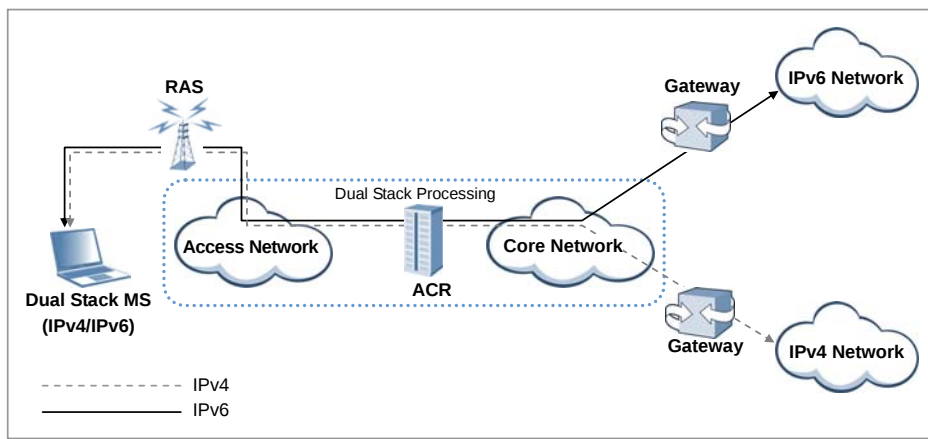
Figure 2.1 IPv4/IPv6 Dual Stack Operation
