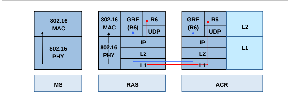
Figure 2.4 Protocol Stack between NEs
