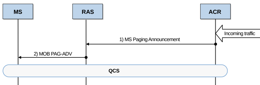
Figure 4.10 Paging Procedure
