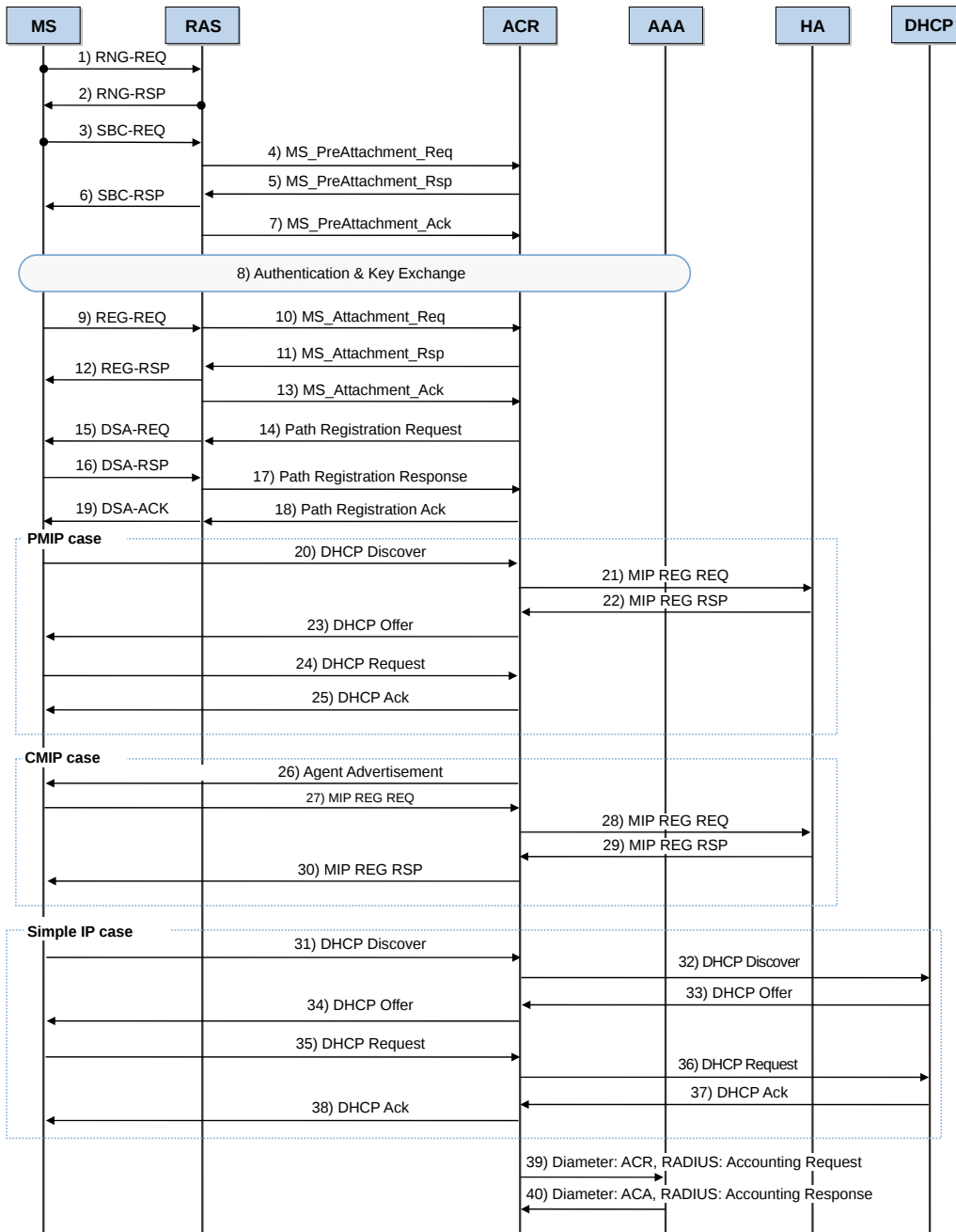
Figure 4.1 Initial Access Process
