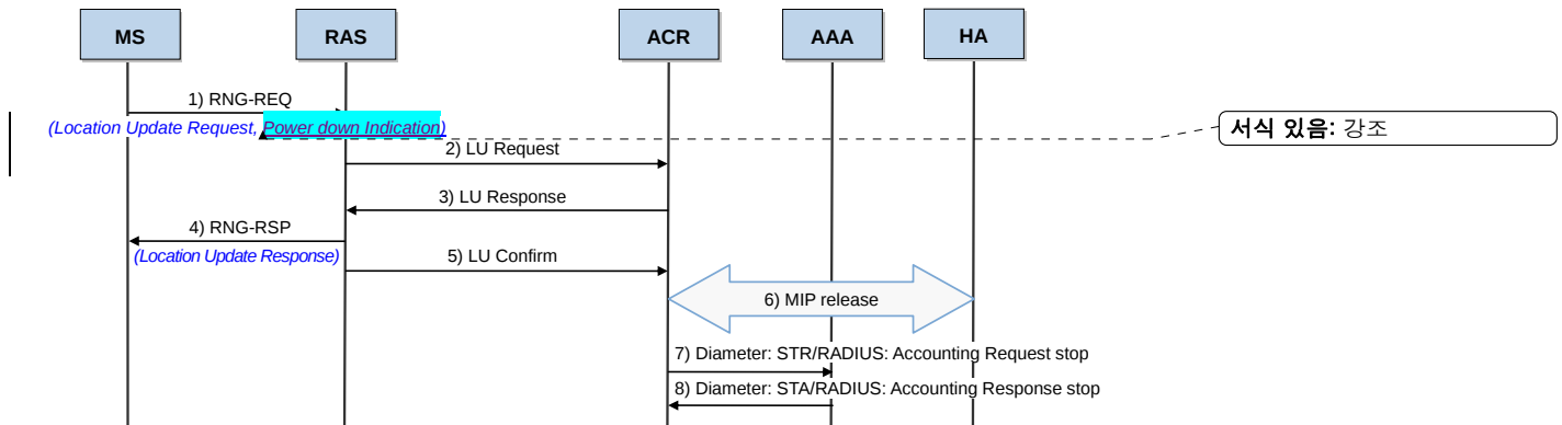
Figure 4.15 Access Termination (Idle Mode)
