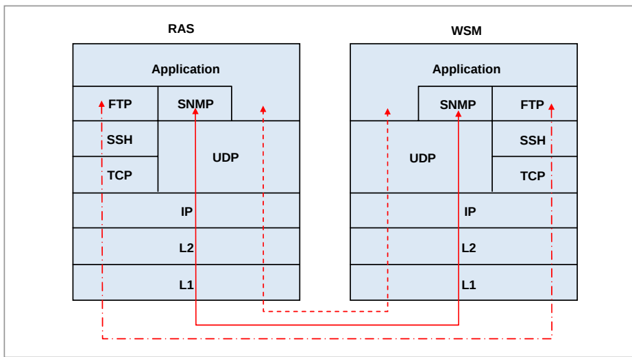
Figure 2.5 Protocol Stack between Outdoor SPI-2210 and WSM
