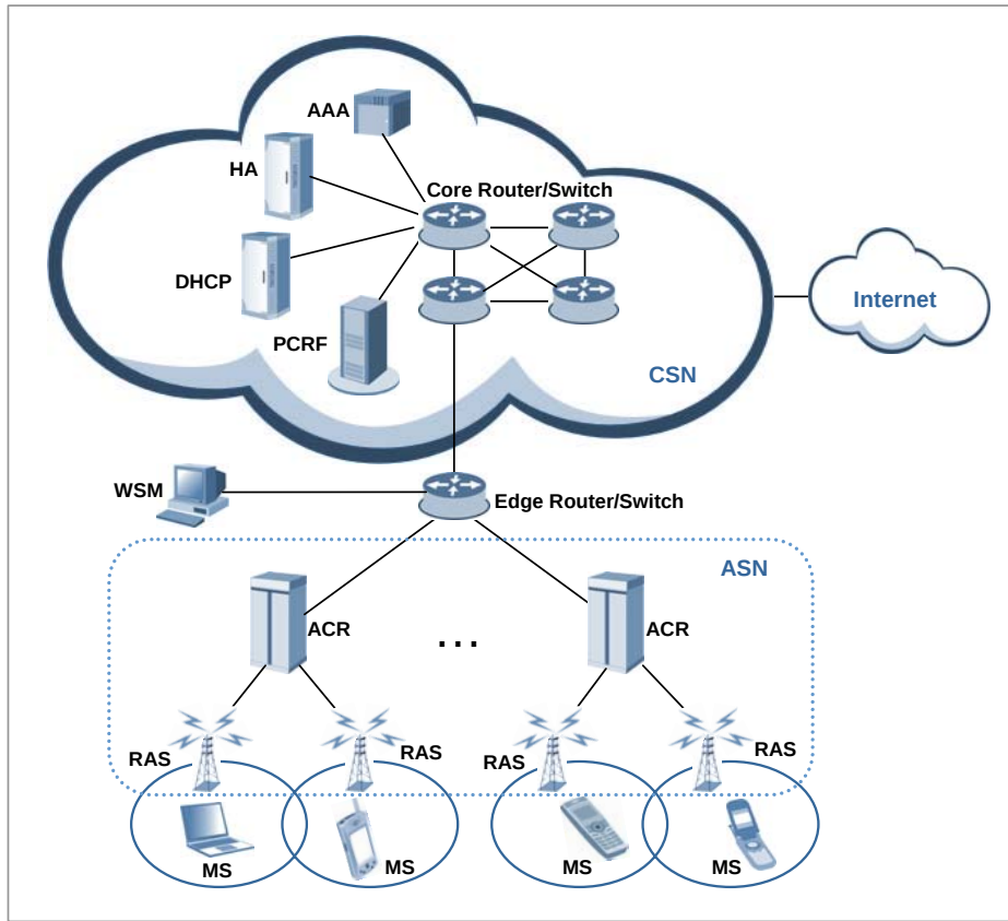
Figure 1.1 Mobile WiMAX Network Configuration
