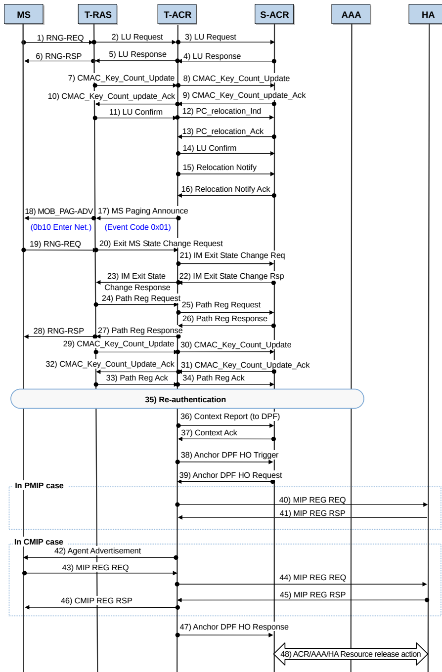
Figure 4.8 Inter-ACR Location Update Procedure (CMIP/PMIP Case)
