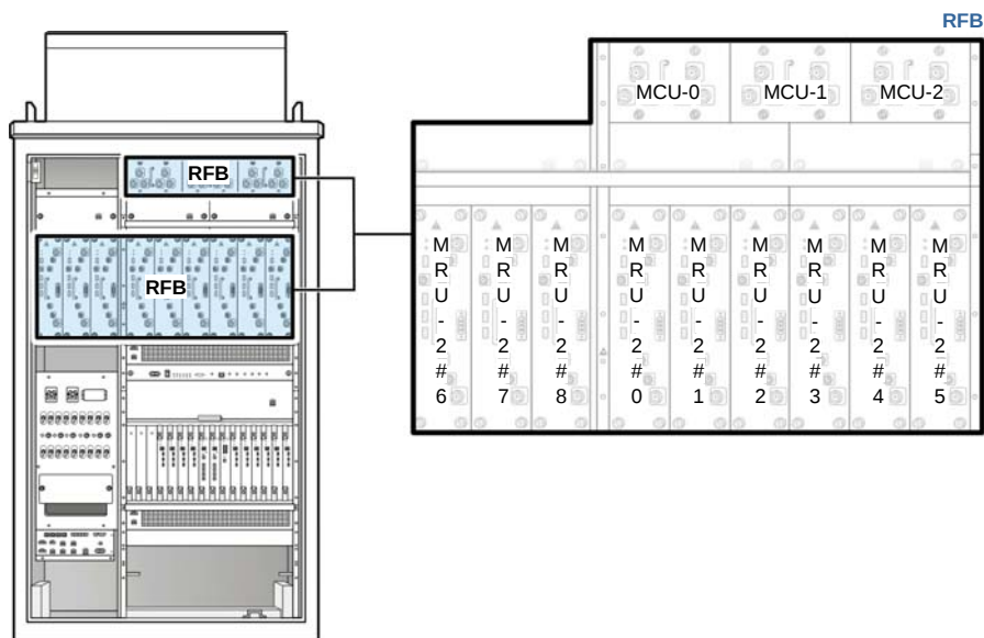
Figure 3.3 RFB Configuration
