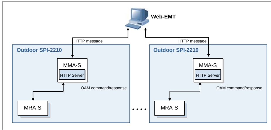
Figure 5.2 Web-EMT Interface
