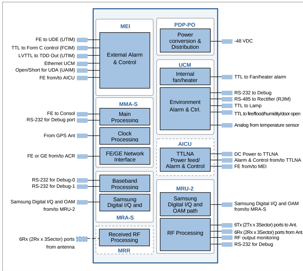
Figure 3.12 External Interfaces of Outdoor SPI-2210
