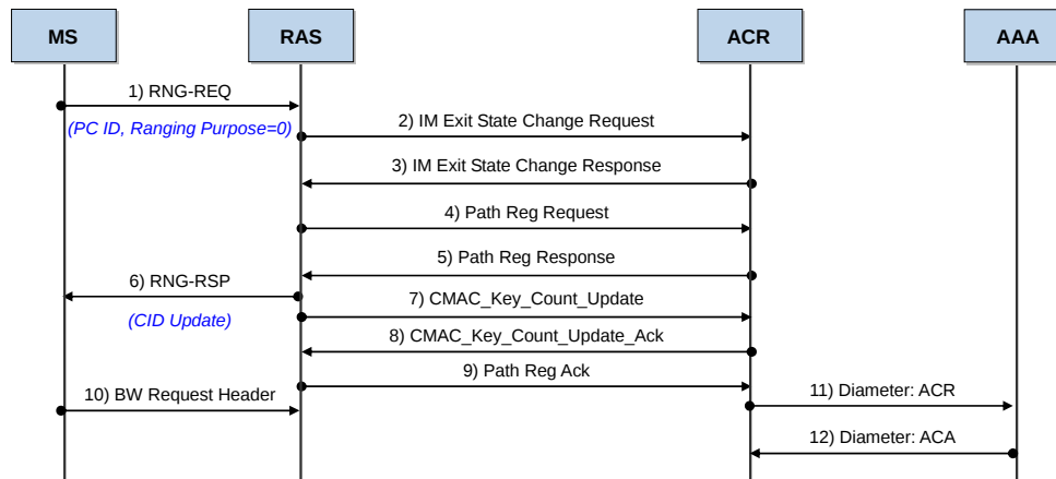
Figure 4.6 Idle Mode → Awake Mode (QCS) Procedure
