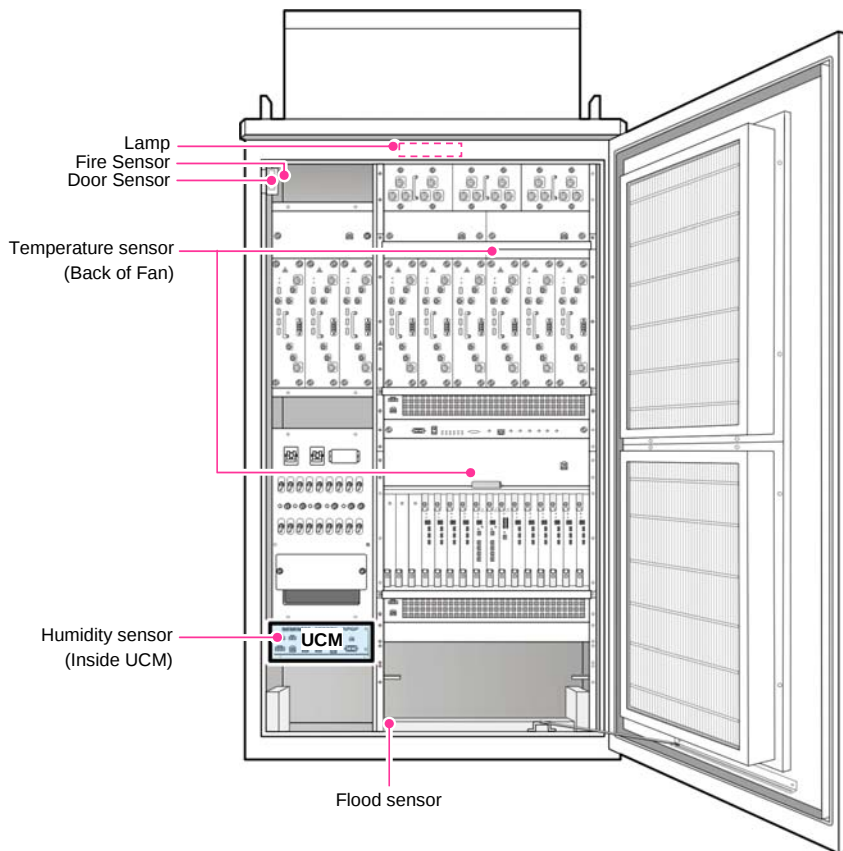
Figure 3.9 UCM and Sensor Configuration
