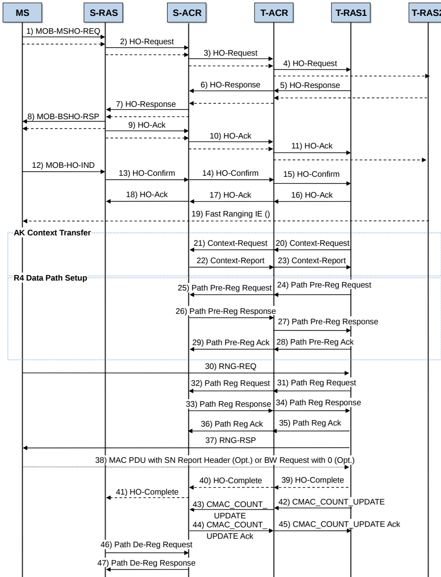
Figure 4.12 Inter-ASN Handover (ASN-Anchored Mobility)
