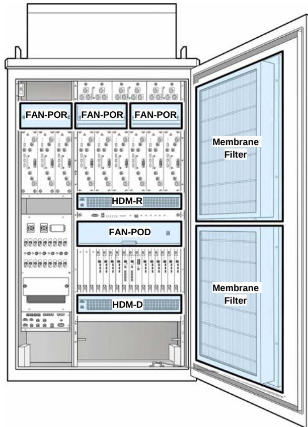
Figure 3.6 DACS Configuration
