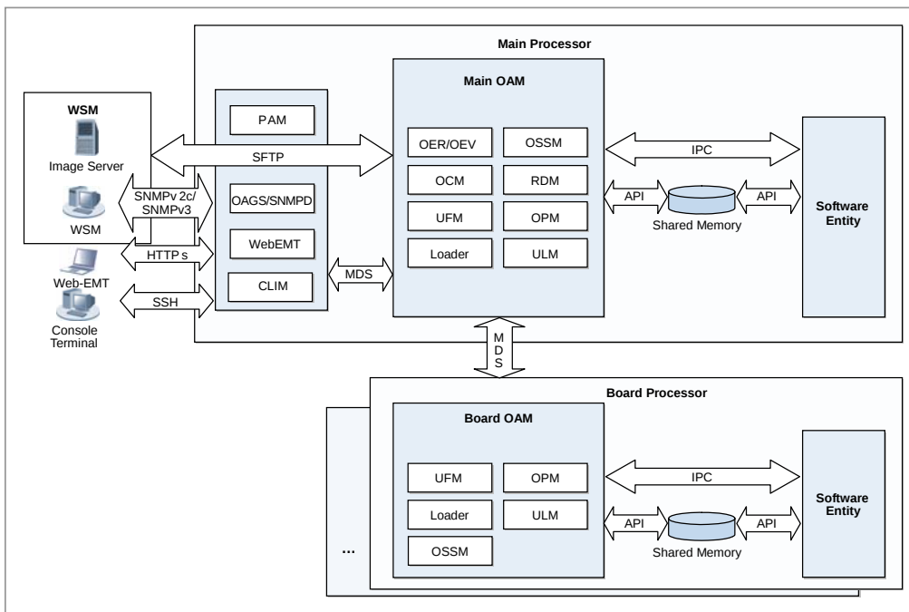
Figure 3.16 Interface between OAM Blocks
