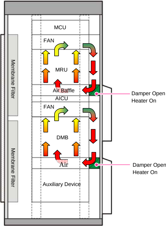
Figure 3.8 Heating Structure of the Outdoor SPI-2210
