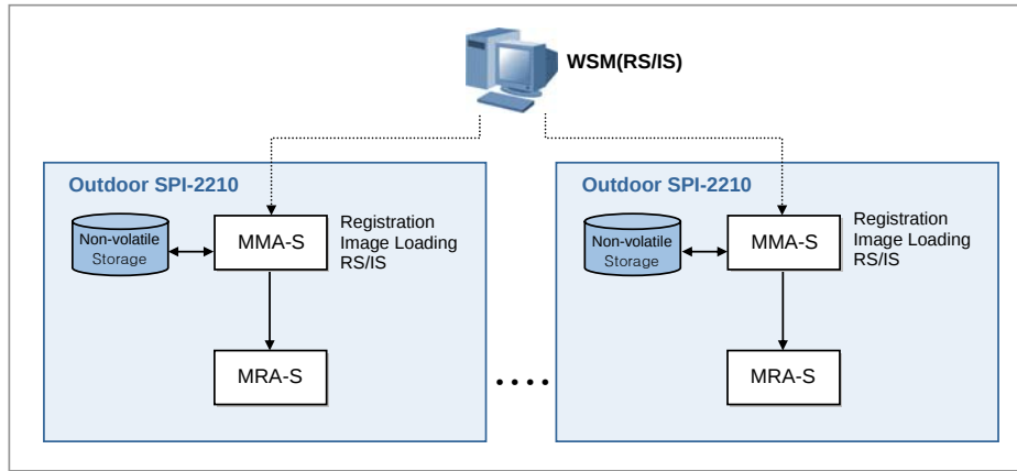
Figure 4.19 Loading Message Flow
