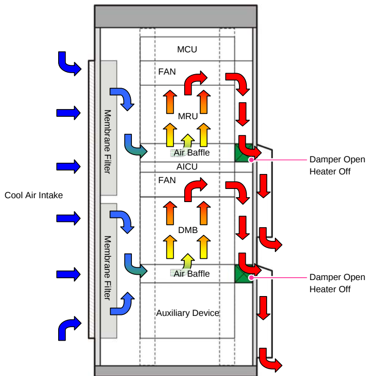
Figure 3.7 Heat Radiation Structure of the Outdoor SPI-2210
