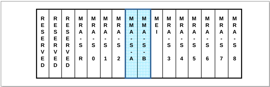
Figure 3.20 CLIM Block
