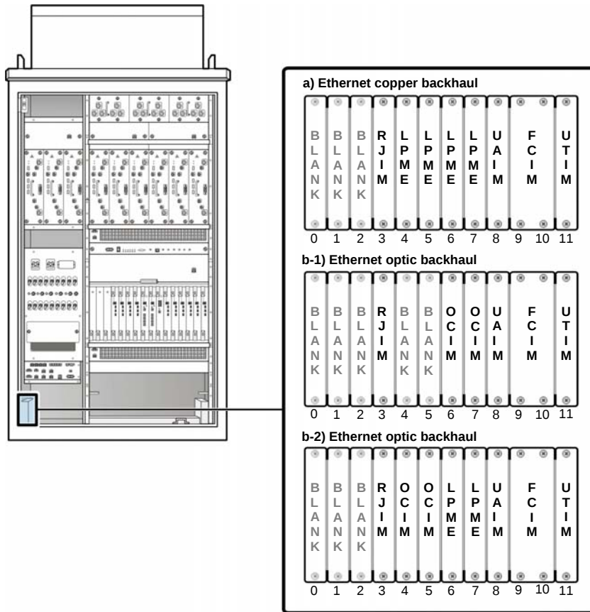
Figure 3.11 I/O Module Configuration
