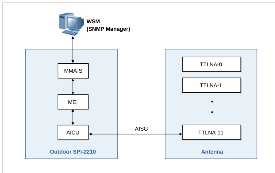
Figure 5.1 TTLNA/RET Interface
