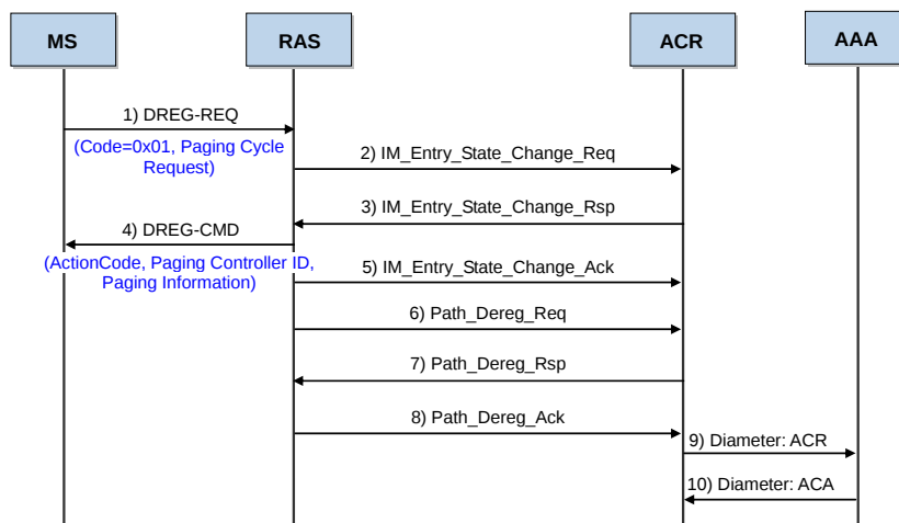
Figure 4.4 Awake Mode → Idle Mode Status Change Procedure
