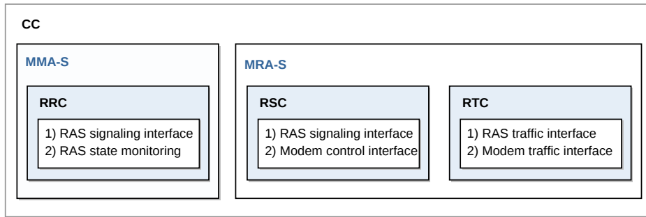
Figure 3.14 CC Block Structure
