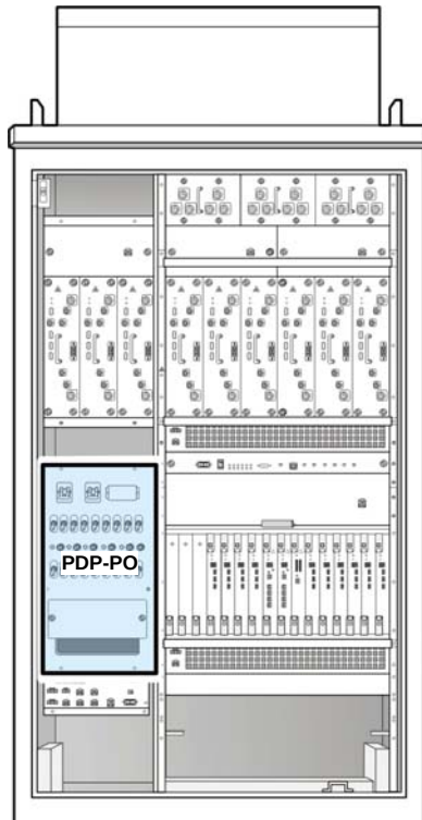
Figure 3.4 PDP-PO Configuration
