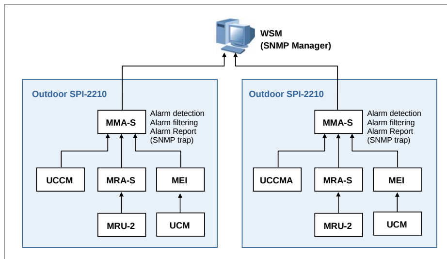
Figure 4.17 Alarm Signal Flow of Outdoor SPI-2210
