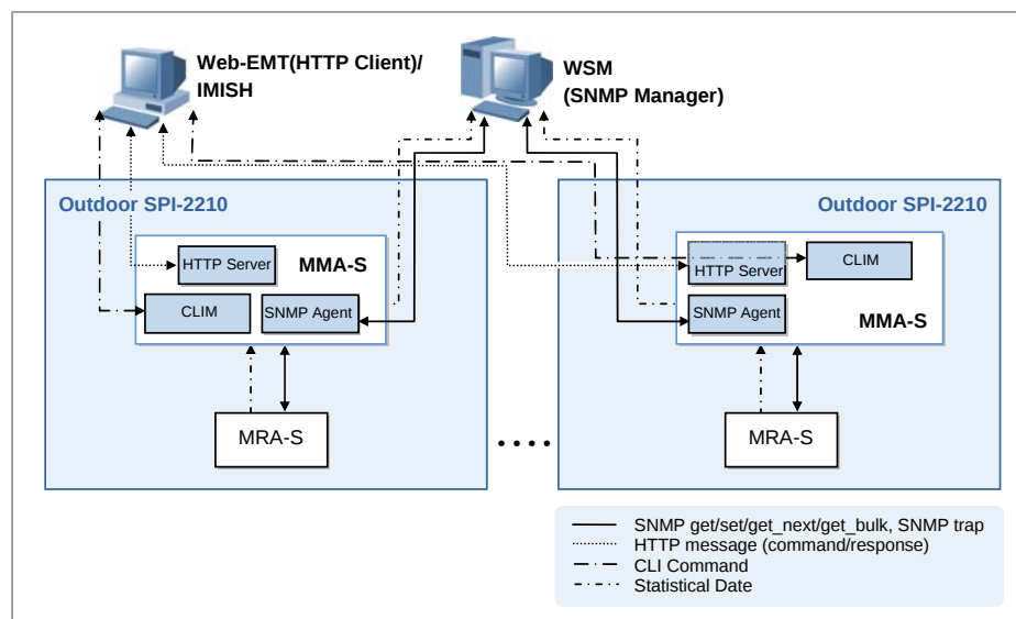
Figure 4.20 Operation and Maintenance Signal Flow
