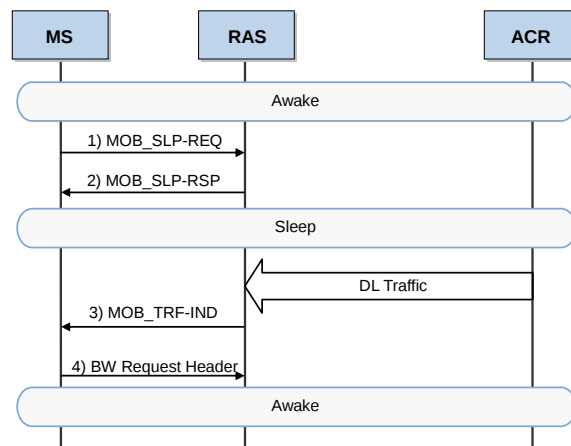
Figure 4.5 Awake Mode ↔ Sleep Mode Status Change Procedure
