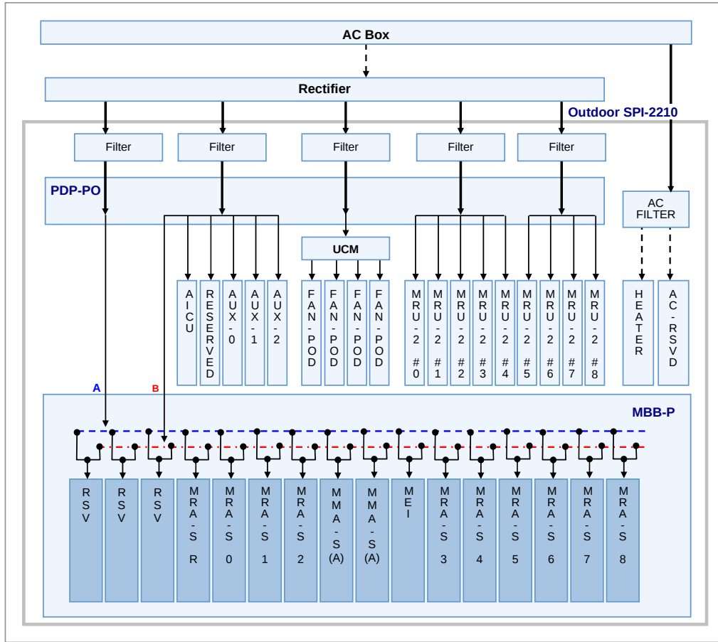
Figure 3.5 Power Structure
