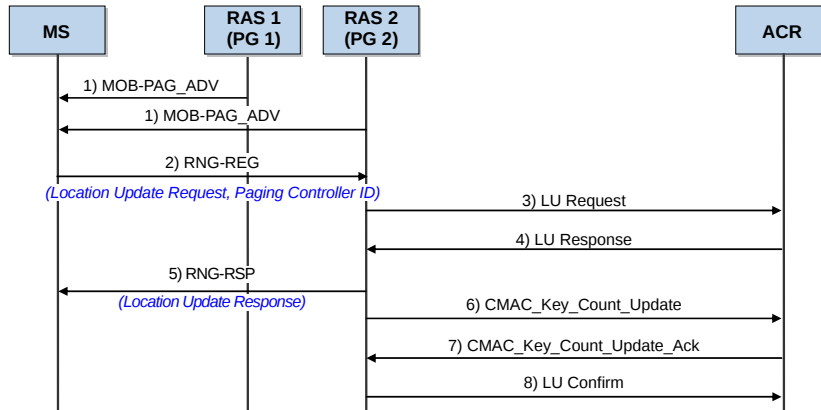
Figure 4.7 Inter-RAS Location Update Procedure
