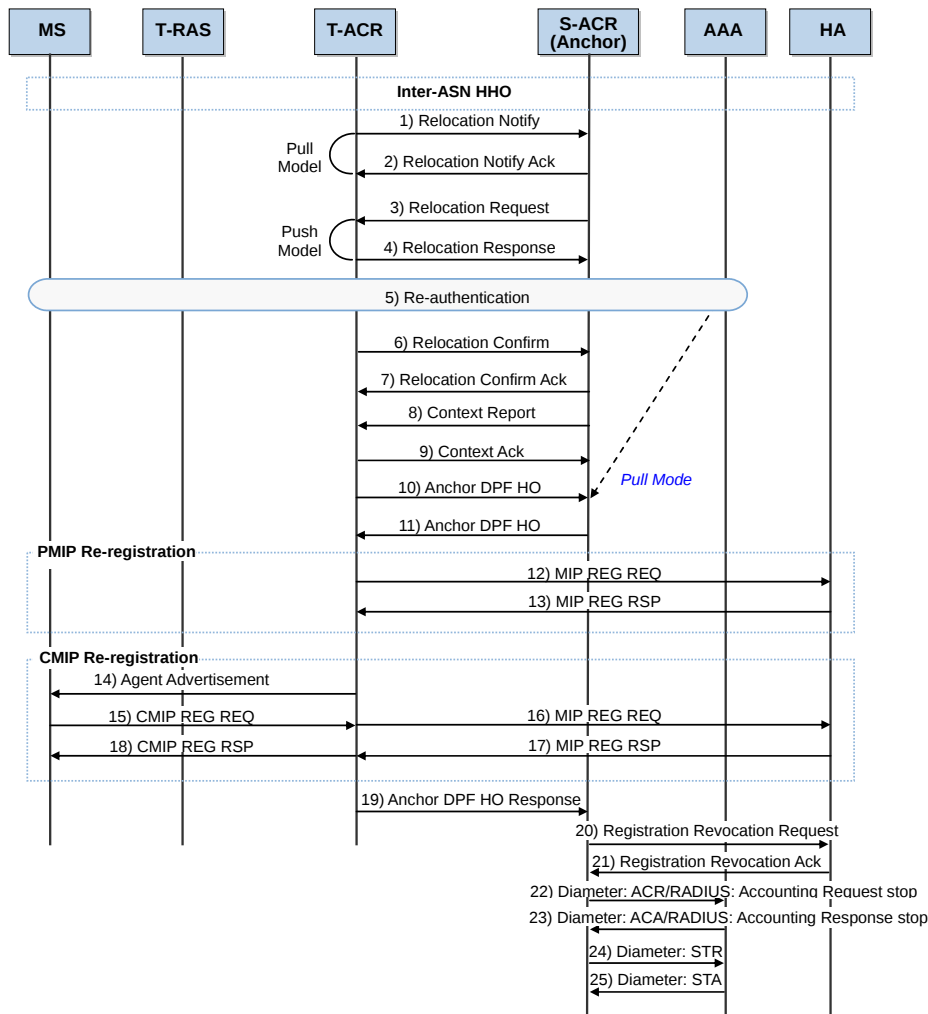
Figure 4.13 Inter-ASN Handover (CSN-Anchored Mobility)
