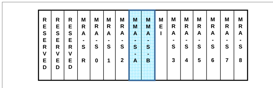
Figure 3.21 PAM Block
