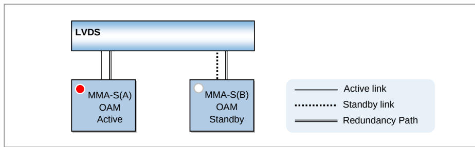
Figure 3.30 Redundancy Structure of OAM Block (MMA-S)
