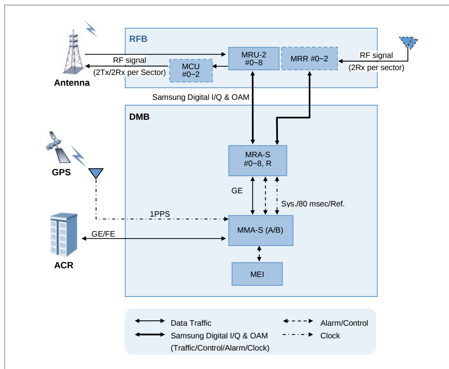
Figure 3.1 Internal Configuration of Outdoor SPI-2210
