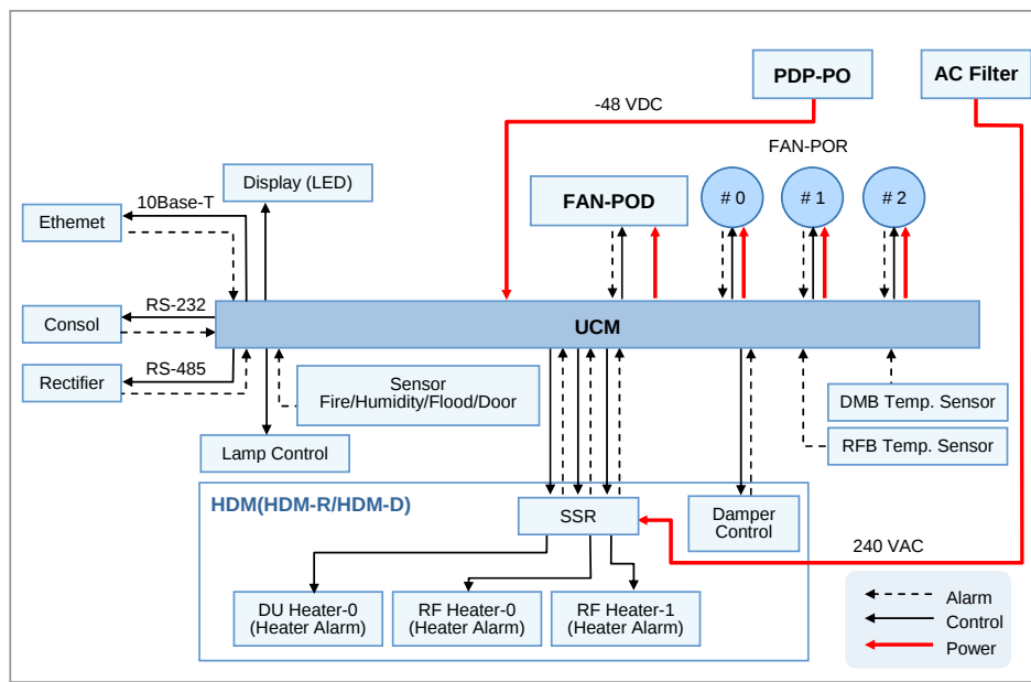
Figure 3.10 UCM Configuration Diagram of the Outdoor SPI-2210
