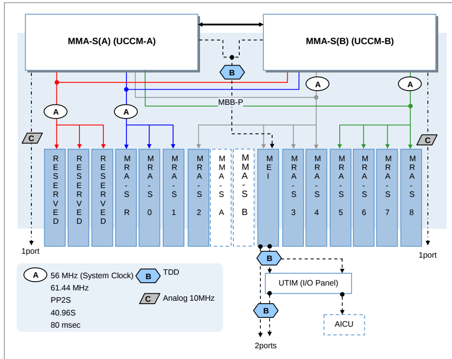
Figure 4.16 Network Synchronization Flow of Outdoor SPI-2210
