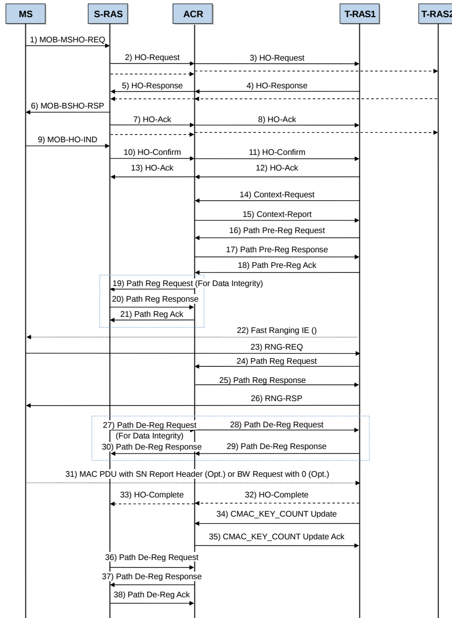
Figure 4.11 Inter-RAS Handover Procedure
