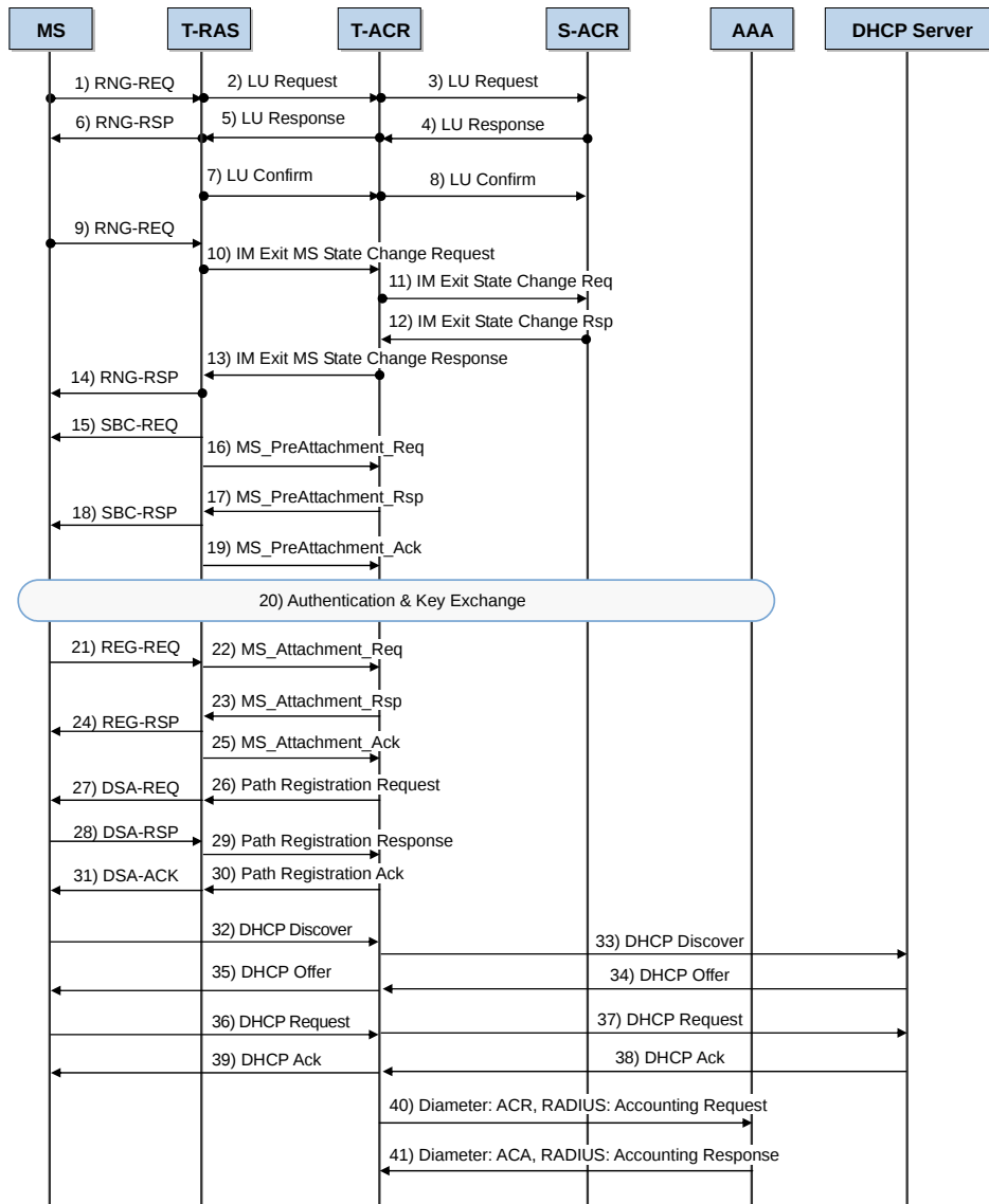
Figure 4.9 Inter-ACR Location Update Procedure (Simple IP Case)
