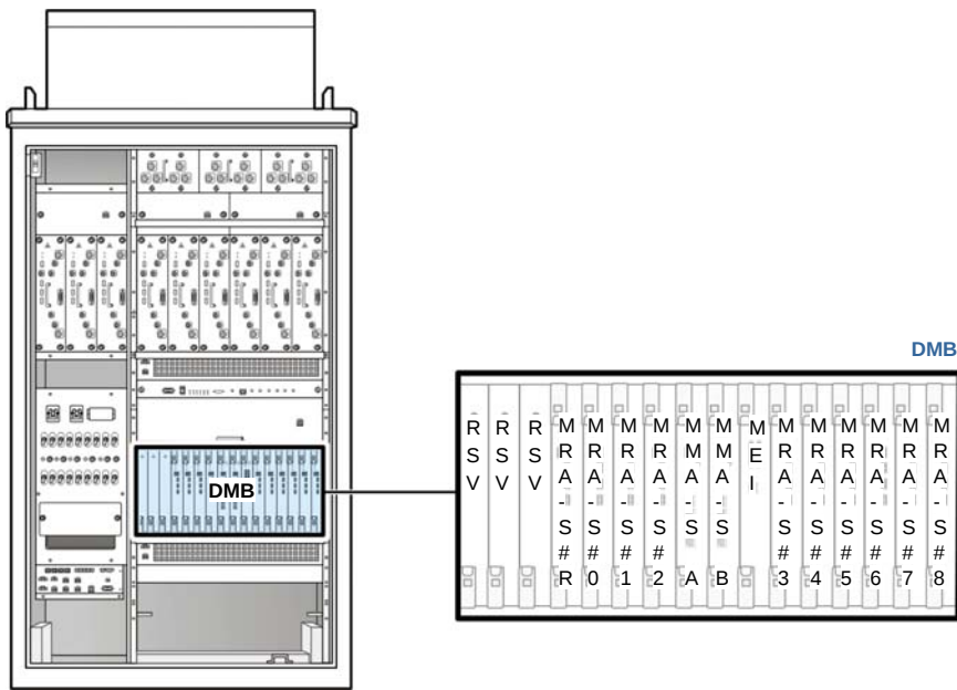
Figure 3.2 DMB Configuration
