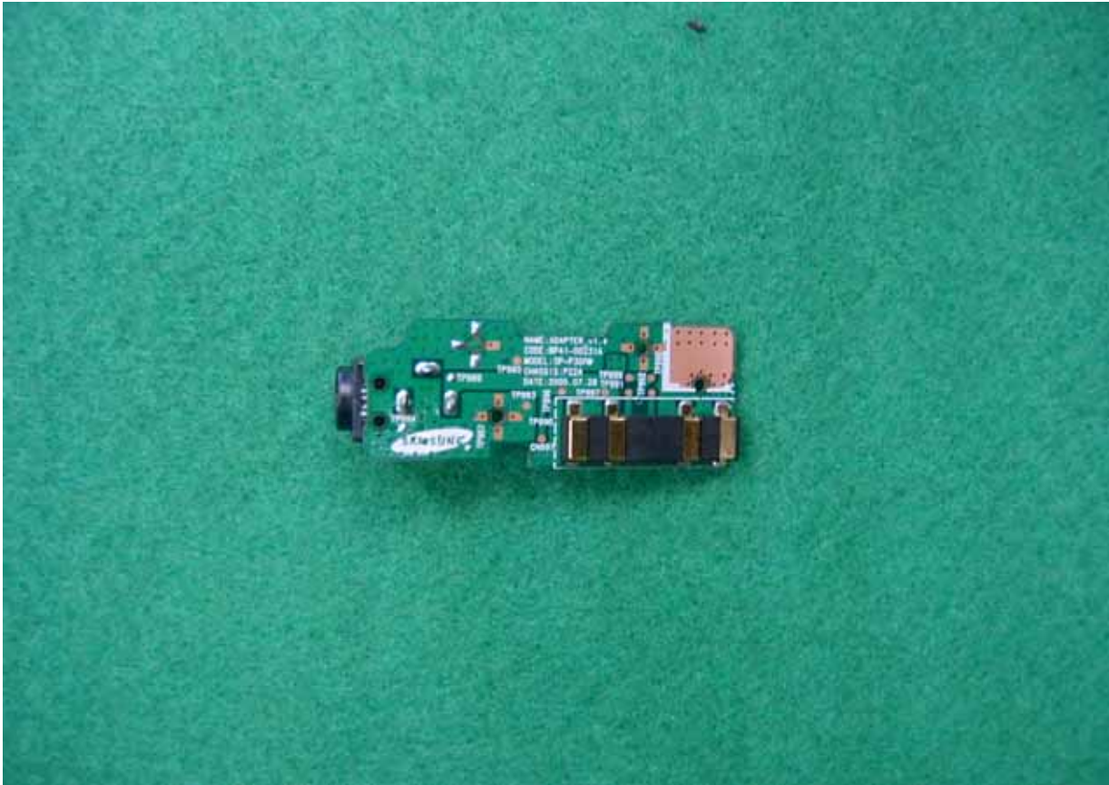
Adaptor board top view
