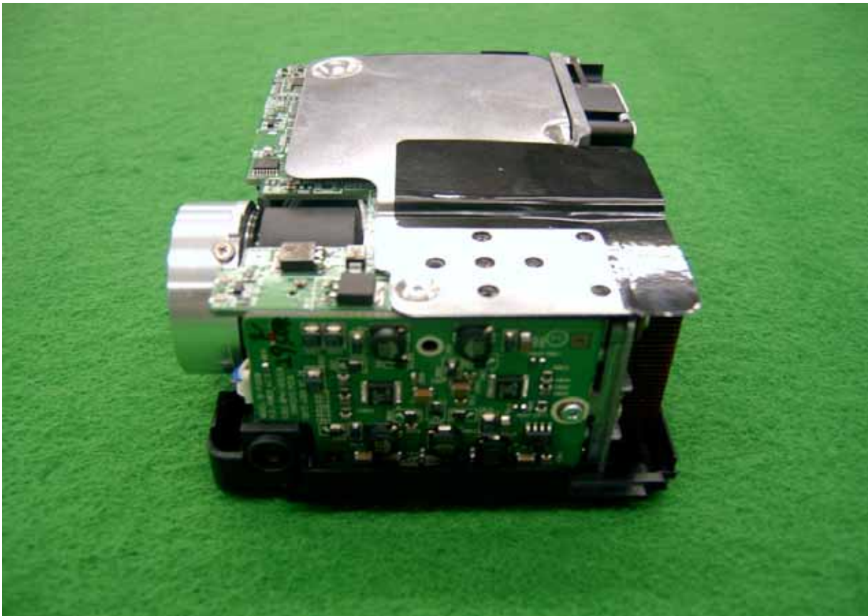
Engine view
