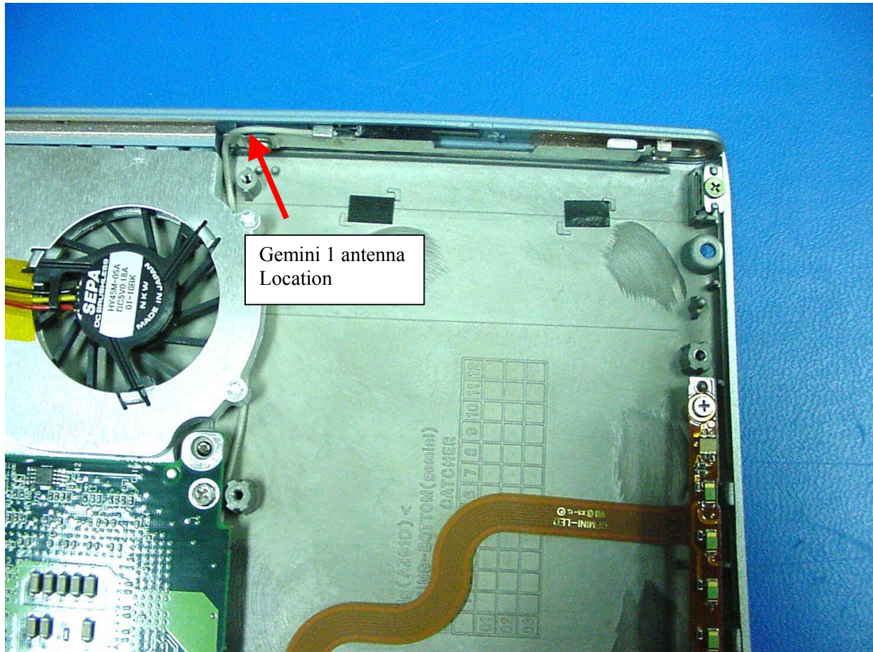
PHOTOGRAPH 12: LOCATION OF GEMINI 1 ANTENNA
