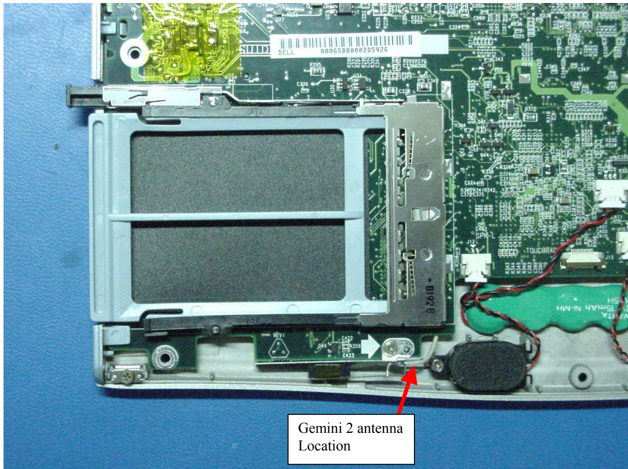
PHOTOGRAPH 9: LOCATION OF GEMINI 2 ANTENNA
