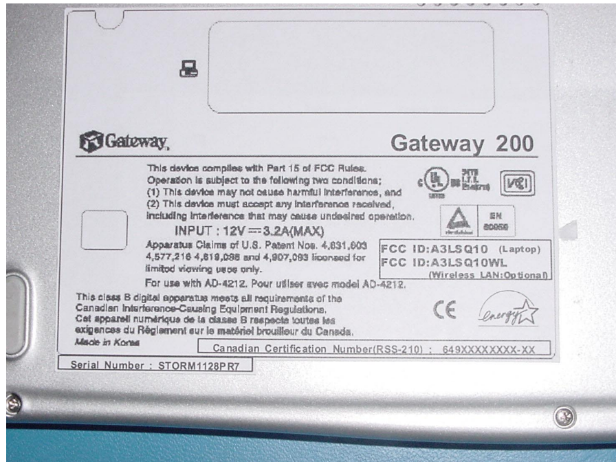
PHOTOGRAPH 1: IDENTIFICATION LABEL
