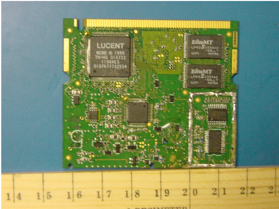
PHOTOGRAPH 16: EUT BOTTOM VIEW OF THE BOARD WITHOUT CAN
