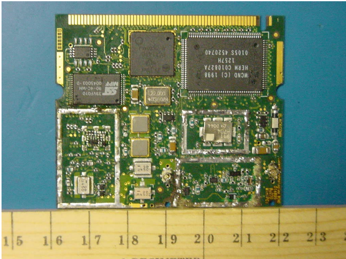
PHOTOGRAPH 15: EUT TOP VIEW OF THE BOARD WITHOUT CAN
