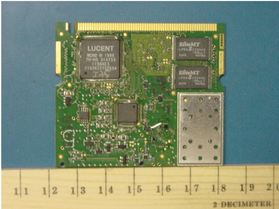
PHOTOGRAPH 14: EUT BOTTOM VIEW
