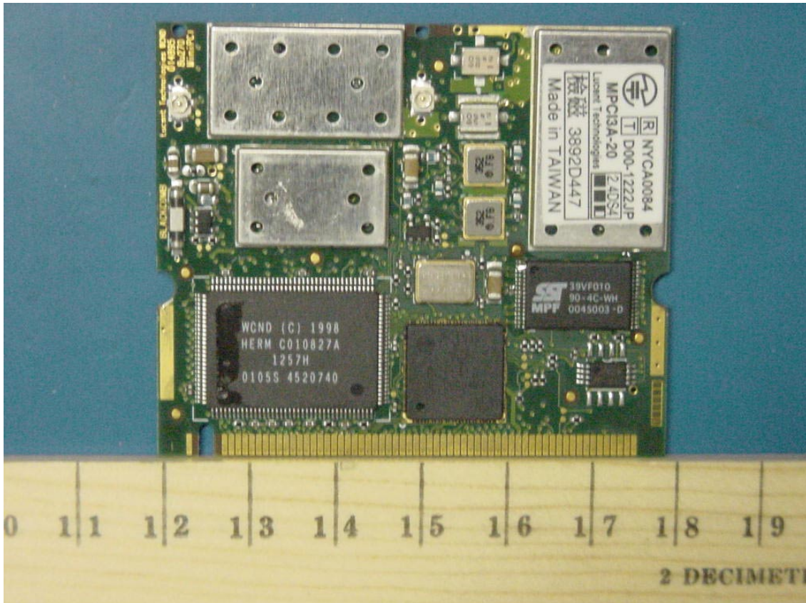
PHOTOGRAPH 13: EUT TOP VIEW
