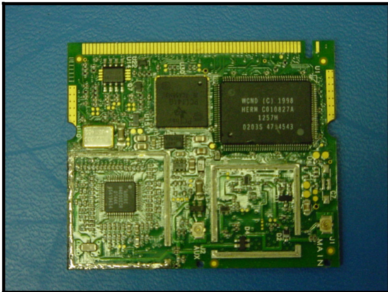
PHOTOGRAPH 15: EUT TOP VIEW OF THE BOARD WITHOUT SHIELD
