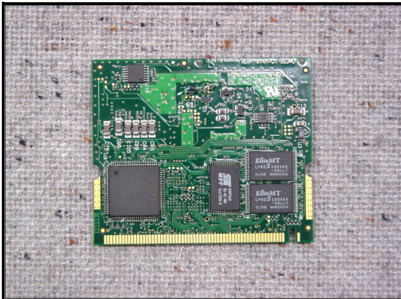
PHOTOGRAPH 14: EUT BOTTOM VIEW
