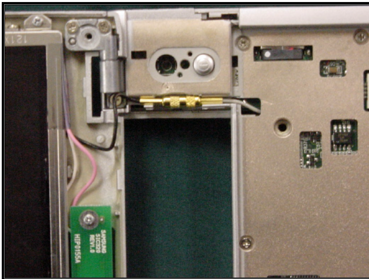
PHOTOGRAPH 16: EUT SHOWING RF CONNECTOR TO ANTENNA
