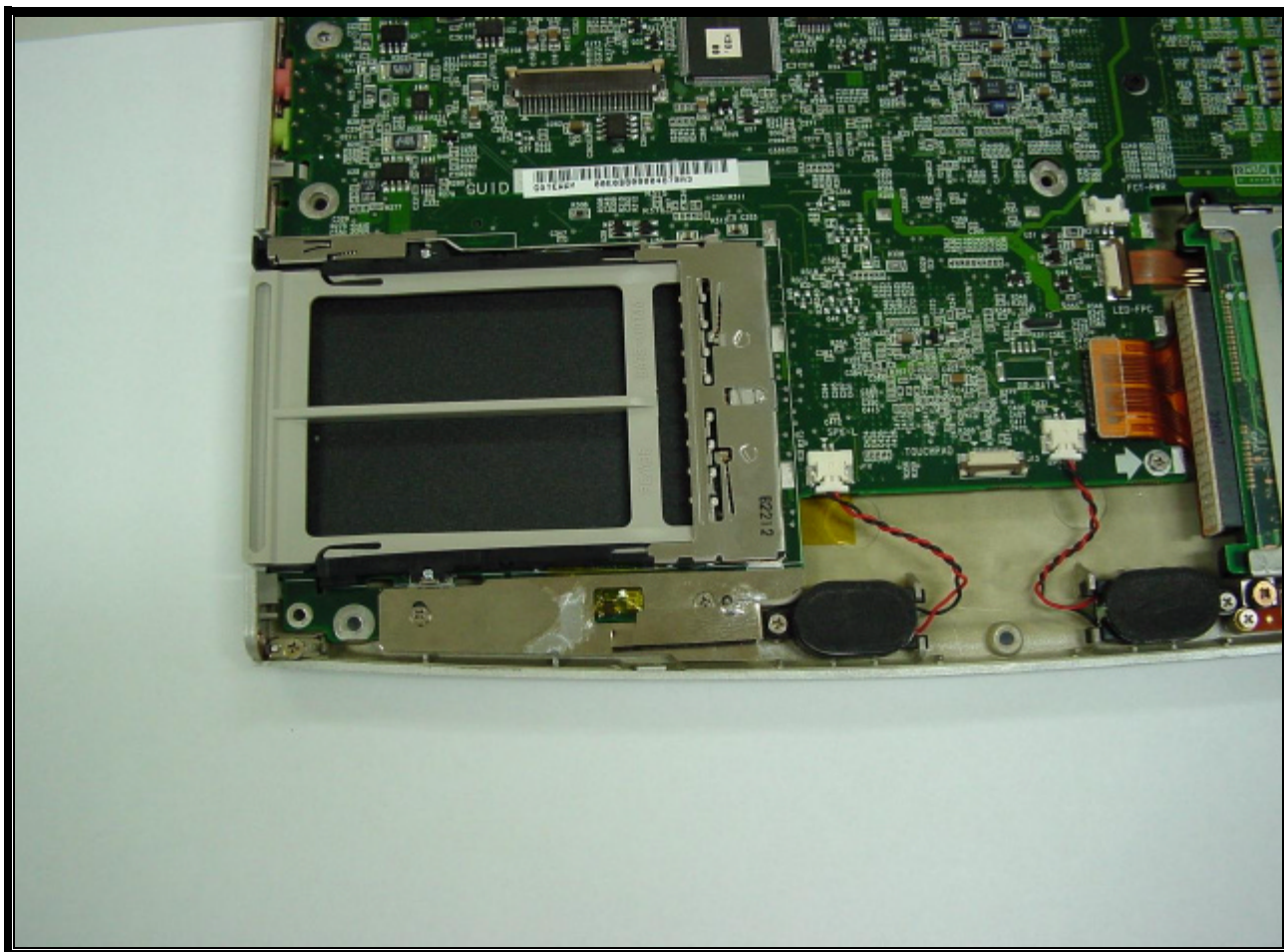
PHOTOGRAPH 11: LOCATION OF RECEIVING ANTENNA
