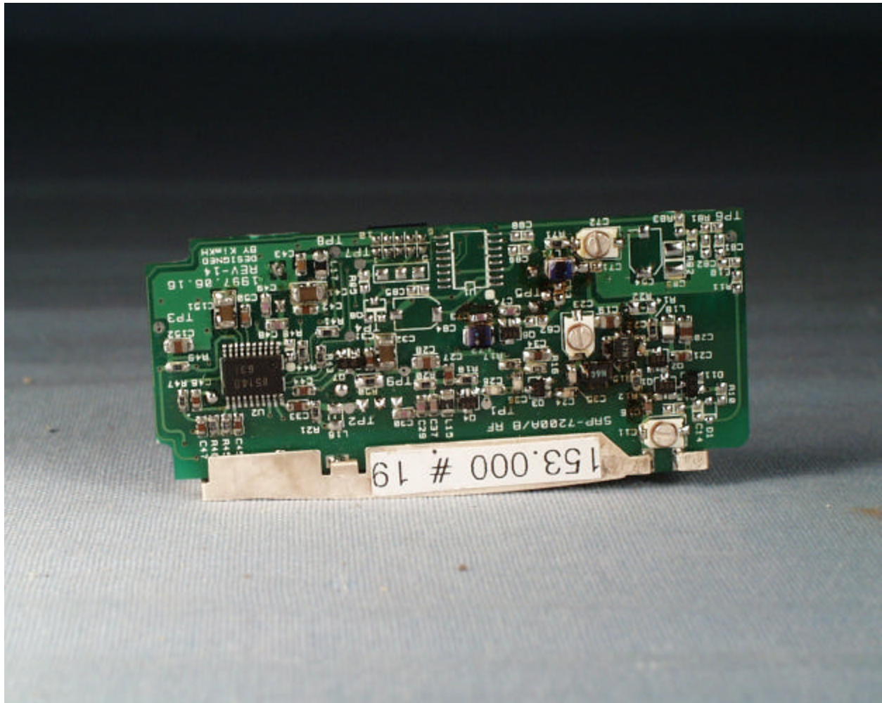
Side B (Digital Board)
