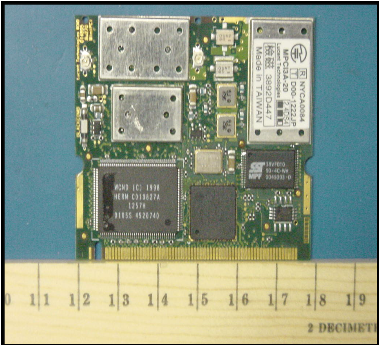
PHOTOGRAPH 9:EUT TOP VIEW
