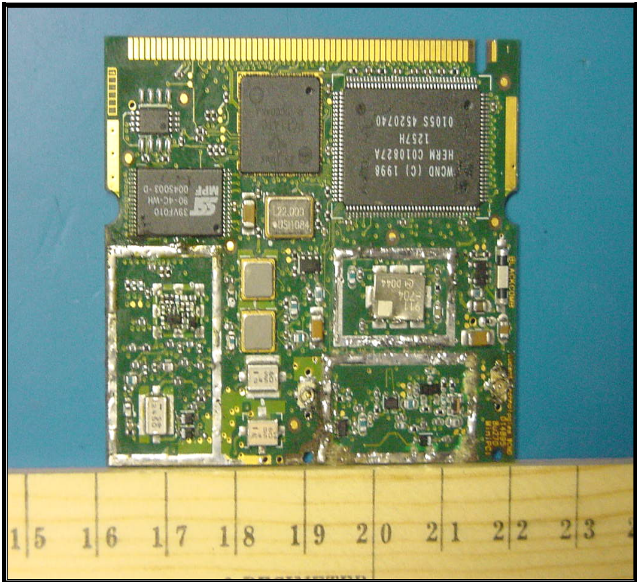
PHOTOGRAPH 11: EUT TOP VIEW OF THE BOARD WITHOUT CAN
