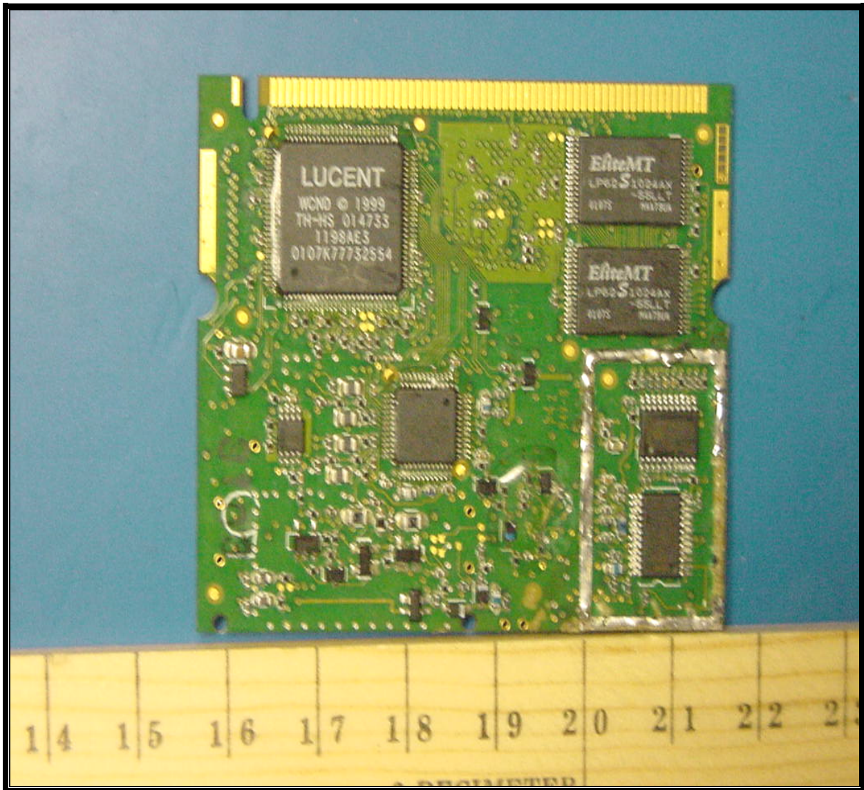
PHOTOGRAPH 12: EUT BOTTOM VIEW OF THE BOARD WITHOUT CAN
