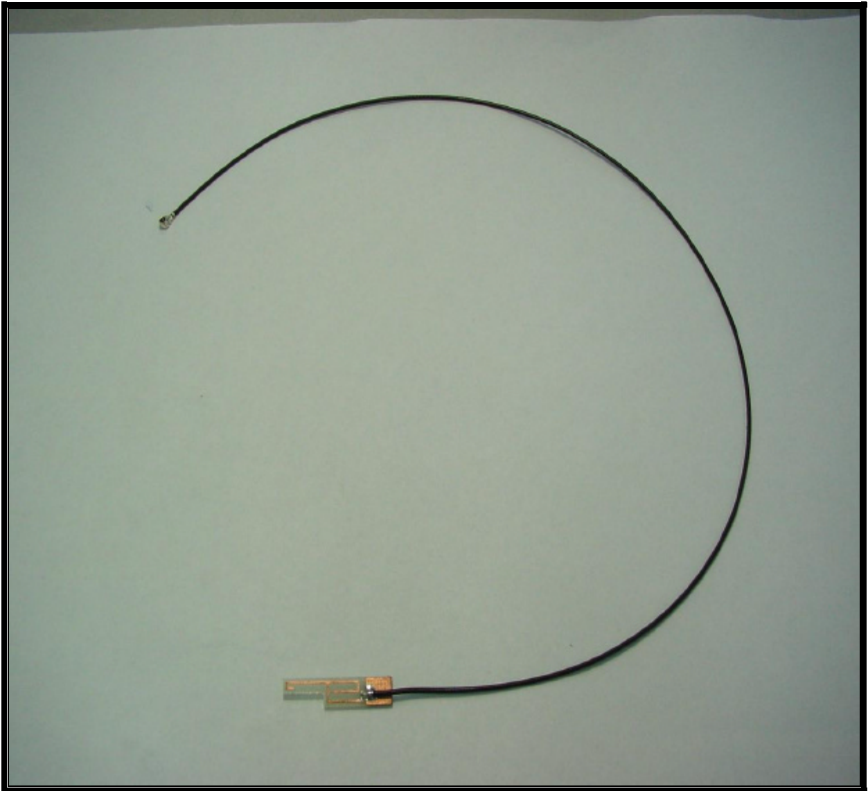
PHOTOGRAPH 5: MICROSTRIP RX ANTENNA
