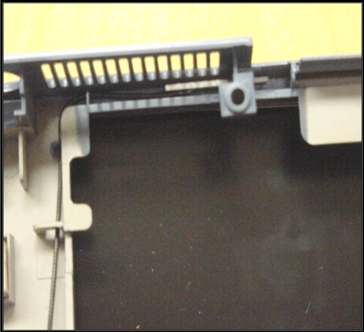
PHOTOGRAPH 7:AUX RX ANTENNA ( MICROSTRIP )
