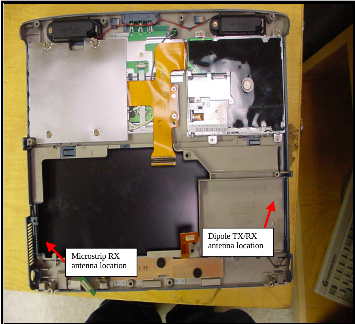
PHOTOGRAPH 6: LOCATION OF ANTENNAS INSIDE NOTEBOOK
