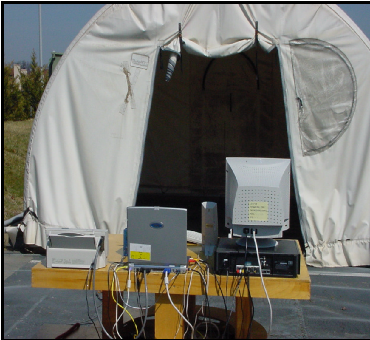
PHOTOGRAPH 3:RADIATED EMISSION REAR VIEW CASE CONFIGURATION
