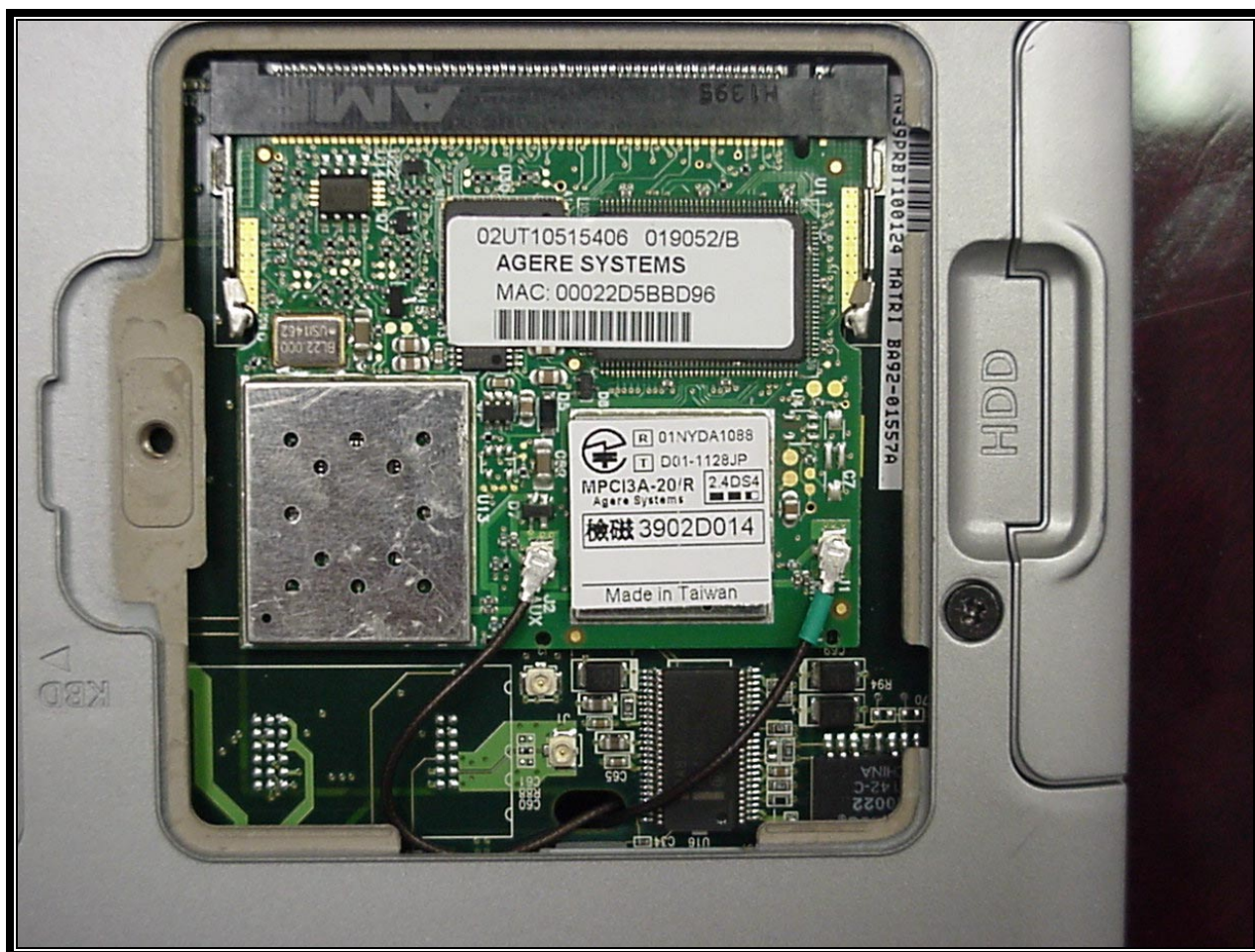
PHOTOGRAPH 9: EUT INSTALLED IN PC VIEW
