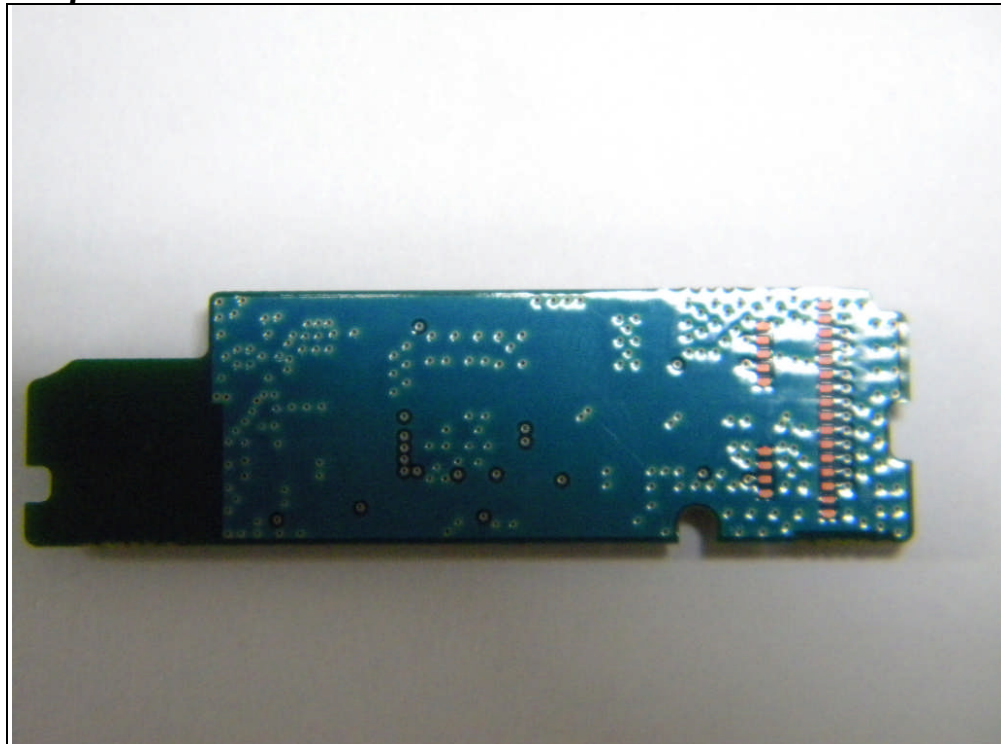
Bottom view of Wi-Fi module PCB
