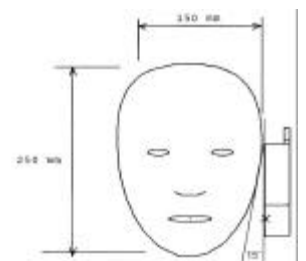
Figure 14. Ear/15° Tilt Position
