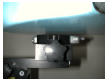
Figure 26. Body SAR Test Setup
