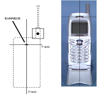
Figure 11. Ear Reference Point
