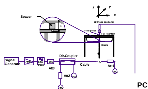
Figure 7.1 Dipole Validation Test Setup
