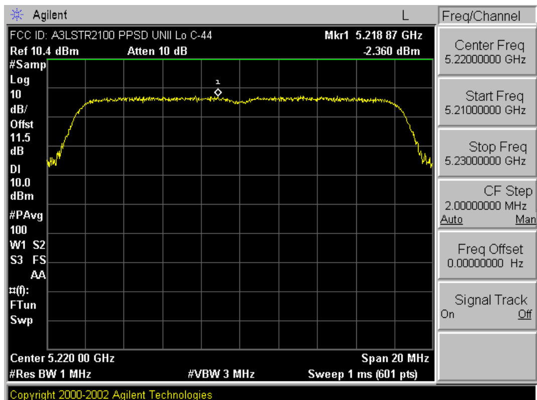
Plot 6-9. Peak Power Spectral Density Plot [Industry Canada] (802.11a (UNII) – Ch. 44)
