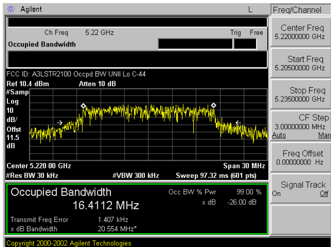
Plot 6-3. 26dB Bandwidth Plot (802.11a (UNII) – Ch. 44)
