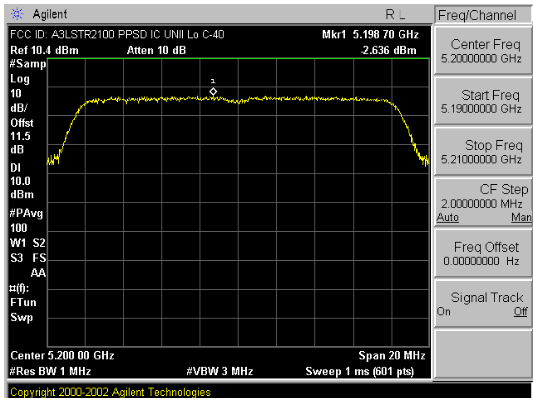
Plot 6-7. Peak Power Spectral Density Plot [Industry Canada] (802.11a (UNII) – Ch. 40)
