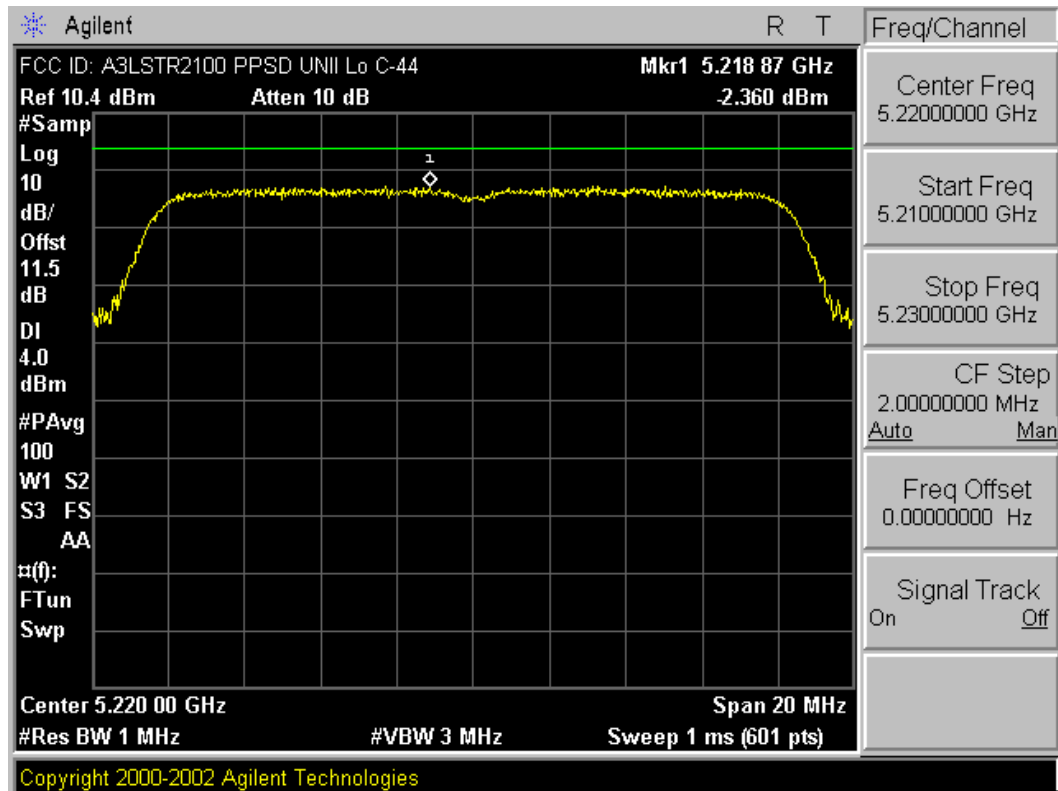
Plot 6-8. Peak Power Spectral Density Plot (802.11a (UNII) – Ch. 44)
