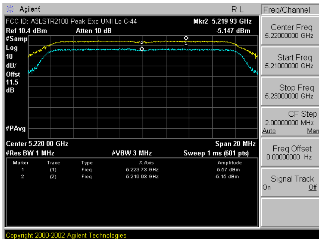
Plot 6-12. Peak Excursion Ratio Plot (802.11a (UNII) – Ch. 44)
