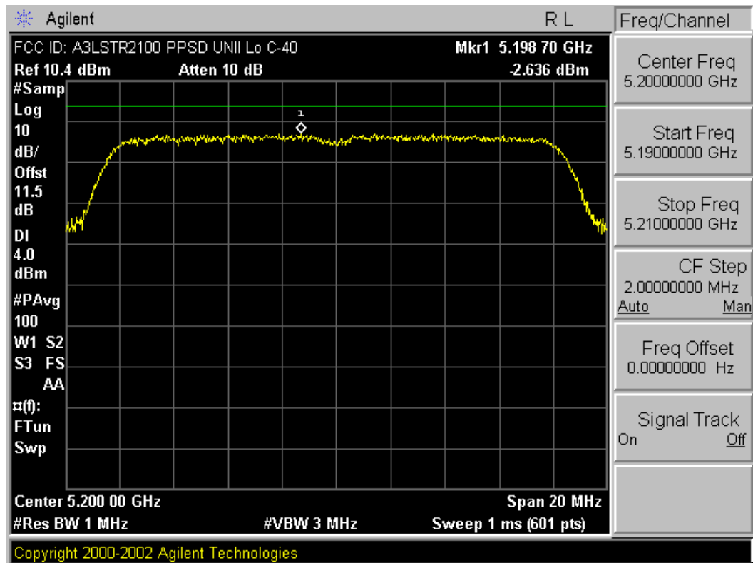
Plot 6-6. Peak Power Spectral Density Plot (802.11a (UNII) – Ch. 40)
