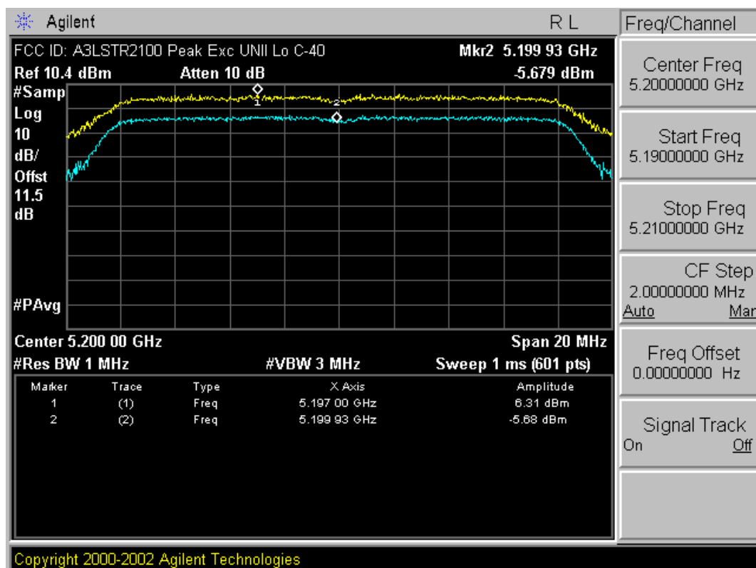
Plot 6-11. Peak Excursion Ratio Plot (802.11a (UNII) – Ch. 40)
